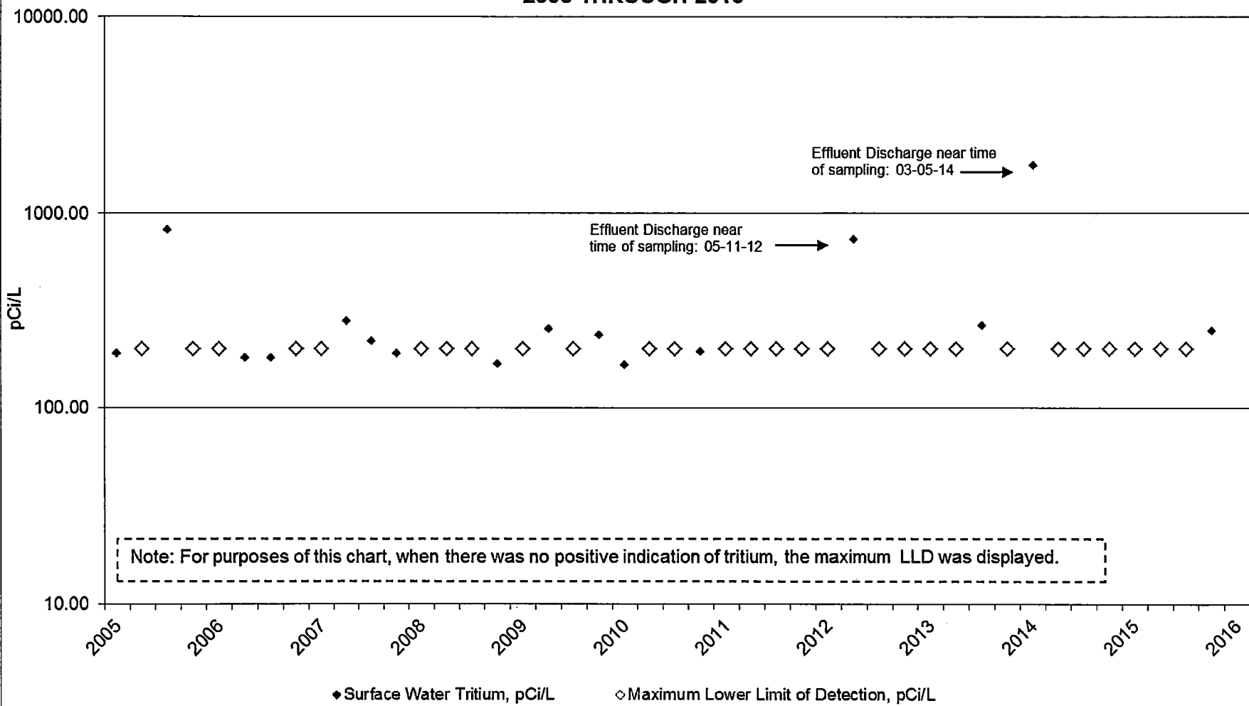
FIGURE 3 TRITIUM ACTIVITY IN SURFACE WATER - QUARTERLY AVERAGE 2005 THROUGH 2015
