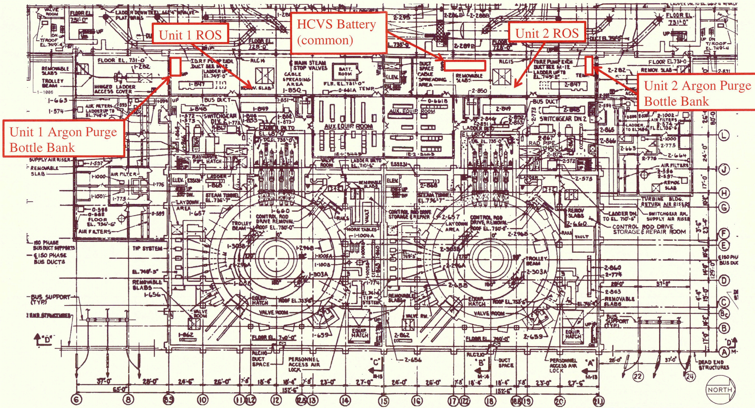
Sketch 2C: Remote Operating Station
