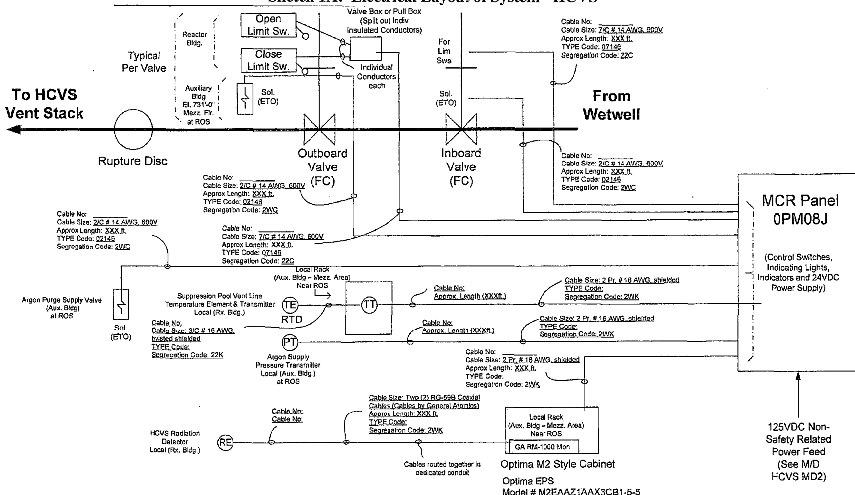
Sketch 1A: Electrical Layout of System - HCVS
