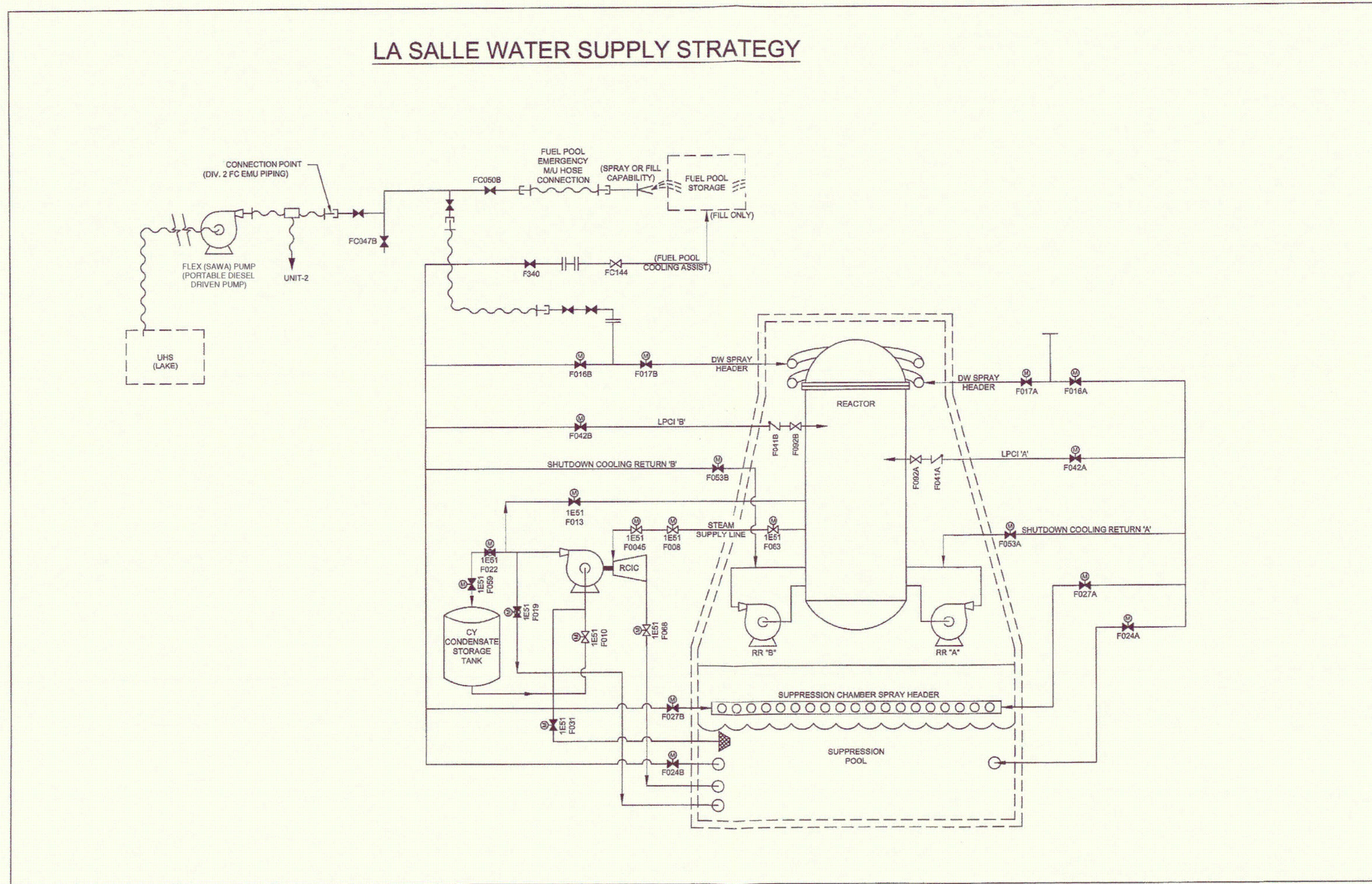
Sketch 3A: P&ID Layout of SAWA (Note - Same as FLEX)
