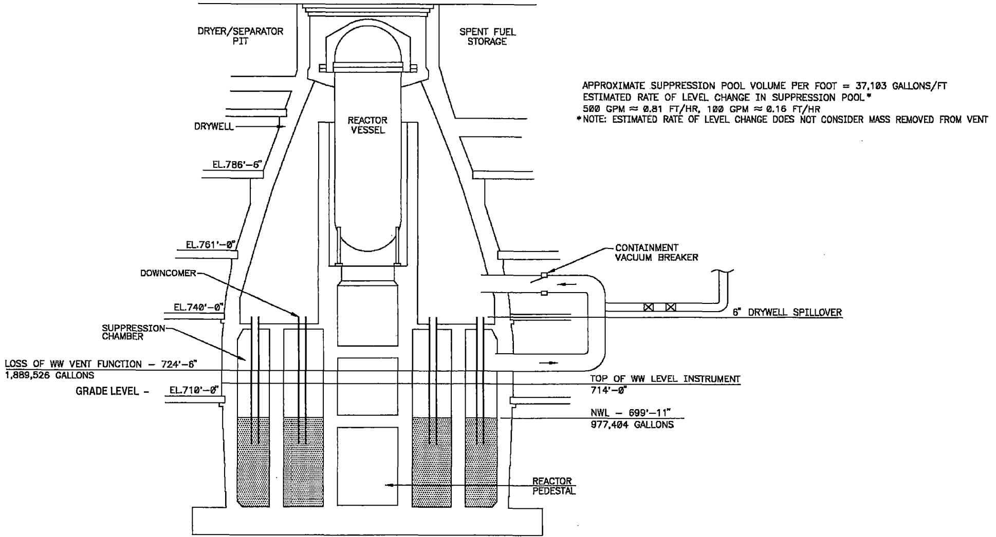
LASALLE PRIMARY CONTAINMENT OUTLINE
