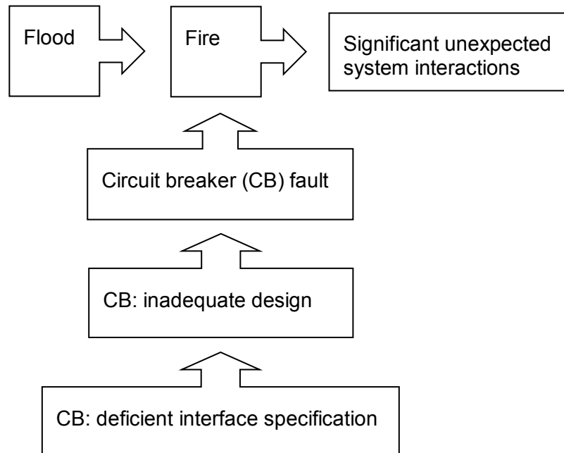
Figure 13: Example from event on June 7, 2011, at Ft Calhoun nuclear power plant (NPP).
