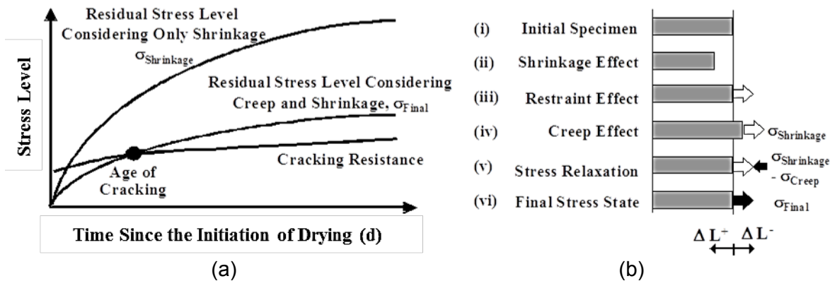
Figure 5- (a) Stress development and (b) conceptual description of relaxation (after Weiss 1999).
