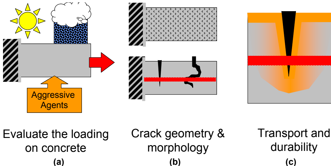
Figure 10- A schematic of how crack formation can influence transport processes in concrete: a) environmental causes of cracking, b) distributed (micro-cracks) and coalesced cracks, and c) pathways for both ingress and egress of moisture, gases, and dissolved species.
