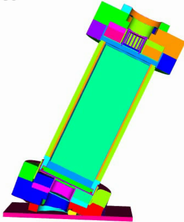
Figure C-8 Rail-Steel cask corner impact at 48 kph (30 mph)
