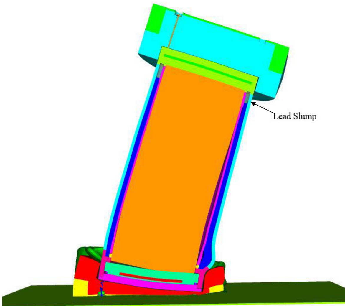
Figure 3-10 Deformed shape of the Rail-Lead cask following the 193-kph (120-mph) impact onto an unyielding target in the corner orientation
