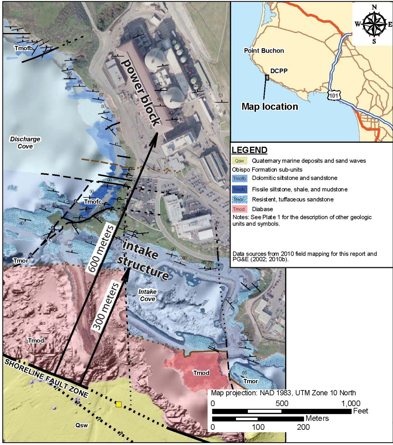
Figure C-9 Distance of Shoreline fault from intake structure and power block.
