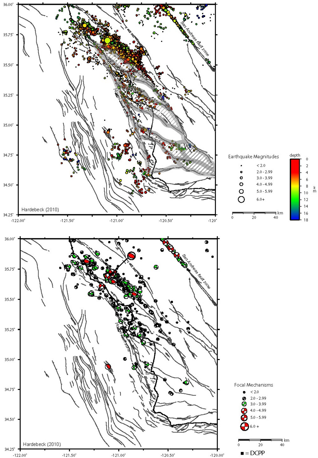
Figure 3-4 Seismicity patterns and focal mechanisms of the DCP region from 1987 through 2008 (extracted from Figure 3-2 of the PG&E Shoreline Fault Report).
