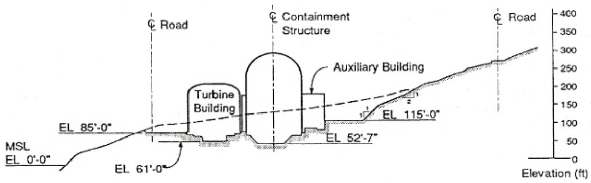
Figure 5-5 Cross section of DCPP (Figure 5-3 in DCPP LTSP Report).
