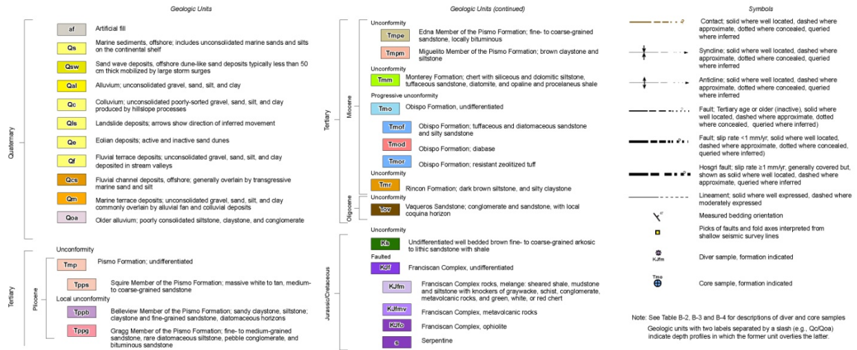
Figure 3-5 Geology underlying DCPD (extracted from Plate B-1B of the PG&E Shoreline Fault Report).
