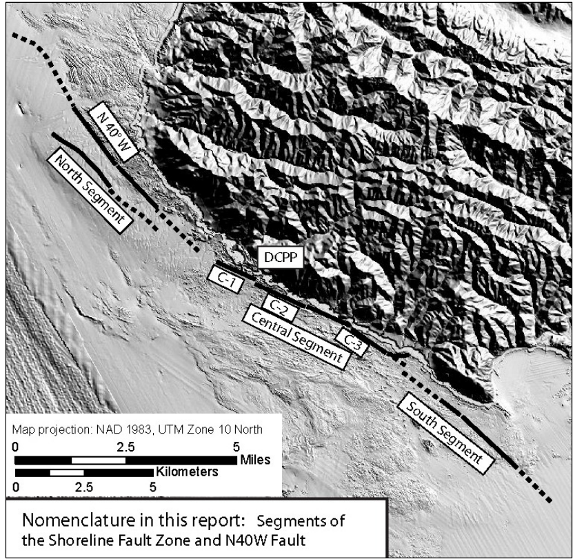
Figure 3-2 Shoreline fault location and segments (from Figure 4-1 of the PG&E Shoreline Fault Report).
