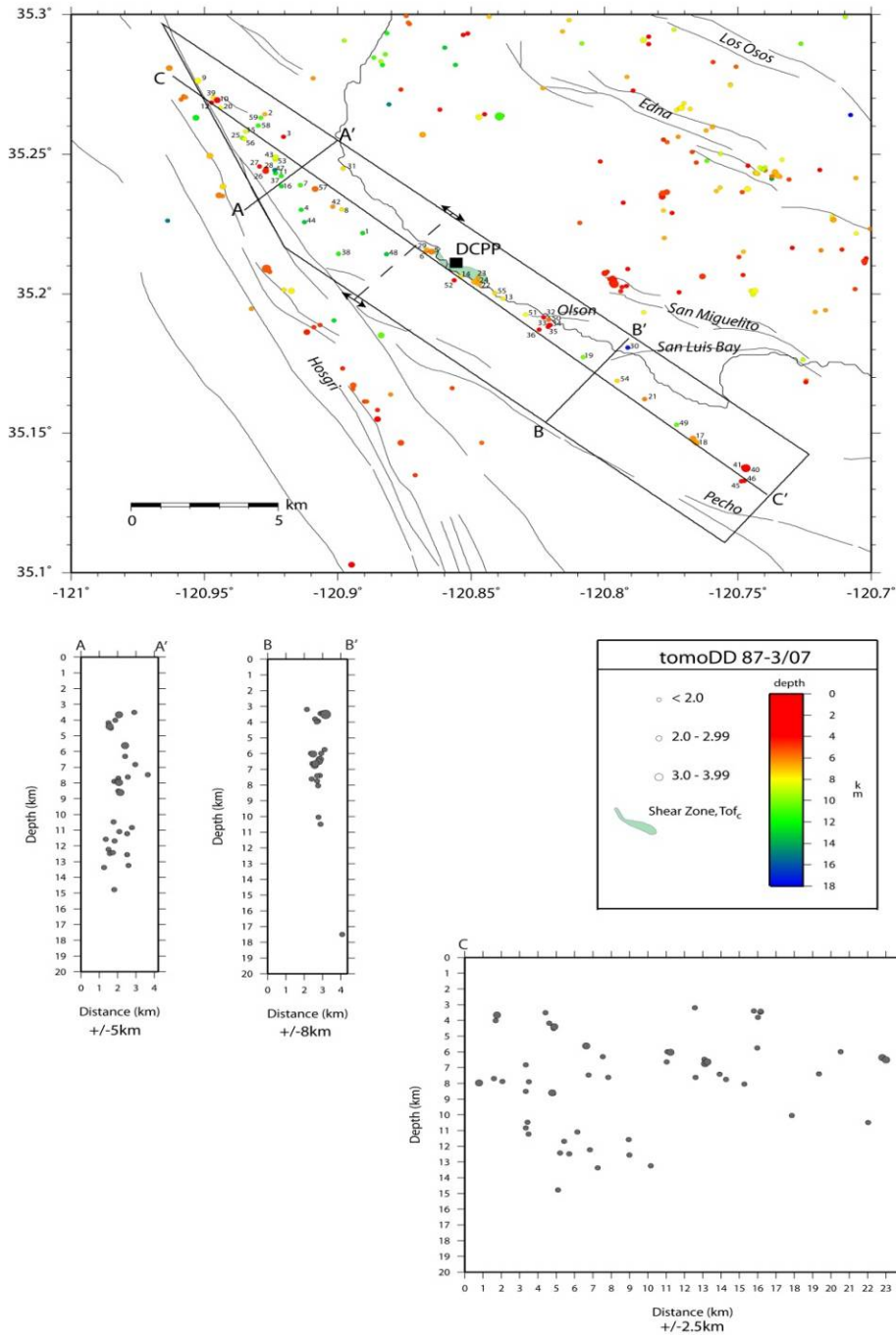
Figure 5-3 Seismicity in vicinity of DCP, figures and underlying data from the PG&E CRADA (Hardebeck, 2010).
