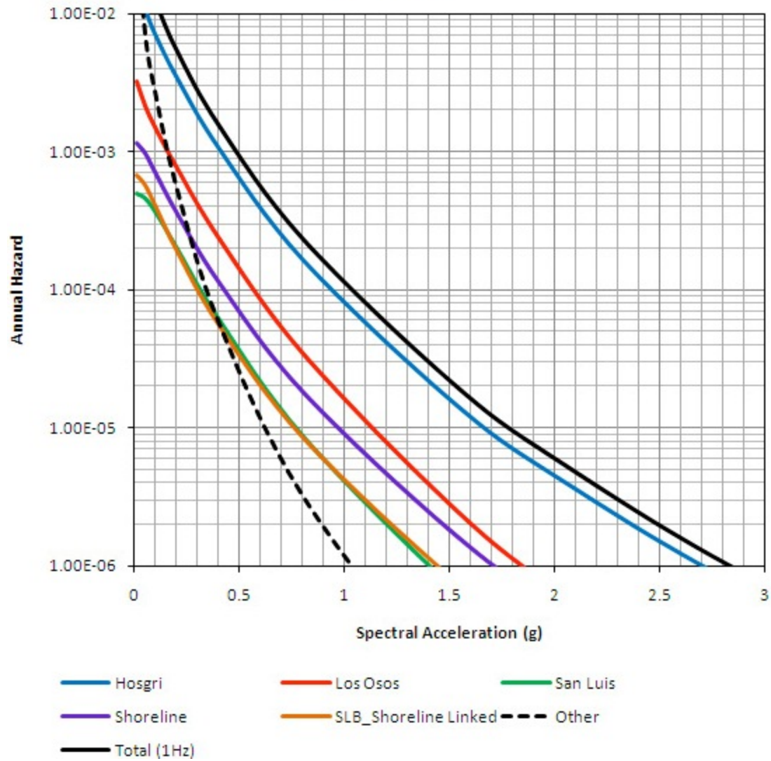
Figure 5-20 Contribution to seismic hazard by seismic source for 1 Hz (Figure 6-20 (c) of the PG&E Shoreline Fault Report).
