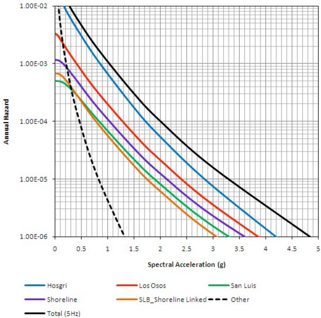
Figure 5-19 Contribution to seismic hazard by seismic source for 5 Hz (Figure 6-20 (b) of the PG&E Shoreline Fault Report).
