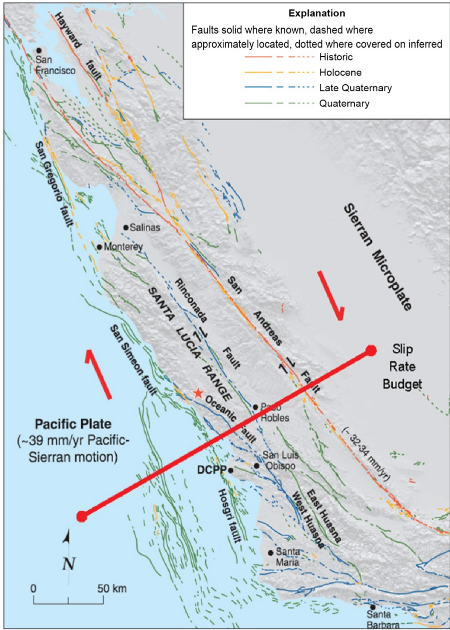
Figure D-1 Diagram illustrating the relative plate motions and the relative motions of major fault systems (base figure from Unruh presentation at the DCPD SSHAC WS#1, annotated for this report)
