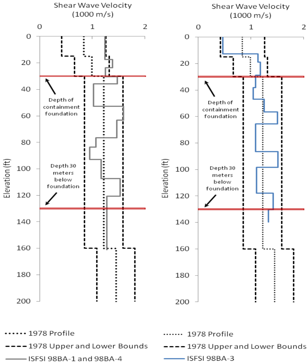
Figure 5-7 Comparison of 2010 DCPD ISFSI velocity profiles to that of the 1978 velocity profile.
