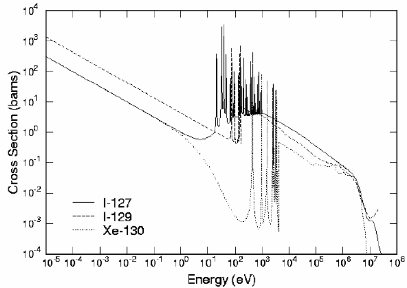
Capture Cross Sections of I-127, I-129 and Xe-130 (ENDF-B/V1)
