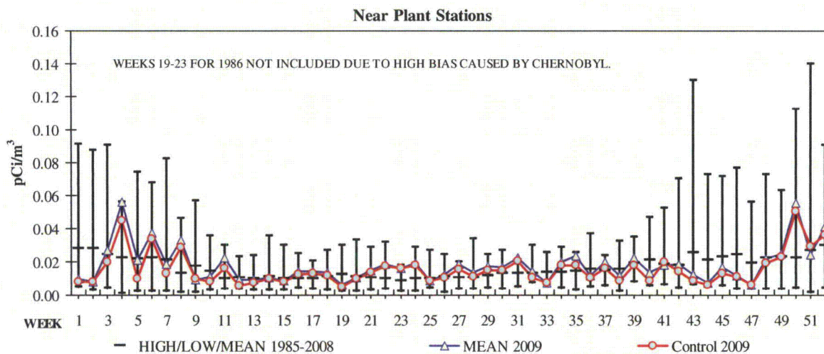
Figure 5-4 1985-2008 Weekly Hi/Low/Mean and 2009 Weekly Mean Gross Beta in Air - Near Plant Stations
