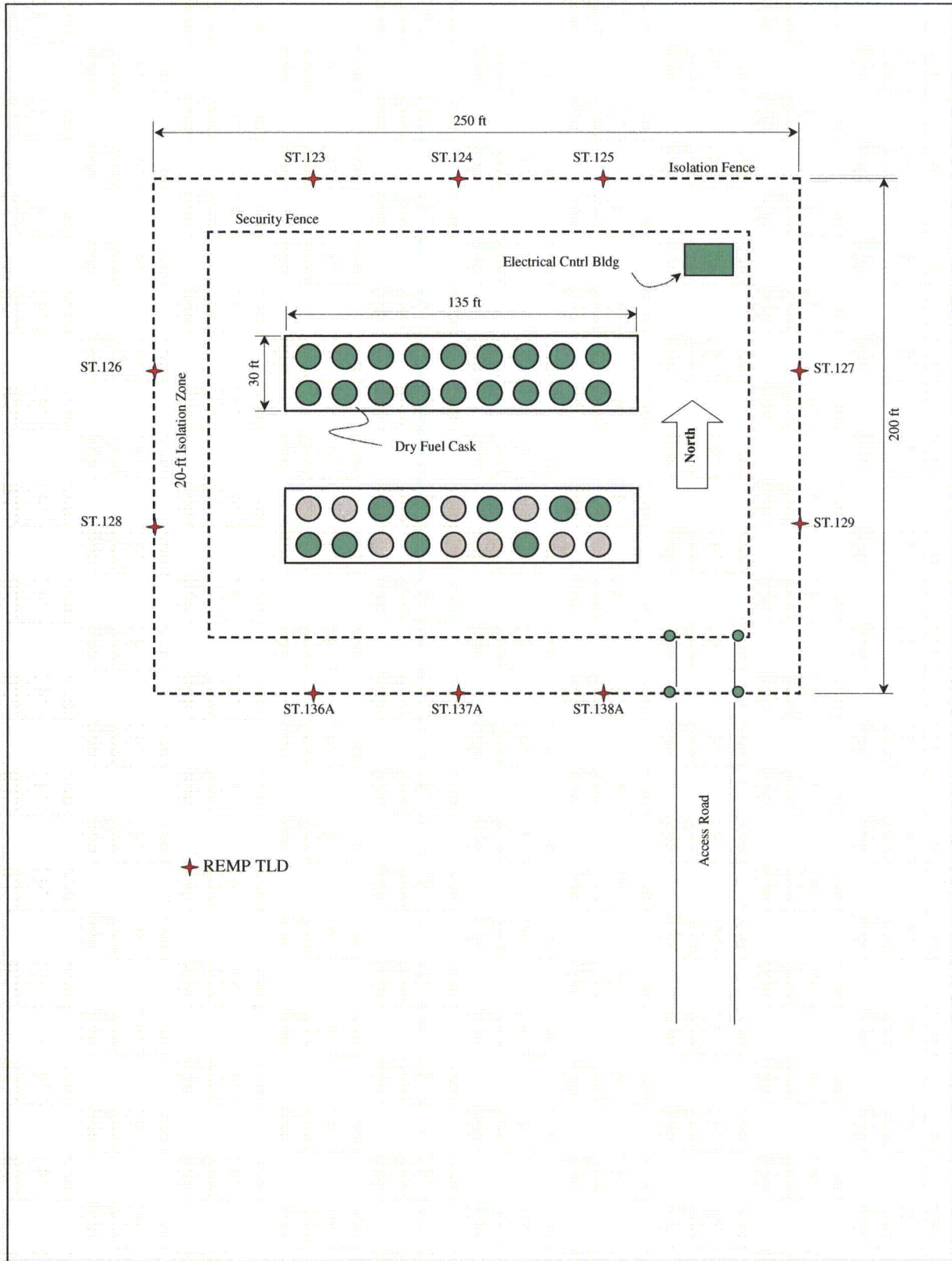
FIGURE 4-4 ISFSI TLD STATION LAYOUT
