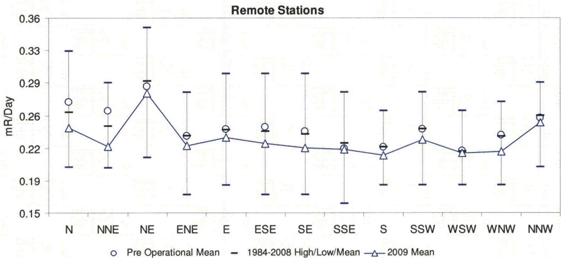
Figure 5-3 Remote Quarterly TLDs 1984-2008 Hi/Low/Mean and 2009 Mean By Sector
