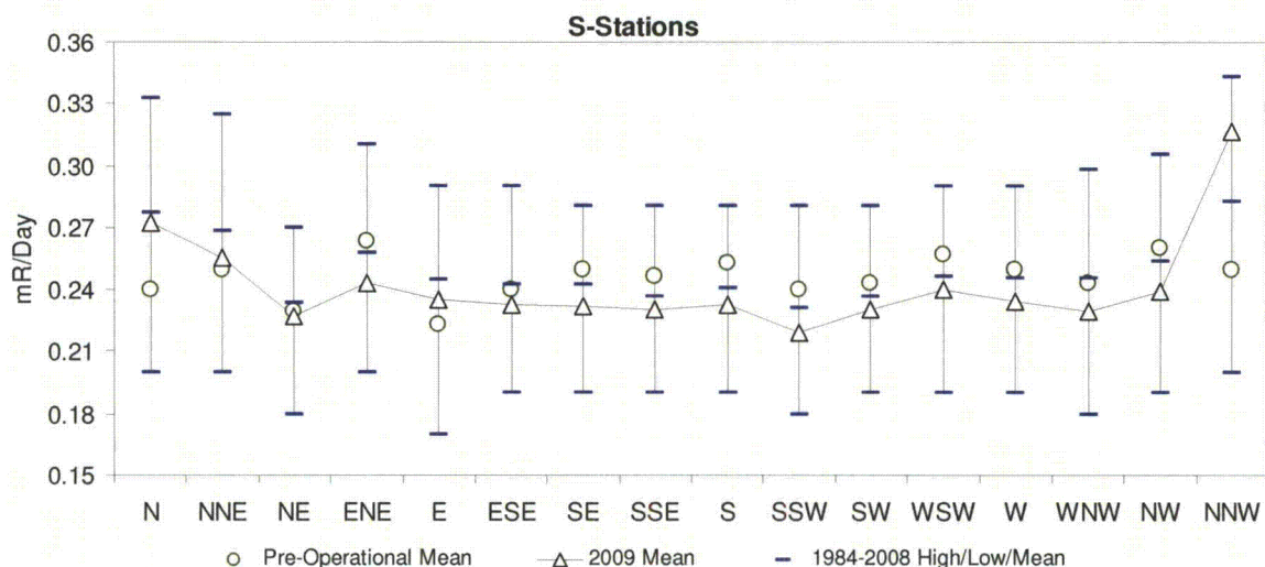
Figure 5-1 Site Boundary Quarterly TLDs 1984-2008 Hi/Low/Mean and 2009 Mean by Sector
