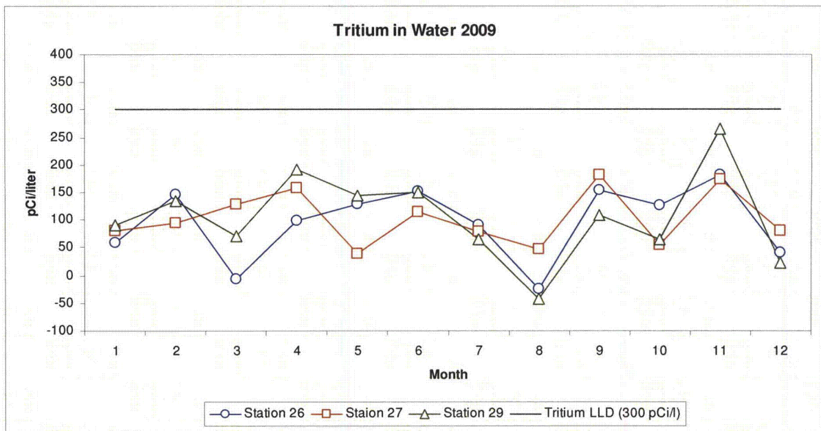
Figure 5-7 Tritium in River/Drinking ( Stations 26 & 29) and Plant Discharge Water (Station 27) for 2009
