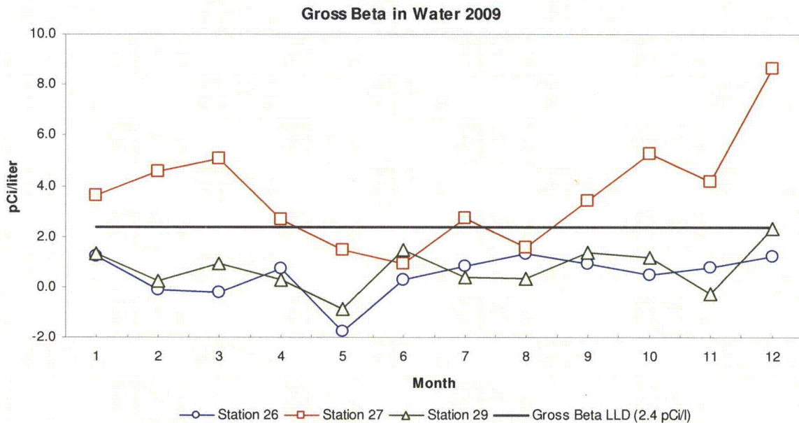
Figure 5-6 Gross Beta in River/Drinking ( Stations 26 & 29) and Plant Discharge Water (Station 27) for 2009
