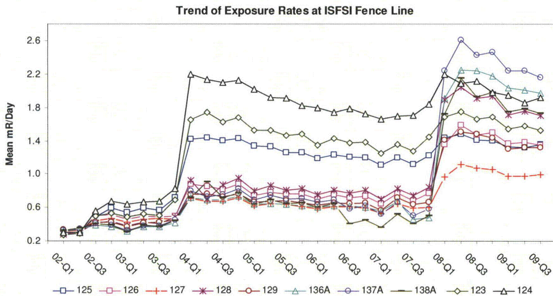
Figure 5-9 ISFSI TLD Trend at CGS (All TLDs located on outer security fence).
