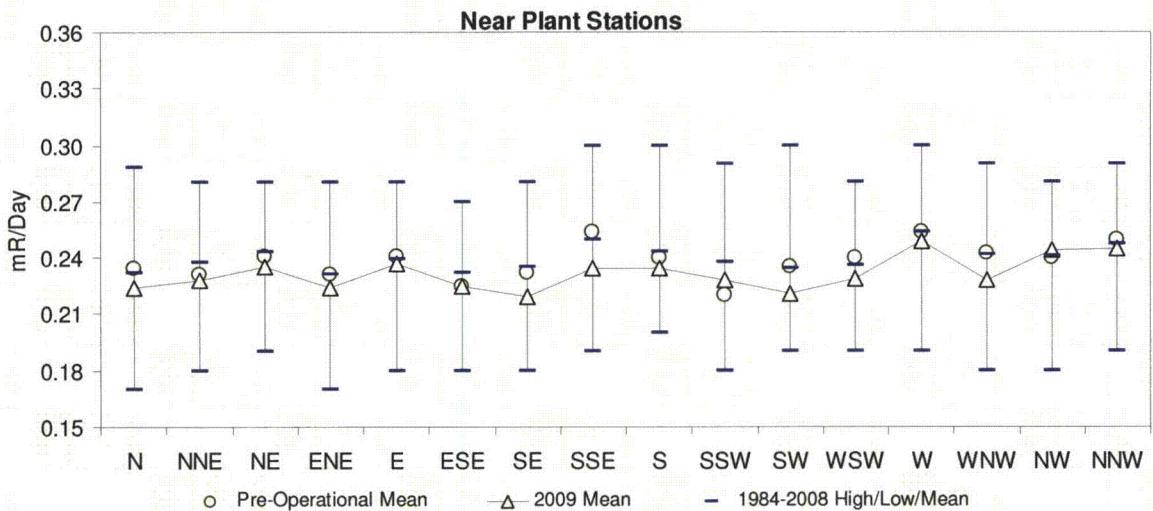
Figure 5-2 Near Plant Stations Quarterly TLDs 1984-2008 Hi/Low/Mean and 2009 Mean by Sector
