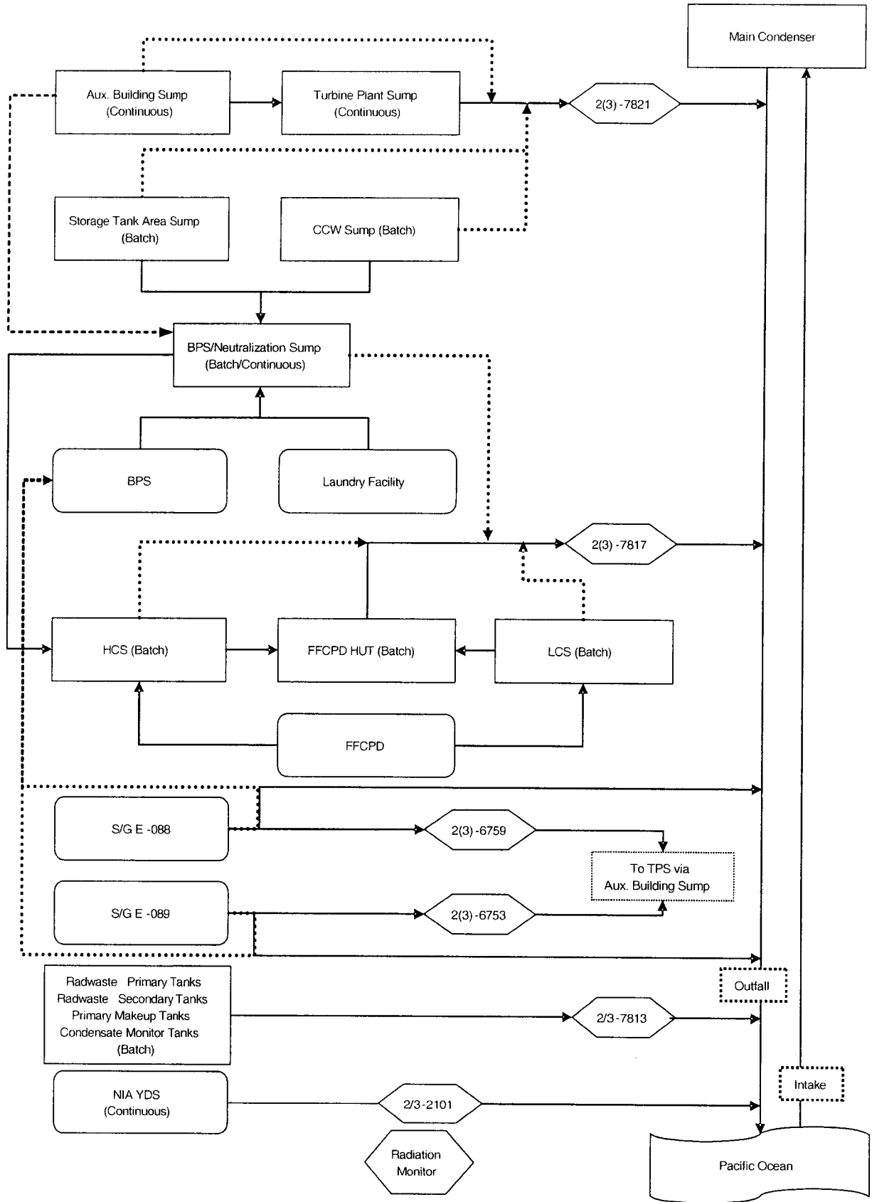
FIGURE 4-5 SONGS RADIOACTIVE LIQUID WASTE TREATMENT SYSTEMS
