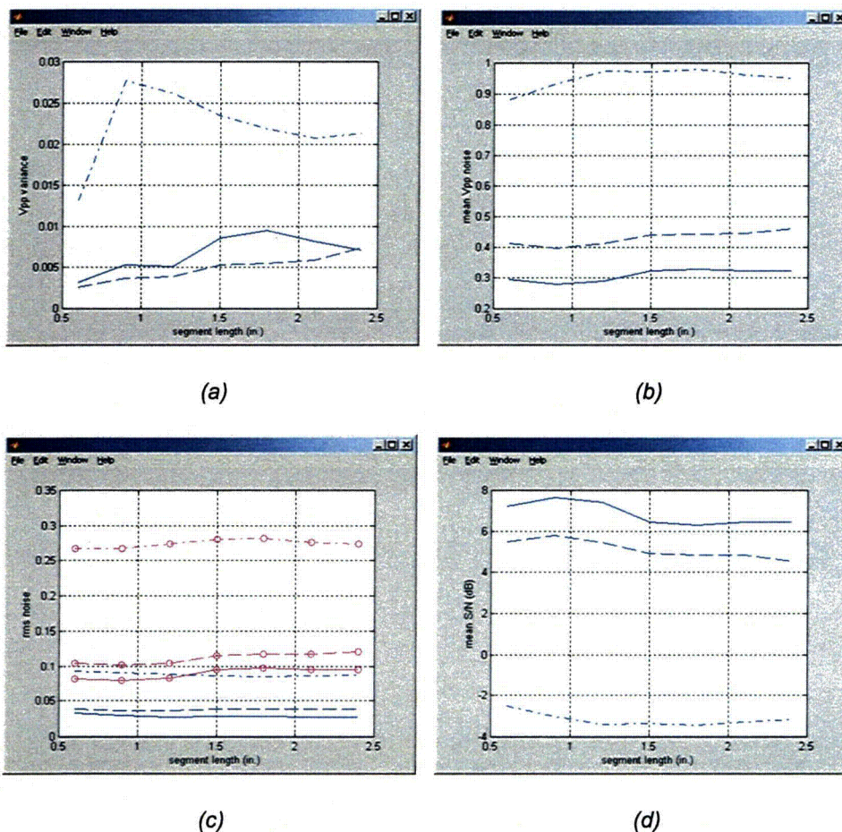
Figure 2.28 Fifth parametric evaluation of the influence of noise on bobbin coil data from mock-up test section of Fig. 2.18. Graphs show (a) variance of peak-to-peak ( V_{pp} ) noise, (b) mean value of V_{pp} noise, (c) vertical component and total (circles) RMS noise, and (d) mean value of S/N in dB, all as a function of segment length. Results are shown for processed channel data without (solid curves) and with random (dashed curves) and composite (dash-dot curves) noise. A fixed window length of \approx 15 mm (0.6 in) was used in all cases. The region of interest started outside the TSP edge (outer markings in Fig. 2.18) on both sides of the indication.
