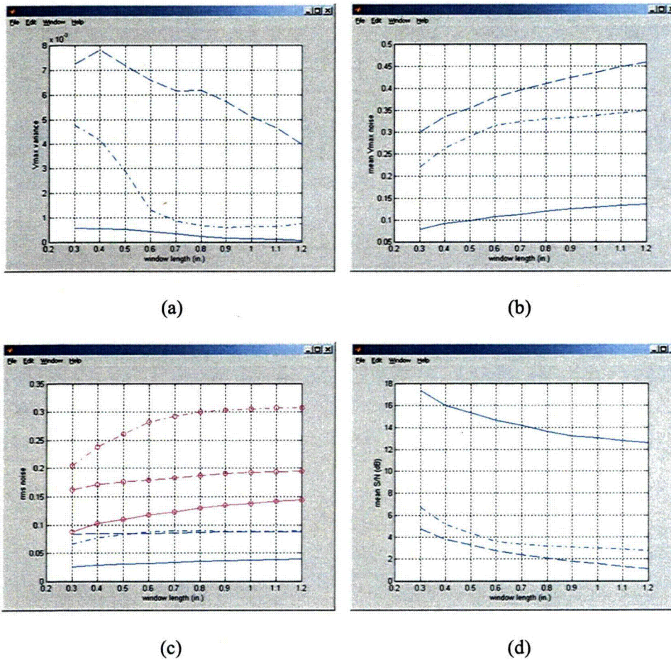
Figure 2.25 Second parametric evaluation of the influence of noise on bobbin coil data from mock-up test section of Fig. 2.23. Graphs show (a) variance of vertical component of noise ( V_{max} ), (b) mean value of V_{max} , (c) vertical component and total (circles) RMS noise, and (d) mean value of S/N in dB, all as a function of window length. Results are shown for processed channel data without (solid curves) and with random (dashed curves) and composite (dash-dot curves) noise. A fixed segment length of 45.7 mm (1.8 in) was used in all cases. The region of interest started outside the TSP edge (outer markings in Fig. 2.23) on both sides of the indication.
