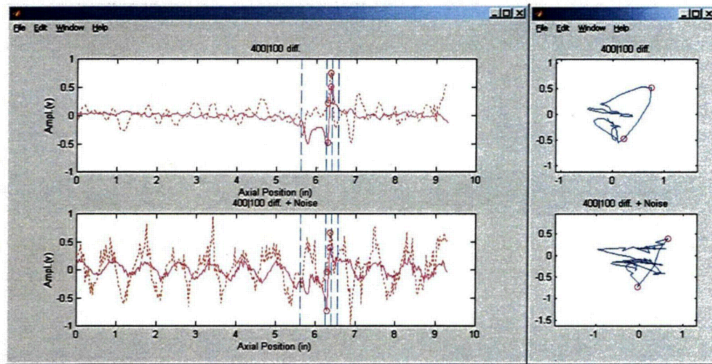
Figure 2.17 Second evaluation of the influence of noise on bobbin coil data from mock-up test section #14 with an ODSCC indication at a TSP intersection. Graphics show the processed channel data without (top) and with (bottom) the added noise. Also shown are the inner and outer markings that identify the approximate location of flaw and TSP ends, respectively. Composite noise consisted of a small random component using the same parameters as those in Fig. 2.10 and a periodic component with amplitude of 0.25 V ( V_{pp} = 0.5 V) and phase of 15^\circ .
