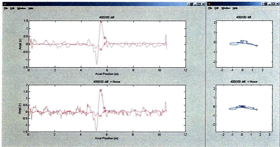
Figure 3.8 Eddy current data collected with bobbin coil from test section #8 with flaw at TSP intersection. Graphics show representative display of data in strip chart (left) and lissajous (right) format without (top) and with (bottom) simulated composite noise consisting of a small random and a periodic component.
