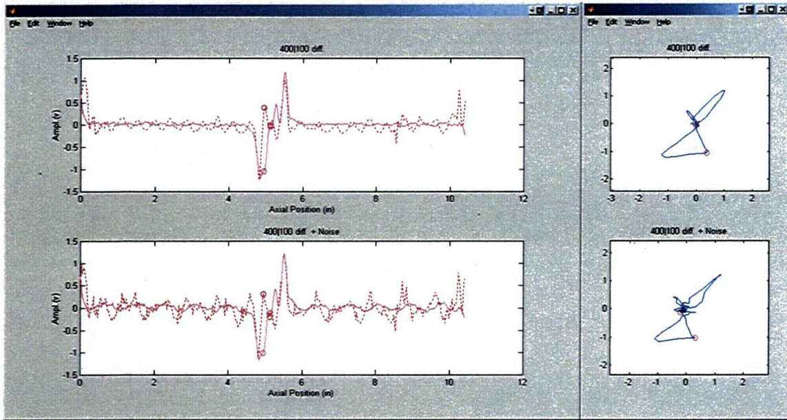
Figure 3.5 Eddy current data collected with bobbin coil from test section #5 with flaw at TSP intersection. Graphics show representative display of data in strip chart (left) and lissajous (right) format without (top) and with (bottom) simulated composite noise consisting of a small random and a periodic component.
