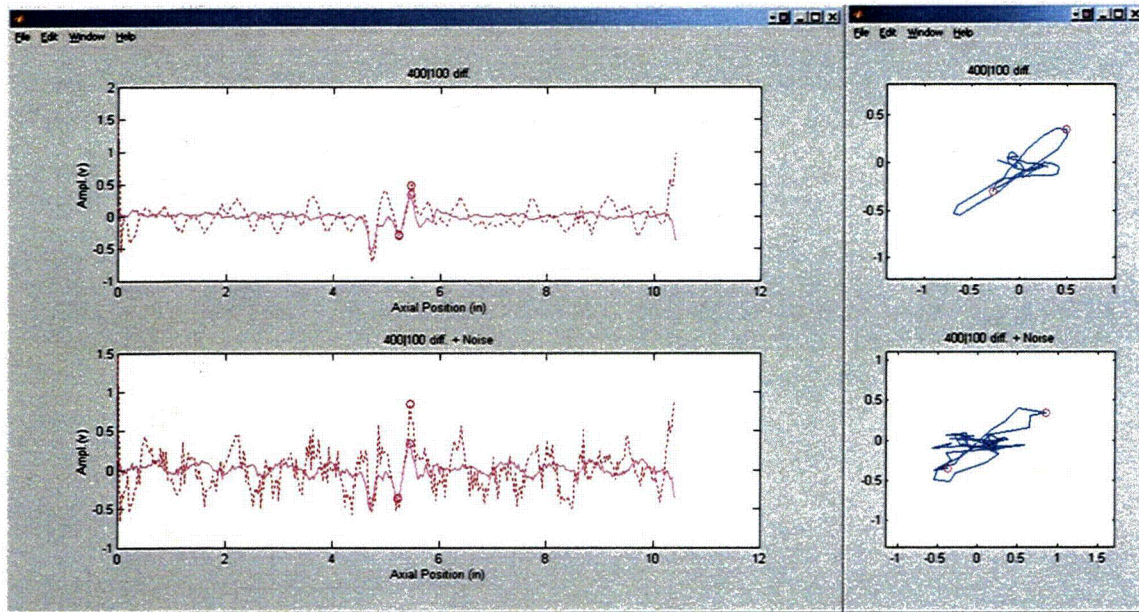
Figure 3.9 Eddy current data collected with bobbin coil from test section #9 with flaw at TSP intersection. Graphics show representative display of data in strip chart (left) and lissajous (right) format without (top) and with (bottom) simulated composite noise consisting of a small random and a periodic component.
