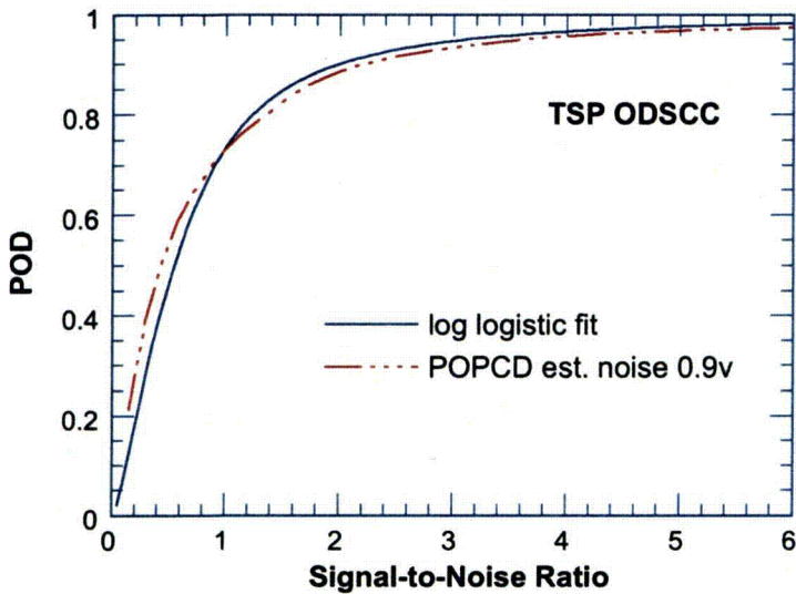
Figure 3.20 Probability of detection as a function of (S/N)^v . The log logistic fit to the data from the round-robin is shown as solid curve. For comparison, a POD vs (S/N)^v curve estimated from the POPCD curve for TSPs is also shown. A value of 0.9 V was assumed for all specimens in the POPCD database.
