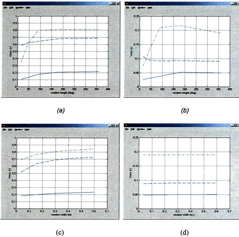
Figure 2.38 Parametric evaluation of noise influence on rotating probe data from mock-up test section of Fig. 2.36(b). Graphs show (a) mean V_{max} and (b) V_{rms} noise as a function of window height for a fixed window width of 7.6 mm (0.3 in), and (c) mean V_{max} and (d) V_{rms} as a function of window width for a fixed window height of 360^\circ . Results are shown for 2.92-mm (0.115-in)-diameter pancake at 300 kHz without (solid curves) and with random (dashed curves) and composite (dash-dot curves) noise. The region of interest is two 25.4-mm (1.0-in)-long free-span sections on both sides and away from the TSP edges.
