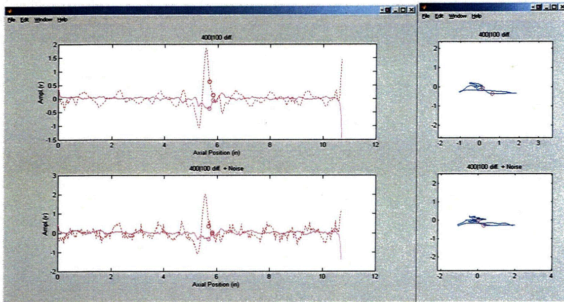
Figure 3.13 Eddy current data collected with bobbin coil from test section #13 with flaw at TSP intersection. Graphics show representative display of data in strip chart (left) and lissajous (right) format without (top) and with (bottom) simulated composite noise consisting of a small random and a periodic component.
