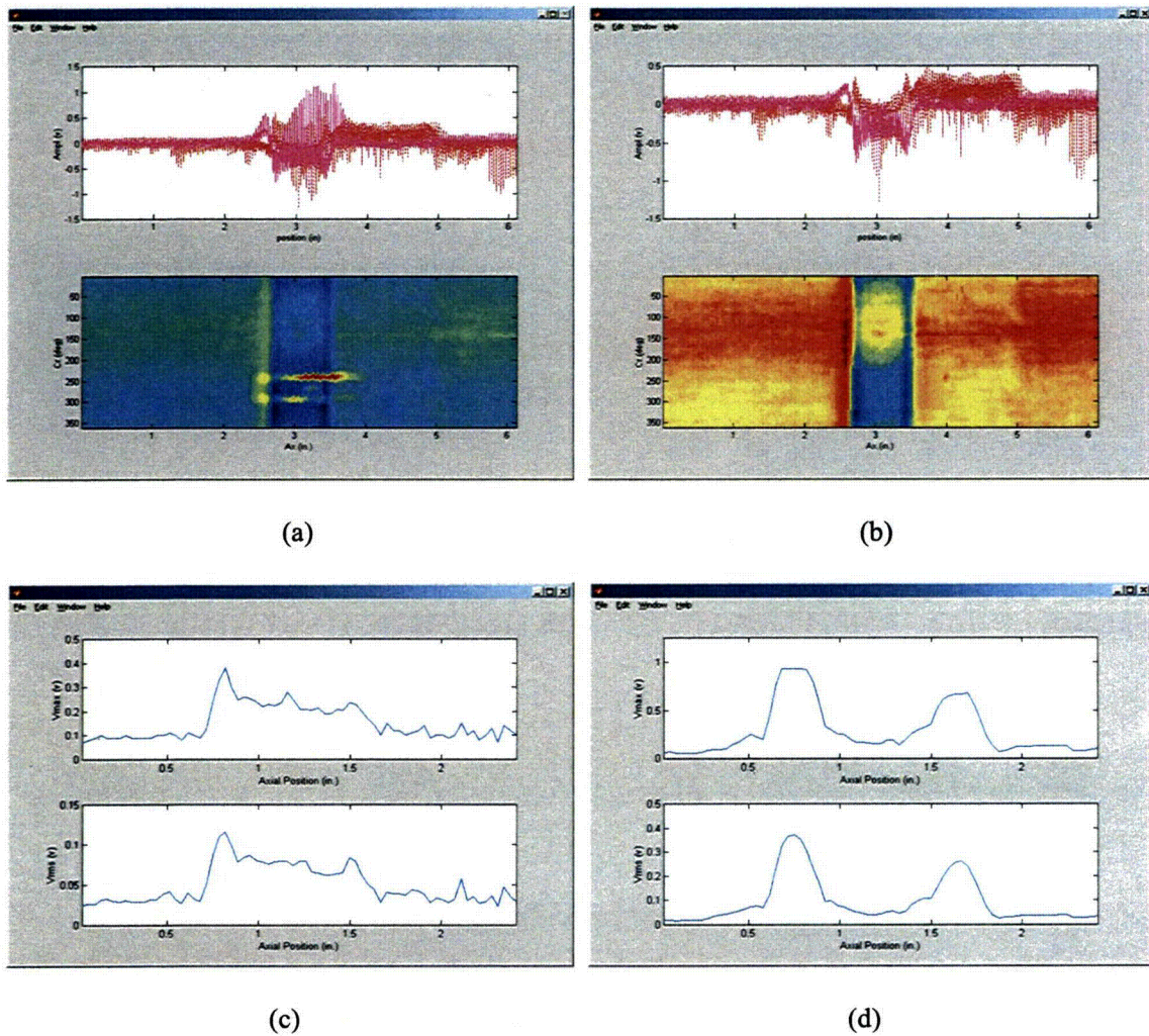
Figure 2.40 Measurement of noise at the same location as the flaw. Graphics display the intermediate stages of the process (a) before and (b) after elimination of the flaw signal from the TSP intersection with ODS/CC indications. Also shown are V_{max} and V_{rms} noise along the tube axis using (c) 0.9-mm (0.035-in) window width and 45° window height and (d) 7.6-mm (0.3-in) window width and 5° window height. The region of interest is a 63.5-mm (2.5-in)-long section of tube centered approximately at the middle of the TSP.
