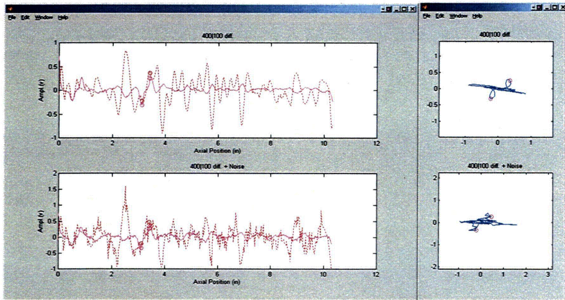
Figure 3.3 Eddy current data collected with bobbin coil from test section #3 with flaw at free-span region. Graphics show representative display of data in strip chart (left) and lissajous (right) format without (top) and with (bottom) simulated composite noise consisting of a small random and a periodic component.
