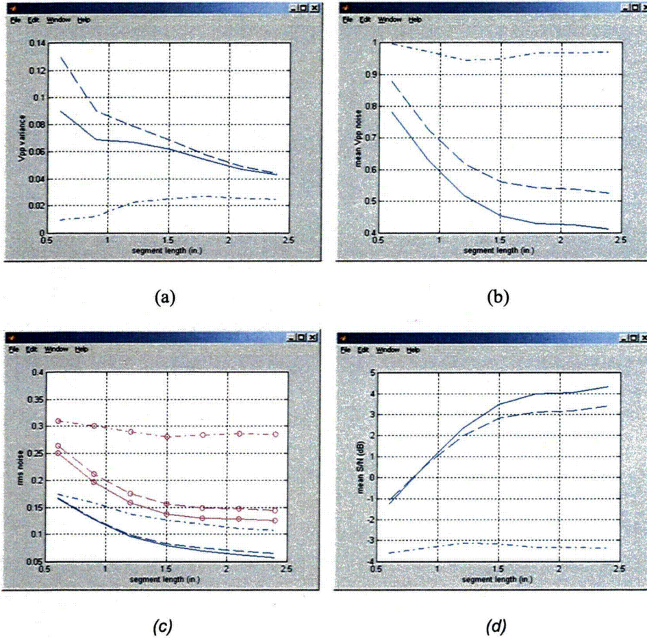
Figure 2.30 Seventh parametric evaluation of the influence of noise on bobbin coil data from mock-up test section of Fig. 2.18. Graphs show (a) variance of peak-to-peak ( V_{pp} ) noise, (b) mean value of V_{pp} noise, (c) vertical component and total (circles) RMS noise, and (d) mean value of S/N in dB, all as a function of segment length. Results are shown for processed channel data without (solid curves) and with random (dashed curves) and composite (dash-dot curves) noise. A fixed window length of \approx 15 mm (0.6 in) was used in all cases. The region of interest started outside the flaw signal (inner markings in Fig. 2.18) on both sides of the indication.
