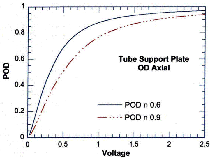
Figure 3.23 Probability of detection as a function of signal voltage for average noise levels of 0.6 V and 0.9 V.
