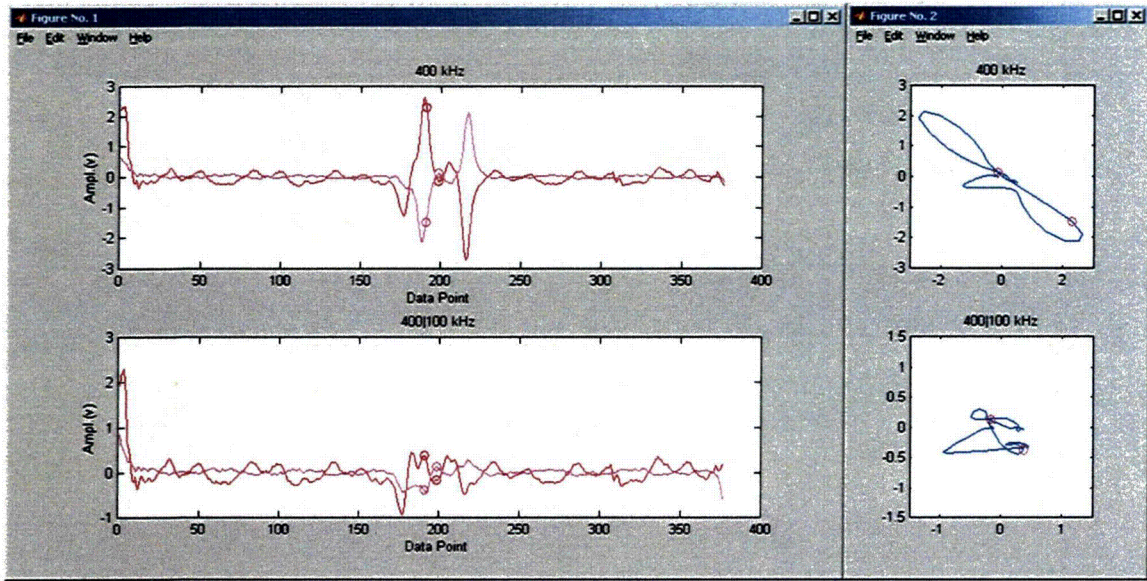
Figure 2.5 Evaluation of bobbin coil mix results for TSP-level test section #4 with ODSCC indication. Graphics show original (top left) and processed (bottom left) traces and lissajous plot of results for TSP zone before (top right) and after (bottom right) mix.
