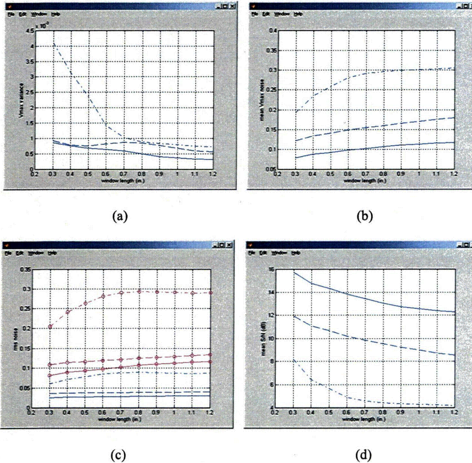
Figure 2.20 Second parametric evaluation of the influence of noise on bobbin coil data from mock-up test section of Fig. 2.18. Graphs show (a) variance of vertical component of noise ( V_{max} ), (b) mean value of V_{max} , (c) vertical component and total (circles) RMS noise, and (d) mean value of S/N in dB, all as a function of window length. Results are shown for processed channel data without (solid curves) and with random (dashed curves) and composite (dash-dot curves) noise. A fixed segment length of 45.7 mm (1.8 in) was used in all cases. The region of interest started outside the TSP edge (outer markings in Fig. 2.18) on both sides of the indication.
