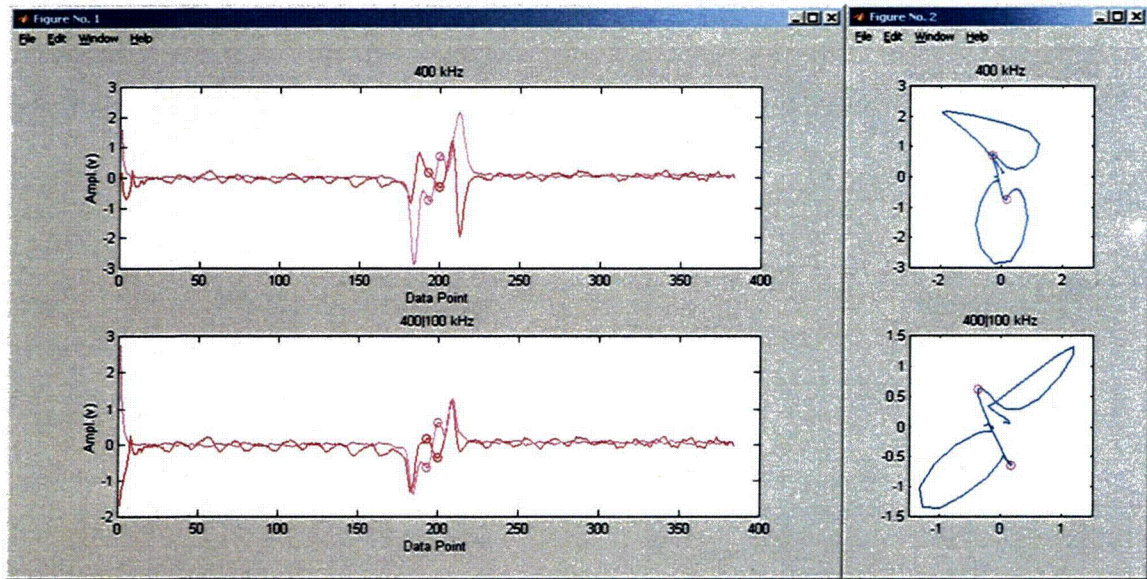
Figure 2.6 Evaluation of bobbin coil mix results for TSP-level test section #6 with ODSCC indication. Graphics show original (top left) and processed (bottom left) traces and lissajous plot of results for TSP zone before (top right) and after (bottom right) mix.
