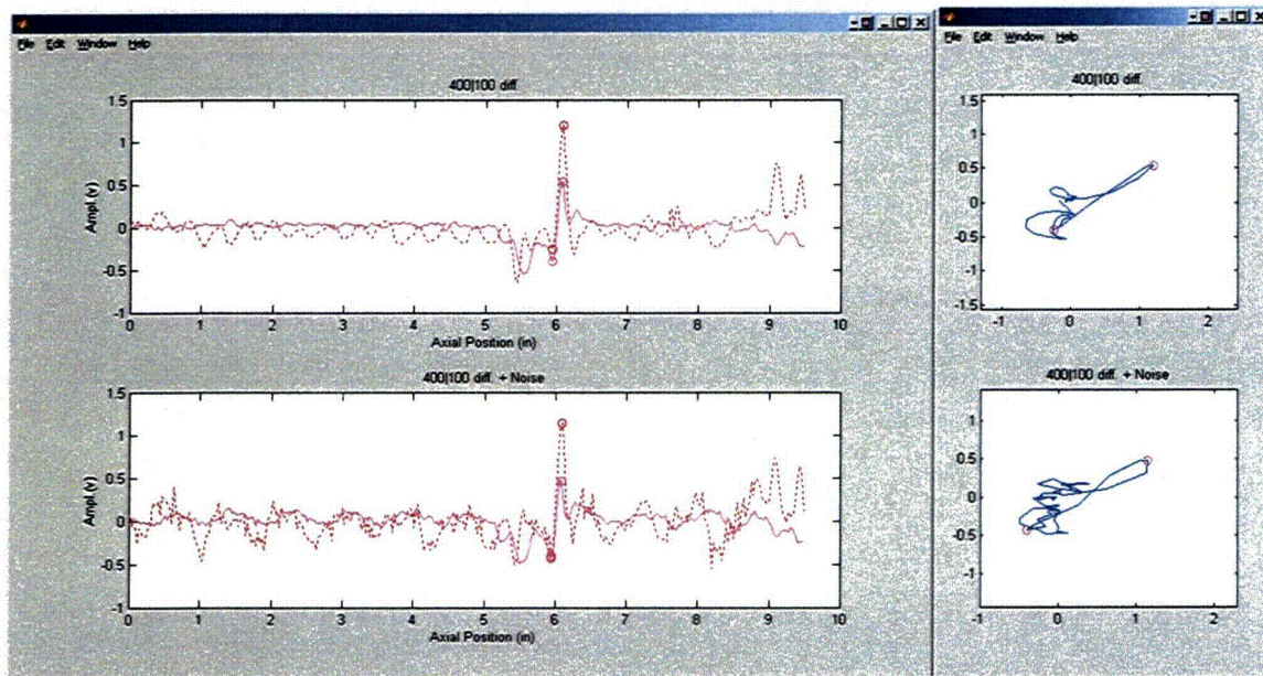
Figure 3.10 Eddy current data collected with bobbin coil from test section #10 with flaw at TSP intersection. Graphics show representative display of data in strip chart (left) and lissajous (right) format without (top) and with (bottom) simulated composite noise consisting of a small random and a periodic component.
