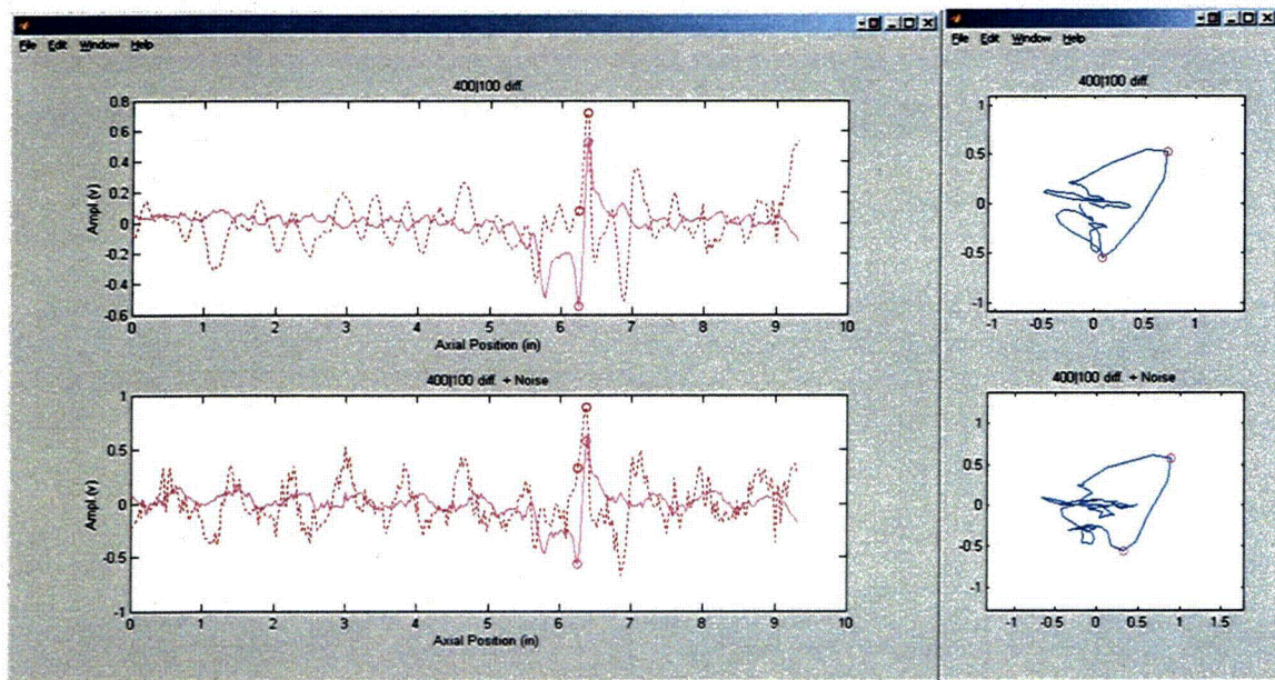
Figure 3.14 Eddy current data collected with bobbin coil from test section #14 with flaw at TSP intersection. Graphics show representative display of data in strip chart (left) and lissajous (right) format without (top) and with (bottom) simulated composite noise consisting of a small random and a periodic component.
