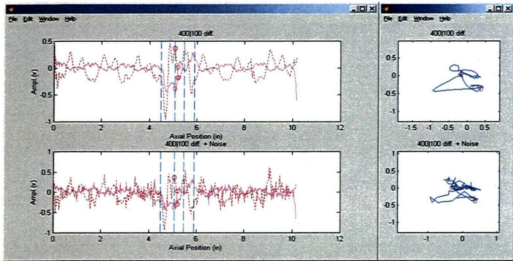
Figure 2.14 Evaluation of the influence of noise on bobbin coil data from mock-up test section #4 with an ODSCC indication at a TSP intersection. Graphics show the processed channel data without (top) and with (bottom) the added noise. Also shown are the inner and outer markings that identify the approximate location of flaw and TSP ends, respectively. Random noise with horizontal amplification factor of 1 and vertical amplification factor of 2 was added to every other data point.
