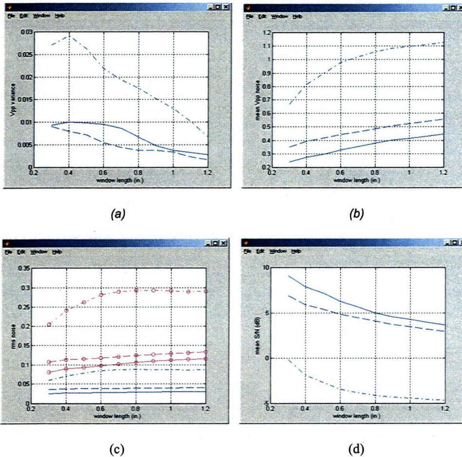
Figure 2.29 Sixth parametric evaluation of the influence of noise on bobbin coil data from mock-up test section of Fig. 2.18. Graphs show (a) variance of peak-to-peak ( V_{pp} ) noise, (b) mean value of V_{pp} noise, (c) vertical component and total (circles) RMS noise, and (d) mean value of S/N in dB, all as a function of window length. Results are shown for processed channel data without (solid curves) and with random (dashed curves) and composite (dash-dot curves) noise. A fixed segment length of \approx 46 mm (1.8 in) was used in all cases. The region of interest started outside the TSP edge (outer markings in Fig. 2.18) on both sides of the indication.
