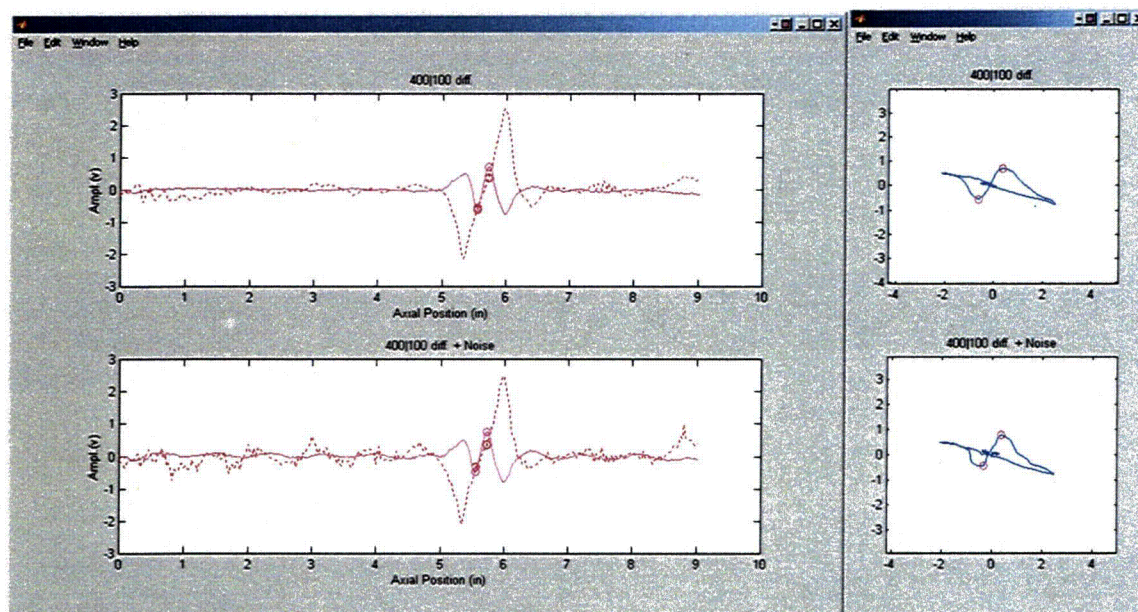
Figure 3.17 Eddy current data collected with bobbin coil from test section #17 with flaw at TSP intersection. Graphics show representative display of data in strip chart (left) and lissajous (right) format without (top) and with (bottom) simulated composite noise consisting of a small random and a periodic component.
