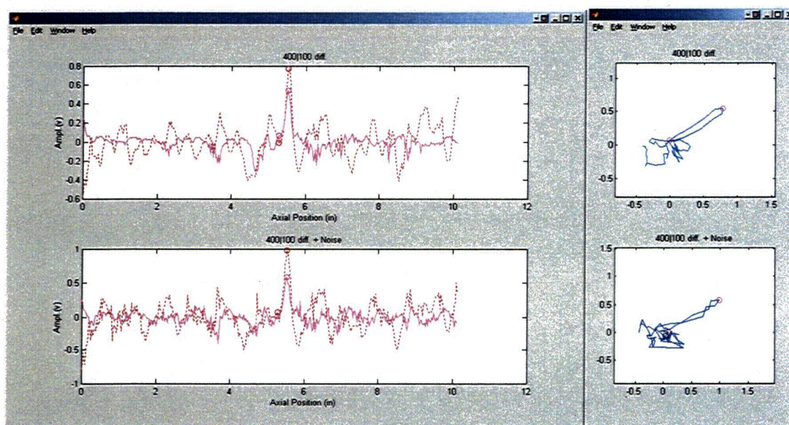
Figure 3.18 Eddy current data collected with bobbin coil from test section #18 with flaw at free-span region. Graphics show representative display of data in strip chart (left) and lissajous (right) format without (top) and with (bottom) simulated composite noise consisting of a small random and a periodic component.
