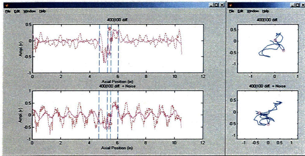
Figure 2.13 Fourth evaluation of the influence of noise on bobbin coil data from mock-up test section #1 with an ODSCC indication at a TSP intersection. Graphics show the processed channel data without (top) and with (bottom) the added noise. Also shown are the inner and outer markings that identify the approximate location of flaw and TSP ends, respectively. Composite noise consisted of a small random component, as that in Fig. 2.10, and a periodic component with amplitude of 0.25 V ( V_{pp} = 0.5 V) and phase of 15^\circ .
