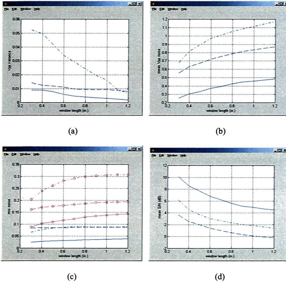
Figure 2.33 Second parametric evaluation of the influence of noise on bobbin coil data from mock-up test section of Fig. 2.23. Graphs show (a) variance of peak-to-peak ( V_{pp} ) noise, (b) mean value of V_{pp} noise, (c) vertical component and total (circles) RMS noise, and (d) mean value of S/N in dB, all as a function of window length. Results are shown for processed channel data without (solid curves) and with random (dashed curves) and composite (dash-dot curves) noise. A fixed segment length of \approx 46 mm (1.8 in) was used in all cases. The region of interest started outside the TSP edge (outer markings in Fig. 2.23) on both sides of the indication.
