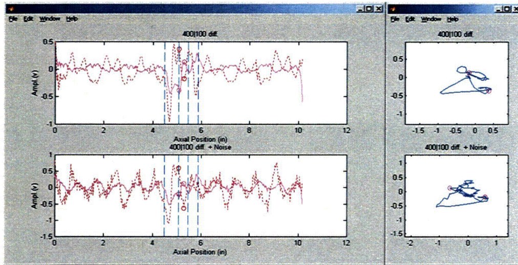
Figure 2.15 Second evaluation of the influence of noise on bobbin coil data from mock-up test section #4 with an ODSCC indication at a TSP intersection. Graphics show the processed channel data without (top) and with (bottom) the added noise. Also shown are the inner and outer markings that identify the approximate location of flaw and TSP ends, respectively. Composite noise consisted of a small random component, as that in Fig. 2.10, and a periodic component with amplitude of 0.25 V ( V_{pp} = 0.5 V) and phase of 15^\circ .
