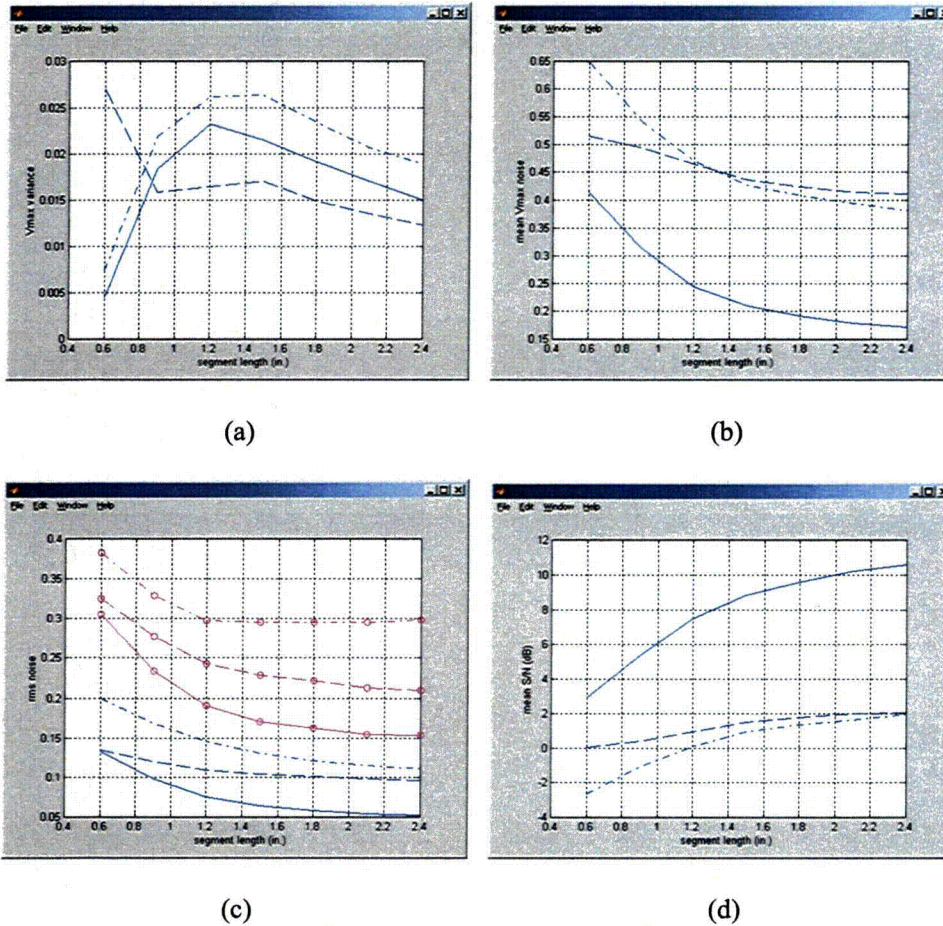
Figure 2.26 Third parametric evaluation of the influence of noise on bobbin coil data from mock-up test section of Fig. 2.23. Graphs show (a) variance of vertical component of noise ( V_{max} ), (b) mean value of V_{max} , (c) vertical component and total (circles) RMS noise, and (d) mean value of S/N in dB, all as a function of segment length. Results are shown for processed channel data without (solid curves) and with random (dashed curves) and composite (dash-dot curves) noise. A fixed window length of 15.2 mm (0.6 in) was used in all cases. The region of interest started outside the flaw signal (inner markings in Fig. 2.23) on both sides of the indication.
