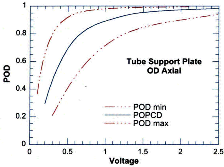
Figure 3.26 Range of probabilities of detection expected for a given voltage for log-normal noise with a mean value of 0.9 V based on the POPCD curve.
