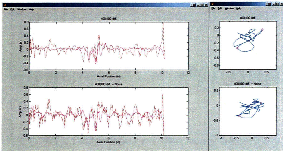
Figure 3.11 Eddy current data collected with bobbin coil from test section #11 with flaw at TSP intersection. Graphics show representative display of data in strip chart (left) and lissajous (right) format without (top) and with (bottom) simulated composite noise consisting of a small random and a periodic component.
