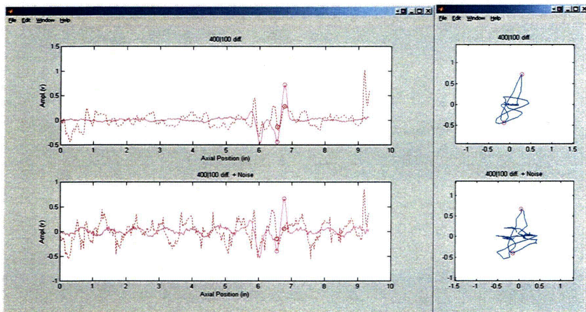
Figure 3.12 Eddy current data collected with bobbin coil from test section #12 with flaw at TSP intersection. Graphics show representative display of data in strip chart (left) and lissajous (right) format without (top) and with (bottom) simulated composite noise consisting of a small random and a periodic component.
