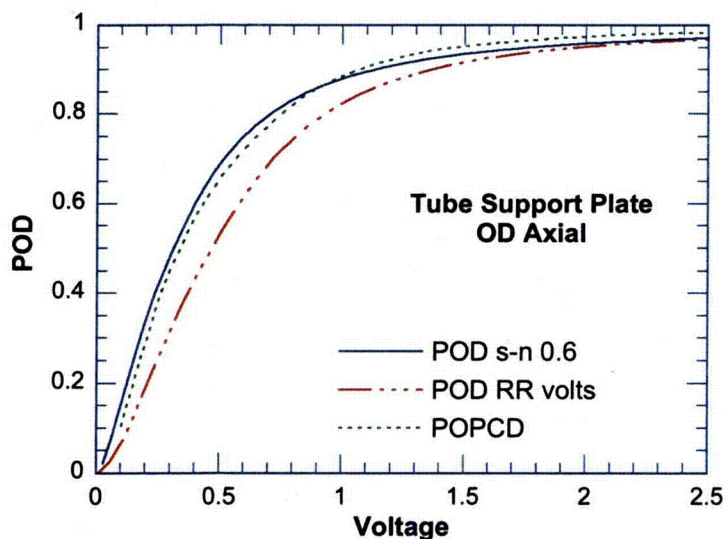
Figure 3.22 Probability of detection as a function of voltage. POD RR denotes the probability of detection
