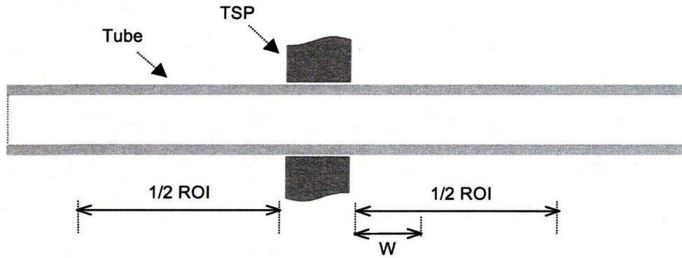
Figure 2.9 Depiction of the measurement region and the associated variables for the measurement of noise outside a TSP intersection. The total segment length, i.e., the region of interest (ROI), is composed of two equal segments on both sides of the TSP. Also shown is the size of each measurement window, W . For standard measurement of noise, six successive measurements that encompass ROI are averaged.
