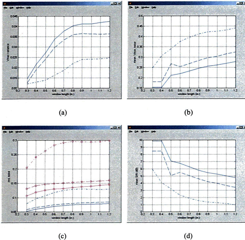
Figure 2.22 Fourth parametric evaluation of the influence of noise on bobbin coil data from mock-up test section of Fig. 2.18. Graphs show (a) variance of vertical component of noise ( V_{max} ), (b) mean value of V_{max} , (c) vertical component and total (circles) RMS noise, and (d) mean value of S/N in dB, all as a function of window length. Results are shown for processed channel data without (solid curves) and with random (dashed curves) and composite (dash-dot curves) noise. A fixed segment length of 45.7 mm (1.8 in) was used in all cases. The region of interest started outside the flaw signal (inner markings in Fig. 2.18) on both sides of the indication.
