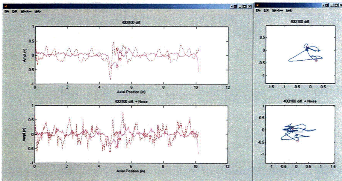
Figure 3.4 Eddy current data collected with bobbin coil from test section #4 with flaw at TSP intersection. Graphics show representative display of data in strip chart (left) and lissajous (right) format without (top) and with (bottom) simulated composite noise consisting of a small random and a periodic component.
