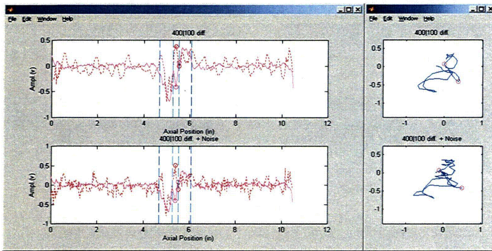
Figure 2.10 Evaluation of the influence of noise on bobbin coil data from mock-up test section #1 with an ODS-CC indication at a TSP intersection. Graphics show the processed channel data without (top) and with (bottom) the added noise. Axial trace of both the vertical (solid line) and the horizontal (dashed line) component of data are shown in each stripchart plot. Also shown are the inner and outer markings that identify the approximate location of flaw and TSP ends, respectively. Random noise with an amplification factor of 1 was added proportionally to both channels and to every other data point.
