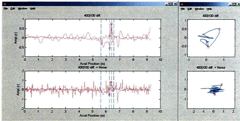
Figure 2.16 Evaluation of the influence of noise on bobbin coil data from mock-up test section #14 with an ODSCC indication at a TSP intersection. Graphics show the processed channel data without (top) and with (bottom) the added noise. Also shown are the inner and outer markings that identify the approximate location of flaw and TSP ends, respectively. Random noise with an amplification factor of 2 was added proportionally to both channels and to every other data point.
