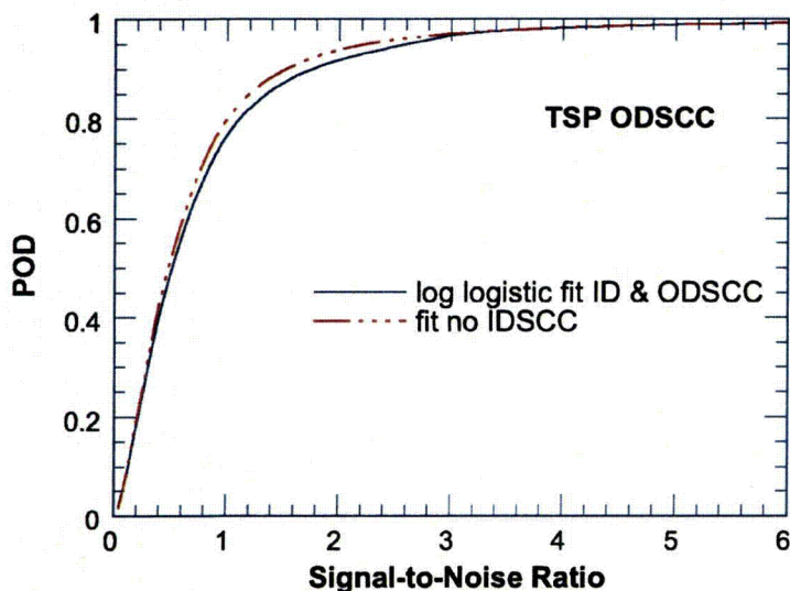
Figure 3.21 Probability of detection as a function of S/N . Although flaws are predominantly ODSCC, the data includes some IDSCC. Excluding the IDSCC data does not significantly change the POD curve.
