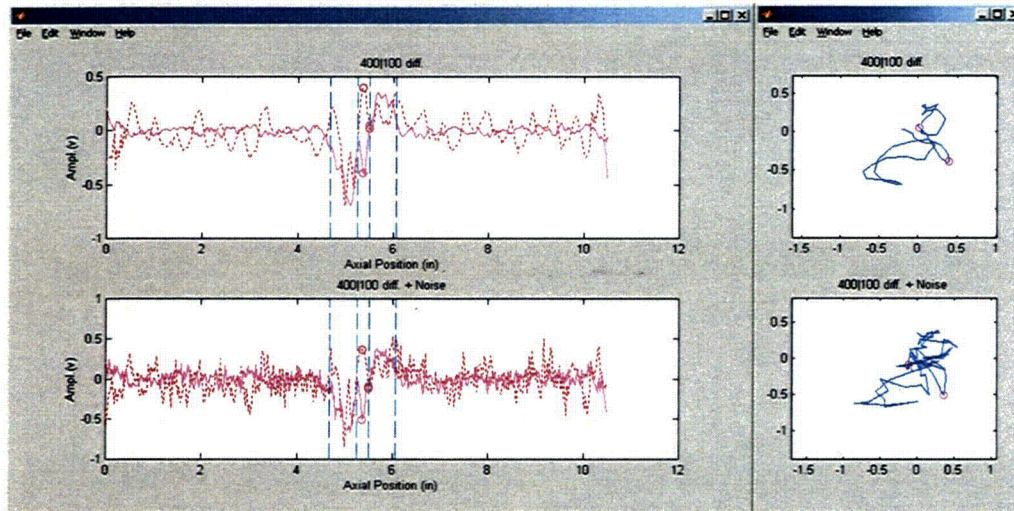
Figure 2.12 Third evaluation of the influence of noise on bobbin coil data from mock-up test section #1 with an ODSCC indication at a TSP intersection. Graphics show the processed channel data without (top) and with (bottom) the added noise. Also shown are the inner and outer markings that identify the approximate location of flaw and TSP ends, respectively. Random noise with horizontal amplification factor of 1 and vertical amplification factor of 2 was added to every data point.
