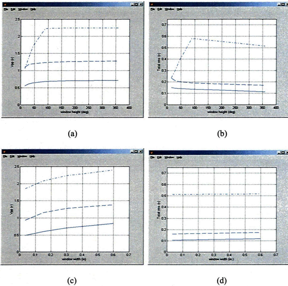
Figure 2.39 Second parametric evaluation of noise influence on rotating probe data from mock-up test section of Fig. 2.36(b). Graphs show (a) mean V_{pp} and (b) total RMS noise that include contributions from horizontal and vertical components as a function of window height for a fixed window width of 7.6 mm (0.3 in), and (c) mean V_{pp} and (d) total RMS noise as a function of window width for a fixed window height of 360^\circ . Results are for 2.92-mm (0.115-in)-diameter pancake at 300 kHz without (solid curves) and with random (dashed curves) and composite (dash-dot curves) noise. The region of interest is two 25.4-mm (1.0-in)-long free-span sections on both sides and away from the TSP edges.
