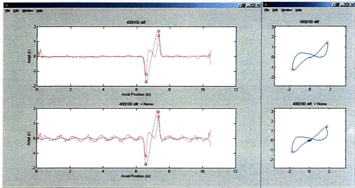
Figure 3.7 Eddy current data collected with bobbin coil from test section #7 with flaw at free-span region. Graphics show representative display of data in strip chart (left) and lissajous (right) format without (top) and with (bottom) simulated composite noise consisting of a small random and a periodic component.
