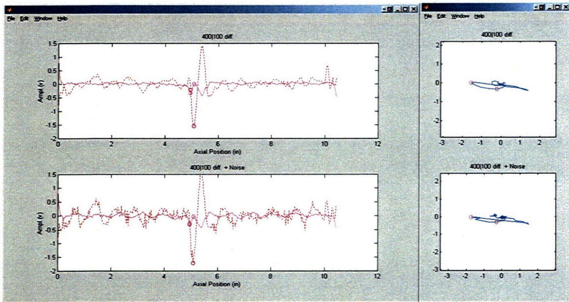
Figure 3.16 Eddy current data collected with bobbin coil from test section #16 with flaw at TSP intersection. Graphics show representative display of data in strip chart (left) and lissajous (right) format without (top) and with (bottom) simulated composite noise consisting of a small random and a periodic component.
