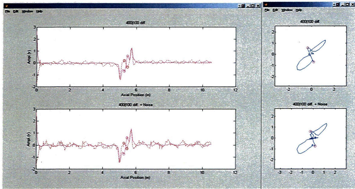
Figure 3.6 Eddy current data collected with bobbin coil from test section #6 with flaw at TSP intersection. Graphics show representative display of data in strip chart (left) and lissajous (right) format without (top) and with (bottom) simulated composite noise consisting of a small random and a periodic component.
