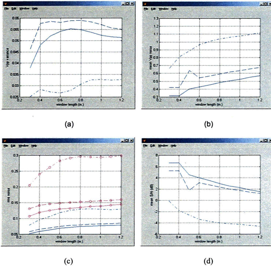
Figure 2.31 Eighth parametric evaluation of the influence of noise on bobbin coil data from mock-up test section of Fig. 2.18. Graphs show (a) variance of peak-to-peak ( V_{pp} ) noise, (b) mean value of V_{pp} noise, (c) vertical component and total (circles) RMS noise, and (d) mean value of S/N in dB, all as a function of window length. Results are shown for processed channel data without (solid curves) and with random (dashed curves) and composite (dash-dot curves) noise. A fixed segment length of \approx 46 mm (1.8 in) was used in all cases. The region of interest started outside the flaw signal (inner markings in Fig. 2.18) on both sides of the indication.
