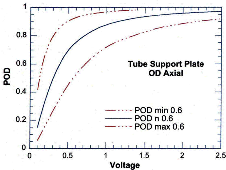
Figure 3.24 Range of probabilities of detection expected for a given voltage for log-normal noise with a mean value of 0.6 V.
