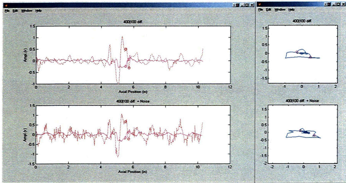
Figure 3.15 Eddy current data collected with bobbin coil from test section #15 with flaw at TSP intersection. Graphics show representative display of data in strip chart (left) and lissajous (right) format without (top) and with (bottom) simulated composite noise consisting of a small random and a periodic component.
