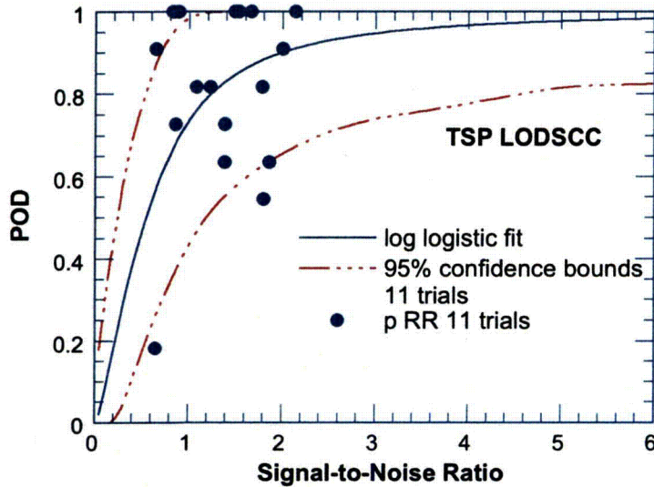
Figure 3.19 Solid dots show probability of detection measured for round-robin (number of hits/11 trials). Solid curve shows log-logistic fit for POD based on round-robin data. Chain-dot curves show estimated bounds (95th percentile) on the expected values of POD obtained in 11 trials if the true binomial POD is given by the log-logistic fit.
