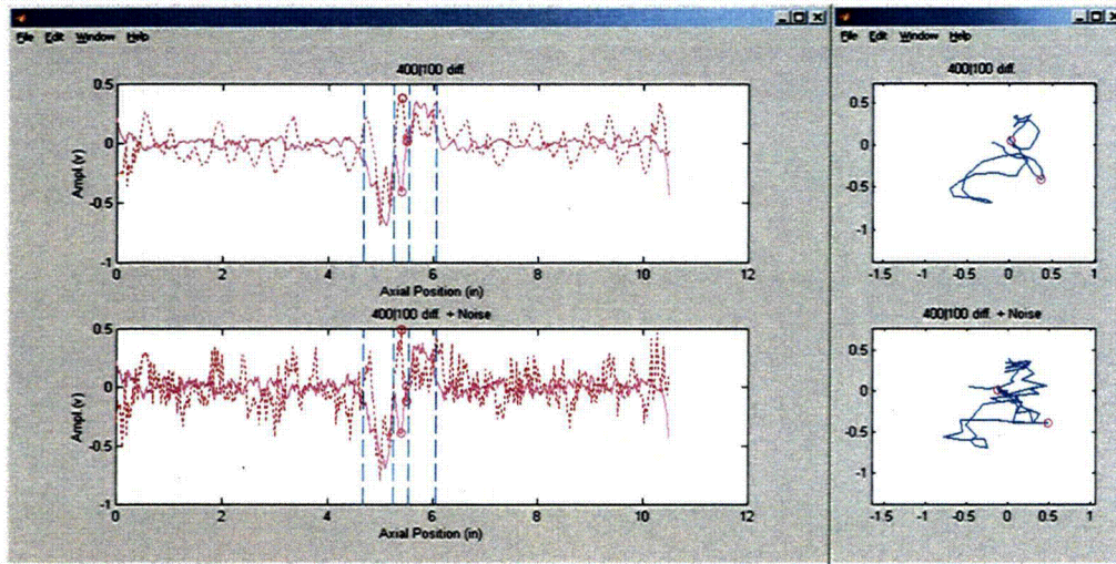
Figure 2.11 Second evaluation of the influence of noise on bobbin coil data from mock-up test section #1 with ODSCC indication at a TSP intersection. Graphics show the processed channel data without (top) and with (bottom) the added noise. Also shown are the inner and outer markings that identify the approximate location of flaw and TSP ends, respectively. Random noise with an amplification factor of 1 was added proportionally to both channels and to every data point.
