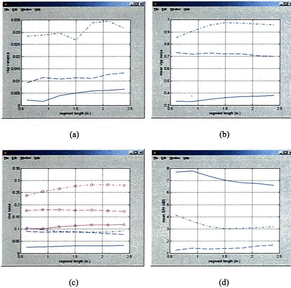
Figure 2.32 Parametric evaluation of the influence of noise on bobbin coil data from mock-up test section of Fig. 2.23. Graphs show (a) variance of peak-to-peak ( V_{pp} ) noise, (b) mean value of V_{pp} noise, (c) vertical component and total (circles) RMS noise, and (d) mean value of S/N in dB, all as a function of segment length. Results are shown for processed channel data without (solid curves) and with random (dashed curves) and composite (dash-dot curves) noise. A fixed window length of \approx 15 mm (0.6 in) was used in all cases. The region of interest started outside the TSP edge (outer markings in Fig. 2.23) on both sides of the indication.
