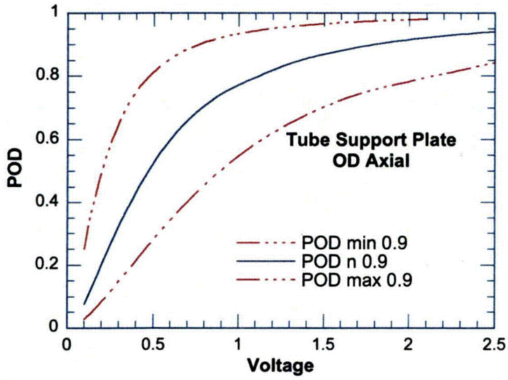
Figure 3.25 Range of probabilities of detection expected for a given voltage for log-normal noise with a mean value of 0.9 V.
