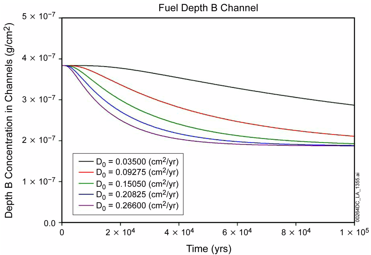
Figure 2.3.11-17. Integrated Waste to the Biosphere Depth in Channels Versus Time for Various Channel Diffusivity Values
