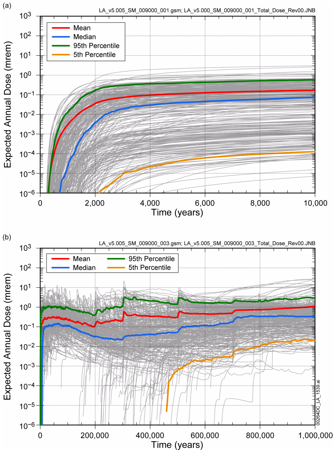
Figure 2.4-25. Distribution of Expected Annual Dose for the Seismic Ground Motion Modeling Case for (a) 10,000 Years and (b) 1 Million Years after Repository Closure
