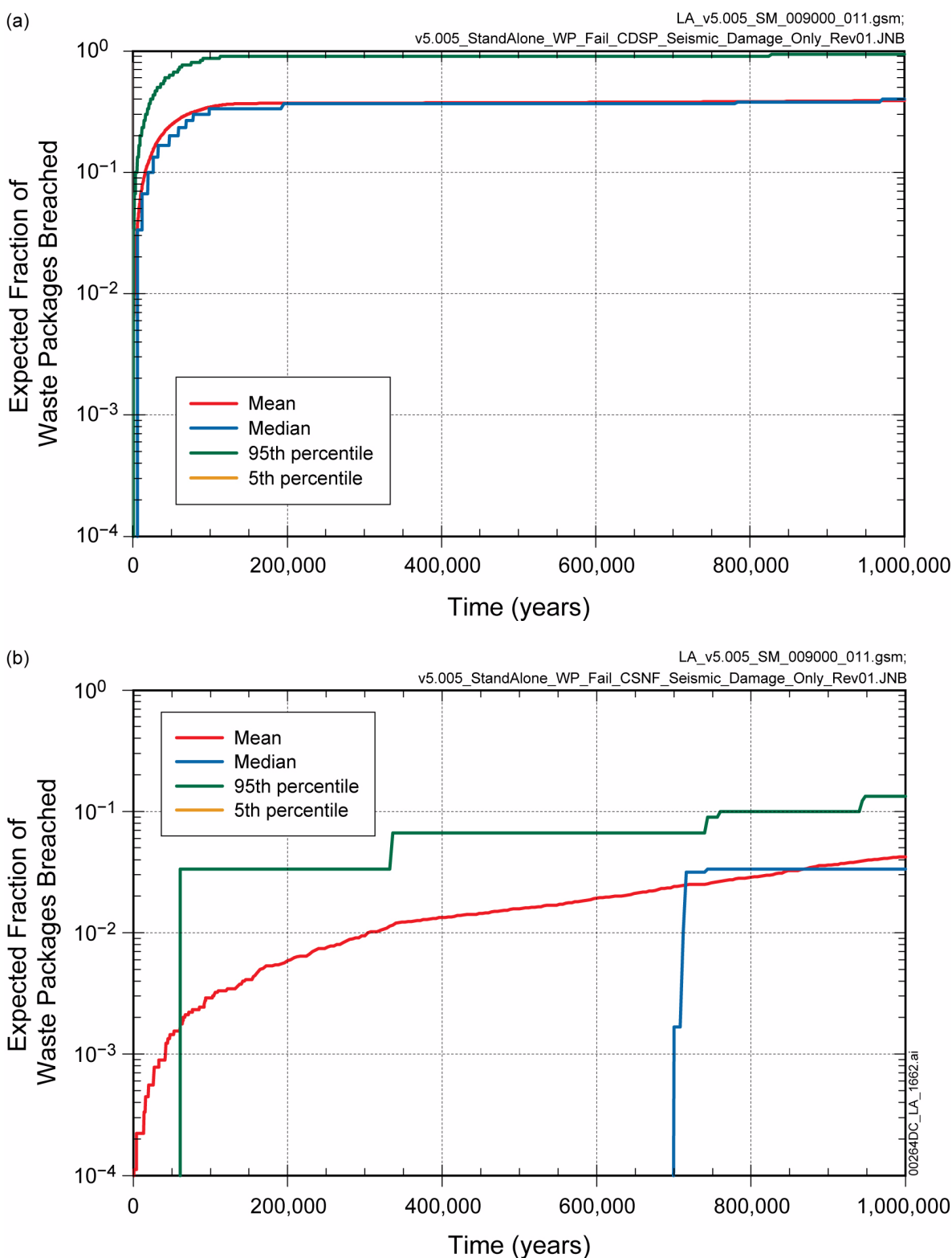
Figure 2.4-19. Expected Fraction of (a) Codisposal Waste Packages Failed and (b) Commercial SNF Waste Packages Failed by Seismic Damage for Percolation Subregion 3
