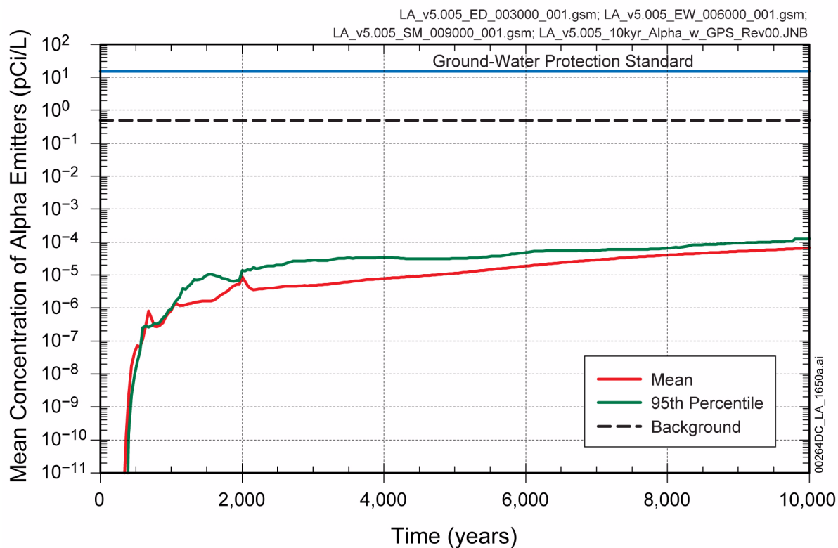
Figure 2.4-13. Summary Statistics for Activity Concentration of Gross Alpha (Including ^{226}\text{Ra} but Excluding Radon and Uranium) in Groundwater for 10,000 Years after Repository Closure
