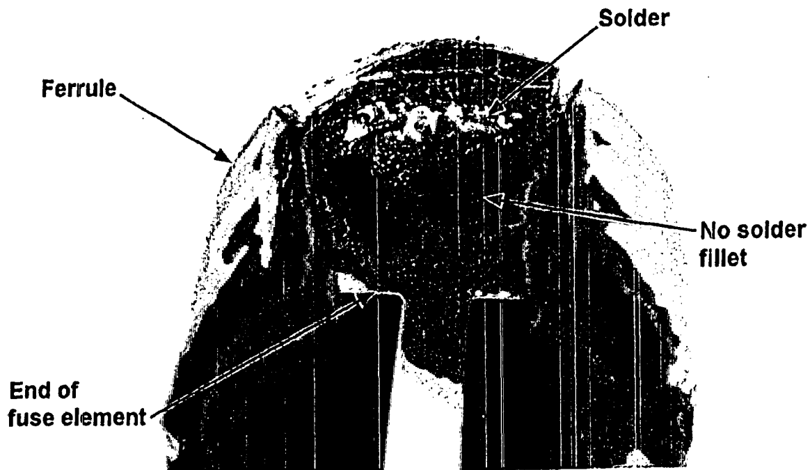
Figure 2: Detailed view of bad solder joint in failed fuse.
