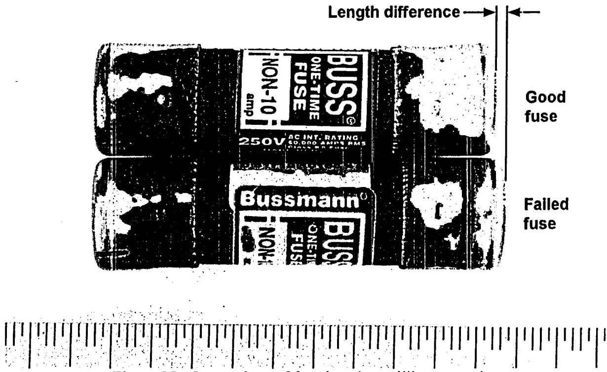
Figure 1: Difference in length between good fuse and failed fuse (millimeter scale).
