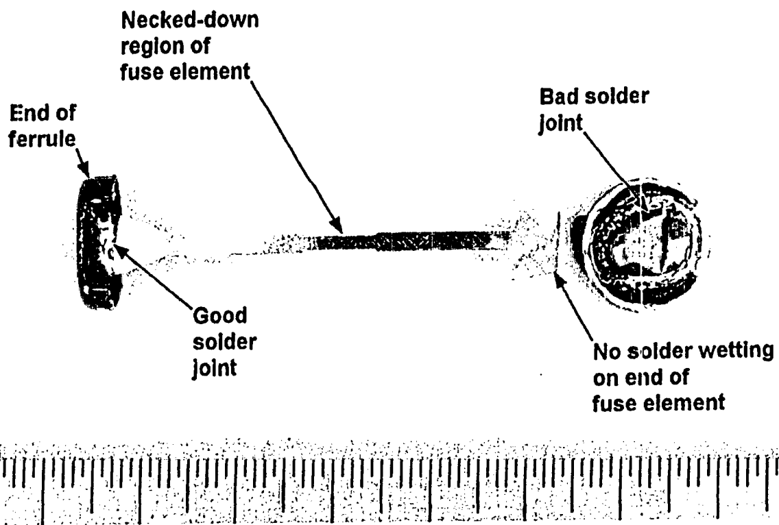
Figure 3: Failed fuse with fiber tube and most of ferrules removed (millimeter scale).
