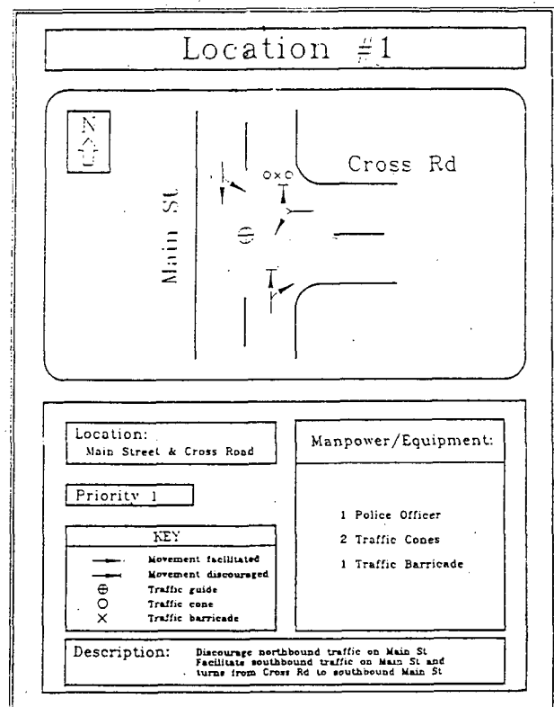
Figure 1. Traffic management diagram.
