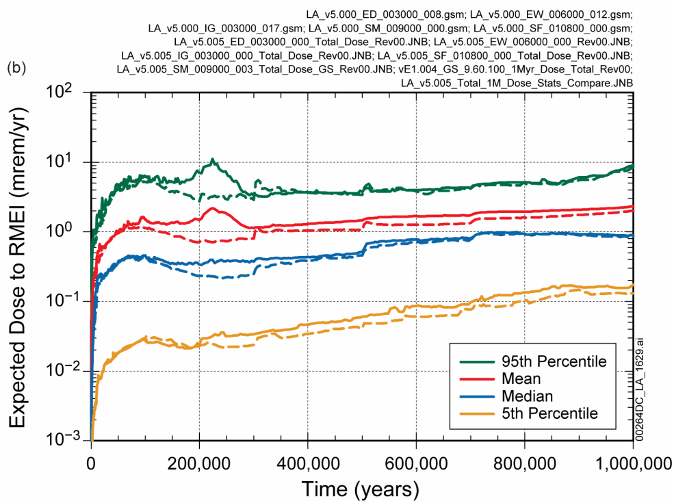
Figure 2.4-111. Comparison of Statistics for Total Expected Annual Dose over between TSPA Model v5.000 and TSPA Model v5.005 (a) 20,000 Years and (b) 1 Million Years after Repository Closure
