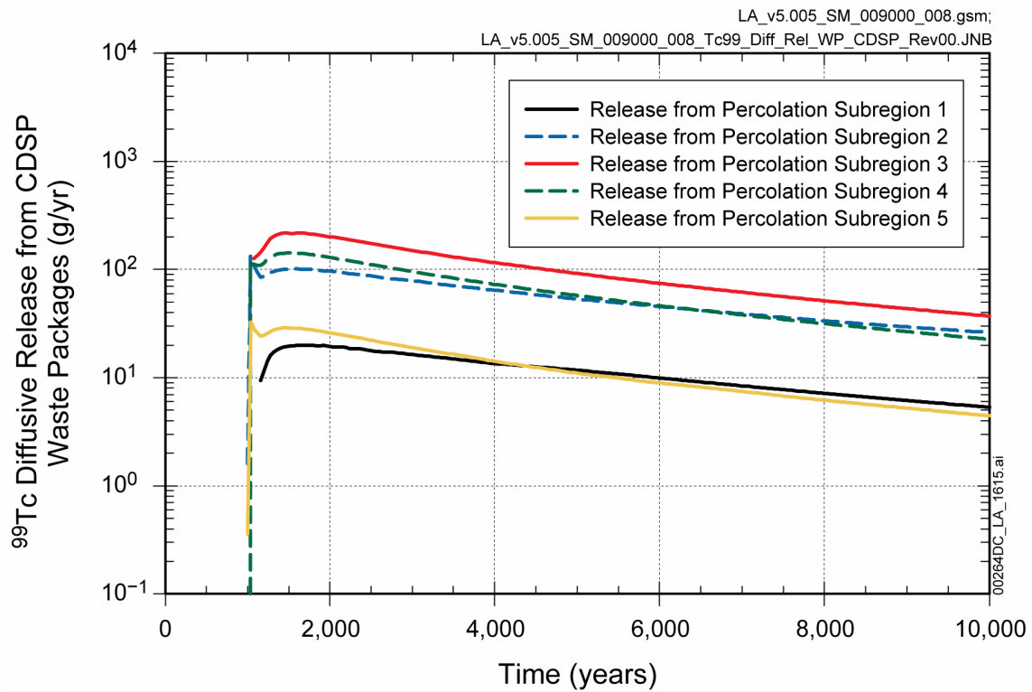
Figure 2.4-78. Diffusive Release Rates of 99 Tc from Codisposal Waste Packages from Each Percolation Subregion for Realization 4,628 of the Seismic Ground Motion Modeling Case for the 10,000-Year Period after Repository Closure
