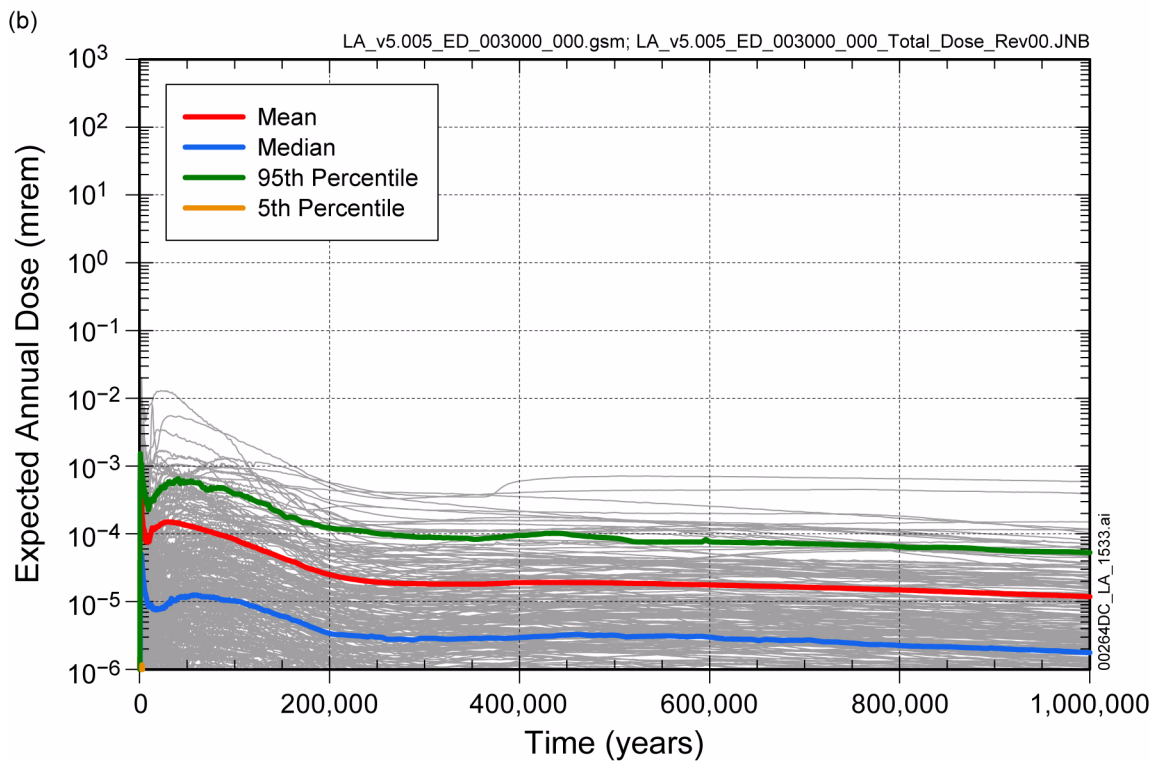
Figure 2.4-33. Distribution of Expected Annual Dose for the Drip Shield Early Failure Modeling Case for (a) 10,000 Years and (b) 1 Million Years after Repository Closure
