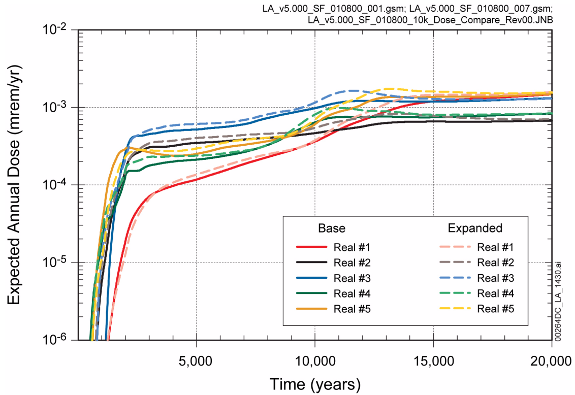
Figure 2.4-61. Expected Annual Dose over 20,000 Years for Seismic Fault Displacement Modeling Case Considering Additional Specified Event Times and Damage Areas
