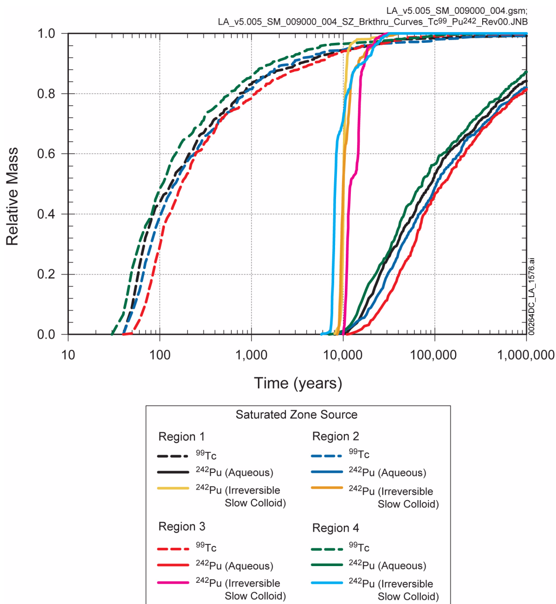
Figure 2.4-109. Comparison of Saturated Zone Breakthrough Curves for ^{99}\text{Tc} and ^{242}\text{Pu} for All Four Saturated Zone Source Regions for Realization 4,641 of the Seismic Ground Motion Modeling Case for the 1-Million-Year Period after Repository Closure
