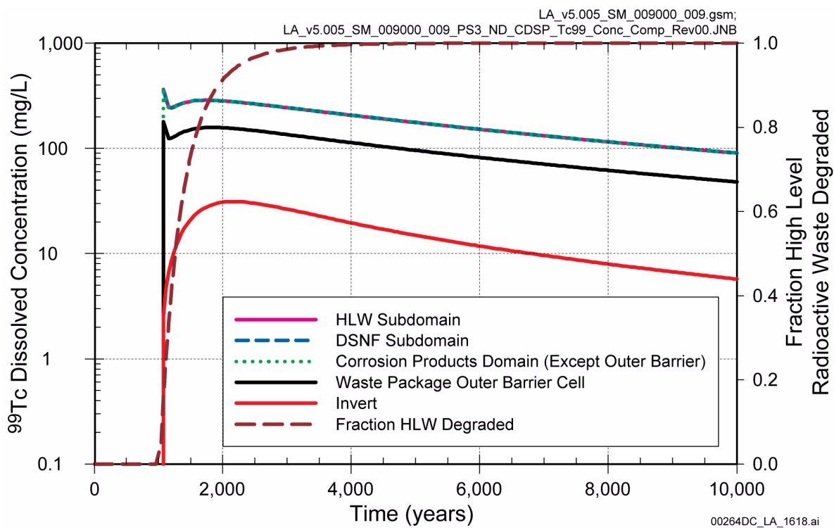
Figure 2.4-81. Comparison of Dissolved Concentration of 99 Tc from the Various Engineered Barrier System Transport Domains and Fraction of HLW Degraded for Codisposal Perculation Subregion 3, Nonseeping Environment for Realization 4,628 of the Seismic Ground Motion Modeling Case for the 10,000-Year Period after Repository Closure
