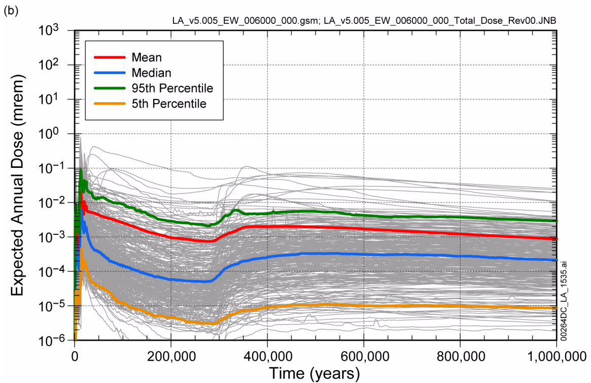
Figure 2.4-35. Distribution of Expected Annual Dose for the Waste Package Early Failure Modeling Case for (a) 10,000 Years and (b) 1 Million Years after Repository Closure
