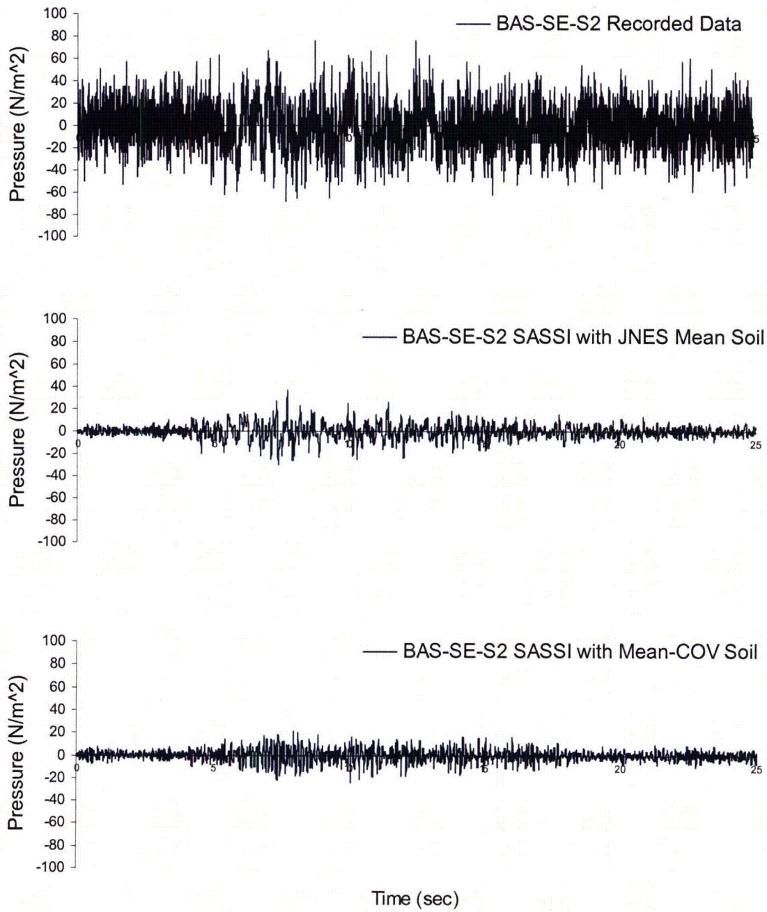
Figure 3.1-9 Comparison of Seismic Induced Soil Pressure at Sensor BAS-SE-S2
