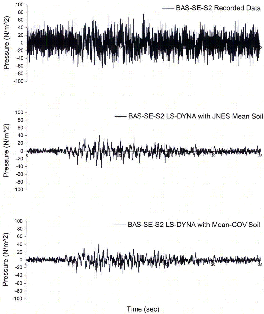
Figure 4.1-6 Comparison of Seismic Induced Soil Pressure at Sensor BAS-SE-S2
