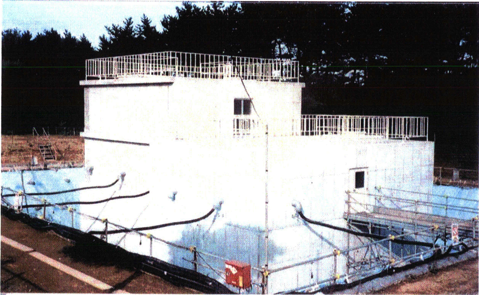
Figure 2-8 NUPEC Field Test Model of Adjacent Reactor -Turbine Buildings without Embedment
