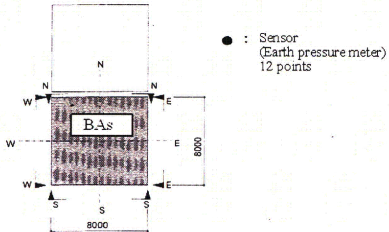
Figure 2-18 Locations of Pressure Sensors for the BAs Structure on Side Wall [unit: mm]
