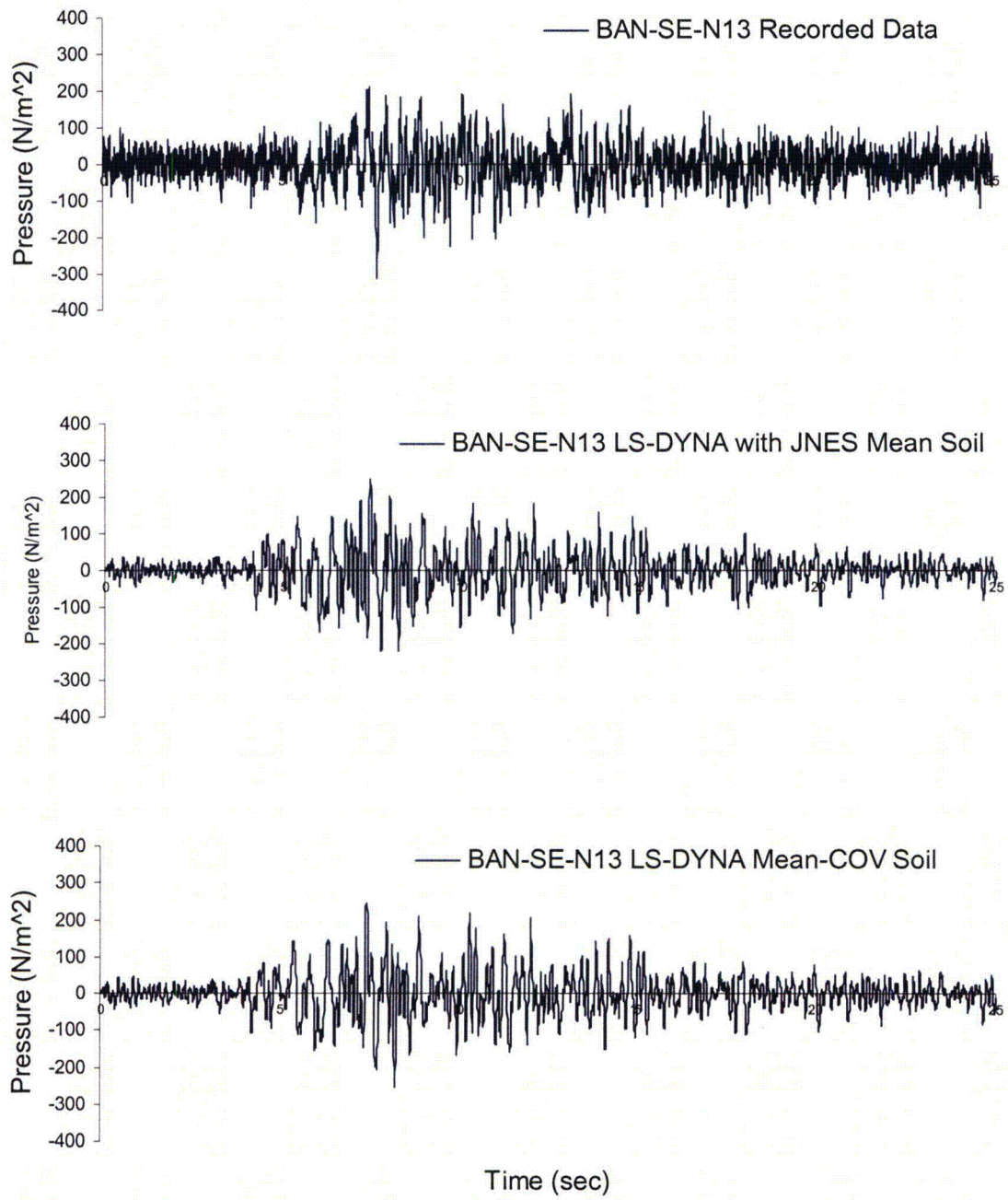
Figure 4.1-10 Comparison of Seismic Induced Soil Pressure at Sensor BAN-SE-13
