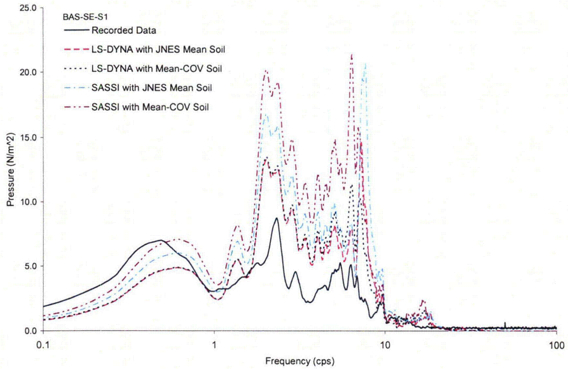
Figure 4.3-3 Comparison of Fourier Spectra of Soil Pressure at Sensor BAS-SE-S1 of Twin Reactors Model between LS-DYNA and SASSI
