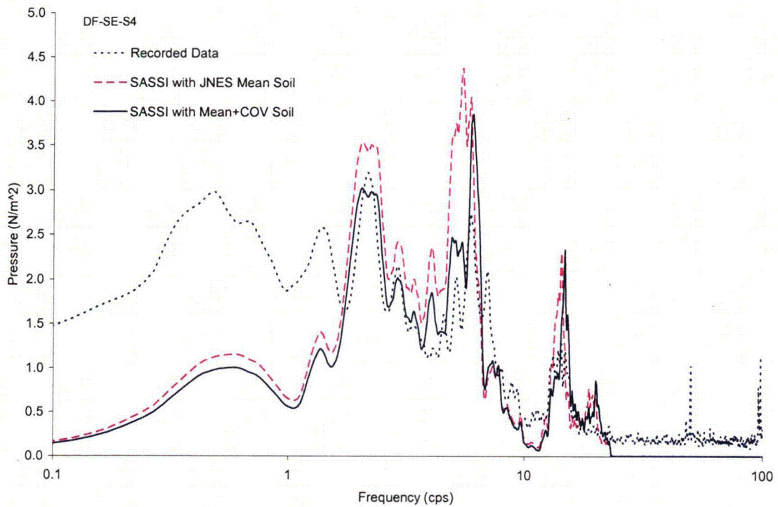
Figure 3.2-22 Comparison of Fourier Spectra of Soil Pressure at Sensor DF-SE-S4
