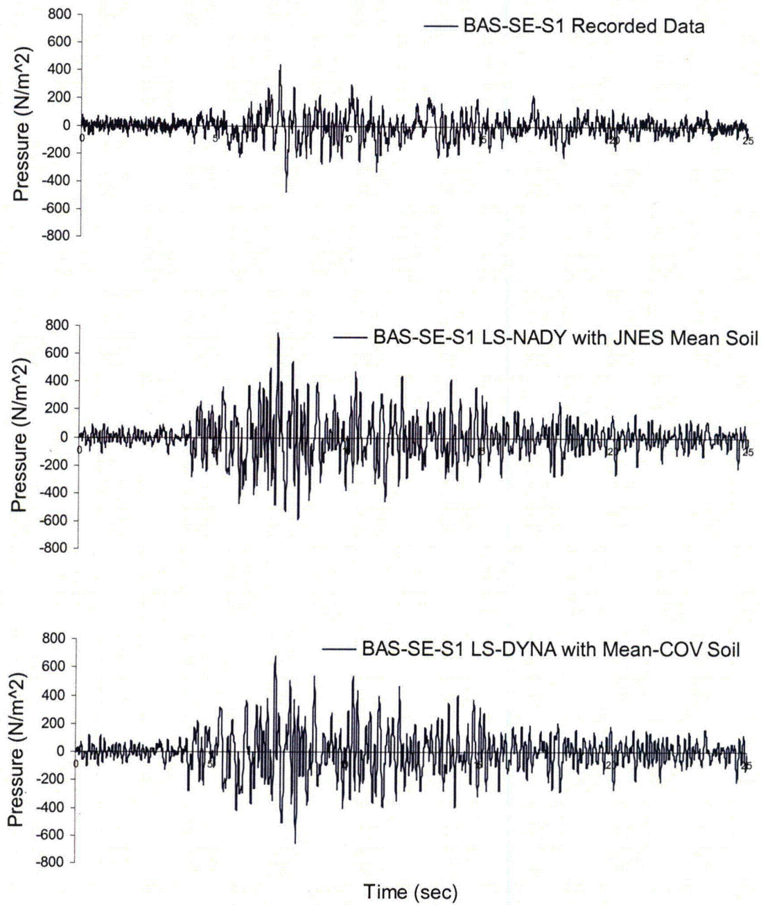
Figure 4.1-5 Comparison of Seismic Induced Soil Pressure at Sensor BAS-SE-S1
