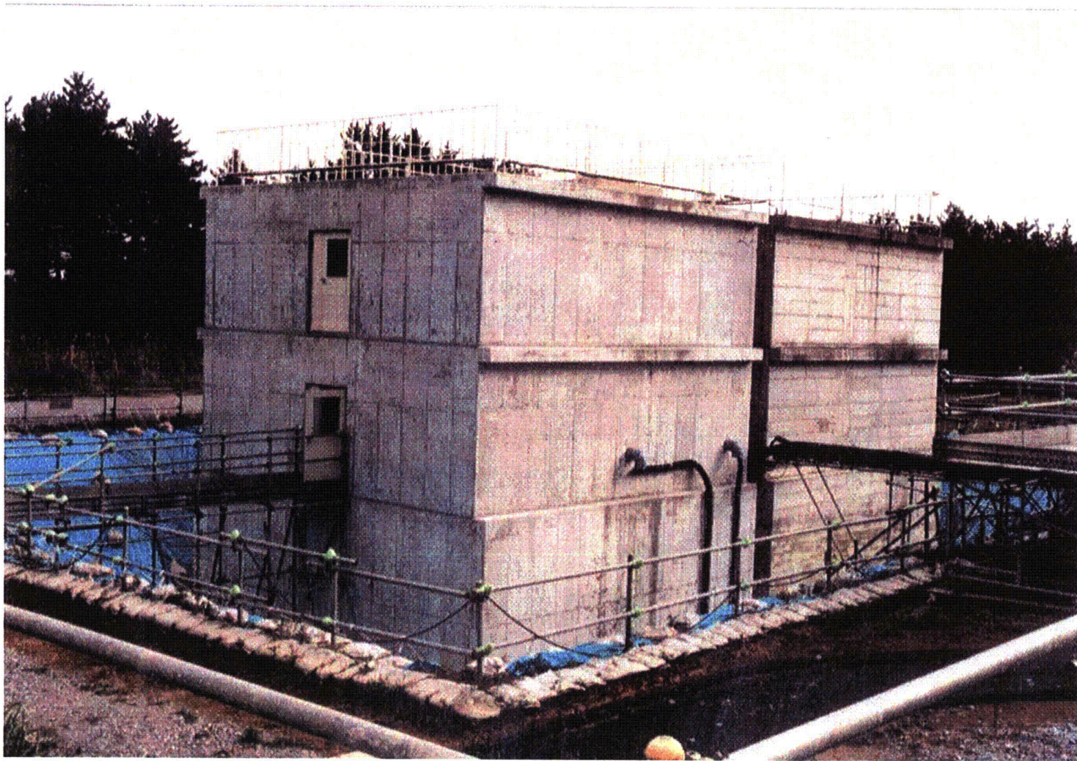
Figure 2-7 NUPEC Field Test Model of Adjacent Twin Reactor Buildings without Embedment
