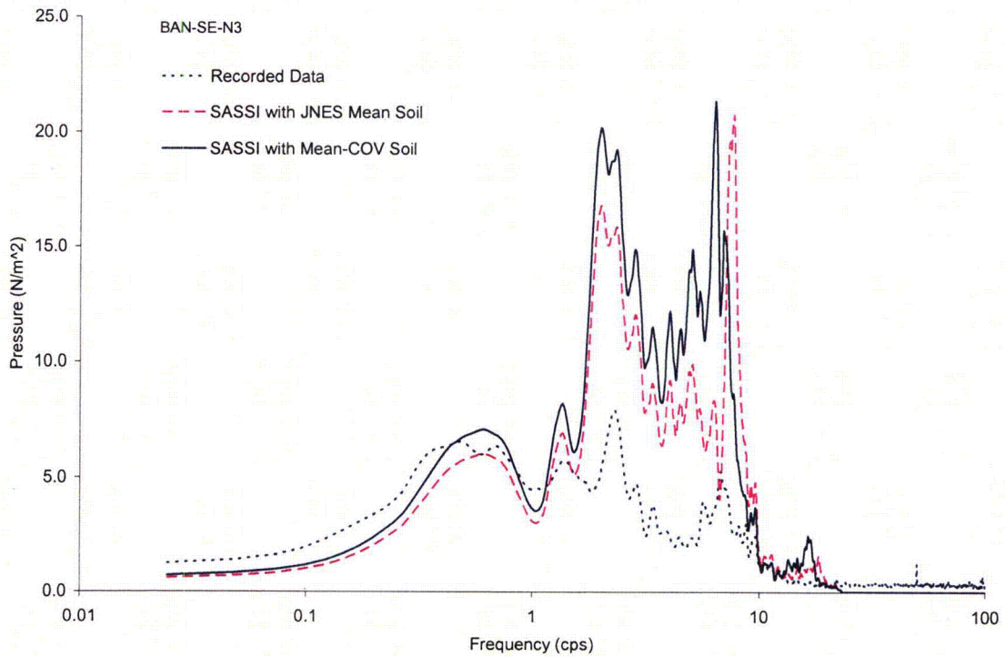
Figure 3.1-17 Comparison of Fourier Spectra of Soil Pressure at Sensor BAN-SE-N3
