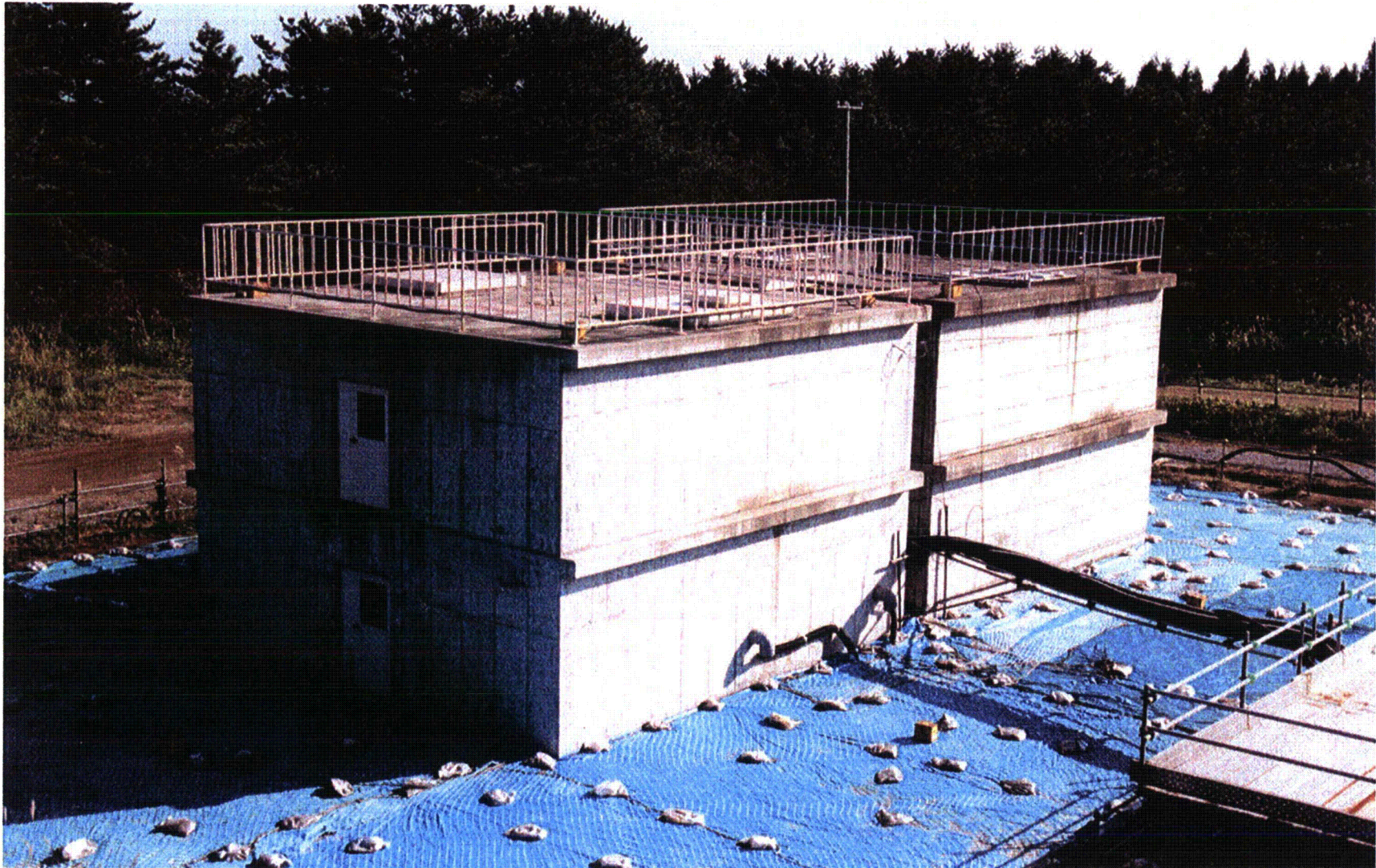
Figure 2-10 NUPEC Field Test Model of Adjacent Twin Reactor Buildings with Embedment
