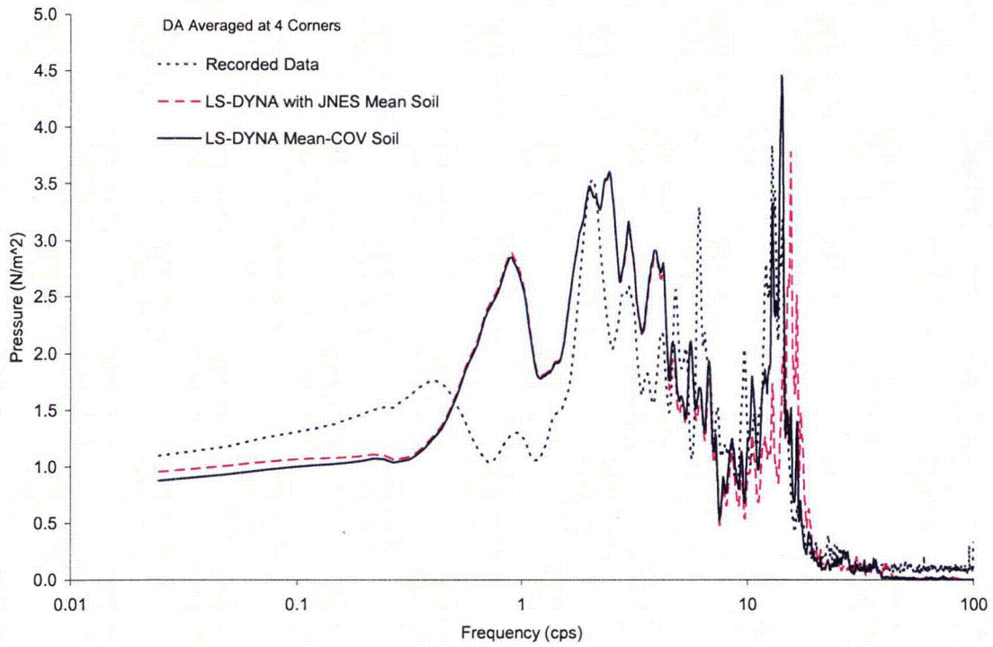
Figure 4.2-25 Comparison of Fourier Spectra for Vertical Soil Pressure on Basemat of R-T Reactor
