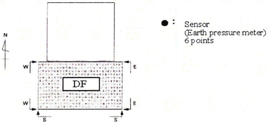
Figure 2-21 Locations of Pressure Sensors for the DF Structure on Side Wall [unit: mm]
