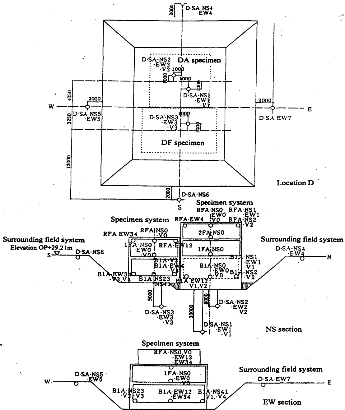
Location of seismometer of DA,DF specimen
