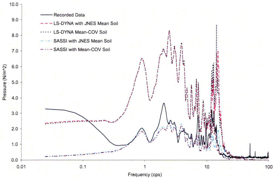
Figure 4.3-12 Comparison of Fourier Spectra of Vertical Soil Pressure on BAS Basemat of Twin Reactors Model
