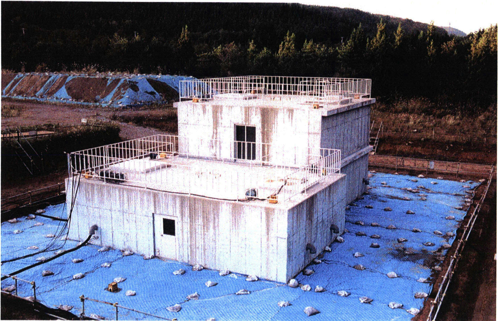
Figure 2-11 NUPEC Field Test Model of Adjacent Reactor-Turbine Buildings with Embedment
