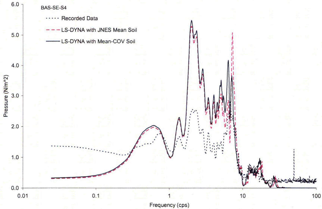
Figure 4.1-13 Comparison of Fourier Spectra of Soil Pressure at Sensor BAS-SE-S4
