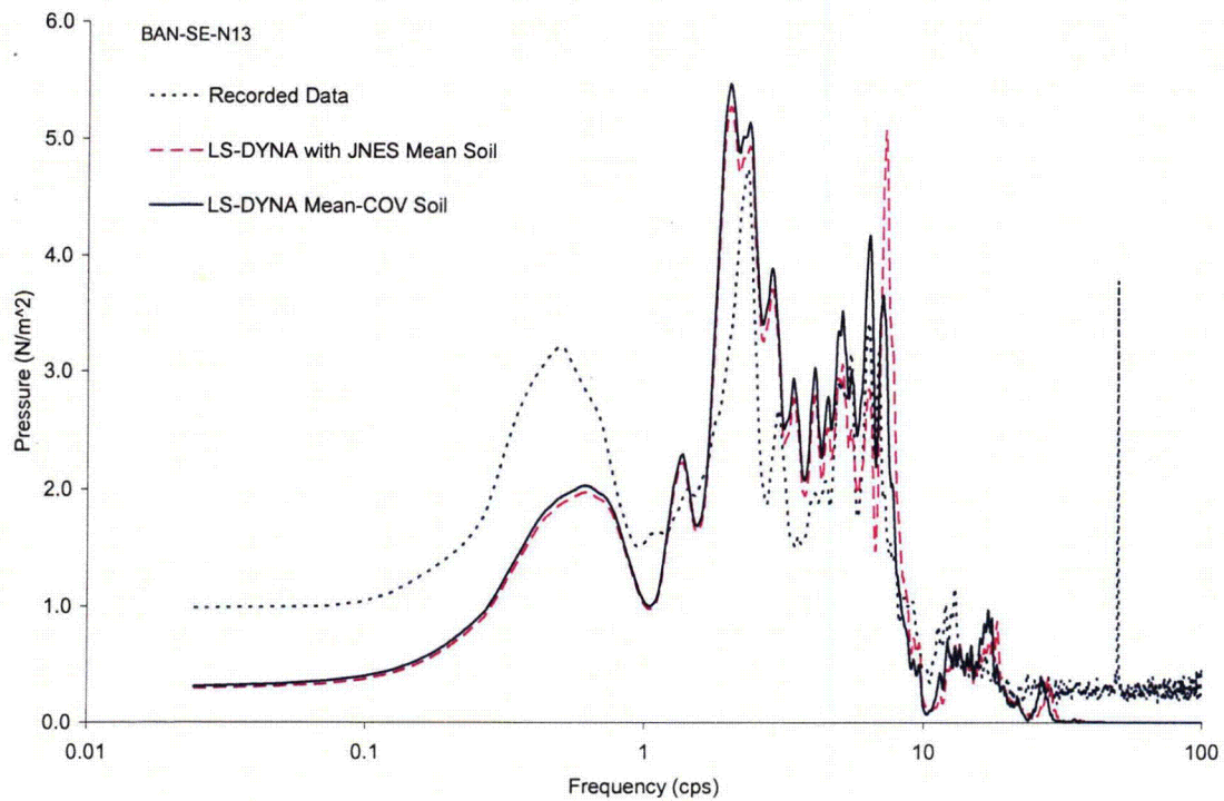
Figure 4.1-16 Comparison of Fourier Spectra of Soil Pressure at Sensor BAN-SE-N13
