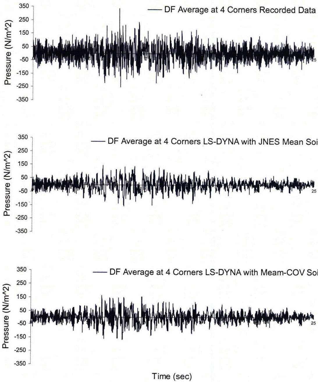
Figure 4.2-24 Comparison of Seismic Induced Vertical Soil Pressure on Basemat of R-T Turbine
