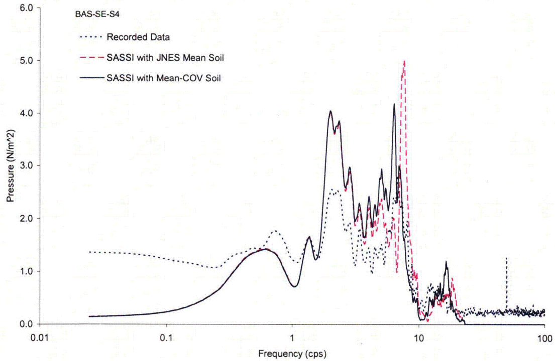
Figure 3.1-16 Comparison of Fourier Spectra of Soil Pressure at Sensor BAS-SE-S4
