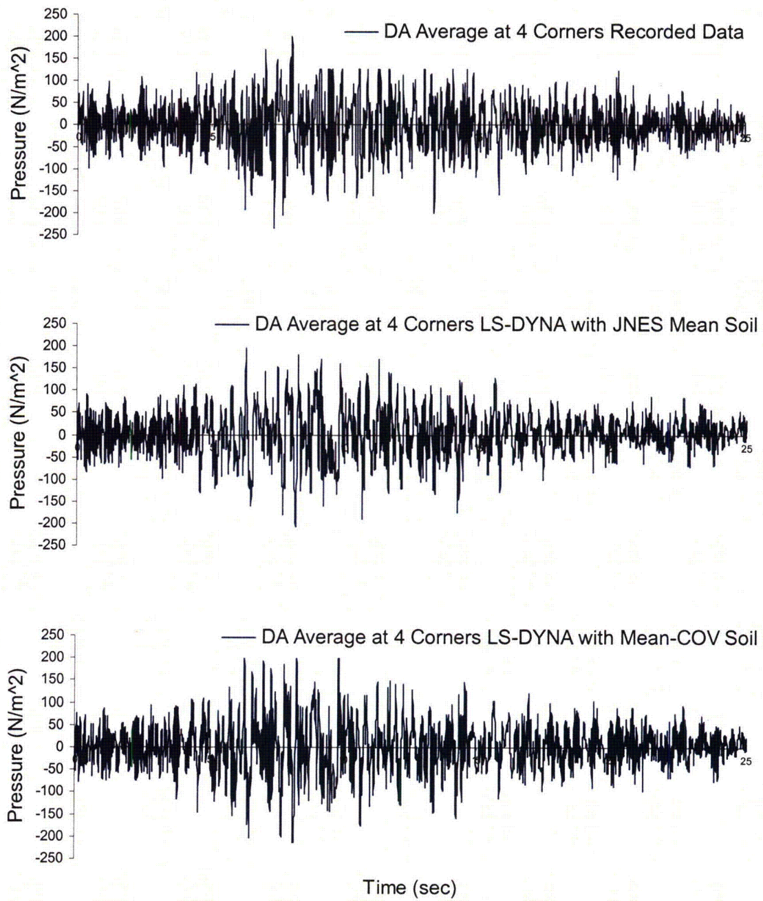
Figure 4.2-23 Comparison of Seismic Induced Vertical Soil Pressure on Basemat of R-T Reactor
