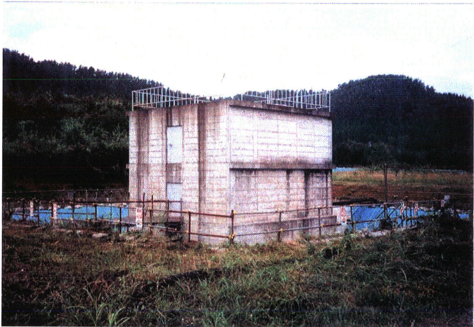
Figure 2-6 NUPEC Field Test Model of Reactor Building without Embedment
