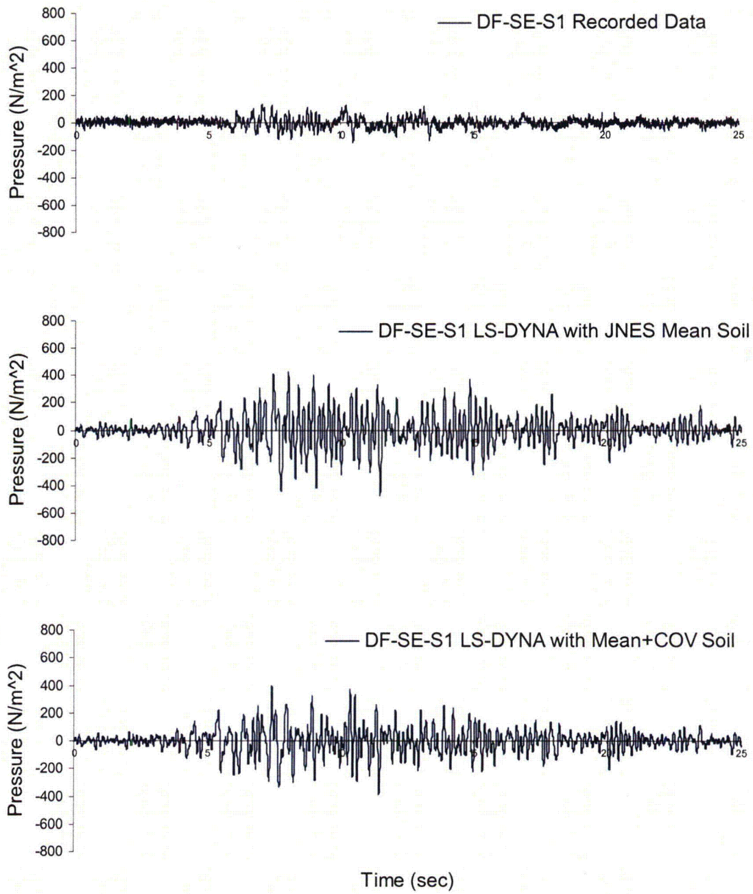
Figure 4.2-10 Comparison of Seismic Induced Soil Pressure at Sensor DF-SE-S1
