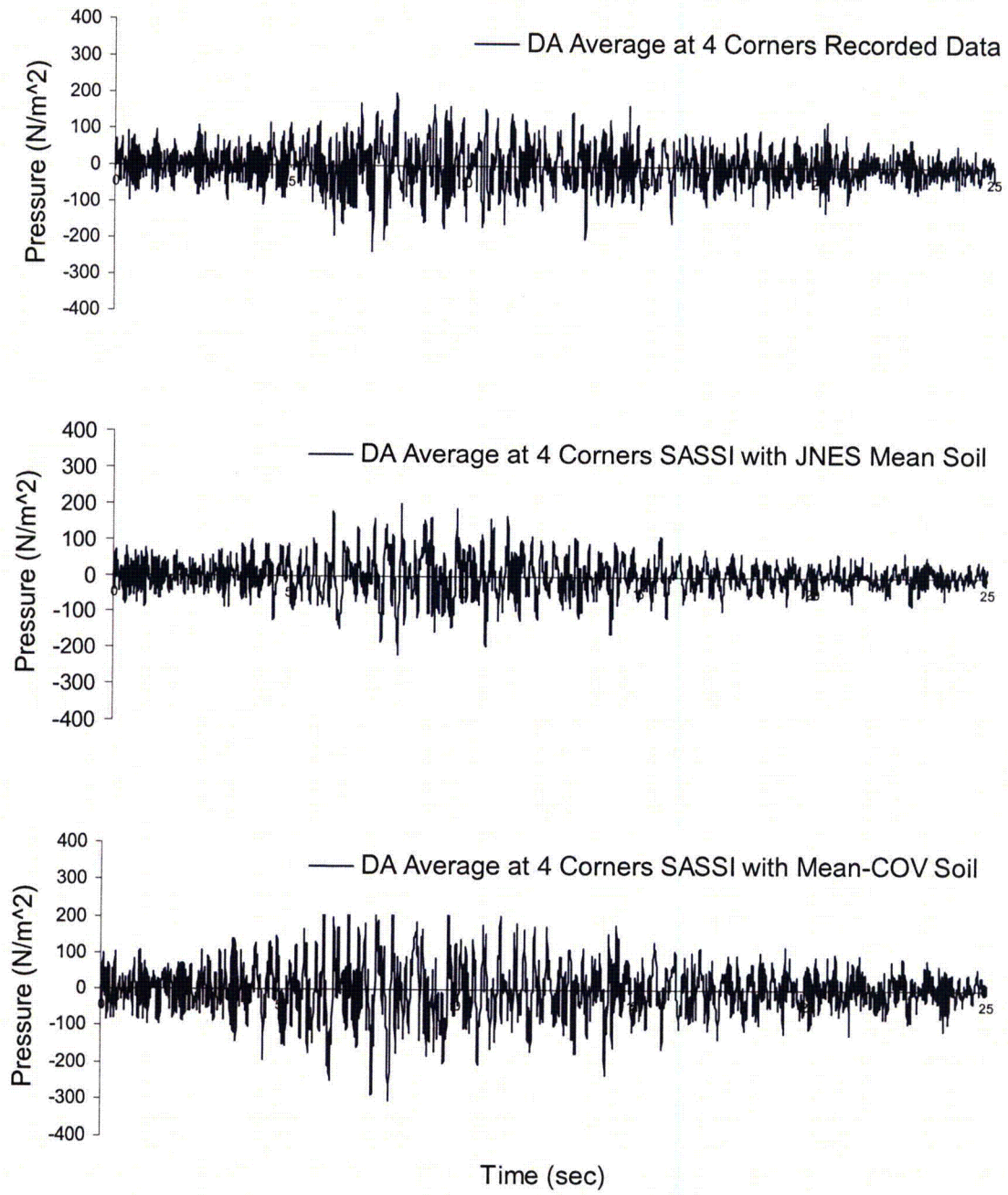
Figure 3.2-27 Comparison of Averaged Vertical Seismic Induced Soil Pressure for DA
