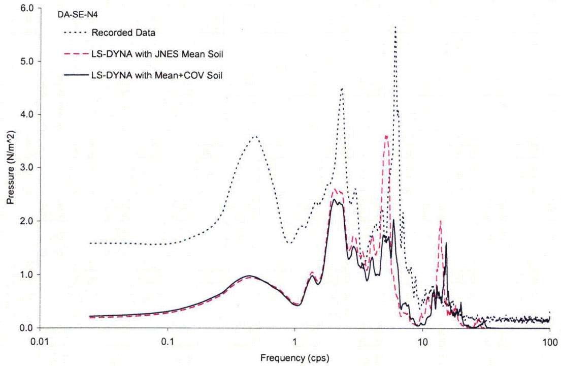
Figure 4.2-15 Comparison of Fourier Spectra of Soil Pressure at Sensor DA-SE-N4
