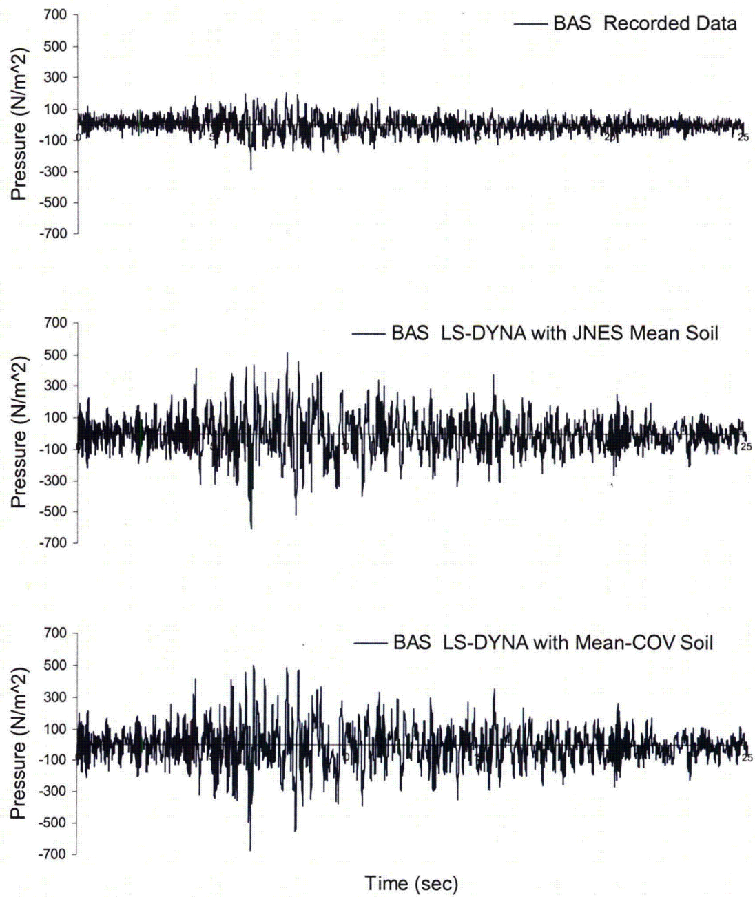
Figure 4.1-20 Comparison of Vertical Soil Pressure on BAS Basemat of Twin Reactors Model
