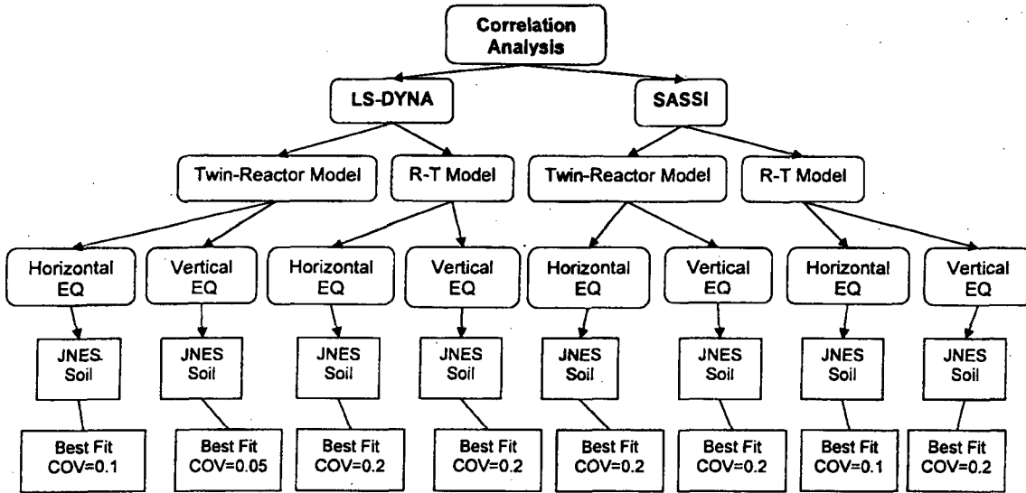
Figure 4.3-13 Summary of Analytical Cases and Associated Soil Uncertainties Performed for this Report
