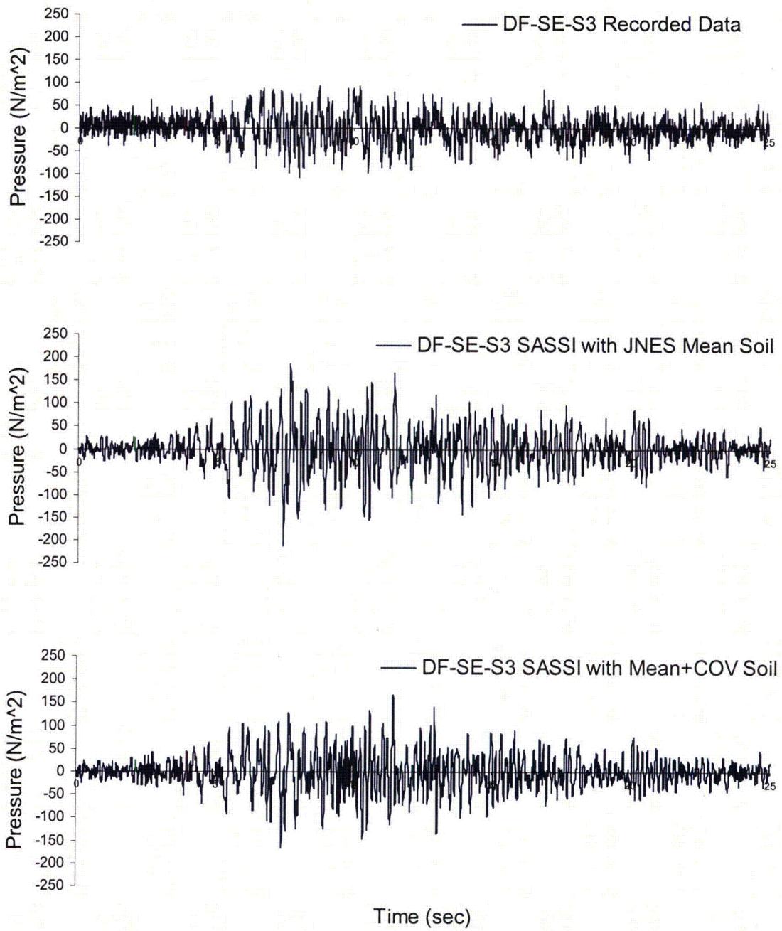
Figure 3.2-15 Comparison of Seismic Induced Soil Pressure at Sensor DF-SE-S3
