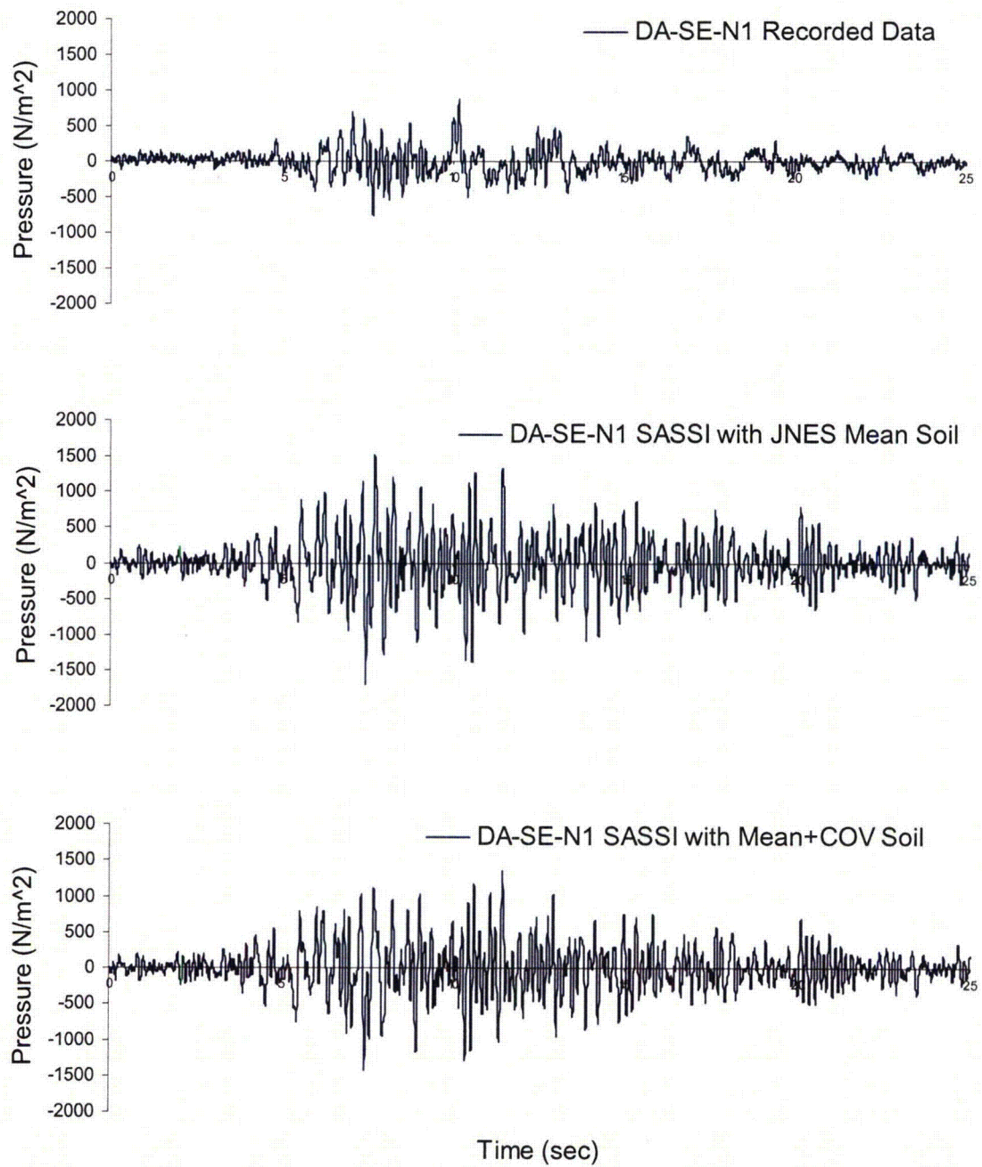
Figure 3.2-11 Comparison of Seismic Induced Soil Pressure at Sensor DA-SE-N1
