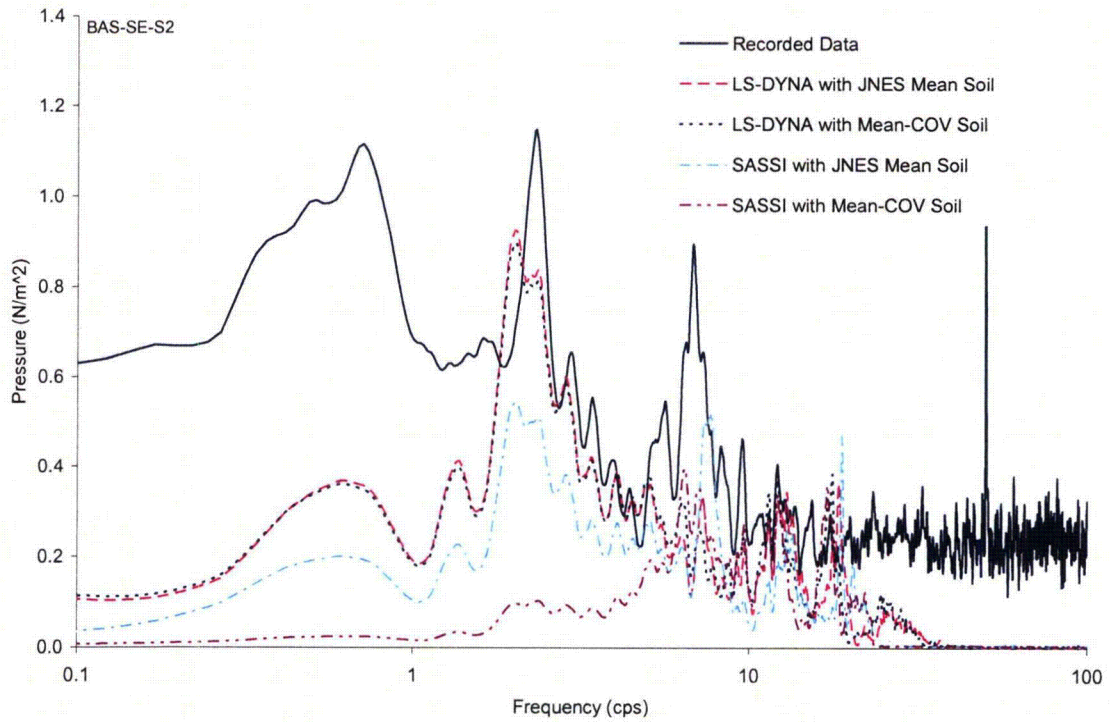
Figure 4.3-4 Comparison of Fourier Spectra of Soil Pressure at Sensor BAS-SE-S2 of Twin Reactors Model between LS-DYNA and SASSI
