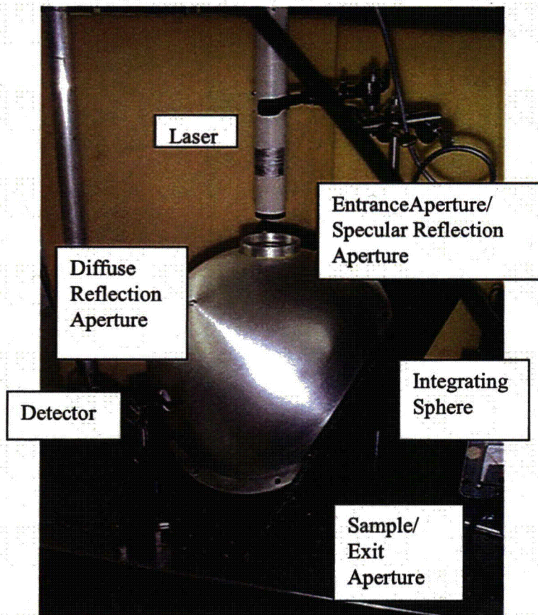
Figure 3.4 Experimental Setup for Specularity Measurements
