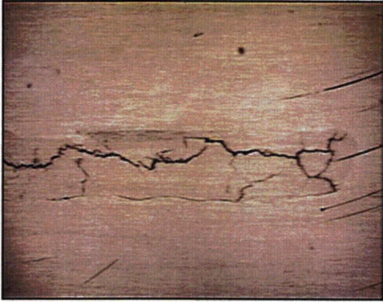
Figure B.157 - Sample 8 Diffuse On-Axis Lighting
