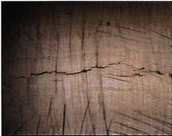
Figure B.187 - Sample 9 Diffuse On-Axis Lighting
