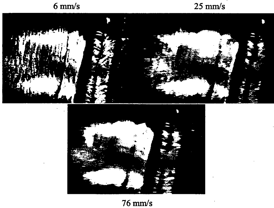
Figure 4.6 Sample Images of a 125-mm COD Crack Imaged at Three Scanning Speeds
