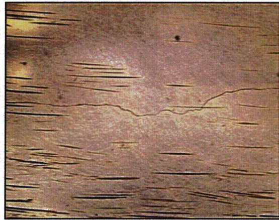
Figure B.128 - Sample 7 Diffuse Ring Lighting
