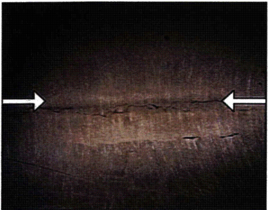
Figure B.107 - Sample 6 Spotlighting from Indicated Direction
