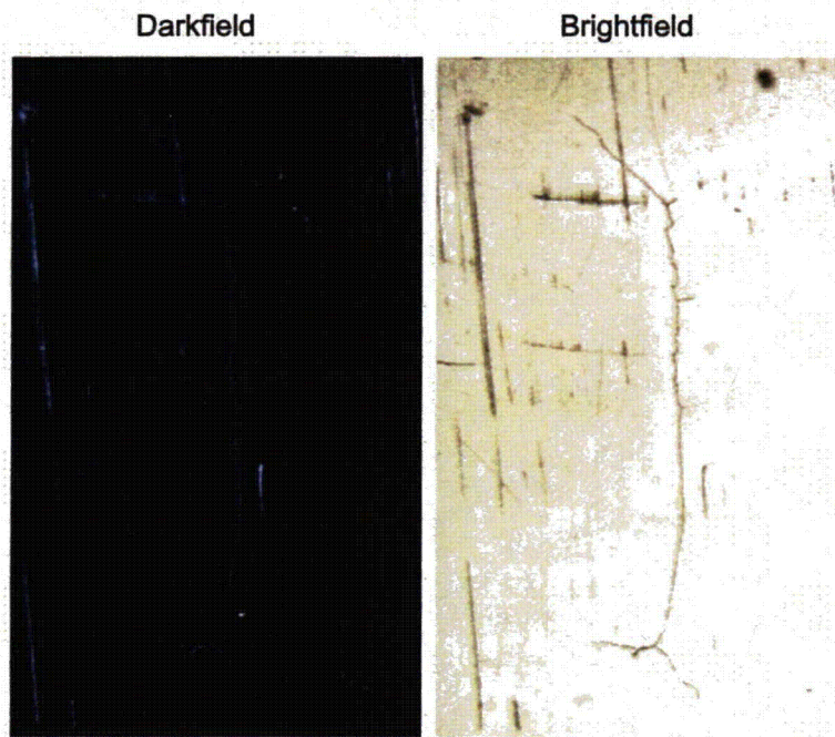
Figure 2.6 Crack with 12- \mu m Crack Opening Depth Imaged Using Both Darkfield and Brightfield Illumination
