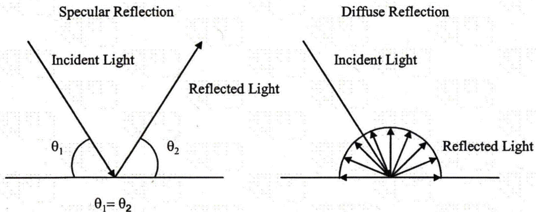
Figure 2.8 Specular and Diffuse Reflection. When light strikes a highly specular surface (left), the light is reflected away at the incident angle. When light strikes a diffusely reflecting surface (right), it reflects isotropically.
