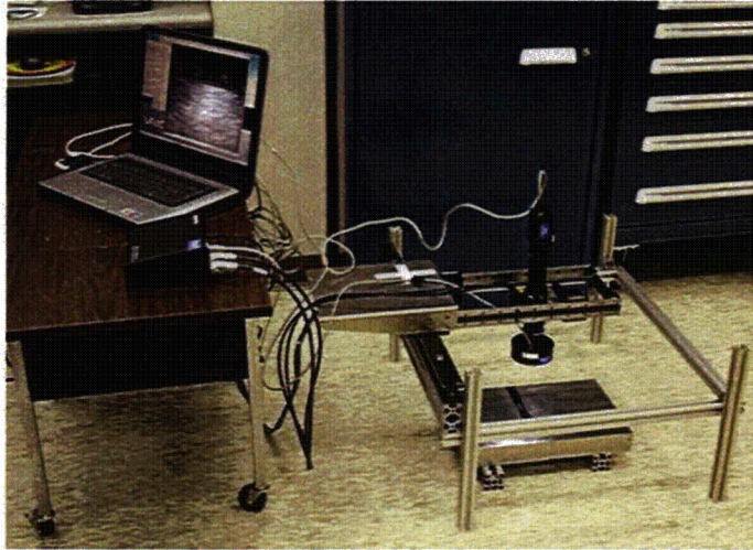
Figure 3.1 Visual Testing Apparatus and Sample
