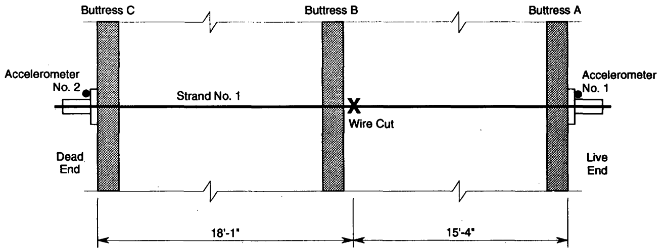
Accelerometer and Wire Cut Locations for Test No.'s 1, 2 and 3
