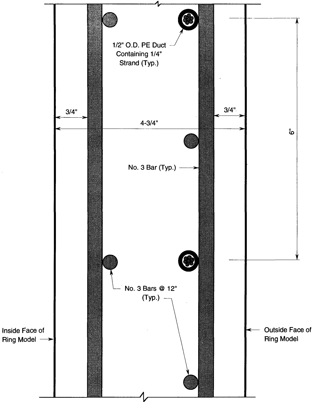
Figure 3. Reinforcement details.
