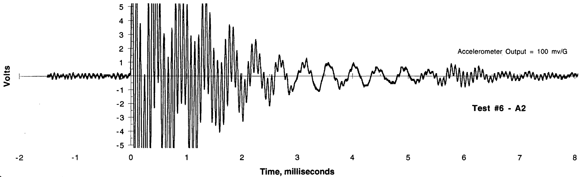
Figure 21. Time domain response of A1 and A2 in Test No. 6.
