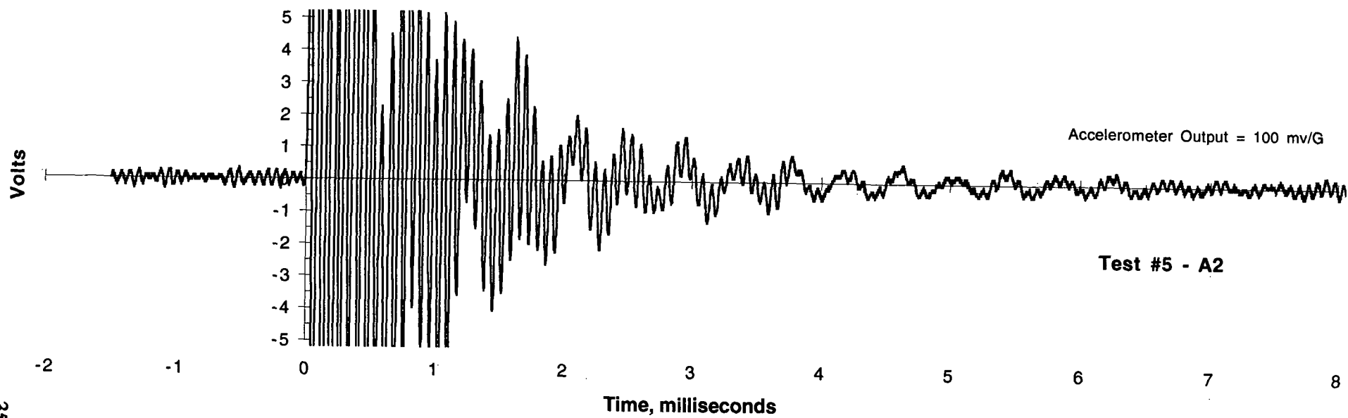
Figure 19. Time domain response of A1 and A2 in Test No. 5.
