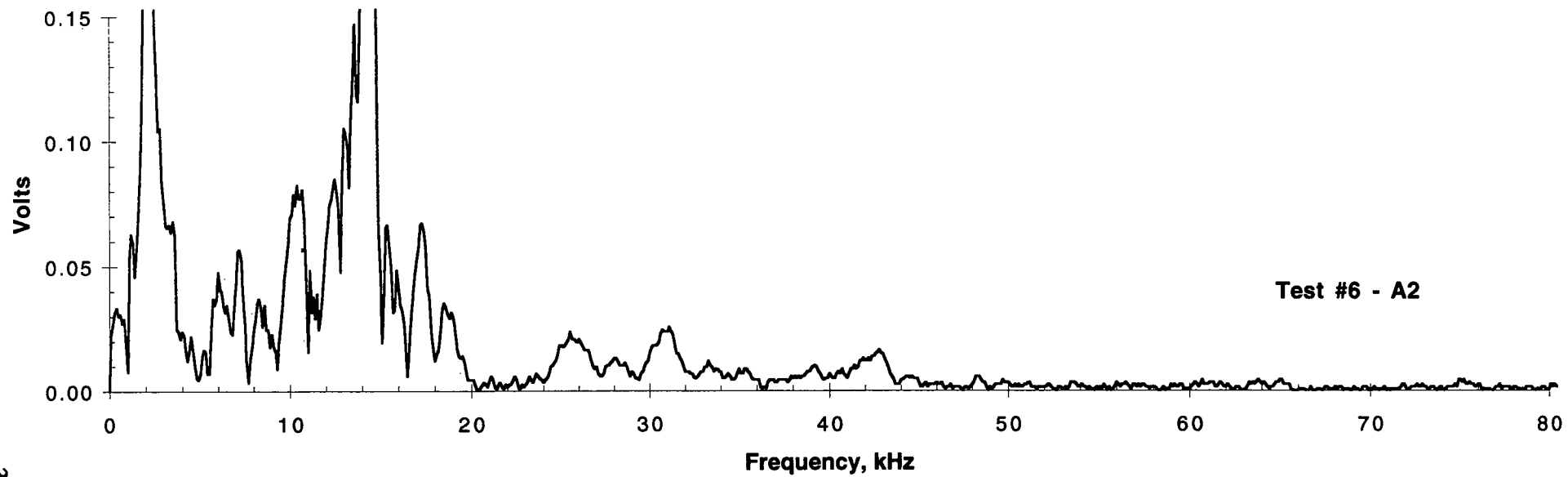
Figure 22. Frequency domain response of A1 and A2 in Test No. 6.
