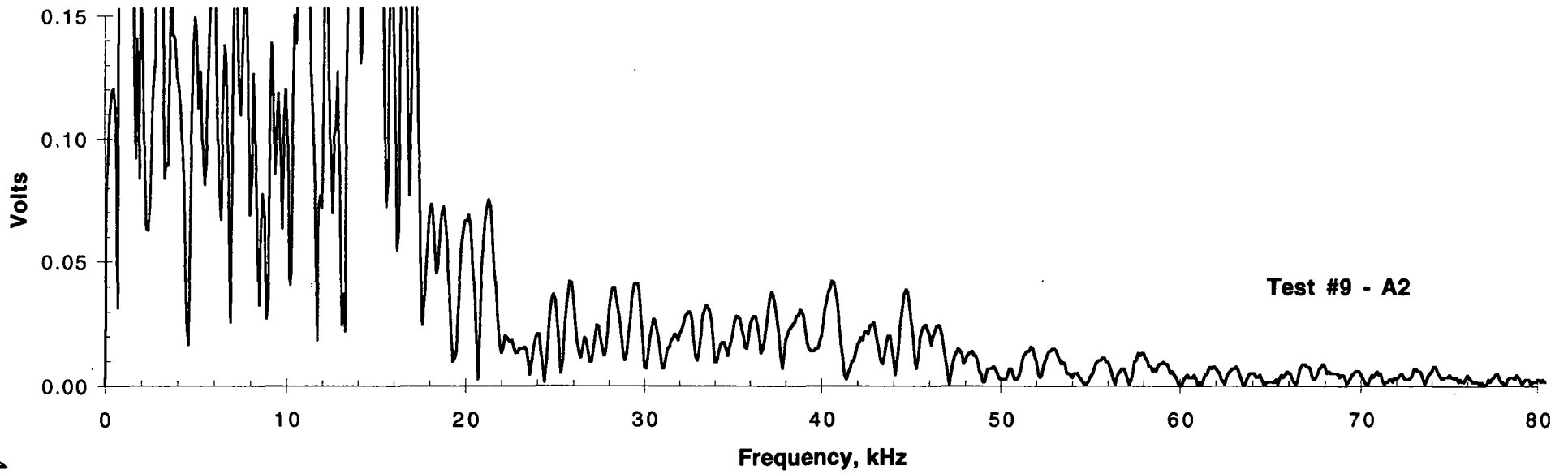
Figure 28. Frequency domain response of A1 and A2 in Test No. 9.
