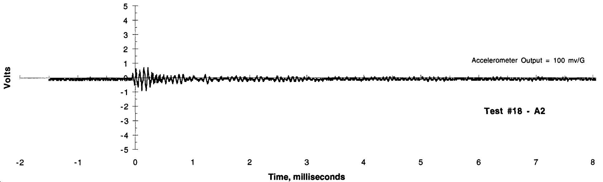
19 Figure 45. Time domain response of A1 and A2 in Test No. 18.
