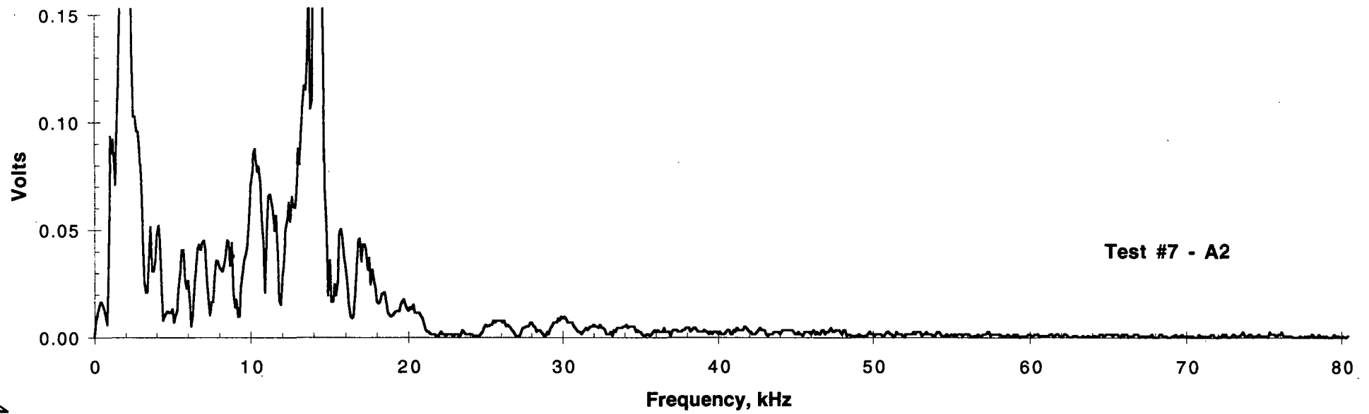
Figure 24. Frequency domain response of A1 and A2 in Test No. 7.
