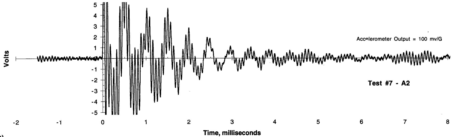
Figure 23. Time domain response of A1 and A2 in Test No. 7.
