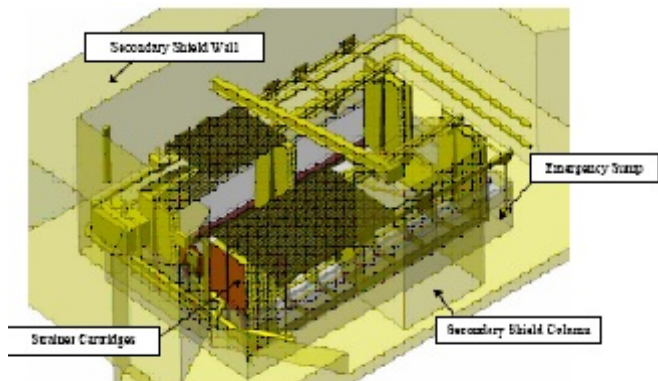
Figure 3 CCI Strainer Cartridge
