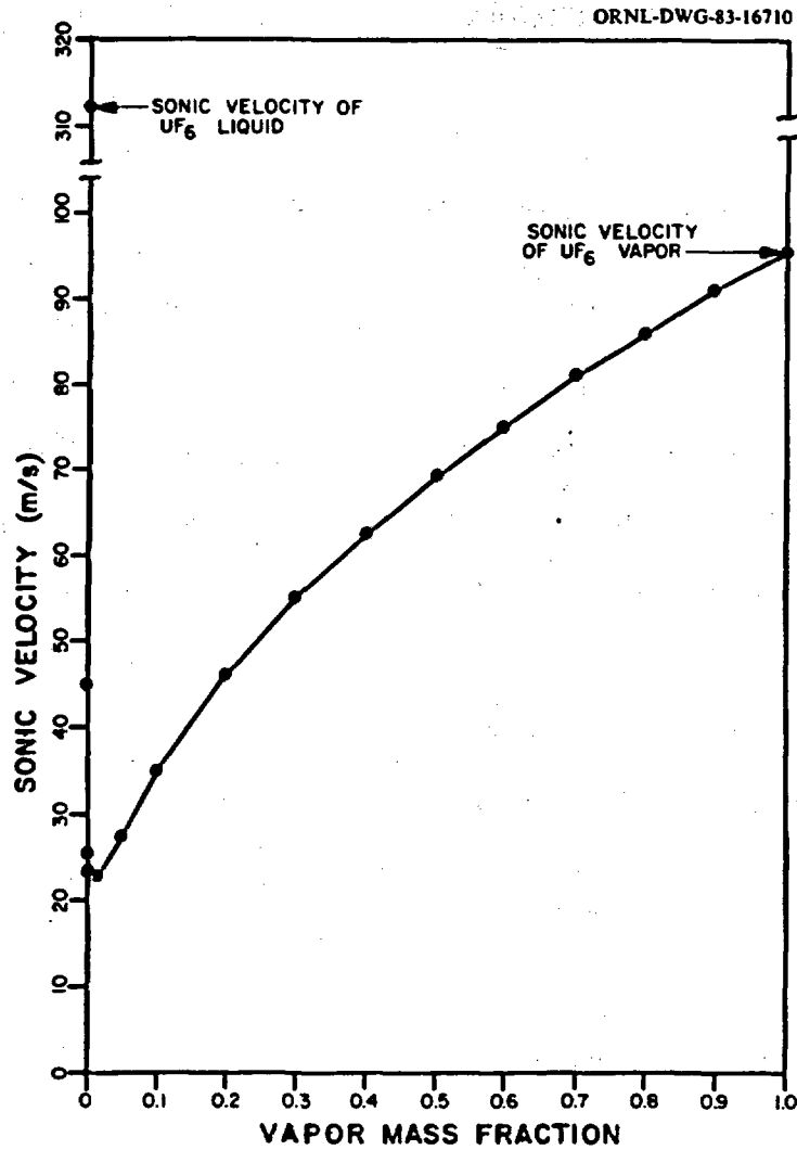
Fig. 15. Predicted sonic velocity as a function of vapor mass fraction for saturated \text{UF}_6 at 100^\circ\text{C} and 4.12 atm.
