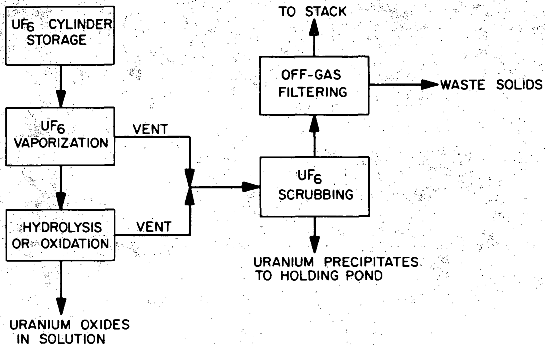
Fig. 5. Flow diagram for UF_6 handling operations at a typical fuel fabrication facility.
