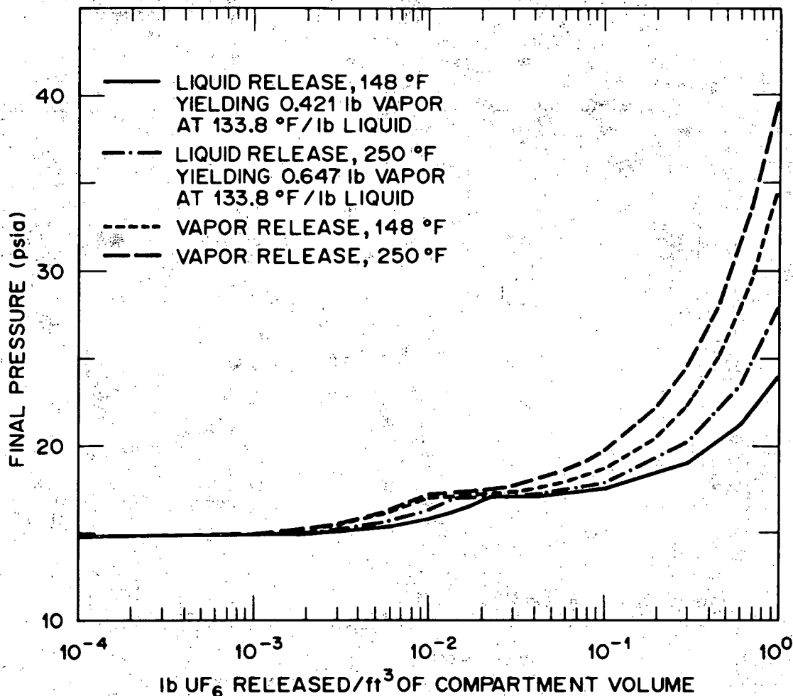
Fig. 7. Compartment pressure change due to an instantaneous UF 6 release assuming perfect mixing of released UF 6 in a closed compartment containing air at atmospheric pressure and 80°F with a relative humidity of 60%. UF 6 temperatures were selected based on ANSI N14.1 concerning cylinder fill limits (95% of cylinder volume at 250°F) and the triple point of UF 6 (147.2°F).
