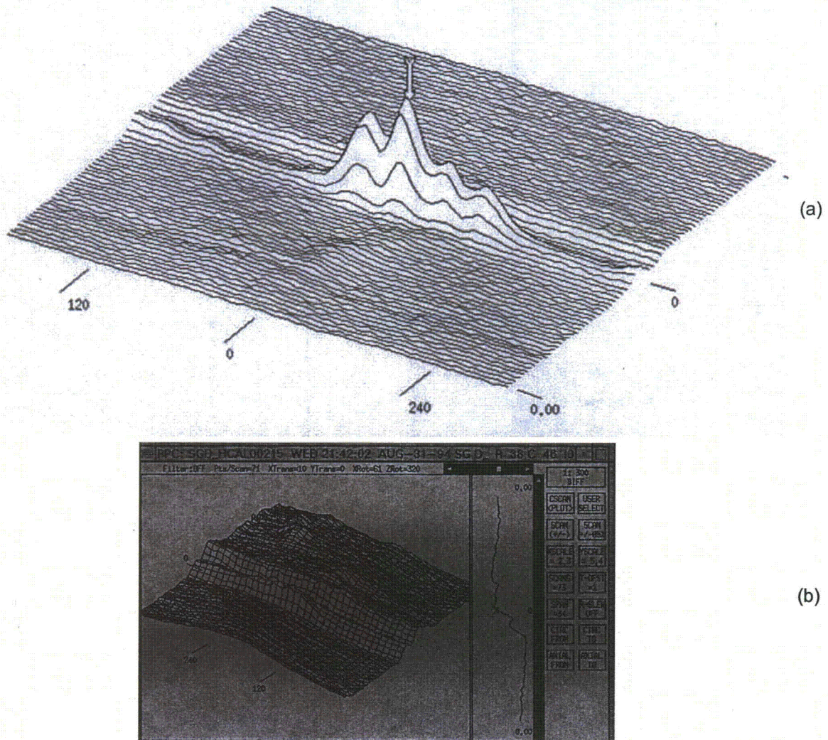
Figure 3.15 Comparison of (a) +Point C-scan of 2004 with (b) pancake coil C-scan of 1994 when retired SG tube sheet #10 was scanned.
