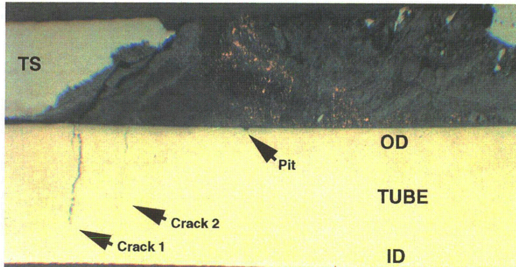
Figure 3.29 Cross-sectional optical metallograph of SG R39 C44 (ANL No. 7) specimen showing Alloy 600 tube, tube sheet, and various phases in deposit. There are multiple phases in the deposit, including metallic copper.
