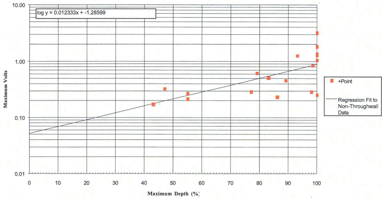
Figure 5.1 Maximum voltage vs. depth from +Point measurements in hard-roll expansions. Reproduced from Figure G-14b contained in Appendix G of EPRI Report TR-107 197-P2 [1]. Used by permission of EPRI.
