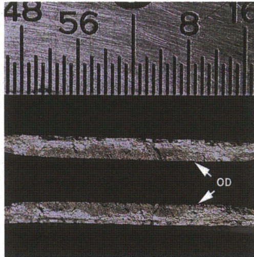
Figure 3.24 Comparison of fractography profile (red smooth curve) and NDE (blue dotted curve) for axial ODSCC in 19-mm (3/4-in.) diameter tube specimen 14-55-5. Multiple small cracks merged into one large axial crack.
