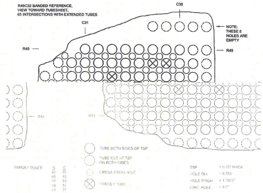
Figure 3.18 Tube support plate section TSP1 removed from steam generator B (SGB).
