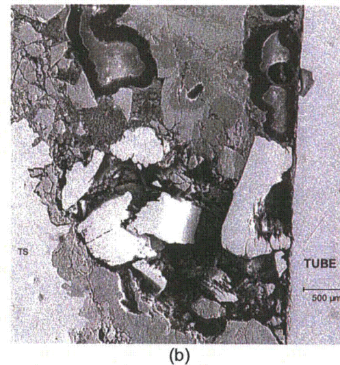
Figure 3.32 (a) Optical metallograph of cross section parallel to tube axis near maximum EC signals of R39 C45 (ANL-8). (b) Micrograph of bottom of the crevice between the top of the tubesheet and the tube.
