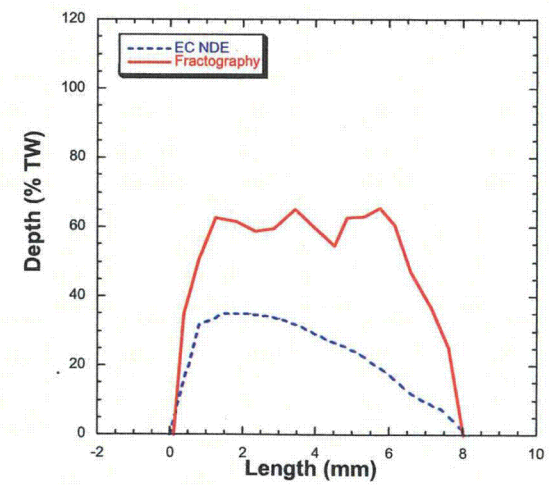
Figure 3.21 Comparison of fractography profile and NDE for axial ODSCC in 19-mm (3/4-in.) diameter tube specimen 5-51-2. The complex character is the cause of the undersizing (NDE, blue dotted curve; fractography, red smooth curve) of the eddy current profiles.
