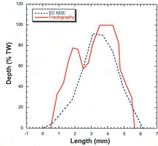
Figure 3.22 Comparison of fractography profile and NDE for axial ODSCC in 19-mm (3/4-in.) diameter tube specimen 7-24-3. The fractography shows that two cracks have merged together. The NDE (blue dotted curve) and fractography (red smooth curve) are in good agreement.
