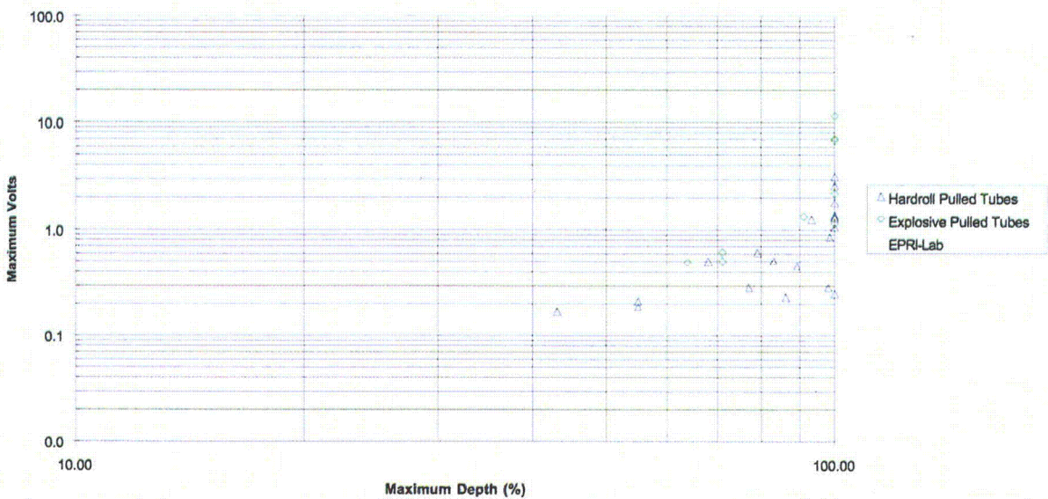
Figure 5.2 Maximum voltage vs. depth for OD indications in hard-roll pulled tubes and explosive pulled tubes. Reproduced from Figure G-15a contained in Appendix G of EPRI Report TR-107 197-P2 [1]. Used by permission of EPRI.
