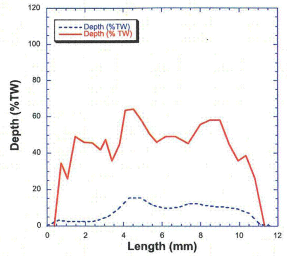
Figure 3.24 Comparison of fractography profile (red smooth curve) and NDE (blue dotted curve) for axial ODSCC in 19-mm (3/4-in.) diameter tube specimen 14-55-5. Multiple small cracks merged into one large axial crack.
