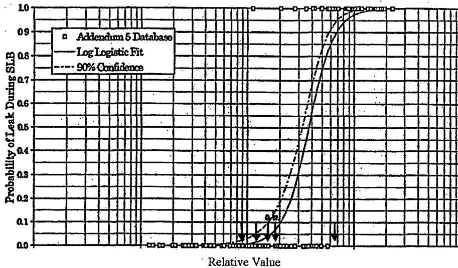
Figure 6.12 Relative bobbin coil amplitudes (before pulling) for the retired SG 19-mm (3/4-in.) diameter tubes with TSP SCC that were pressure tested at room temperature at Argonne are shown as arrows. The Argonne tube data can be compared with other 19-mm (3/4-in.) diameter field tubes that were pressure tested (Ref. 4). Tubes that did not leak at 17.6 MPa (2560 psi) are plotted as a probability of leakage of 0.0; those that did leak are plotted as a probability of leakage of 1.0. None of the retired steam generator tubes tested at Argonne leaked at pressures less than 17.7 MPa (2560 psi). Tubes a and b leaked at much higher pressures.
