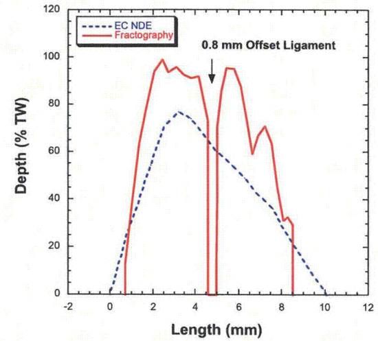
Figure 3.20 Comparison of fractography profile and NDE for axial ODSCC in 19-mm (3/4-in.) diameter tube specimen 4-43-2 (SGD). Area with the darker contrast represents the crack face. The complex character and ligament are the cause of the slight undersizing (NDE, blue dotted curve; fractography, red smooth curve) of the eddy current profiles. The arrow in graph indicates a 0.8-mm offset.
