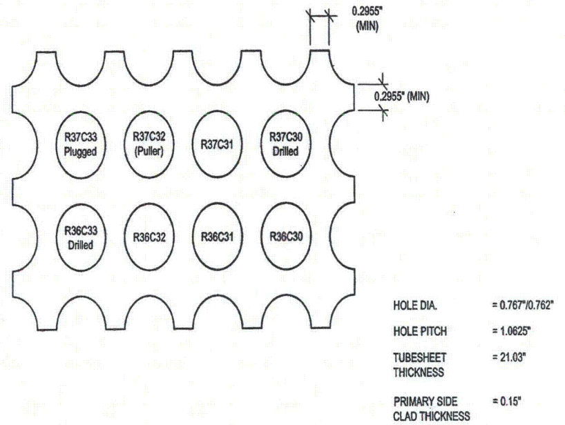
Figure 3.17 Tube sheet section TS2 removed from SGD (4x2 array of 19-mm (3/4-in.) diameter tubes).
