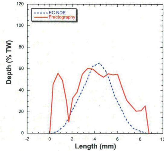
Figure 3.23 Comparison of fractography profile (red smooth curve) and NDE (blue dotted curve) for axial ODSCC in 19-mm (3/4-in.) diameter tube specimen 14-55-3.
