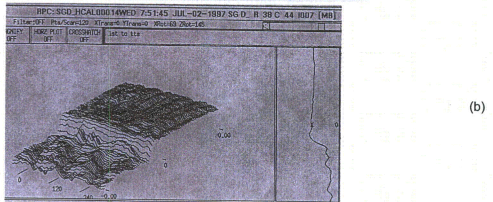
Figure 3.14 +Point signal of retired SG tube sheet #12 in (a) 2004 and (b) 1997. The 2004 image of CODSCC in the RTZ was generated using +Point probe at 300 kHz. The three-letter code for the flaw before the TS section was removed in 1997 was MCI. This tube was never plugged. The +Point at 300 kHz was 0.34 V in 2004 (poor signal-to-noise ratio) and 0.24 V in 1997.
