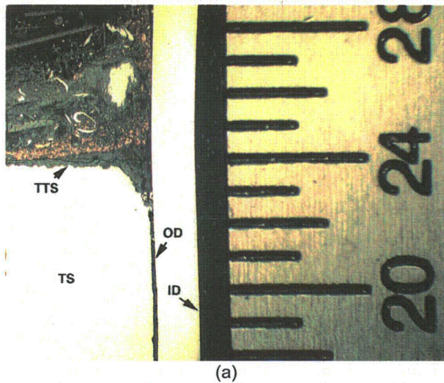
Figure 3.32 (a) Optical metallograph of cross section parallel to tube axis near maximum EC signals of R39 C45 (ANL-8). (b) Micrograph of bottom of the crevice between the top of the tubesheet and the tube.
