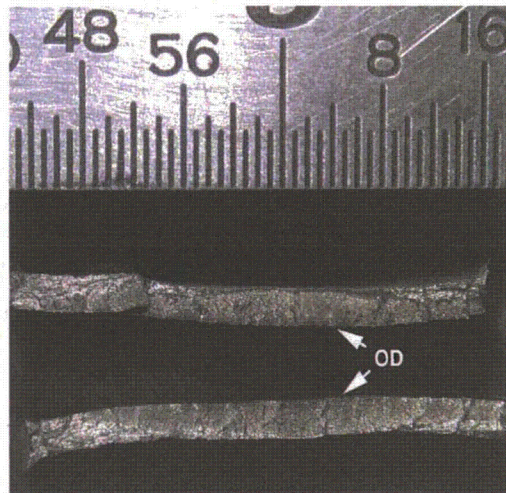
Figure 3.25 Comparison of fractography profile (red smooth curve) and NDE (blue dotted curve) for axial ODSCC in 19-mm (3/4-in.) diameter tube specimen 39-57-2.
