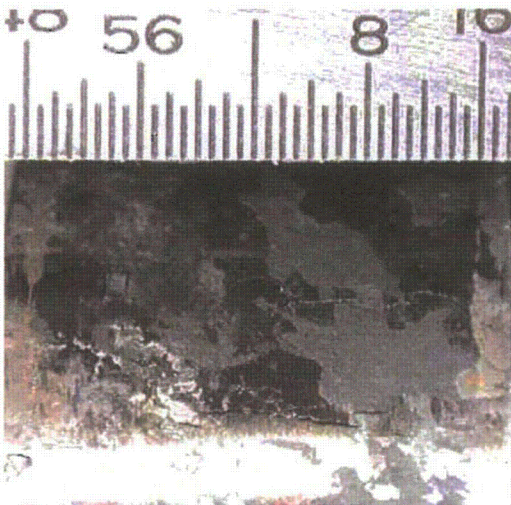
Figure 3.23 Comparison of fractography profile (red smooth curve) and NDE (blue dotted curve) for axial ODSCC in 19-mm (3/4-in.) diameter tube specimen 14-55-3.
