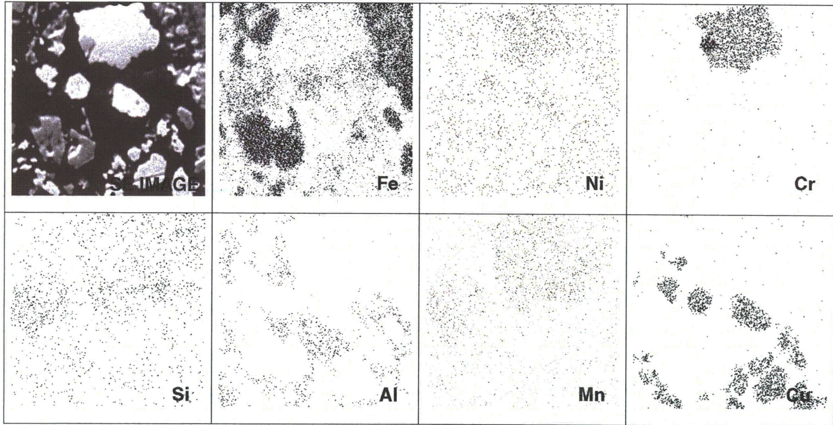
Figure 3.37 SEM image and EDS showing elemental distribution of Fe, Ni, Cr, Al, Si, Mg, Mn, and Cu at a local area in the deposit of the specimen R39 C45 TS801
