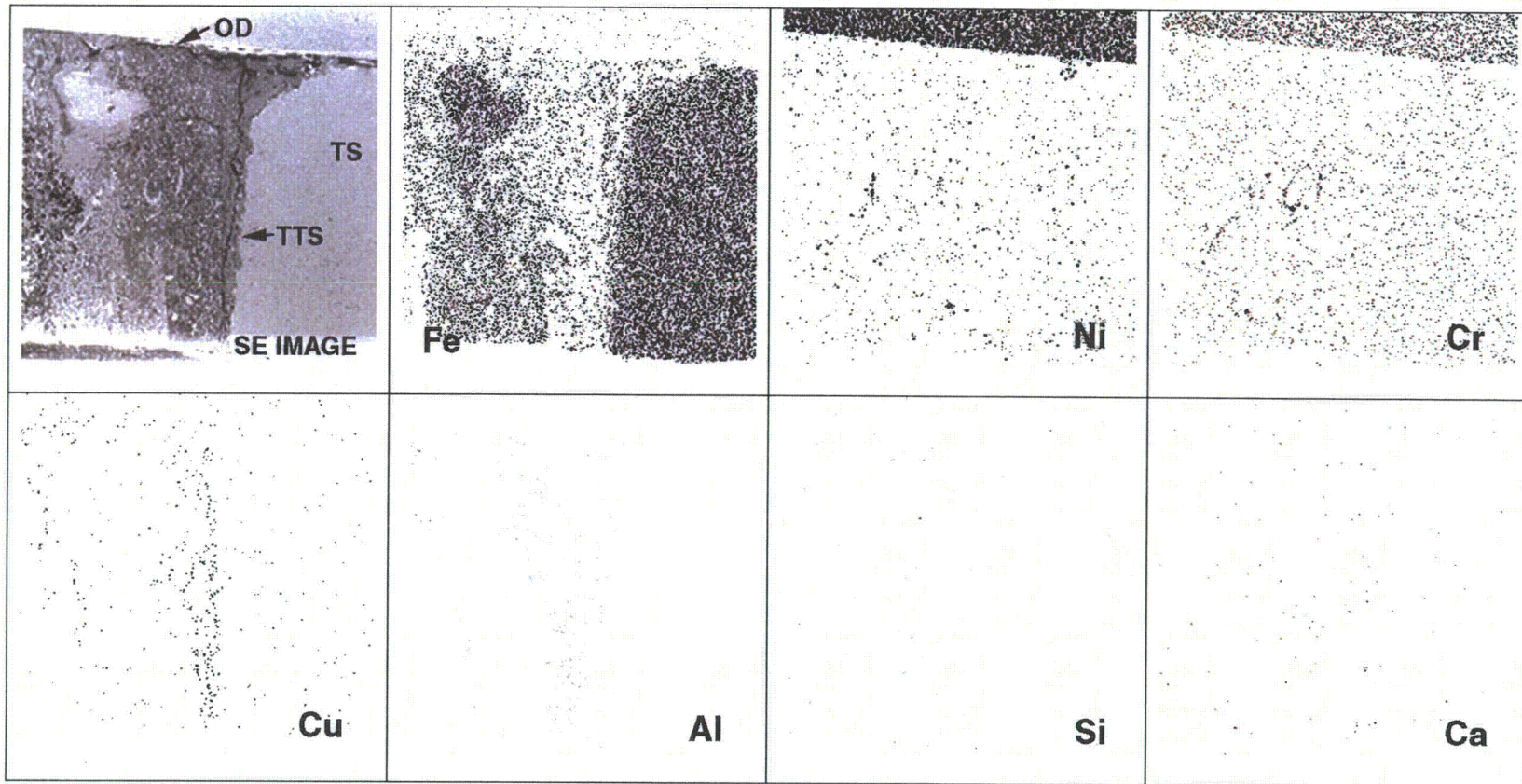
Figure 3.36 SEM image and EDS analysis showing distribution of Fe, Ni, Cr, Al, Si, Ca, Mn, and Cu in the SG tube, TS, and deposits of the specimen R39 C45 TS801 (ANL-8).
