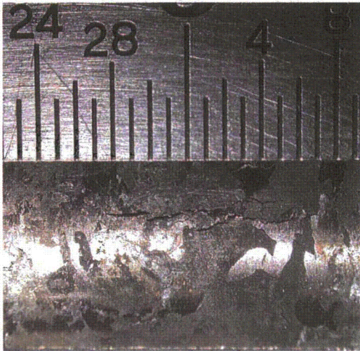
Figure 3.24 Comparison of fractography profile (red smooth curve) and NDE (blue dotted curve) for axial ODSCC in 19-mm (3/4-in.) diameter tube specimen 14-55-5. Multiple small cracks merged into one large axial crack.
