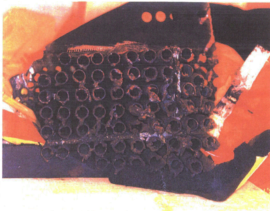
Figure 3.18 Tube support plate section TSP1 removed from steam generator B (SGB).
