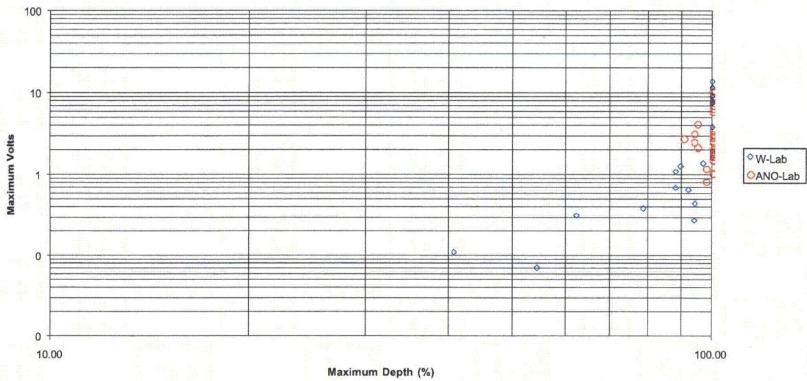
Figure 5.3 Maximum voltage vs. depth for OD indications in W-Lab and ANO-Lab tubes. Reproduced from Figure G-15b contained in Appendix G of EPRI Report TR-107 197-P2 [1]. Used by permission of EPRI.
