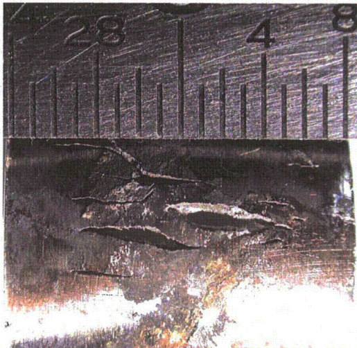
Figure 3.20 Comparison of fractography profile and NDE for axial ODSCC in 19-mm (3/4-in.) diameter tube specimen 4-43-2 (SGD). Area with the darker contrast represents the crack face. The complex character and ligament are the cause of the slight undersizing (NDE, blue dotted curve; fractography, red smooth curve) of the eddy current profiles. The arrow in graph indicates a 0.8-mm offset.
