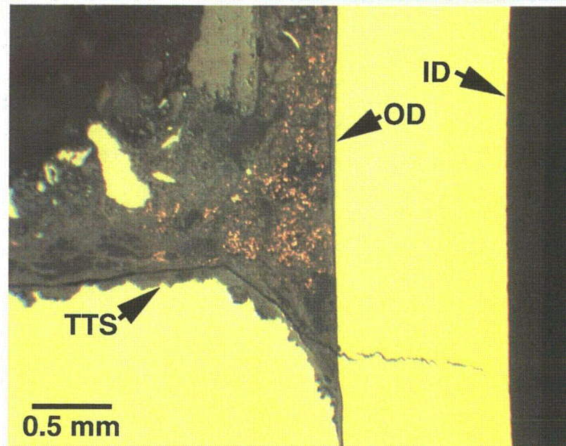
Figure 3.30 Cross-sectional optical metallograph of SG R39 C43 (ANL No. 6) specimen showing ODSCC in Alloy 600 tube. Copper is clearly visible in the deposit.
