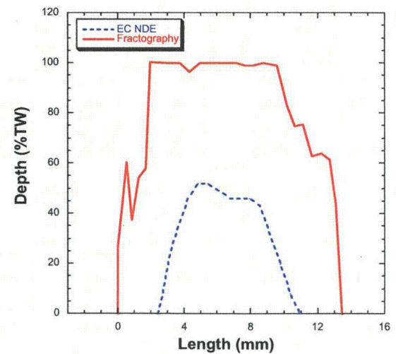
Figure 3.25 Comparison of fractography profile (red smooth curve) and NDE (blue dotted curve) for axial ODSCC in 19-mm (3/4-in.) diameter tube specimen 39-57-2.
