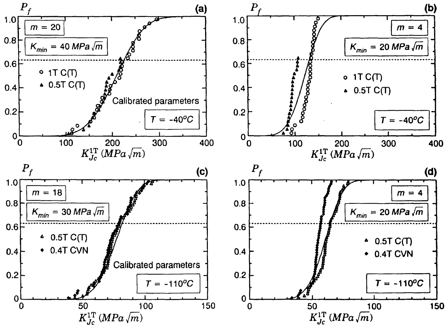
Figure 8. Correction of Euro-material datasets to 1T SSY condition at T = -40^\circ\text{C} and T = -110^\circ\text{C} . Using calibrated values of (m, K_{min}) in (a,c); using other values of (m, K_{min}) to illustrate errors of using non-calibrated values.
