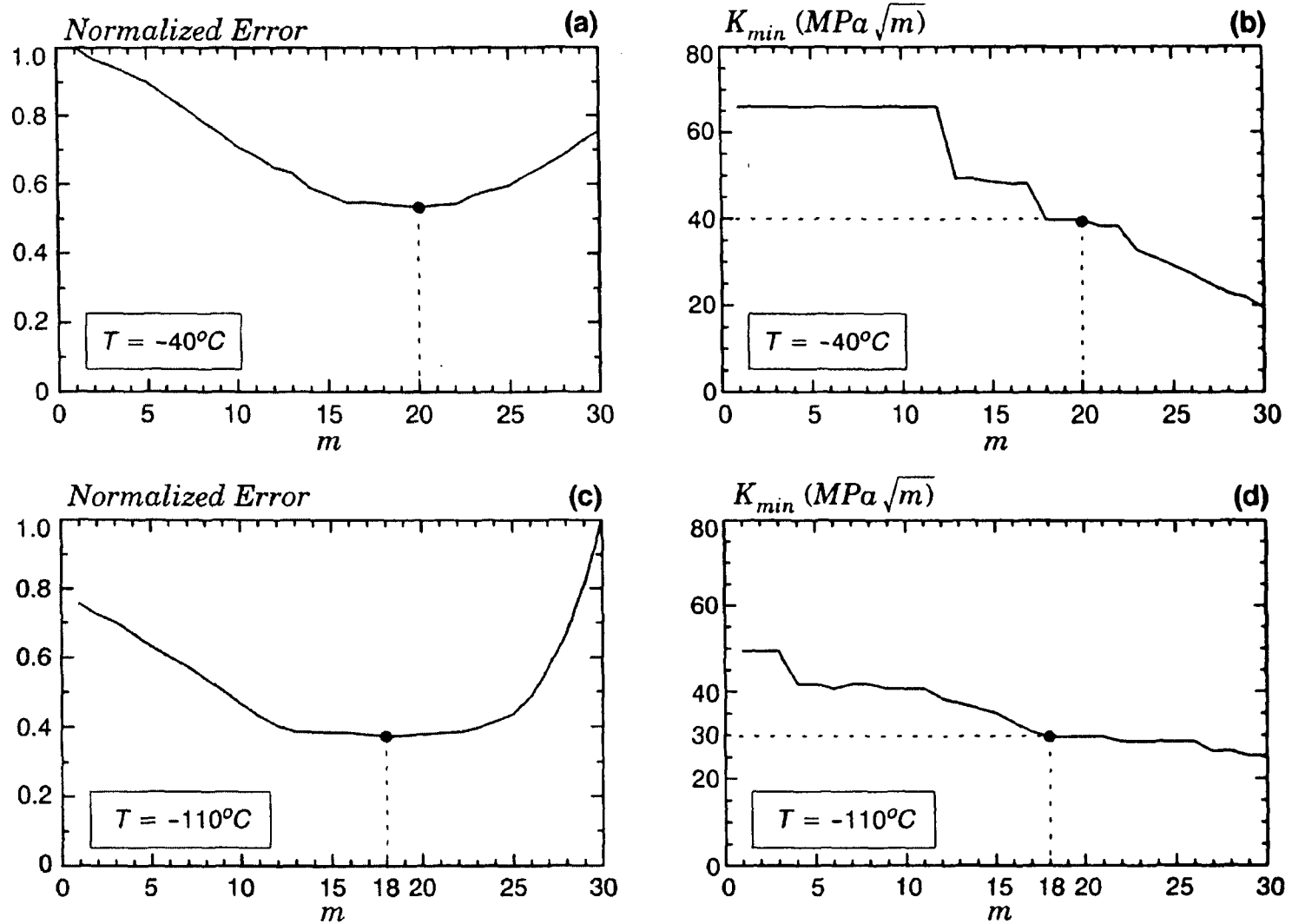
Figure 7. Calibration of Weibull stress parameters for the Euro-material at T = -40^\circ\text{C} and T = -110^\circ\text{C} . Normalized values of error function over range of m -values (a,c); corresponding K_{min} values that lead to minimum error values for each m -value.
