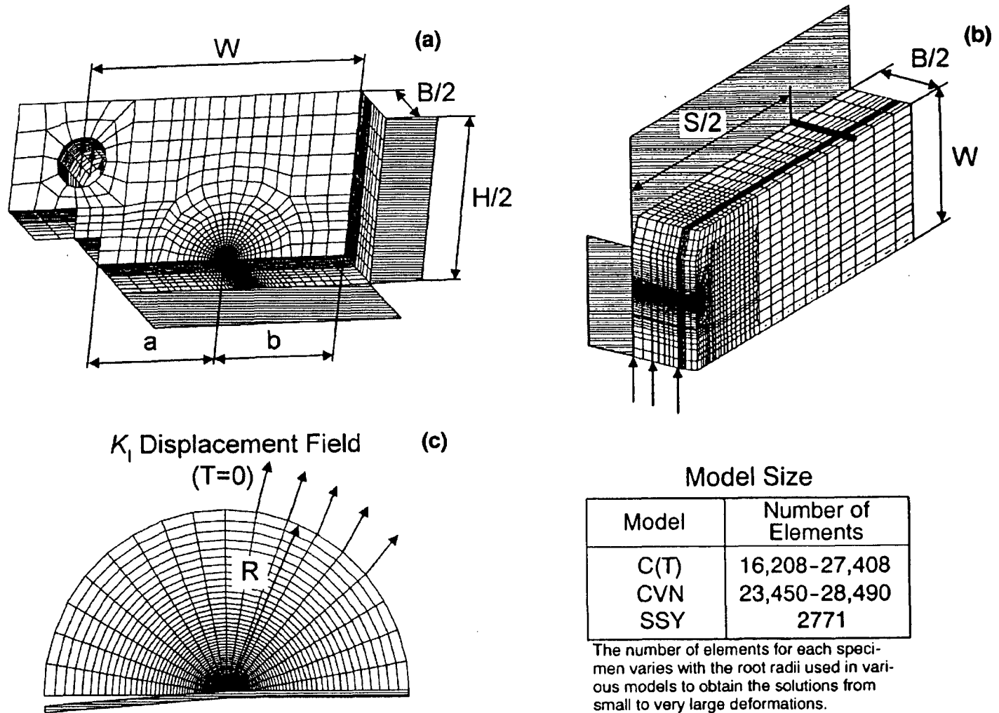
Figure 3. One-quarter symmetric finite element models for (a) C(T) specimen with a/W = 0.56 , (b) pre-cracked, 0.4T Charpy V-Notch specimen with a/W = 0.56 , and (c) small-scale yielding (SSY). All models have finite root radius along crack front.
