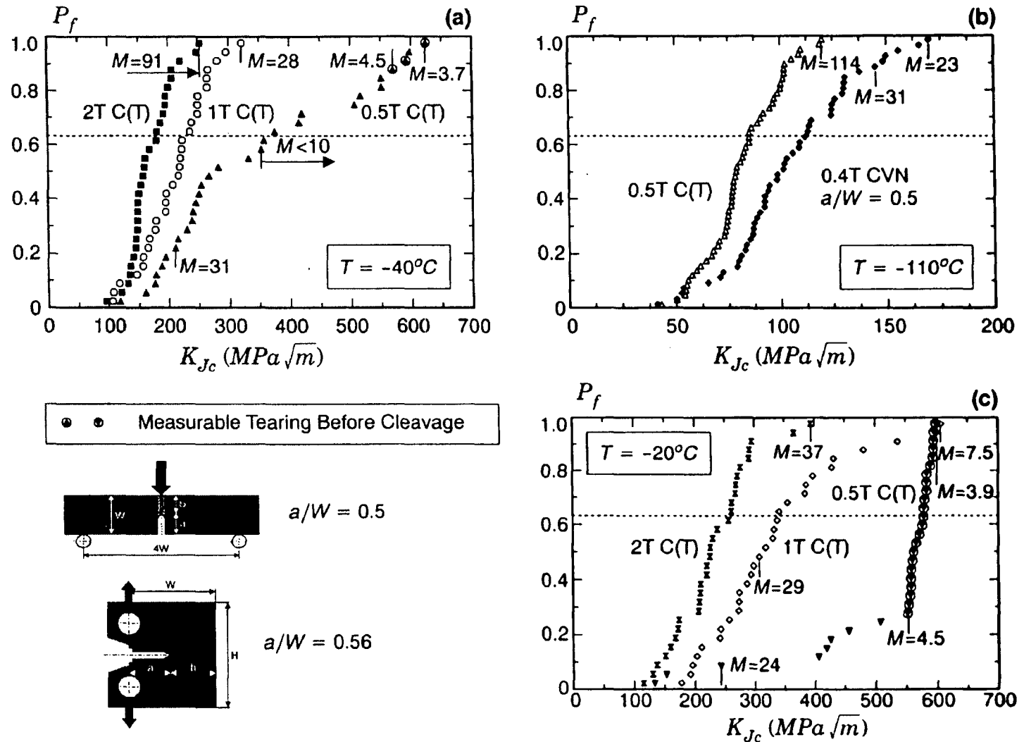
Figure 4. Cumulative (rank) fracture probabilities of raw experimental datasets for the Euro material at (a) T = -40^\circ\text{C} , (b) T = -110^\circ\text{C} , (c) T = -20^\circ\text{C} . These data drive the calibration process for the Weibull stress parameters. The reference temperature T_0 = -90^\circ\text{C} from C(T) specimens.
