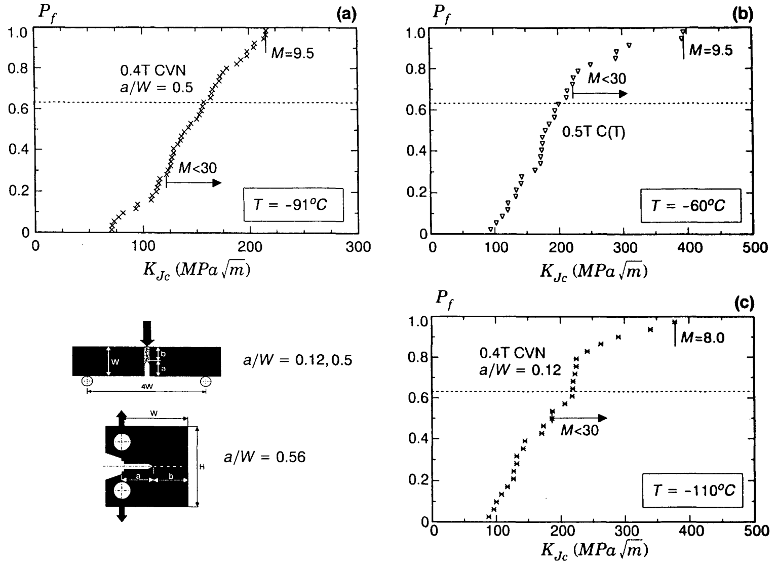
Figure 5. Cumulative (rank) fracture probabilities of raw experimental datasets for the Euro material at (a) T = -91^\circ\text{C} , (b) T = -60^\circ\text{C} , (c) T = -110^\circ\text{C} . These data drive checking of the Weibull stress parameters calibrated using other datasets. The reference temperature T_0 = -90^\circ\text{C} from C(T) specimens.
