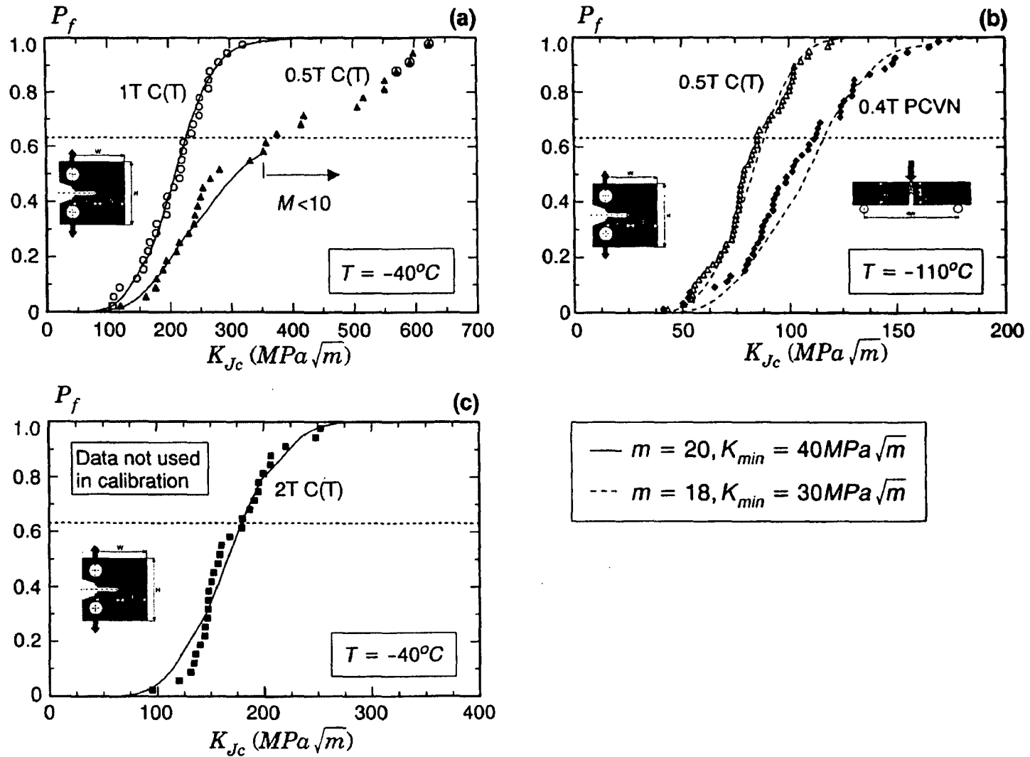
Figure 9. Predicted fracture probabilities of Euro-material using calibrated Weibull stress parameters: (a) T = -40^\circ\text{C} data used in calibration, (b) T = -110^\circ\text{C} data used in calibration and (c) T = -40^\circ\text{C} data not used in calibration.
