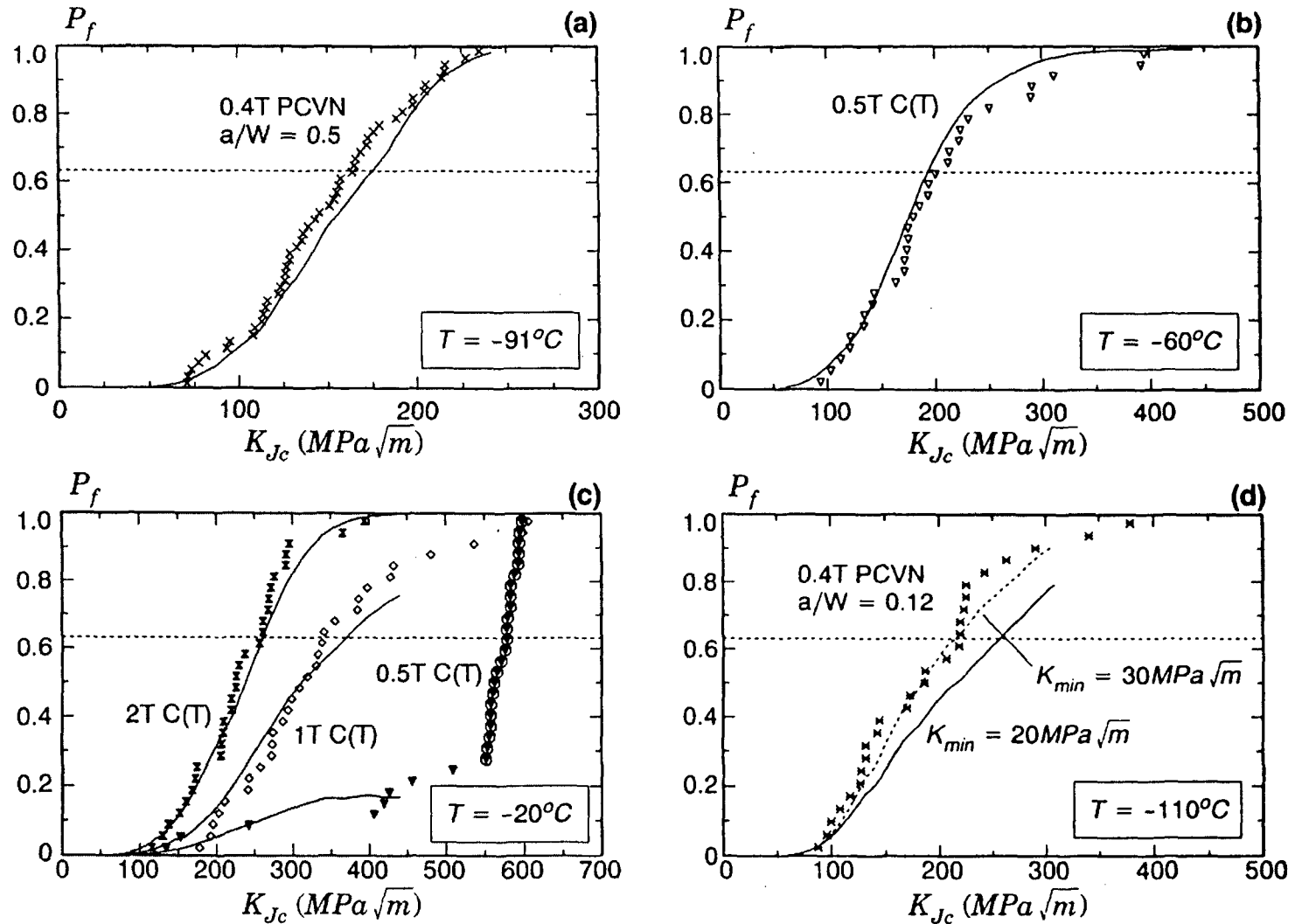
Figure 10. Predicted fracture probabilities for Euro-material specimens not used in any calibrations. Weibull modulus fixed at m = 20 , K_{min} = 20 \text{MPa} \cdot \text{m}^{1/2} with temperature dependent \sigma_u based on the Master Curve. (a) T = -91^\circ\text{C} , (b) T = -60^\circ\text{C} , (c) T = -20^\circ\text{C} and (d) T = -110^\circ\text{C} .
