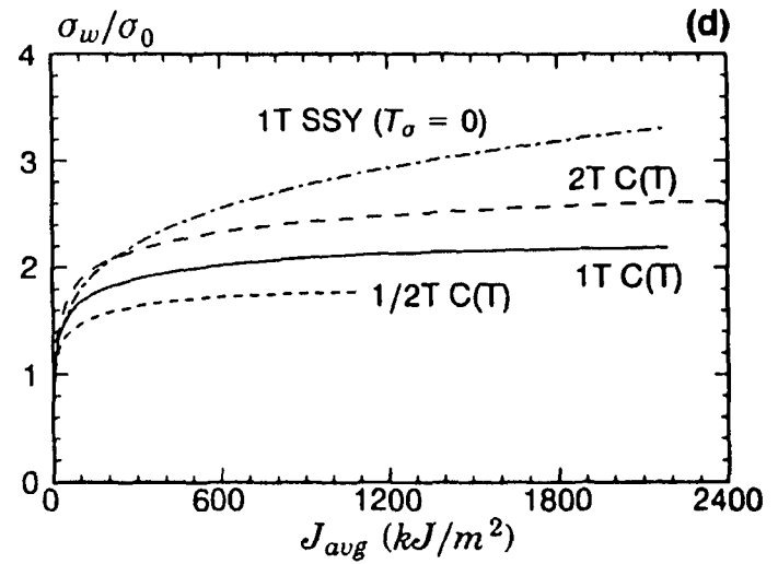
Figure 1. Weibull stress values and constraint correction g -functions computed using stress-strain properties for the Euro material at -40^\circ\text{C} . Weibull stress modulus taken as m = 10 for these illustrative results.
