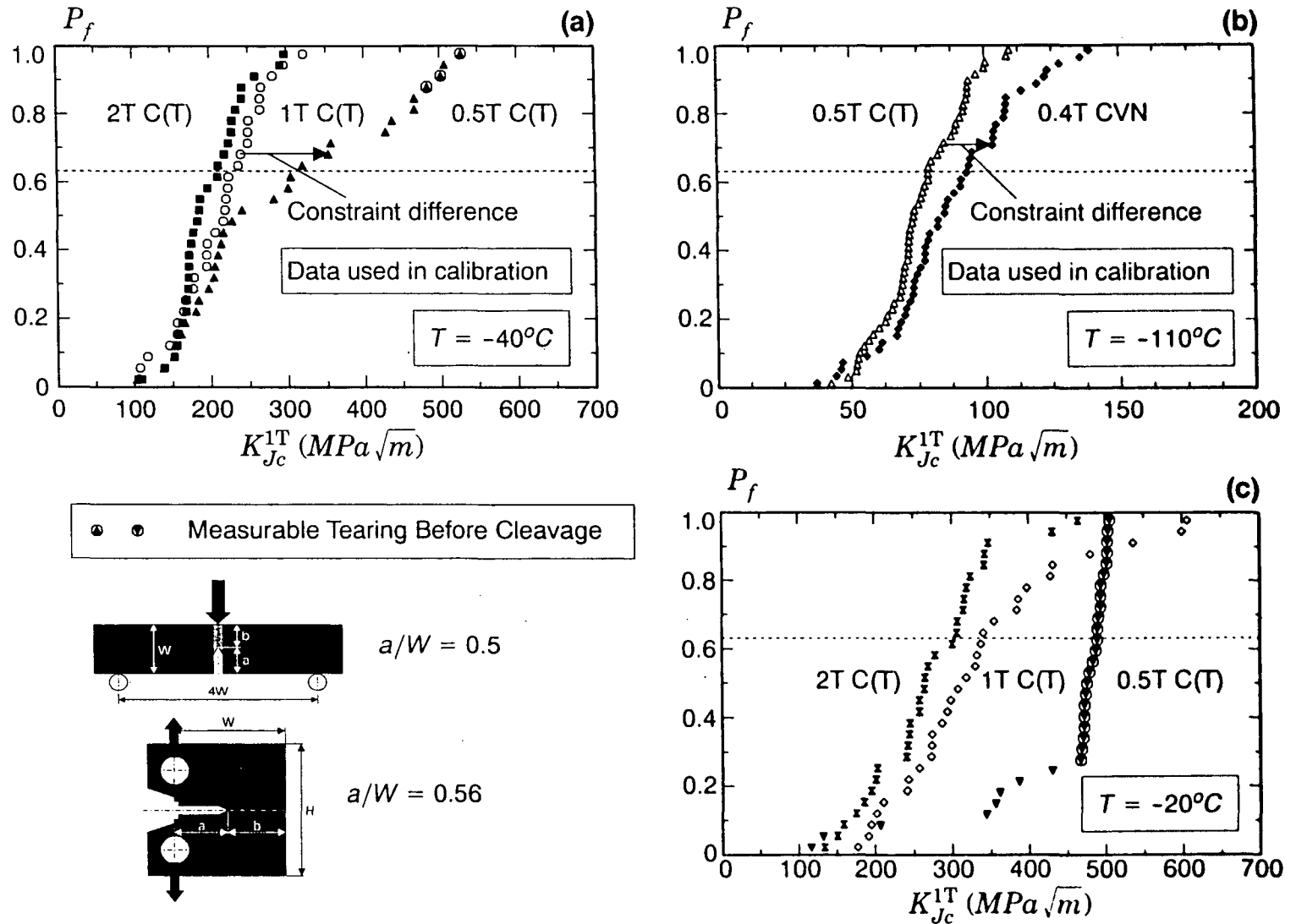
Figure 6. Cumulative (rank) fracture probabilities of experimental datasets for the Euro material crack-front length adjusted to 1T using E1921 procedure at (a) T = -40^\circ\text{C} , (b) T = -110^\circ\text{C} , (c) T = -20^\circ\text{C} . The reference temperature T_0 = -90^\circ\text{C} from C(T) specimens.
