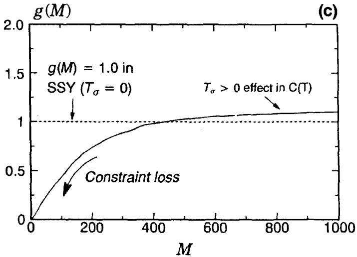
Figure 1. Weibull stress values and constraint correction g -functions computed using stress-strain properties for the Euro material at -40^\circ\text{C} . Weibull stress modulus taken as m = 10 for these illustrative results.
