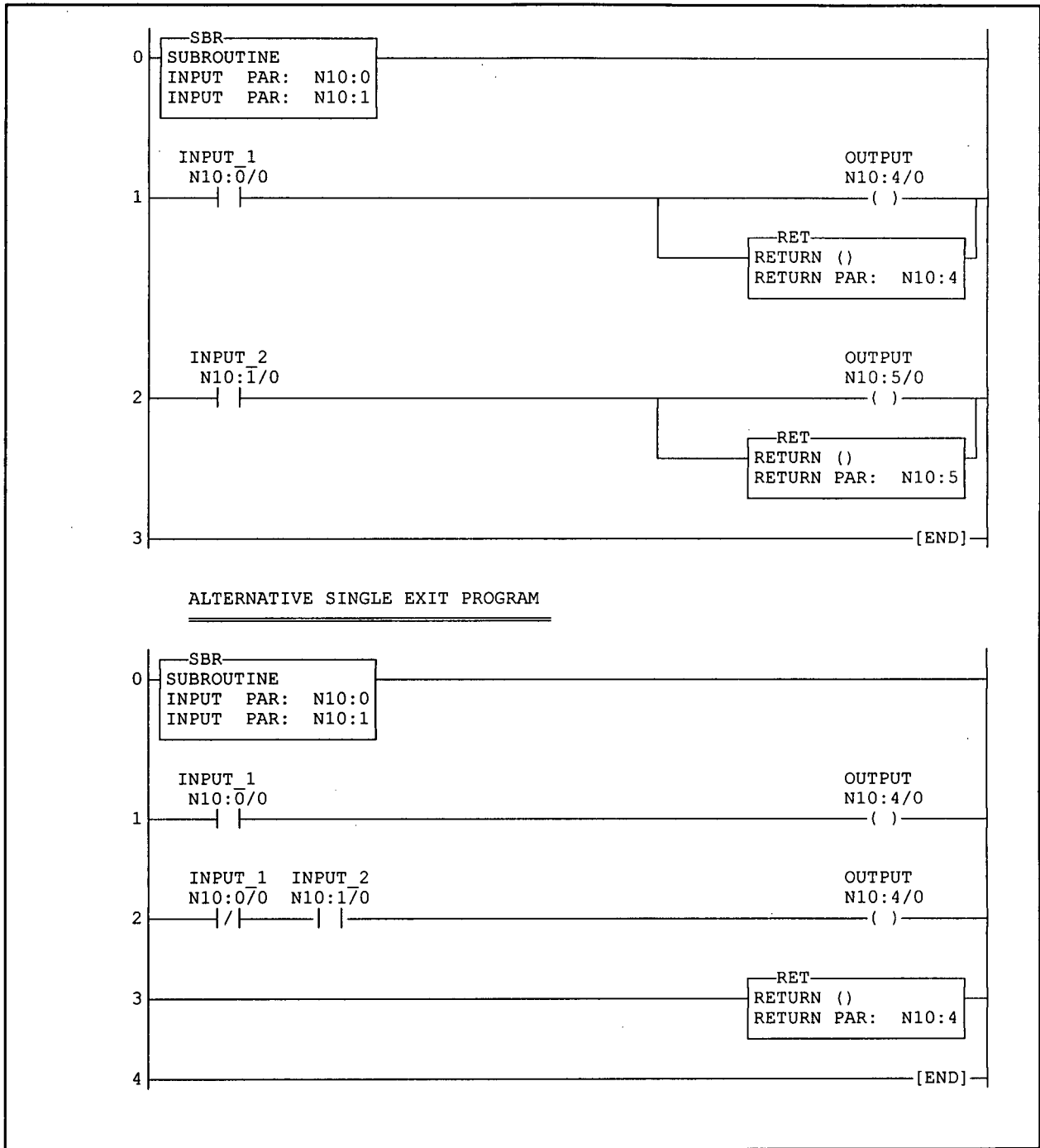
Figure 5-4 Ladder Logic multiple RETURN.
