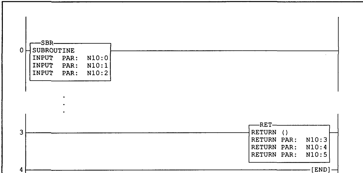
Figure A-6 Subroutine interface (parameter passing).
