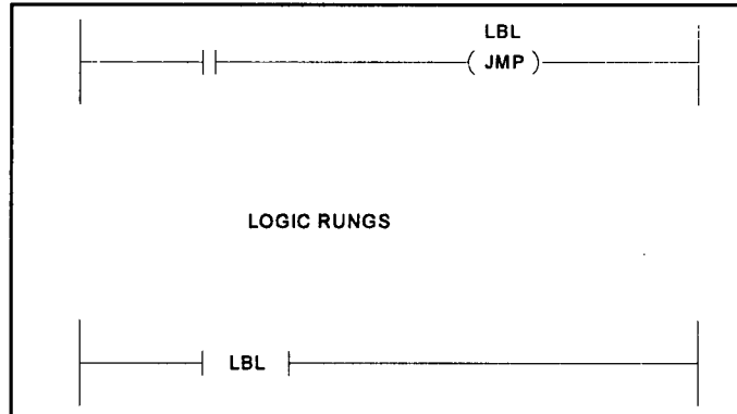
Figure 5-1 Use of goto .
