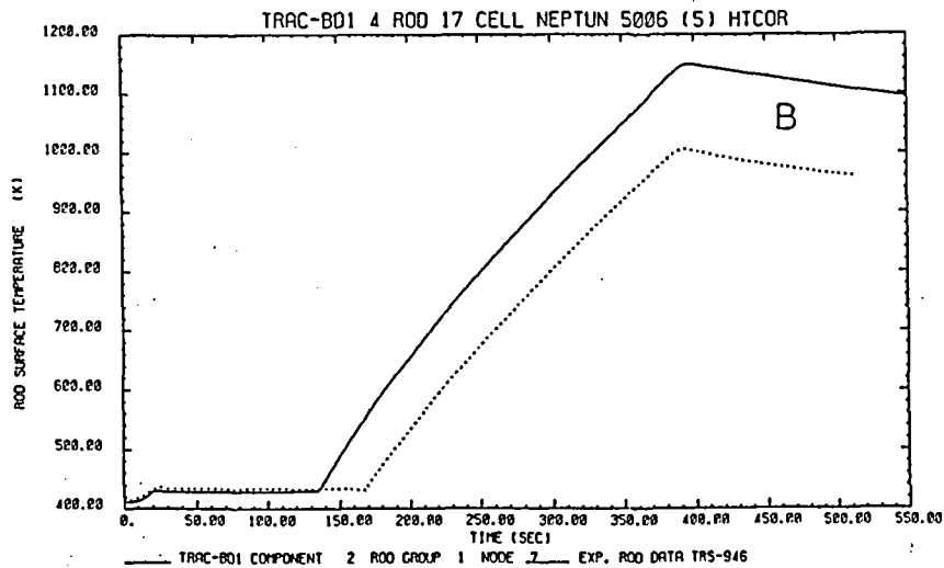
Fig. 19: Comparison of measured and calculated collapsed liquid level and peak axial power level rod surface temperature histories, using frozen version of TRAC-BD1 for NEPTUN boil-off experiment 5006.
