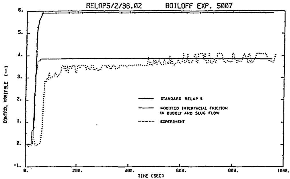
Figure 16: Water entrainment in NEPTUN boil-off experiment 5007, calculated by RELAP5/MOD2, with and without new correlation for the interfacial friction in bubbly and slug flow.
