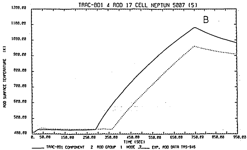
Fig. 20: Comparison of measured and calculated collapsed liquid level and peak axial power level rod surface temperature histories, using frozen version of TRAC-BD1 for NEPTUN boil-off experiment 5007.
