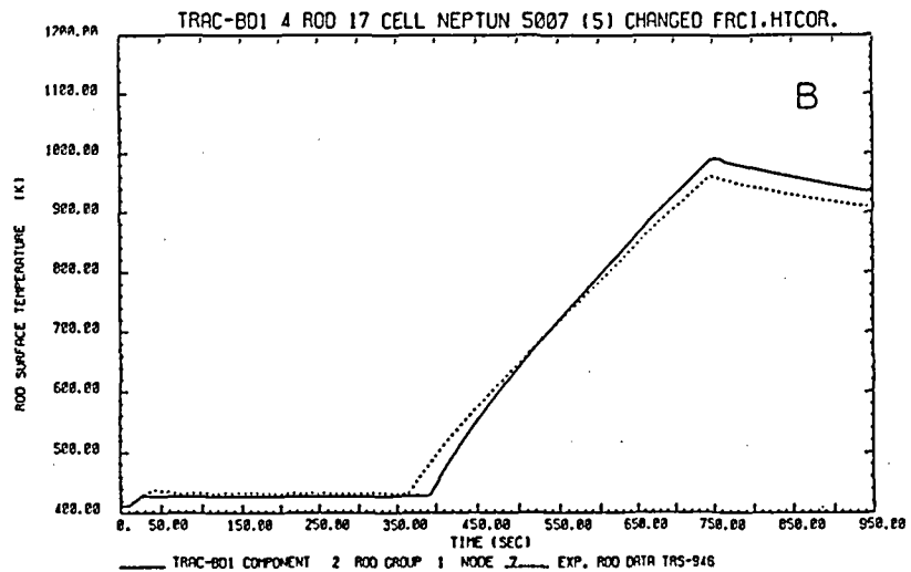
Fig. 25: Comparison of measured and calculated collapsed liquid level and peak axial power level rod surface temperature histories, using frozen version of TRAC-BD1 for NEPTUN boil-off experiment 5007.
