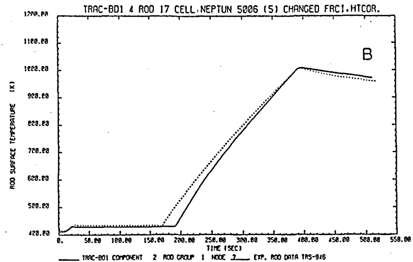
Fig. 24: Comparison of measured and calculated collapsed liquid level and peak axial power level rod surface temperature histories, using frozen version of TRAC-BD1 for NEPTUN boil-off experiment 5006.
