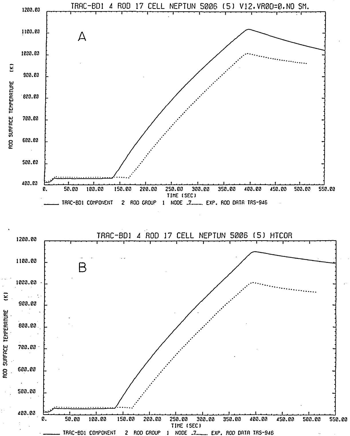
Fig. 28: Rod surface temperature histories at peak axial power level in NEPTUN boil-off experiment 5006 calculated by TRAC-BD1, (a) frozen version, (b) modified for steam cooling.
