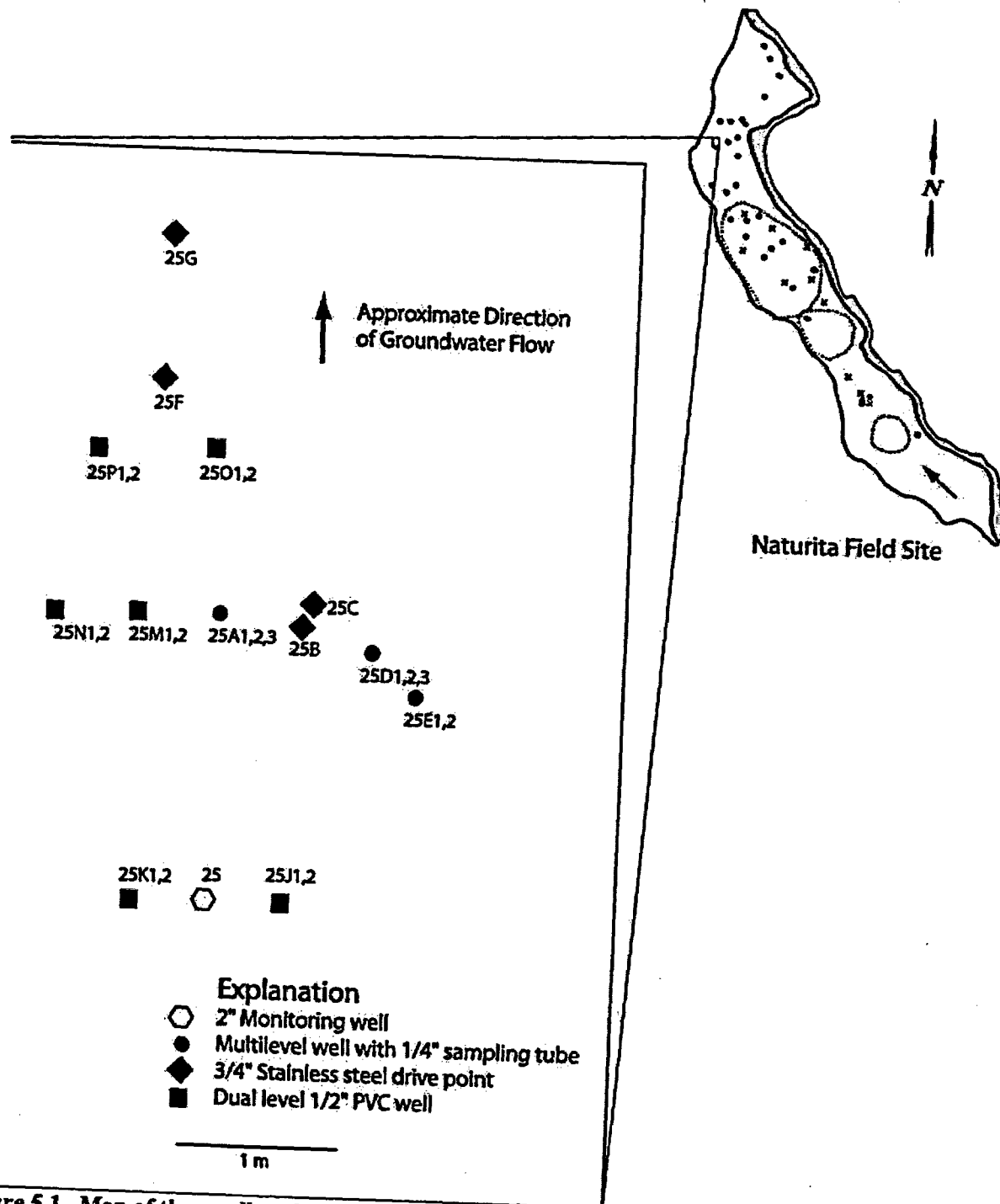
Figure 5.1. Map of the small-scale tracer test site developed near NAT25. The numbers after the well designations indicate the different sampling levels with 1 being the deepest screened interval.
