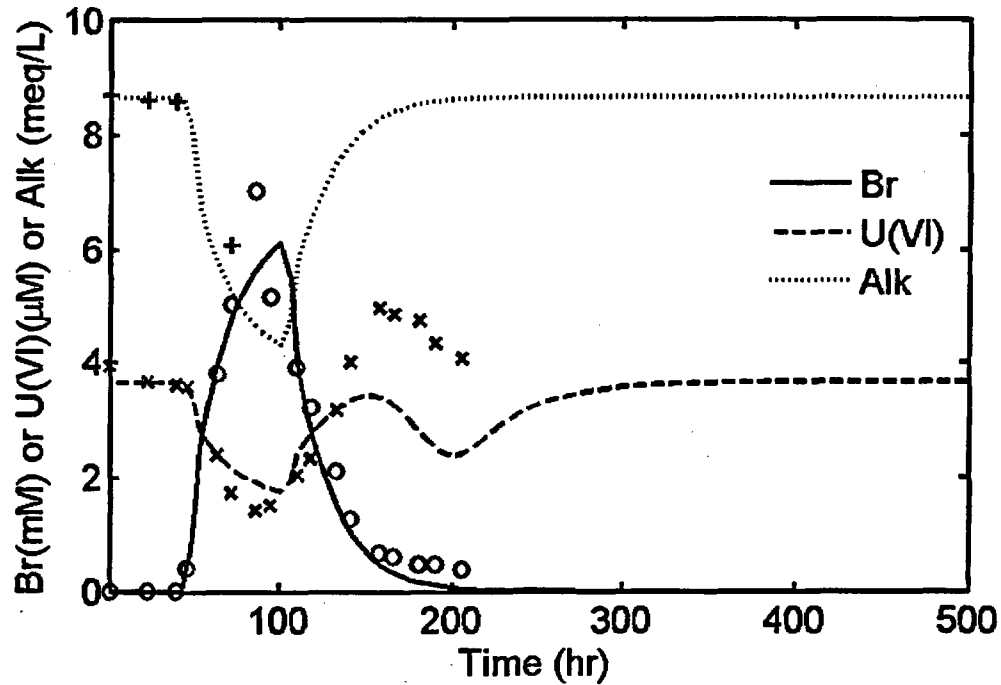
Figure 5.4. Observed and simulated bromide, U(VI) and alkalinity concentrations in migration test MT1 at observation well A1.
