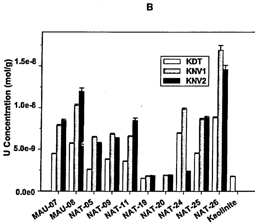
Figure 2.5. Comparison of U(VI) extracted from kaolinite deployed in different sample holder types: KDT (dialysis tubing) and KNV (nylon vial), with U(VI) extracted by carbonate solution (A) and nitric acid (B). Sample labeled 'Kaolinite' shows data for extractions without field deployment.
