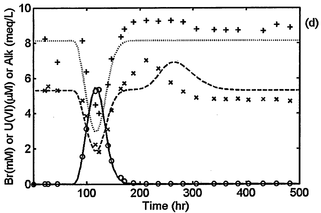
Figure 5.5 (cont). Observed and simulated bromide, U(VI) and alkalinity concentrations in migration test MT2 at observations wells (c) N2, and (d) O1.
