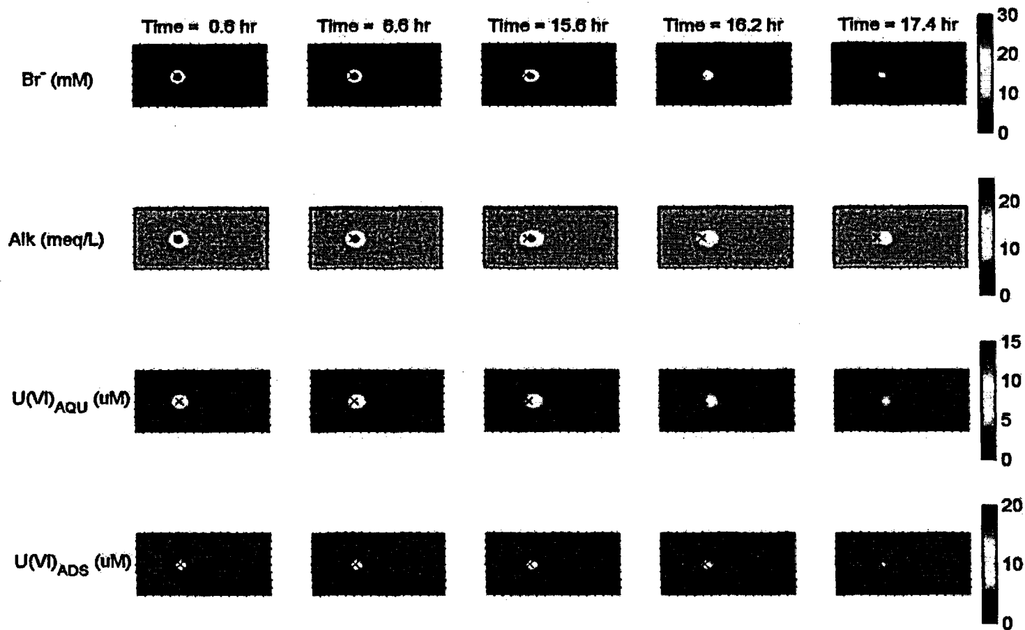
Figure 3.8. Temporal evolution of bromide, alkalinity, total dissolved U(VI), [shown as U(VI) AQU ], and total adsorbed U(VI) [shown as (U(VI) ADS )] for kinetically controlled simulations using Model 1.
