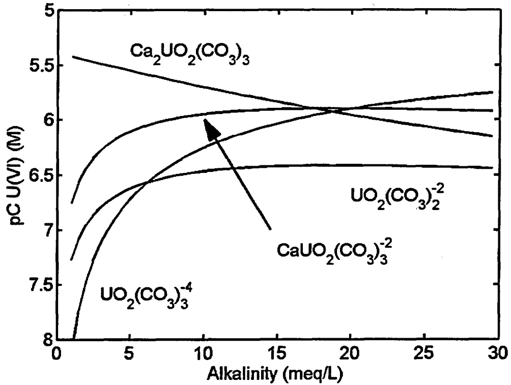
Figure 5.3. Speciation of 4 μM U(VI) in groundwater in equilibrium with calcite at pH 7.1 and with variable alkalinity.
