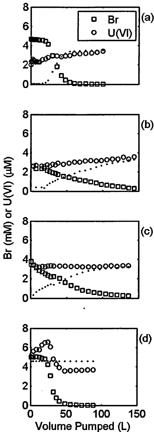
Figure 4.3. Concentrations of U(VI) and Br tracer in push-pull tracer tests conducted with uncontaminated groundwater for various drift periods and injected alkalinities: (a) PPT3, (b) PPT2, (c) PPT5, and (d) PPT9. The dashed line represents U(VI) concentrations expected from the mixing of injected and native groundwater, based on the concentrations of Br tracer.
