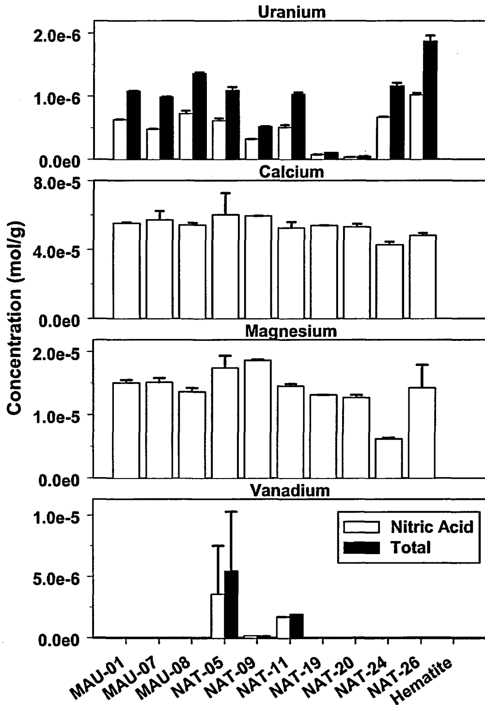
Figure 2.13. Comparison of various elements extracted from hematite by nitric acid alone versus total extracted (sum of carbonate solution and nitric acid extracts) after exposure to groundwater for 1 month. For U(VI) and V, data are corrected for the amount of each element present in entrained water when samples were collected. The data presented represent the average from two dialysis bags containing hematite that were deployed in each well. Data that were below the detection limit for V are not plotted. Sample labeled 'Hematite' shows data for extractions without field deployment.
