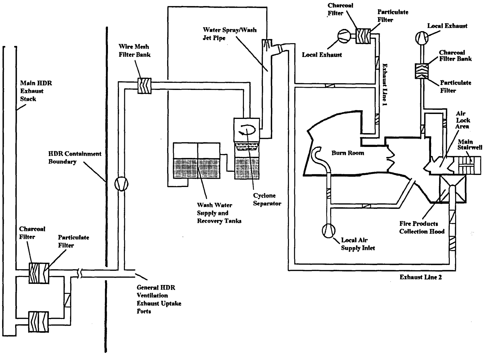
Figure 3.6: Configuration of the Ventilation System for Test Series E42.
