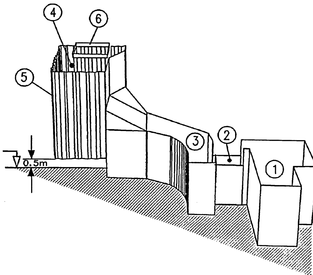
Figure 3.2: Three-Dimensional View of the T51 Fire Area and Adjoining Spaces
