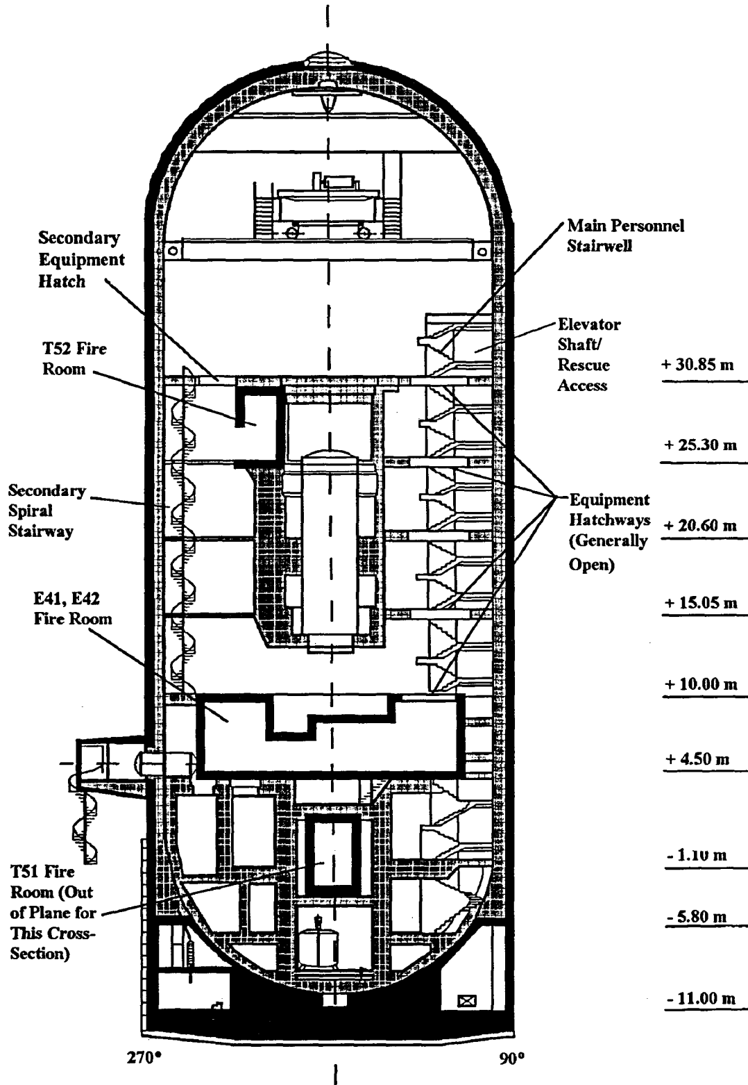
Figure 2.1: General Schematic View of the HDR Containment Structure.
