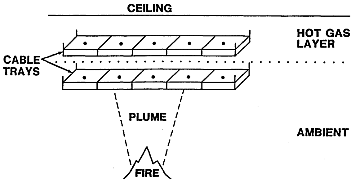
Figure 2: Zone Fire Model Example
