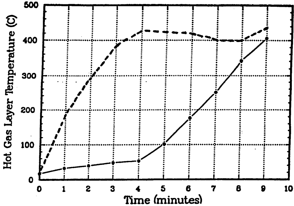
Figure 16: COMPBRN E42.2 Hot Gas Layer Temperatures (Solid = COMPBRN results, Dash = Measured by CT5298)
