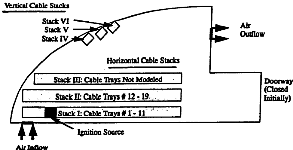
Figure 11 E42.2 Cable Tray Layout Diagram (Plan View)
