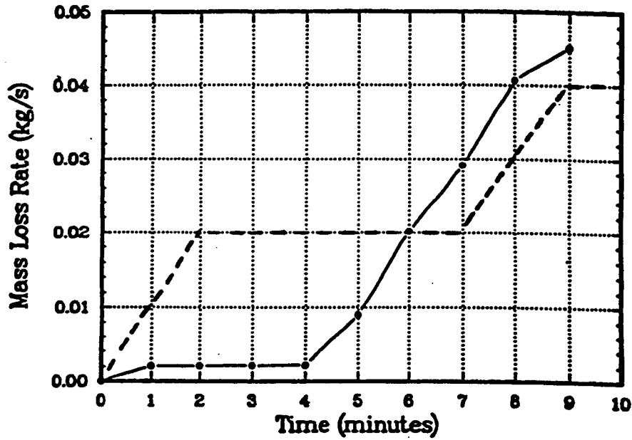
Figure 15: COMPBRN E42.2 Fuel Mass Loss Rate (Solid = COMPBRN results, Dash = Measured)
