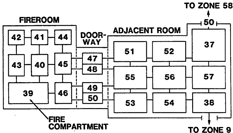
Figure 3: Control Volume Fire Model Example
