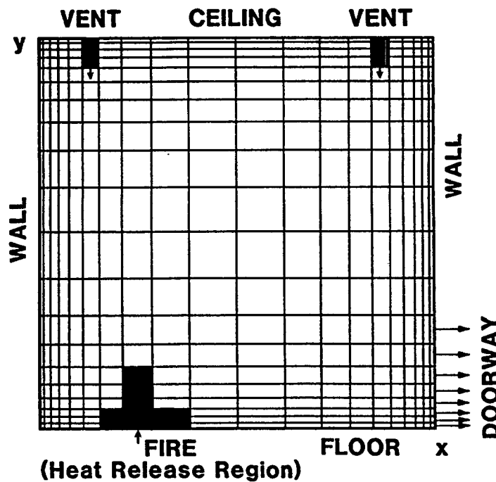
Figure 4: Fire Field Model Example
