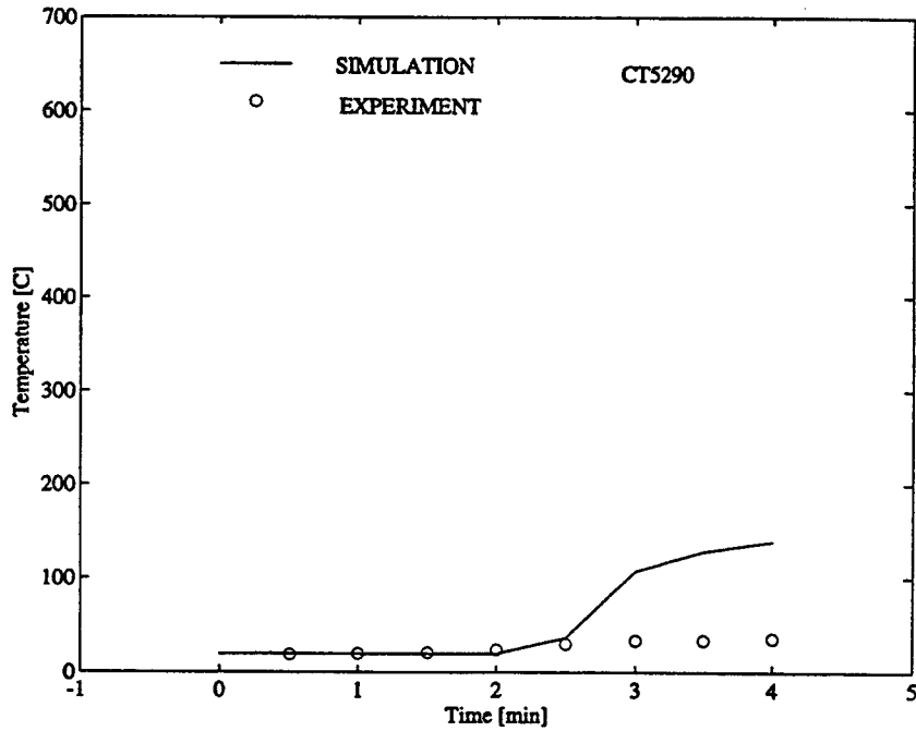
Figure 9: E41.7 CT5290 Temperature (Solid=NDFM, Circle=Data)
