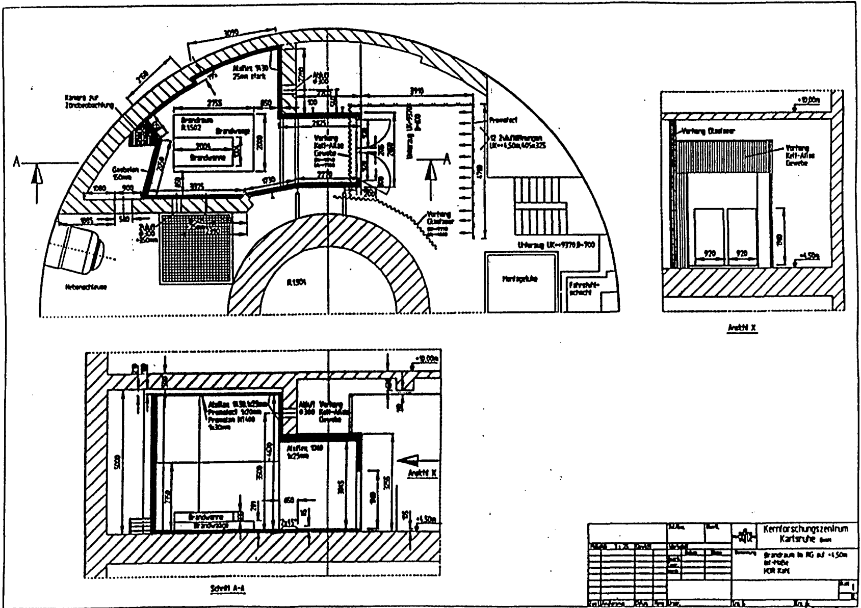
Figure B-1 HDR Fire Room Geometry
