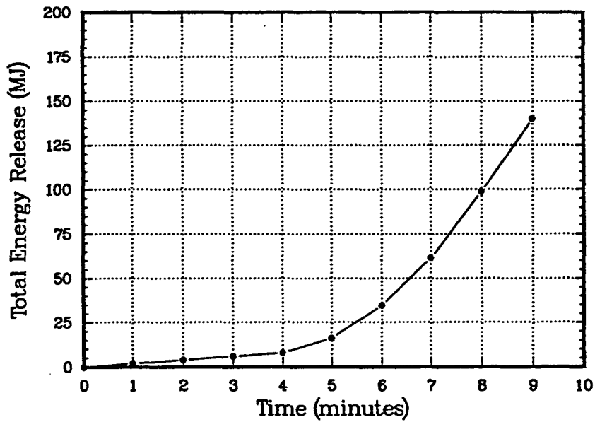
Figure 14: COMPBRN E42.2 Fire Total Energy Output
