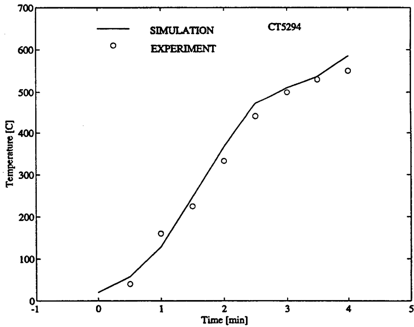
Figure 10: E41.7 CT5294 Temperature (Solid=NDFM, Circle=Data)
