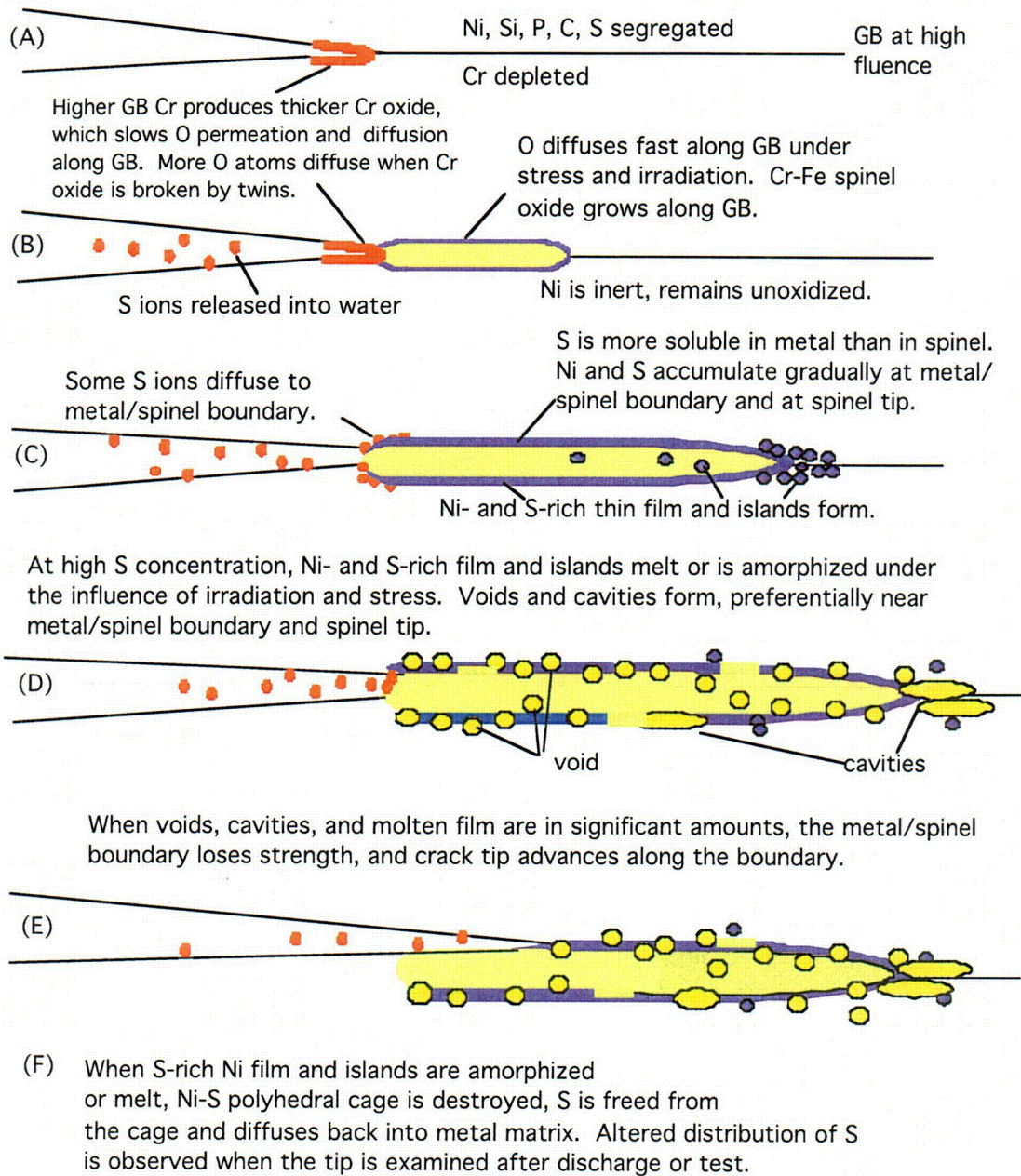
Figure 80. Schematic illustration of an IASCC model
