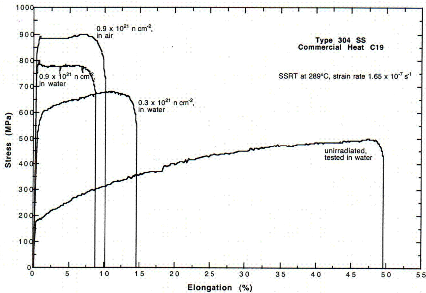
Figure 11. Effects of fluence and test environment on load elongation behavior of Type 304 SS commercial heat C19.
