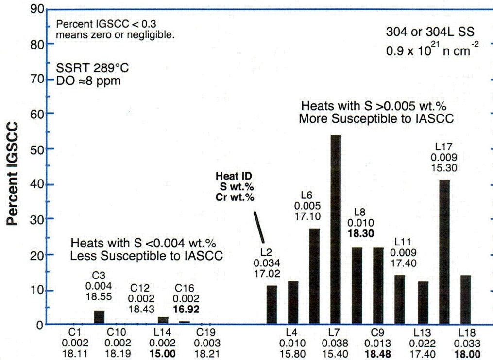
Figure 14. Effect of S on susceptibility to IGSC of Type 304 and 304L steels irradiated to \approx 0.9 \times 10^{21} \text{ n cm}^{-2} ( E > 1 \text{ MeV} ); one group of steels contains < 0.004 wt.% S and the other group contains > 0.005 wt.% S.
