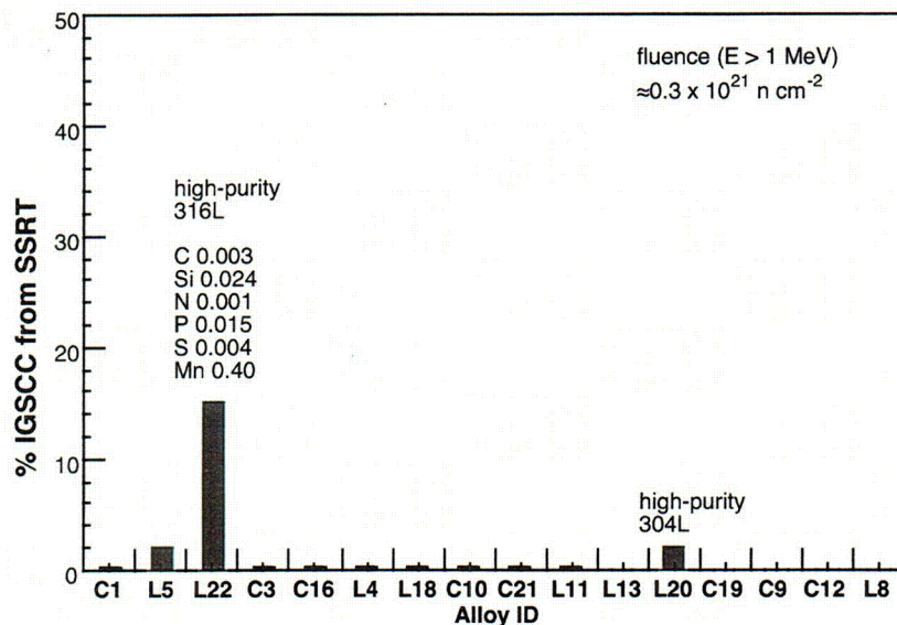
Figure 7. Percent IGSCC of model SS alloys irradiated in He in the Halden reactor to fluence of \approx 0.3 \times 10^{21} n\text{-cm}^{-2} ( E > 1 MeV) and tested at 289°C in BWR-like water.
