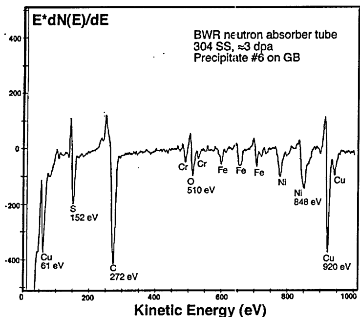
Figure 76. AES signal showing high concentrations of Cu, S, and C in CuS-type precipitate denoted with number "6" in Fig. 72.
