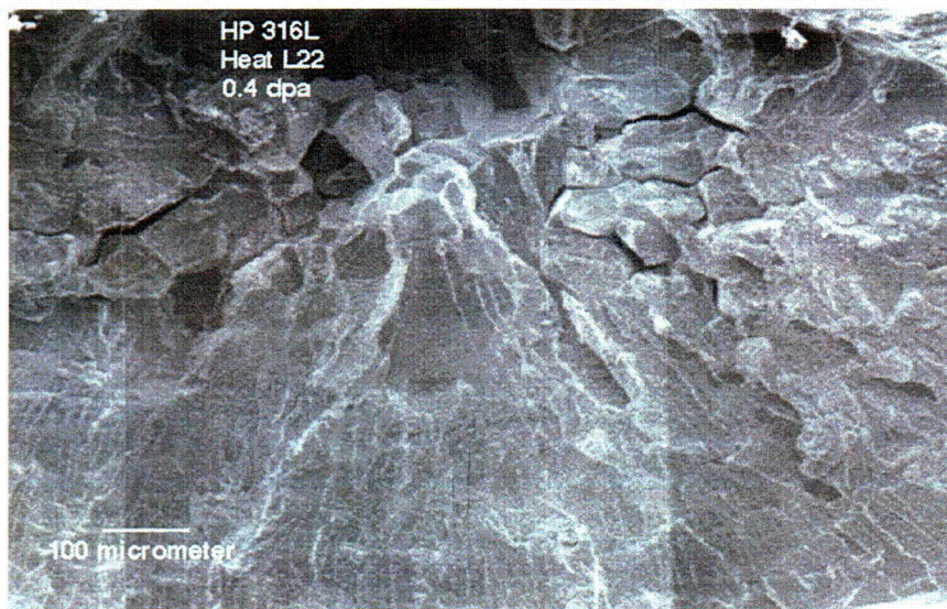
Figure 8. Limited intergranular fracture surface surrounded by transgranular surface in 316L-like SS Heat L22 irradiated to \approx 0.3 \times 10^{21} n\text{-cm}^{-2} ( E > 1 MeV, \approx 0.4 dpa) and tested at 289°C in BWR-like water.
