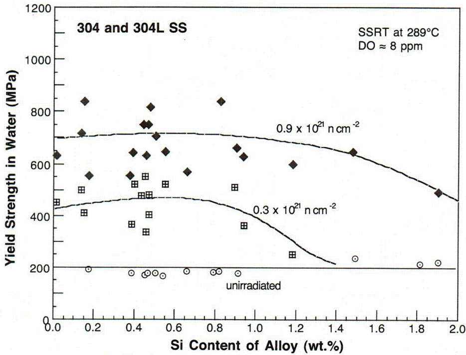
Figure 16. Effect of Si concentration on yield strength of Types 304 and 304L steel measured in 289°C water before and after irradiation.
