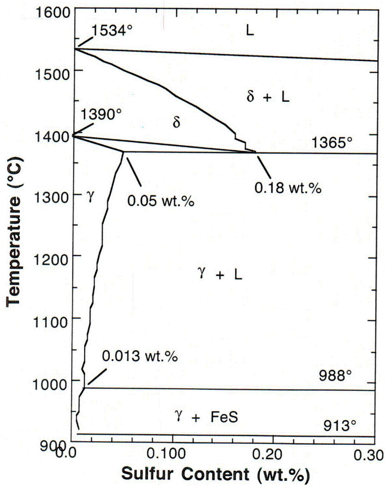
Figure 50. Fe-rich side of Fe-S phase diagram; from Hansen, Ref. 47.
