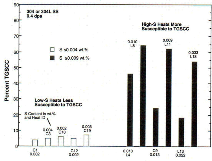
Figure 10. Effect of S content on the susceptibility to TGSCC of Type 304 or 304L heats, irradiated to fluence of \approx 0.3 \times 10^{21} \text{ n cm}^{-2} ( E > 1 \text{ MeV} ) ( \approx 0.4 \text{ dpa} ) and tested at 289°C in BWR-like water.
