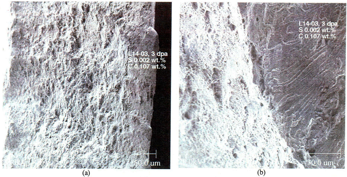
Figure 54. Fracture surface morphology of IASCC-resistant Laboratory Heat L14 of Type 304 SS (3 dpa), showing predominant ductile morphology (a) and limited transgranular morphology (b); intergranular morphology is negligible.
