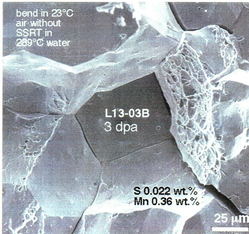
Figure 79. Fracture surface morphology of high-S, low-Mn Type 304 SS Specimen L13-03B (S, 0.022 wt.%; Mn, 0.36 wt.%; ≈3 dpa in helium at 289°C) produced during bending in 23°C air without previous exposure to water or H charging.
