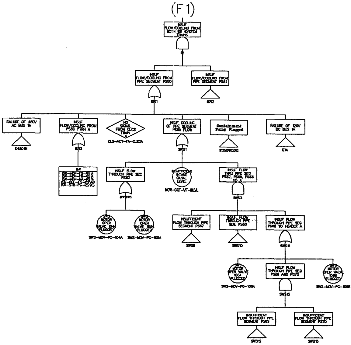
Figure 3.4 Example fault tree for inside spray recirculation
