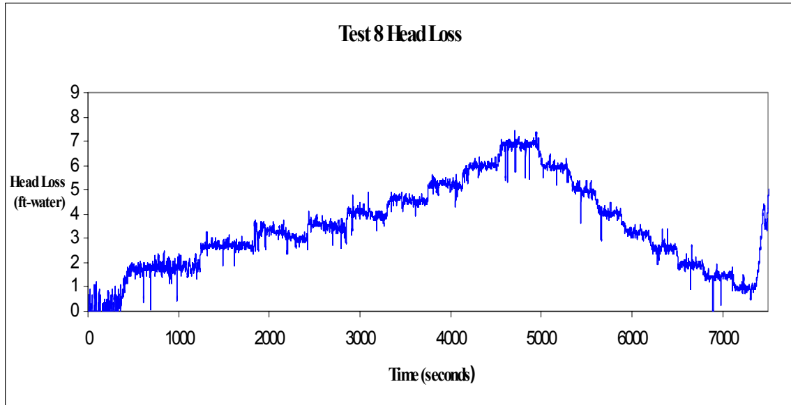
Fig. A-13. Time-dependent head-loss measurements.
