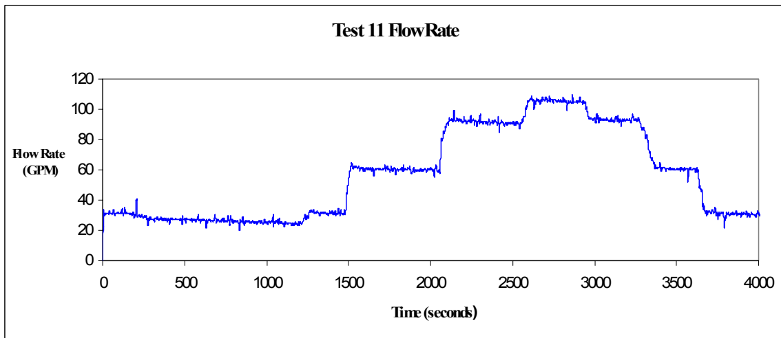
Fig. A-18. Time-dependent flow-rate measurements.
