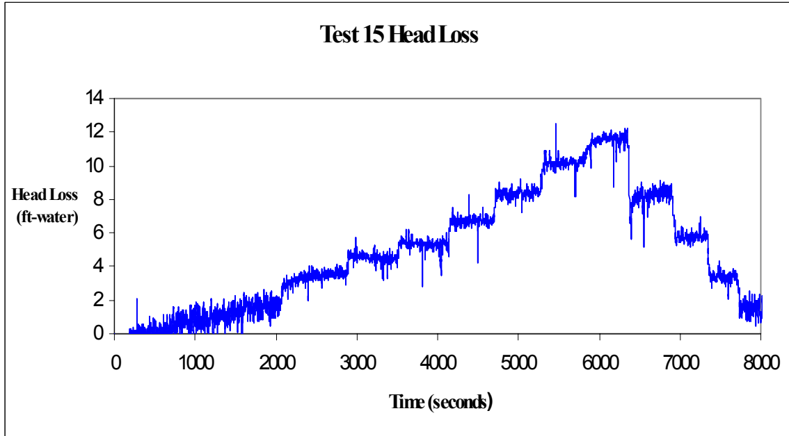
Fig. A-25. Time-dependent head-loss measurements.
