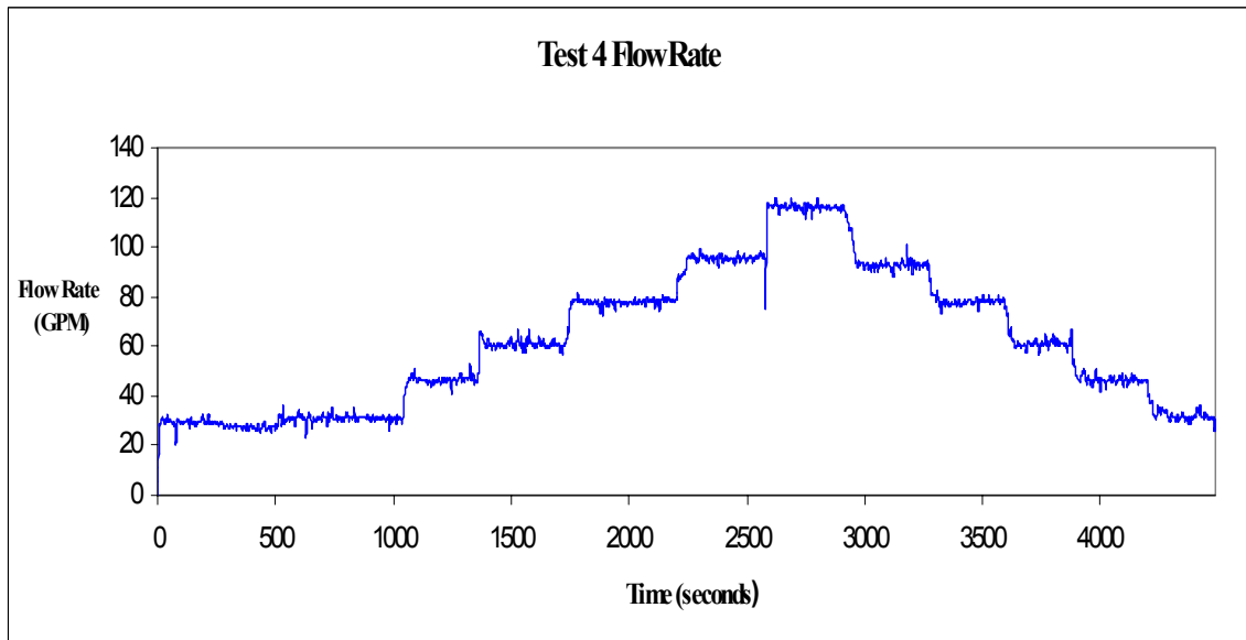
Fig. A-6. Time-dependent flow-rate measurements.
