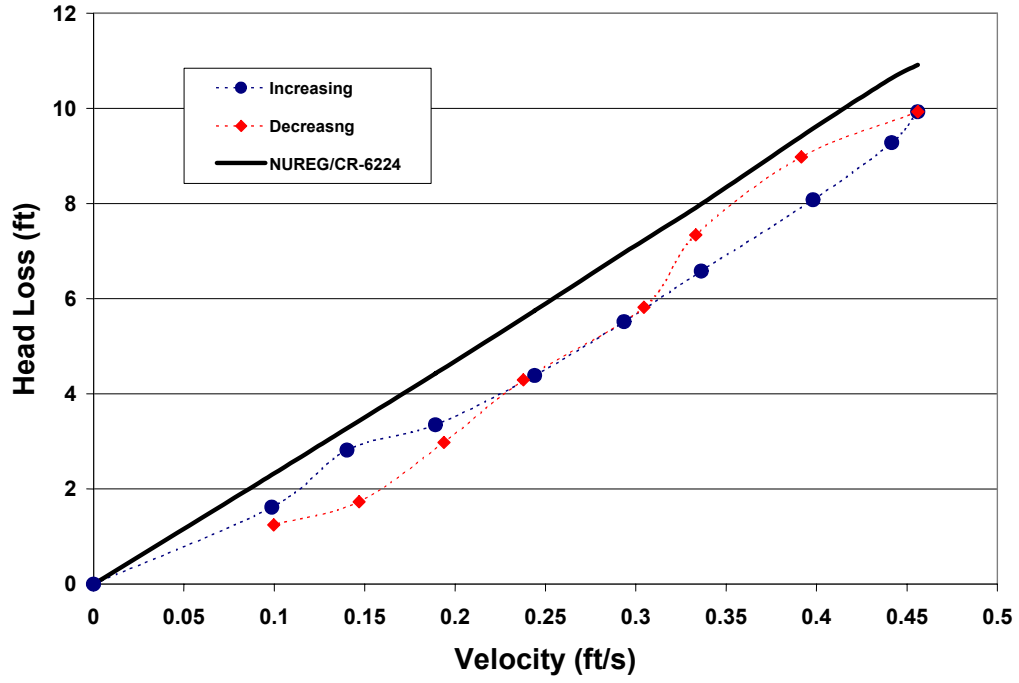
Fig. 52. Test results for Test 16.
