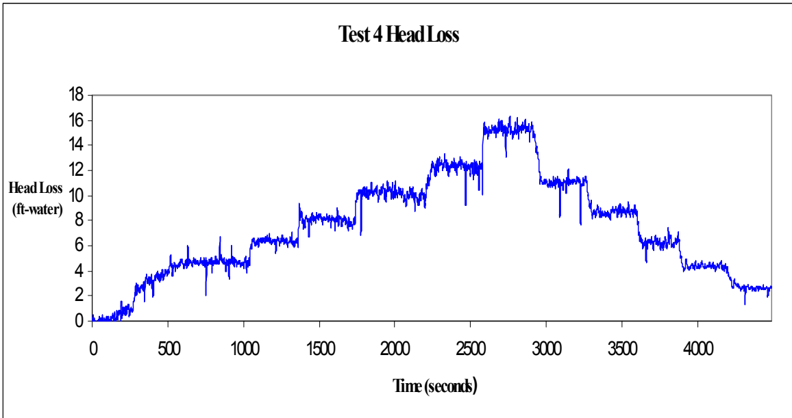
Fig. A-5. Time-dependent head-loss measurements.
