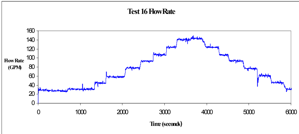
Fig. A-28. Time-dependent flow-rate measurements.
