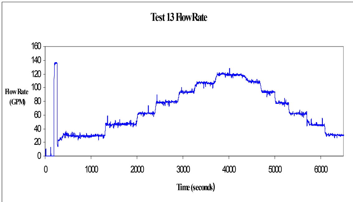
Fig. A-22. Time-dependent flow-rate measurements.
