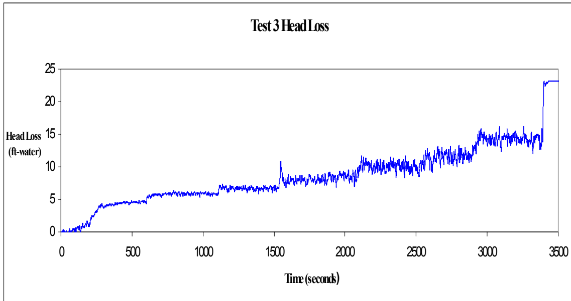
Fig. A-3. Time-dependent head-loss measurements.
