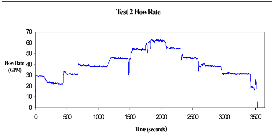
Fig. A-2. Time-dependent flow-rate measurements.
