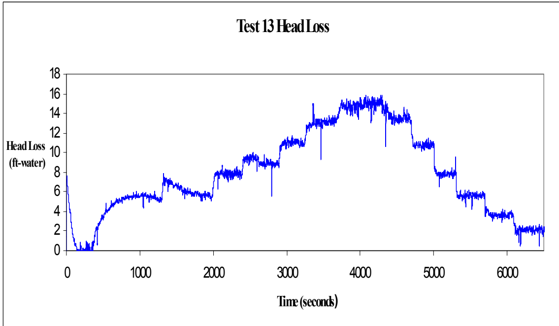
Fig. A-21. Time-dependent head-loss measurements.
