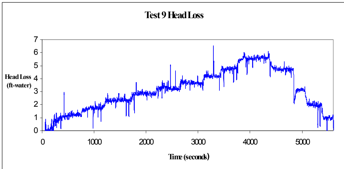
Fig. A-15. Time-dependent head-loss measurements.
