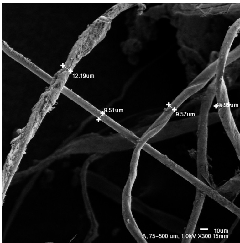
Fig. 33. SEM image of Plant-A fibers at 10 \mu\text{m} .
