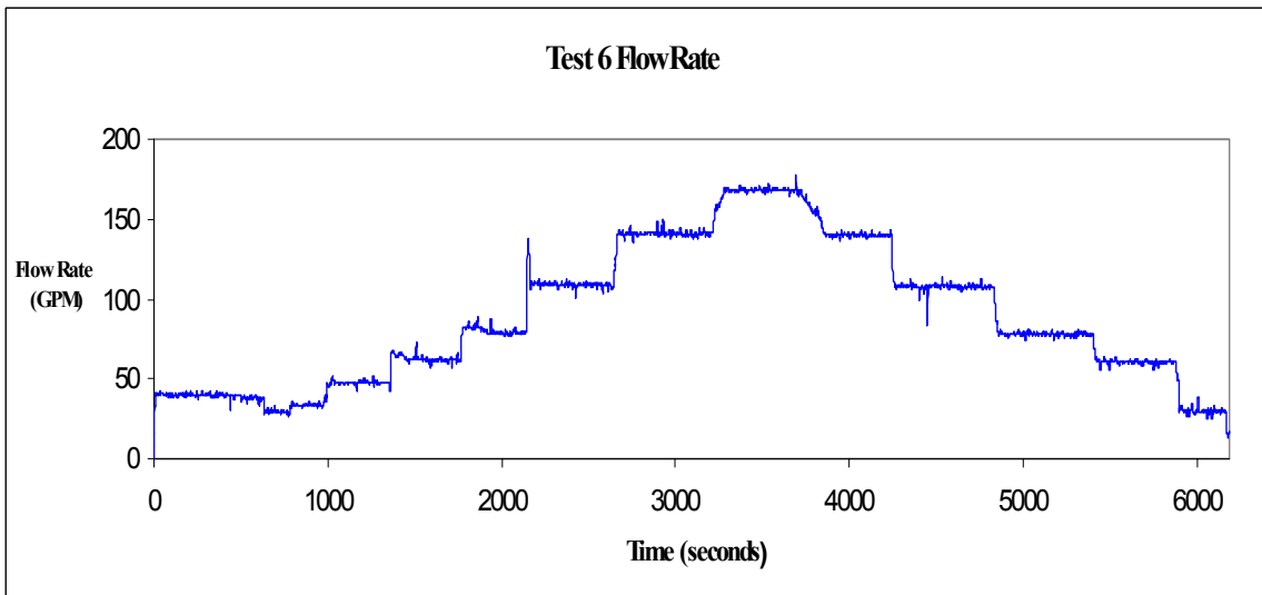
Fig. A-10. Time-dependent flow-rate measurements.
