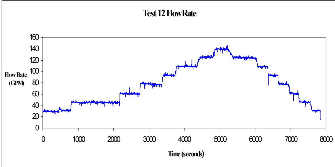
Fig. A-20. Time-dependent flow-rate measurements.
