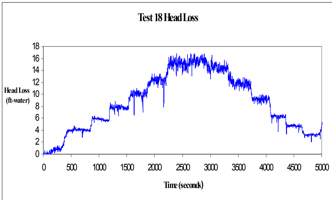
Fig. A-31. Time-dependent head-loss measurements.
