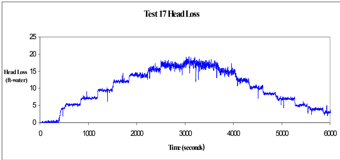
Fig. A-29. Time-dependent head-loss measurements.
