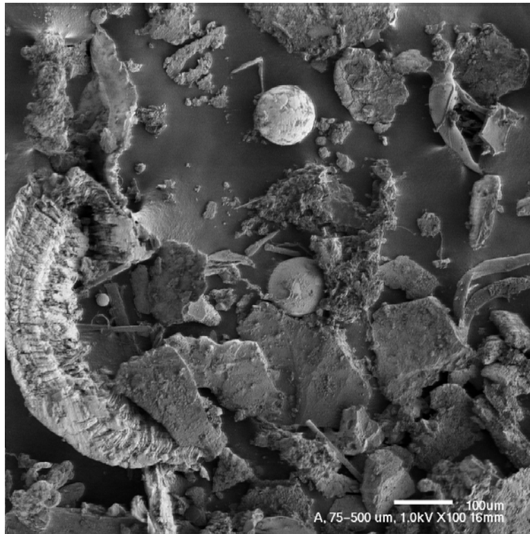
Fig. 36. SEM photo of 75- to 500- \mu m particles from Plant A.
