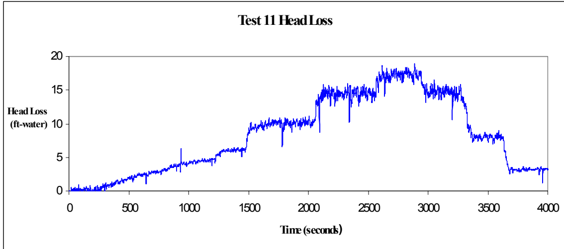
Fig. A-17. Time-dependent head-loss measurements.
