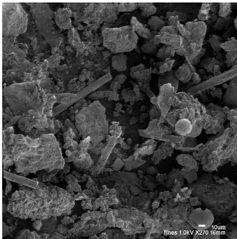
Fig. 37. SEM photo of fines <75 \mu m from Plant B.
