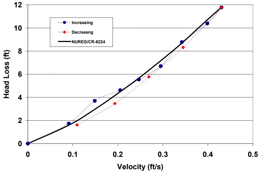
Fig. 55. Test results for Test 15.
