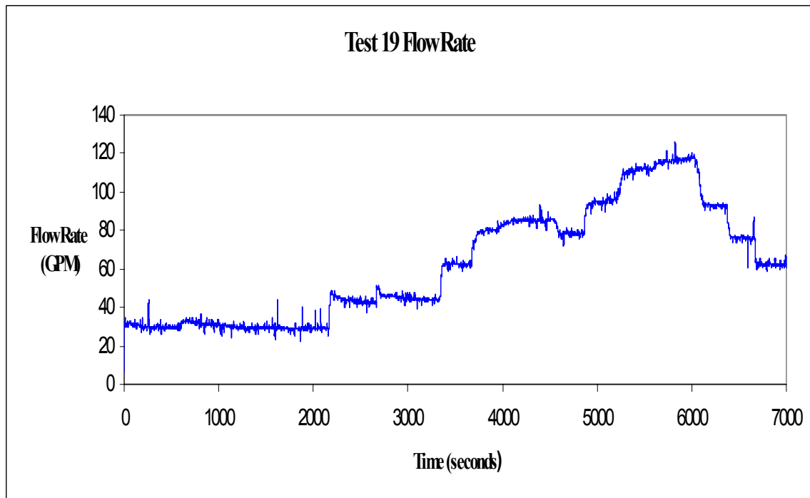
Fig. A-34. Time-dependent flow-rate measurements.
