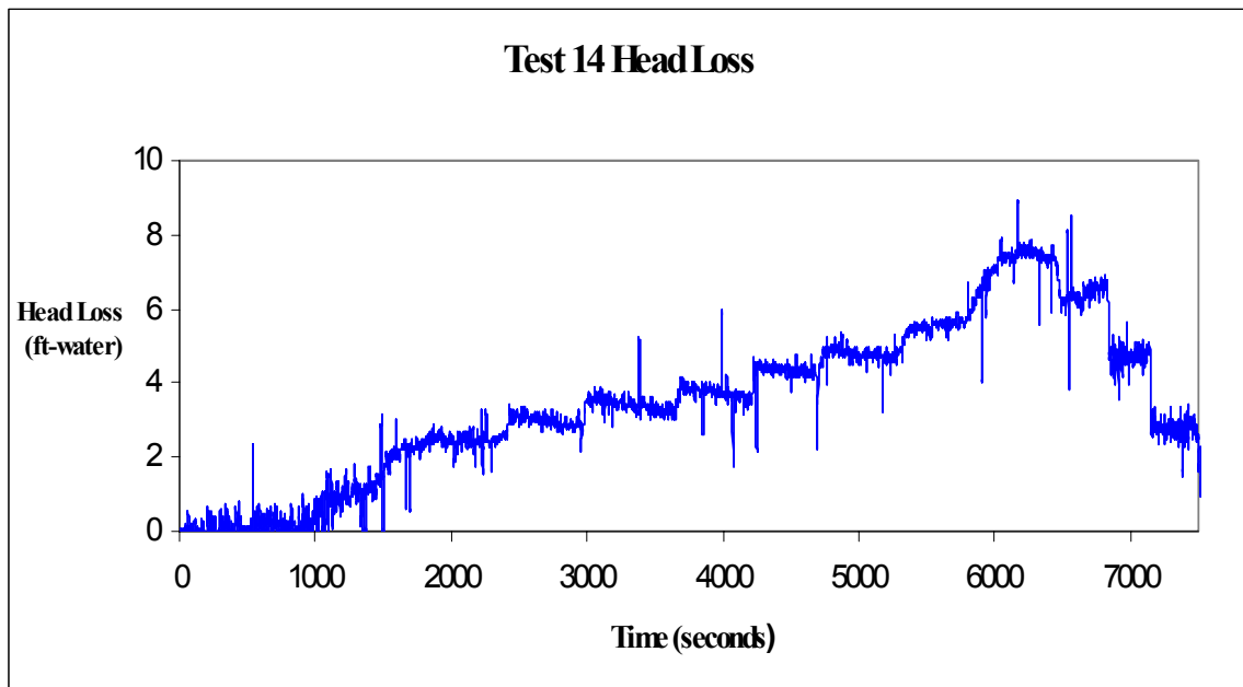
Fig. A-23. Time-dependent head-loss measurements.
