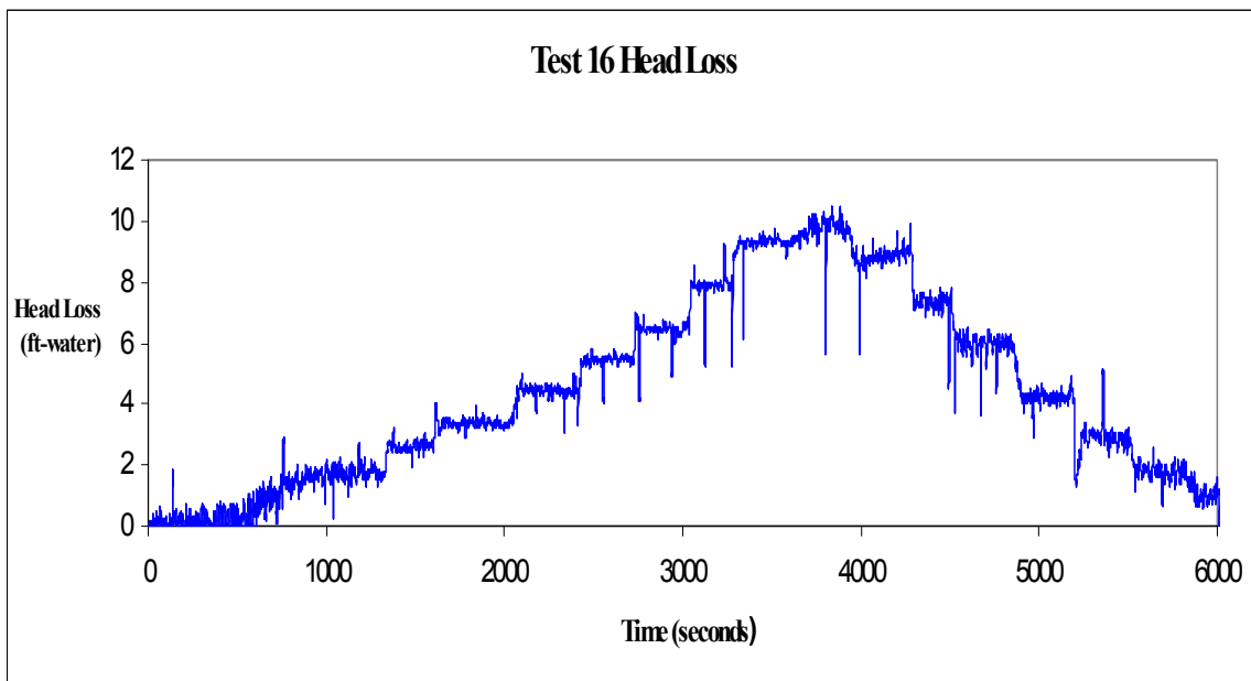
Fig. A-27. Time-dependent head-loss measurements.
