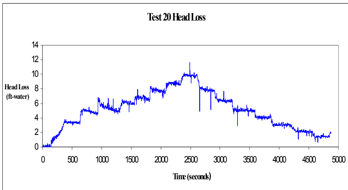
Fig. A-35. Time-dependent head-loss measurements.
