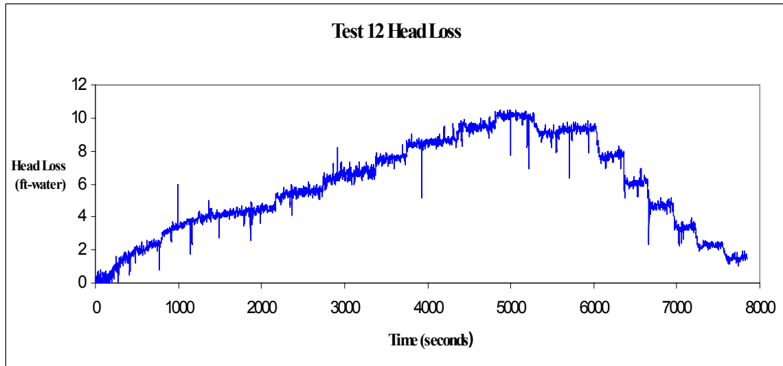
Fig. A-19. Time-dependent head-loss measurements.
