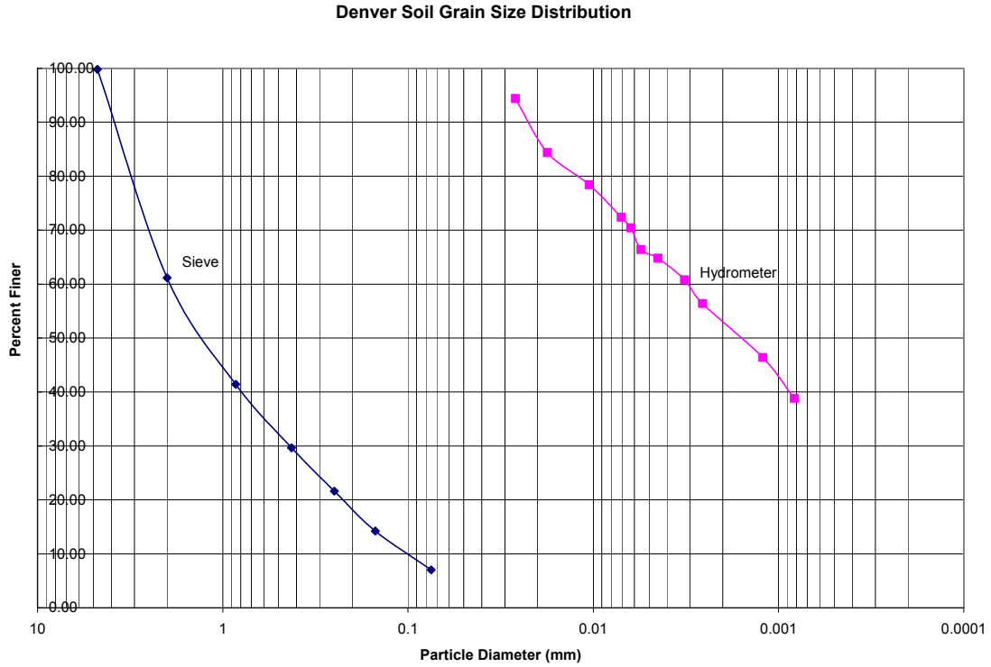
Fig. 46. Original grain-size distributions of bulk soil used to prepare surrogate particulate debris.
