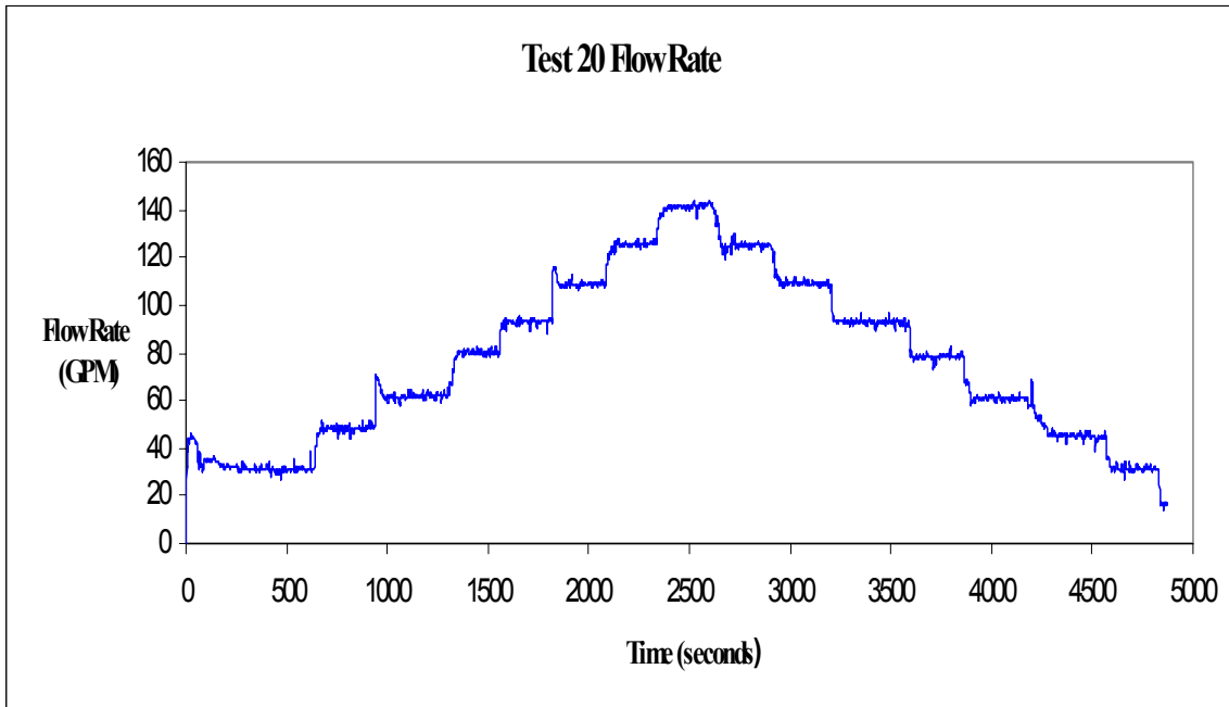
Fig. A-36. Time-dependent flow-rate measurements.
