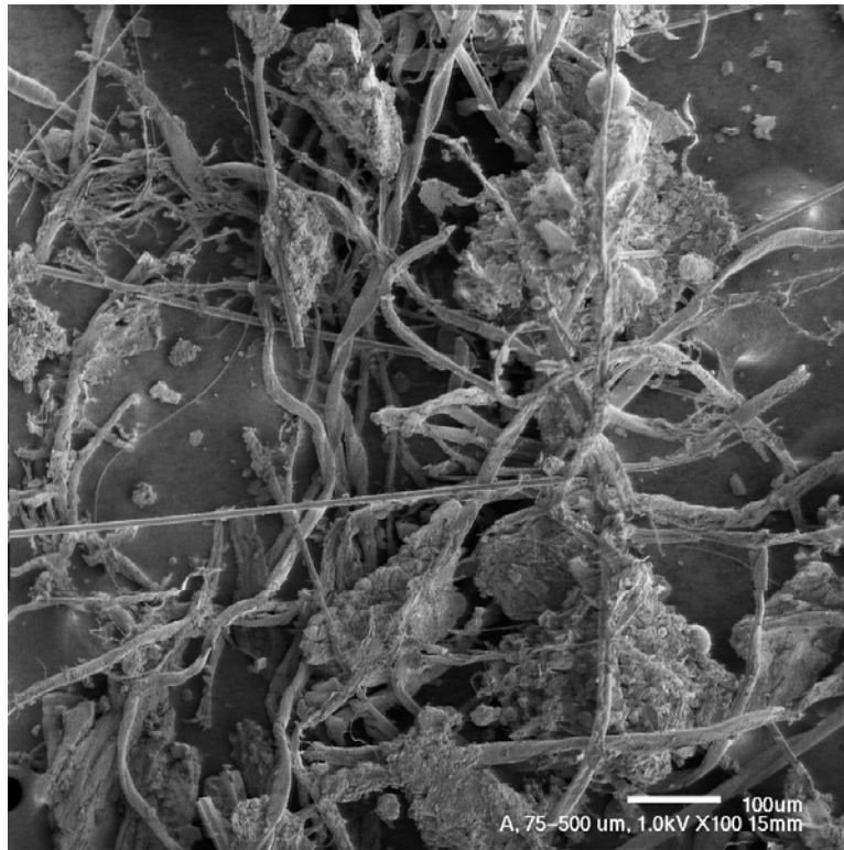
Fig. 32. SEM image of Plant-A fibers at 100 \mu\text{m} .
