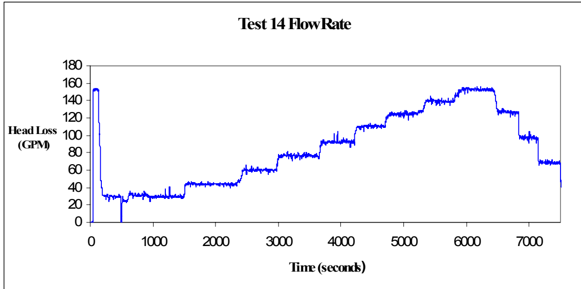
Fig. A-24. Time-dependent flow-rate measurements.
