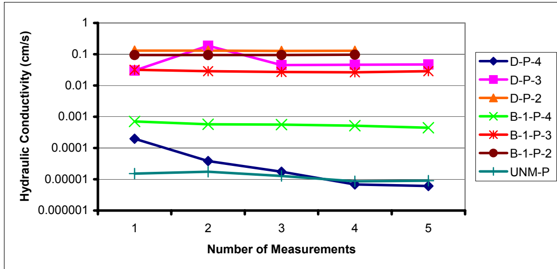
Fig. 50. Hydraulic conductivity of selected latent debris and surrogate soil.
