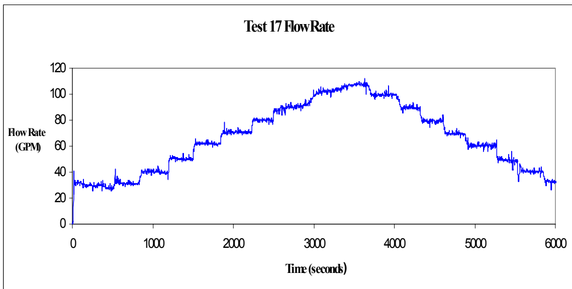
Fig. A-30. Time-dependent flow-rate measurements.
