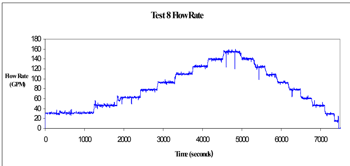
Fig. A-14. Time-dependent flow-rate measurements.
