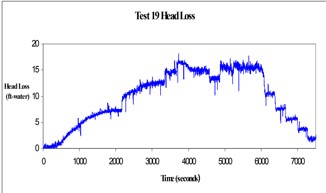
Fig. A-33. Time-dependent head-loss measurements.
