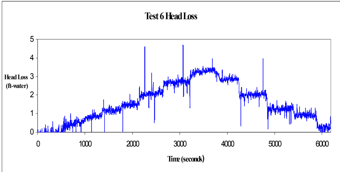
Fig. A-9. Time-dependent head-loss measurements.
