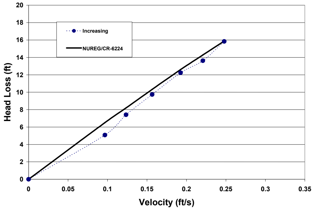
Fig. 57. Test results for Test 17.
