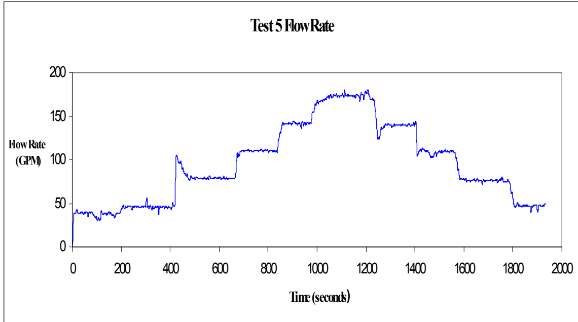
Fig. A-8. Time-dependent flow-rate measurements.
