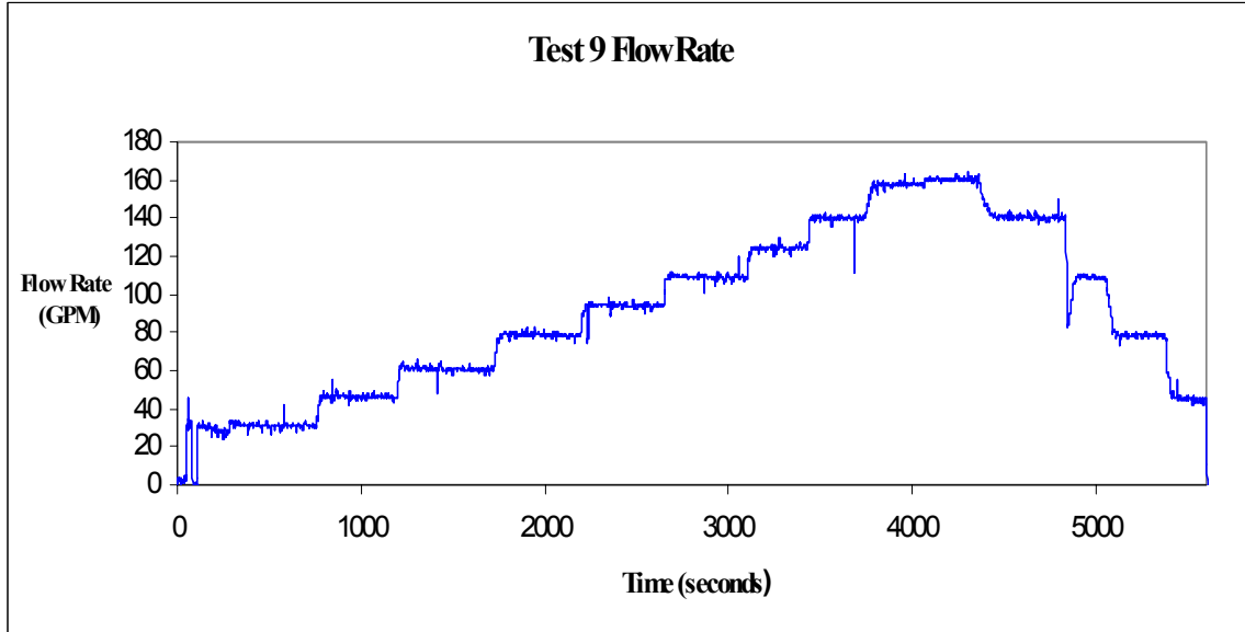
Fig. A-16. Time-dependent flow-rate measurements.
