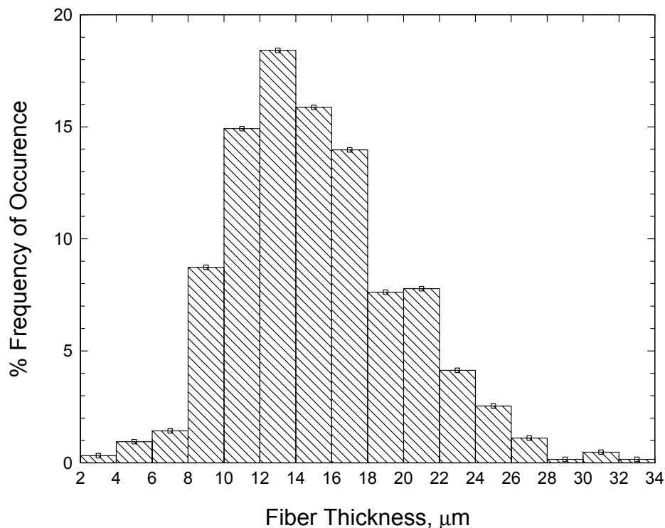
Fig. 41. Collective thickness/diameter distribution.
