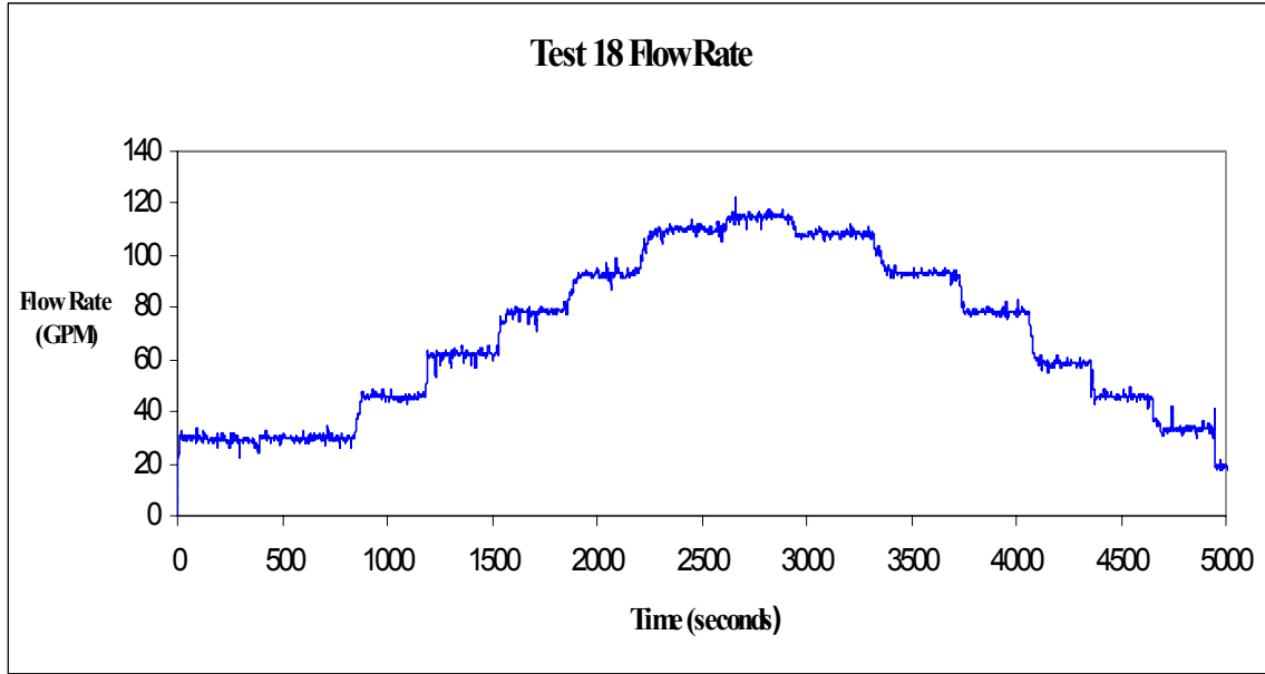
Fig. A-32. Time-dependent flow-rate measurements.
