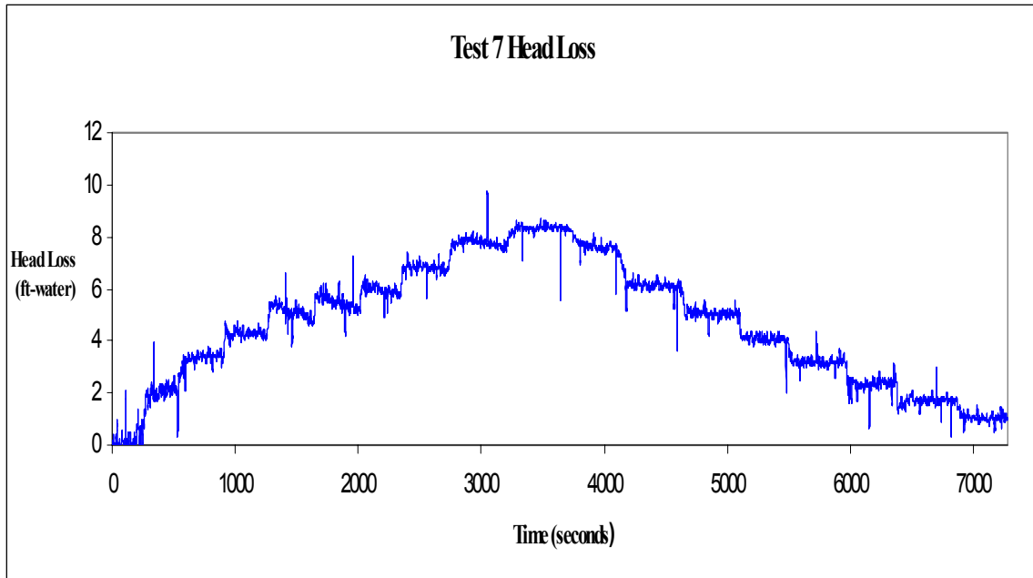
Fig. A-11. Time-dependent head-loss measurements.
