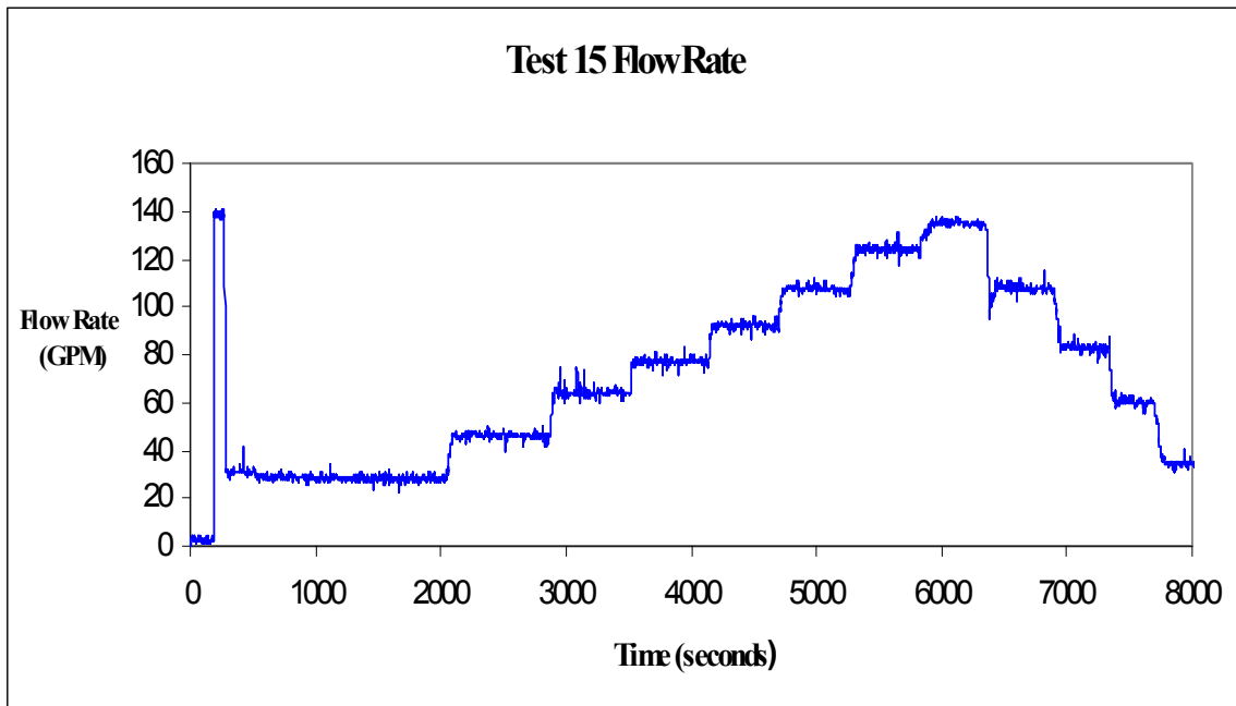
Fig. A-26. Time-dependent flow-rate measurements.
