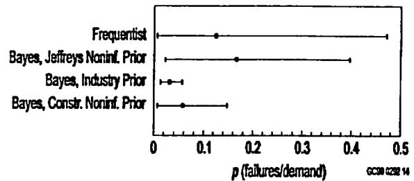
Figure 6.34 Comparison of four point estimates and interval estimates for p .
