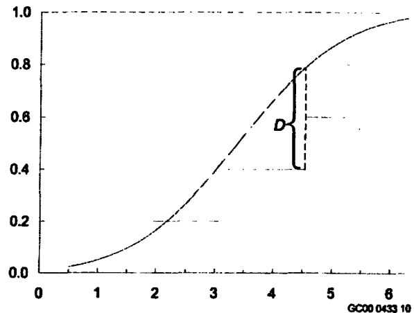
Figure B.3 The hypothesized distribution, the empirical distribution, and the Kolmogorov test statistic, D .
