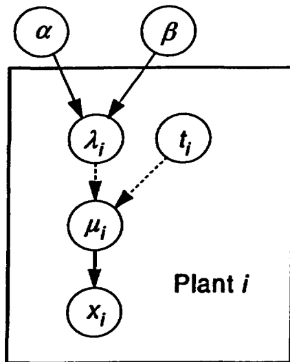
Figure 8.7 Directed graph for the hierarchical Bayes analysis of Example 8.1.
