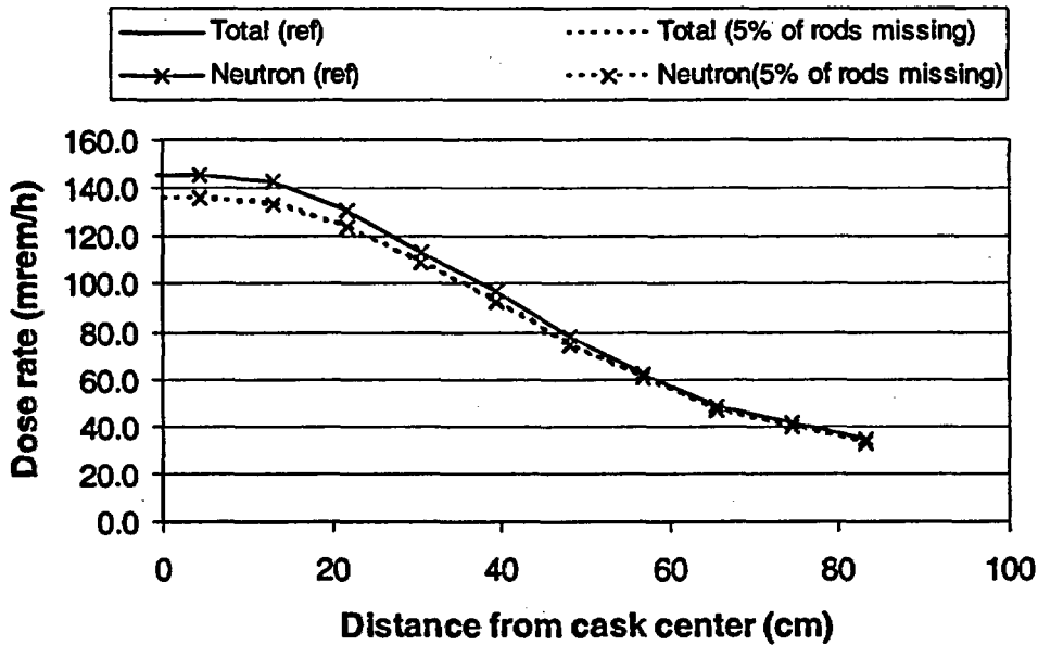
Figure 30 Effect of missing 5% of the fuel rods on dose rate profiles along the bottom surface of the GBC-32 cask (5 wt % 235 U enrichment, 75-GWd/MTU burnup, 20-year cooling). Note that the dose rate curves for the two cases are virtually indistinguishable.
