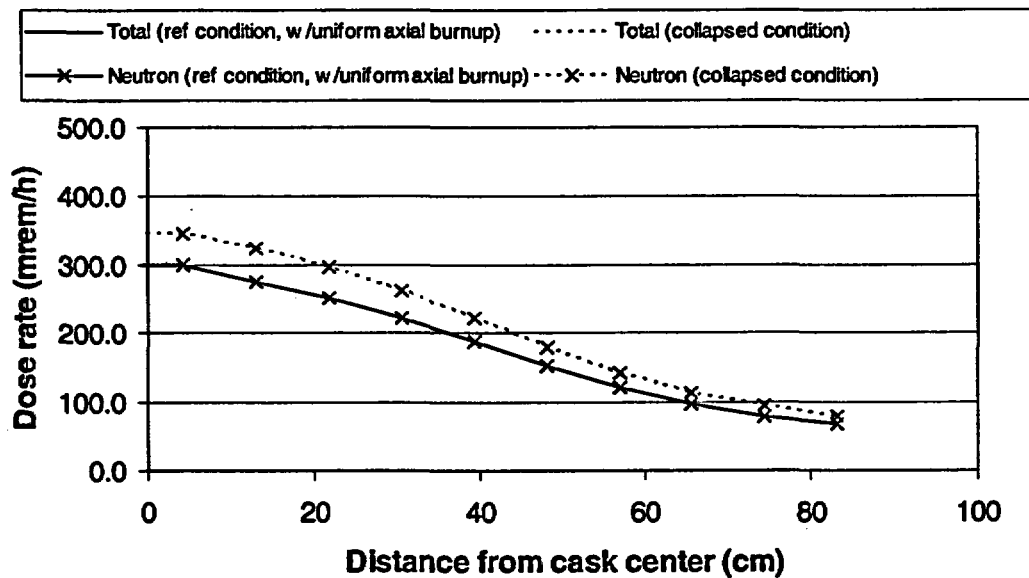
Figure 36 Comparison of surface dose rate profiles along the bottom of the GBC-32 cask (5 wt % 235 U enrichment, 75-GWd/MTU burnup, 20-year cooling)
