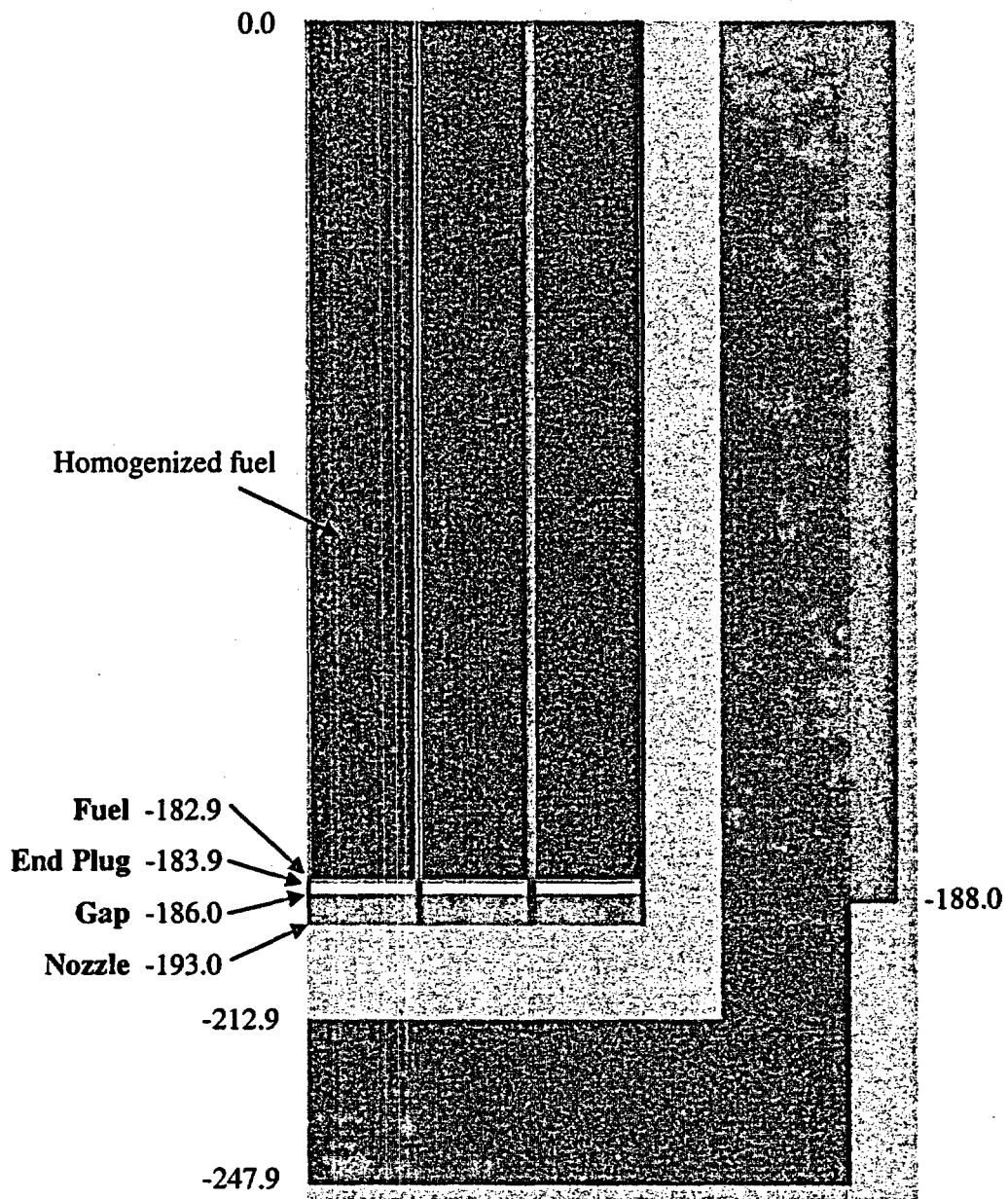
Figure 24 Axial cross section of SAS4 model of the GBC-32 cask (dimensions in units of centimeters)
