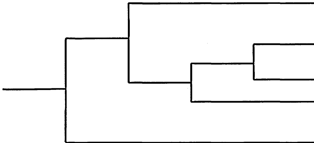
Figure A-2 ATWS Rule Event Tree for General Electric Reactor Group Automatic Standby Liquid Control System
