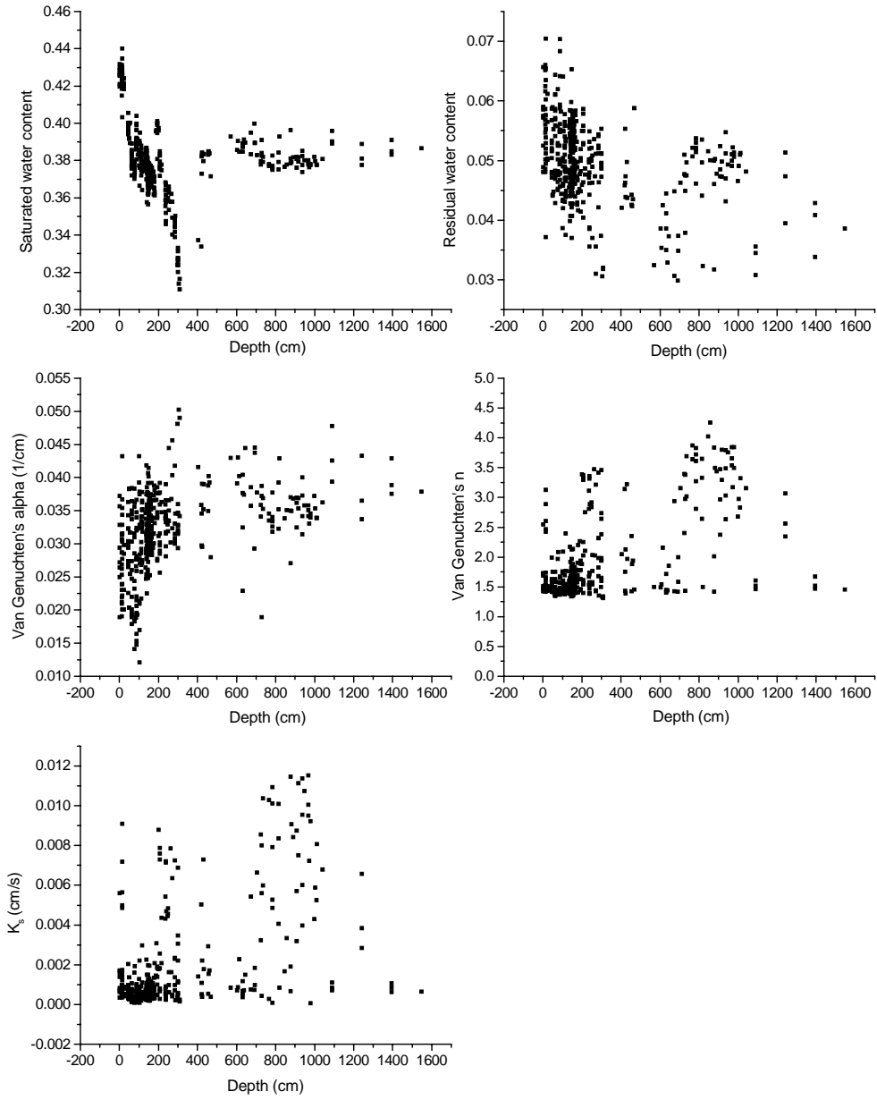
Figure 11-12. Hydraulic parameters at the MAC using Rosetta software with site-specific soil component (all the depths) and bulk density data (above 5 m).
