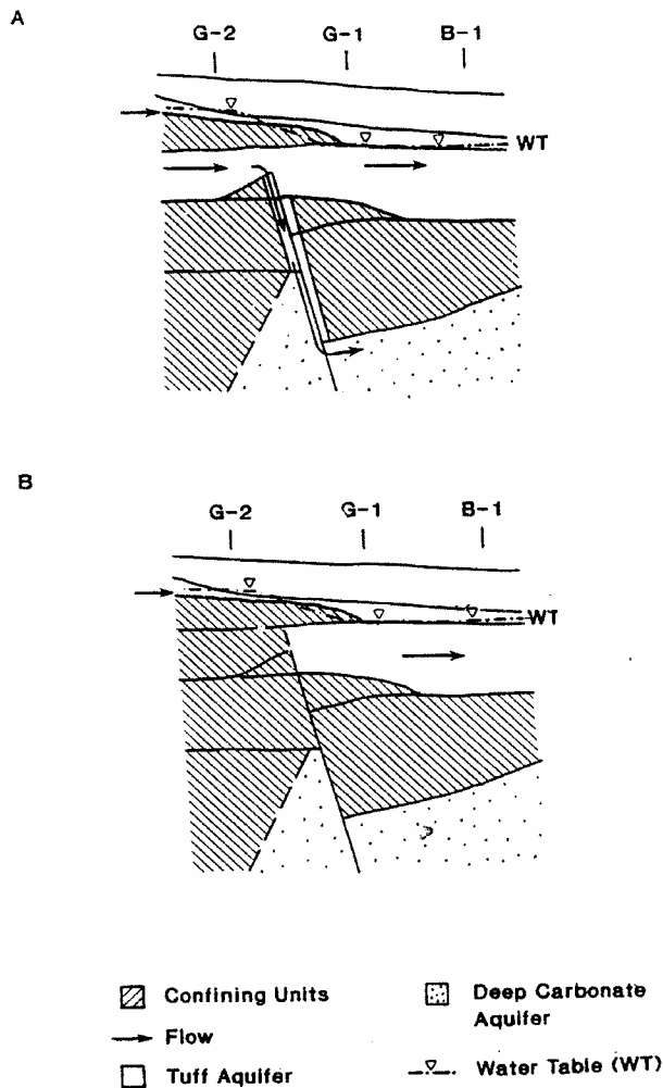
Figure 5-8. Drain (A) and spillway (B) models with section showing postulated buried graben (after Fridrich et al. , 1994).
