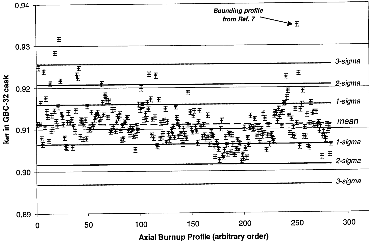
Figure B.6 Plot of k_{eff} values for axial burnup profiles in burnup group 6 ( 26 < \text{burnup} < 30 GWd/MTU). Total number of profiles in this burnup group is 283.
