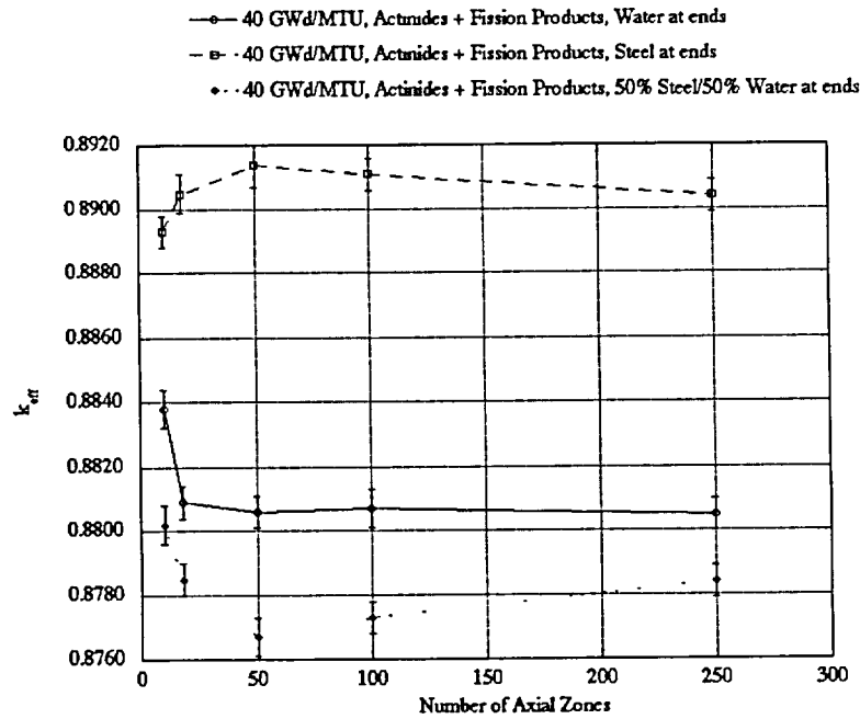
Figure A.14 Computed results for 40 GWd/MTU burnup fuel, actinides and fission products
