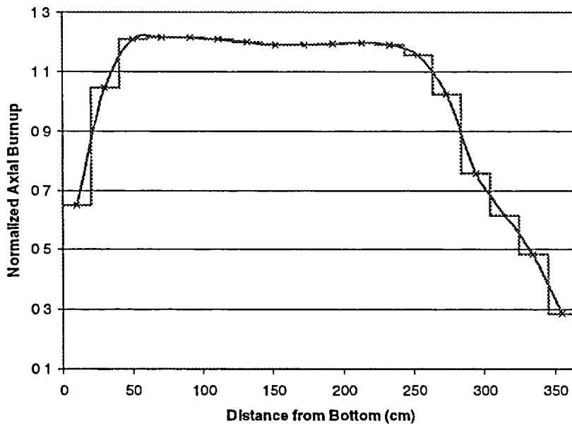
Figure 15 Bounding profile for burnup group 9 (14 < burnup < 18 GWd/MTU)
