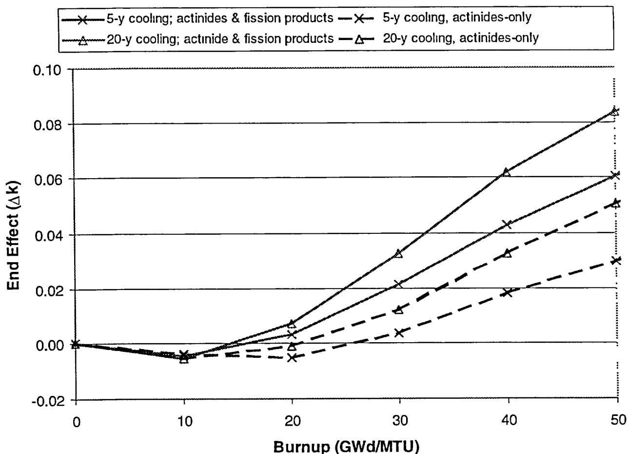
Figure 2 Example of end effect as a function of burnup for two cooling times with and without fission products present
