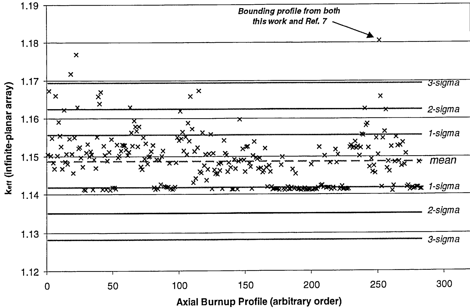
Figure 24 Plot of k_{eff} values for axial-burnup profiles in burnup group 6 ( 26 < \text{burnup} < 30 \text{ GWd/MTU} ). Total number of profiles in this burnup group is 283.
