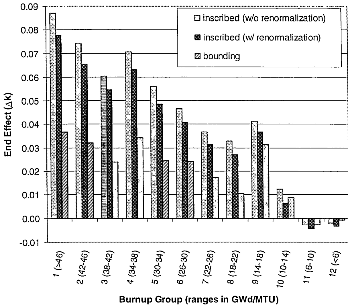
Figure 59 Illustration of the impact of profile inscribing (with and without profile renormalization) on the end effect in the GBC-32 cask with fission products present (5-year cooling)
