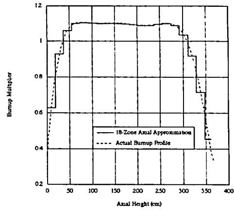
Figure A.3 18-Zone axial-burnup model
