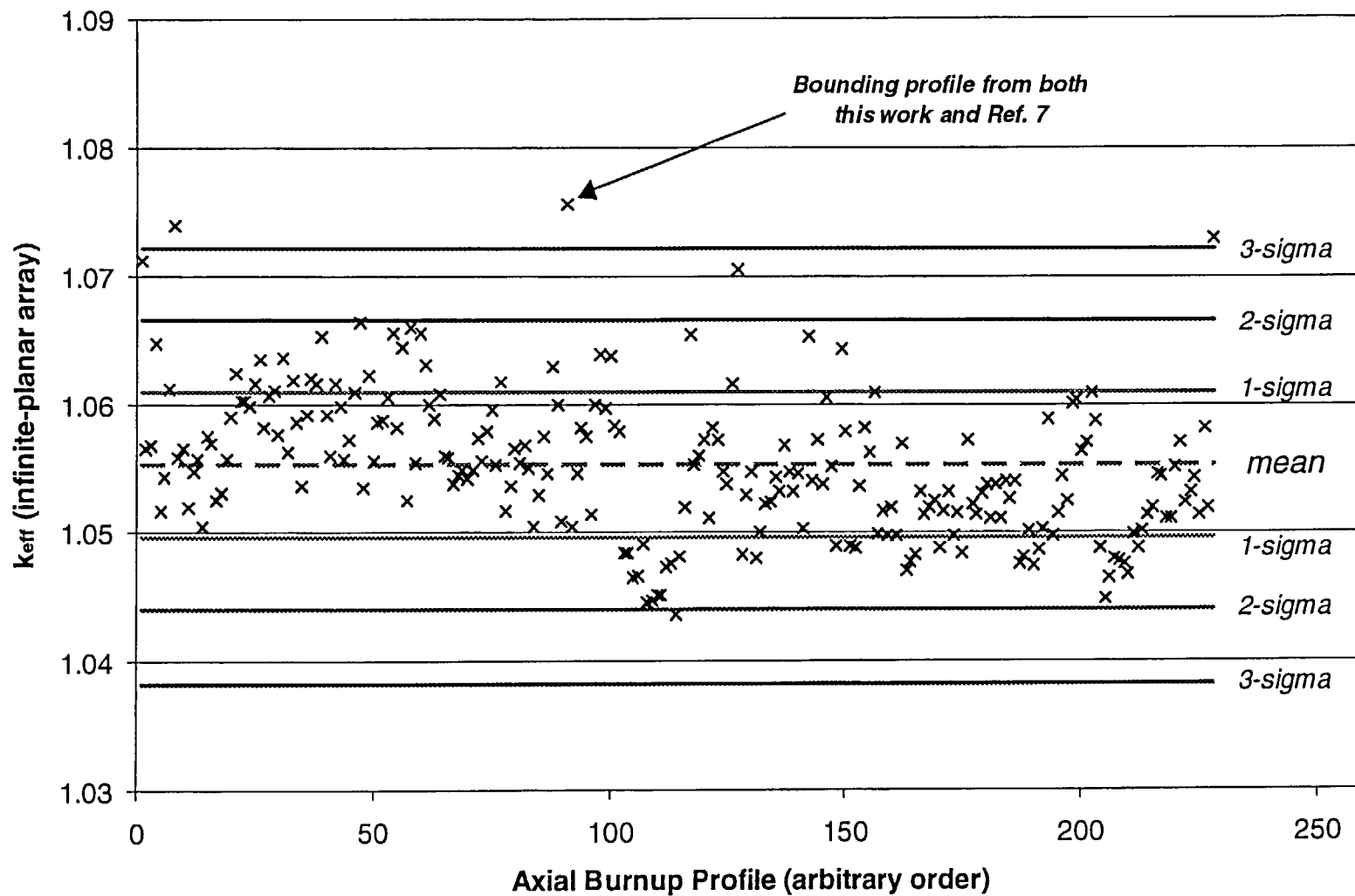
Figure 21 Plot of k_{eff} values for axial-burnup profiles in burnup group 3 ( 38 < \text{burnup} < 42 GWd/MTU). Total number of profiles in this burnup group is 228.
