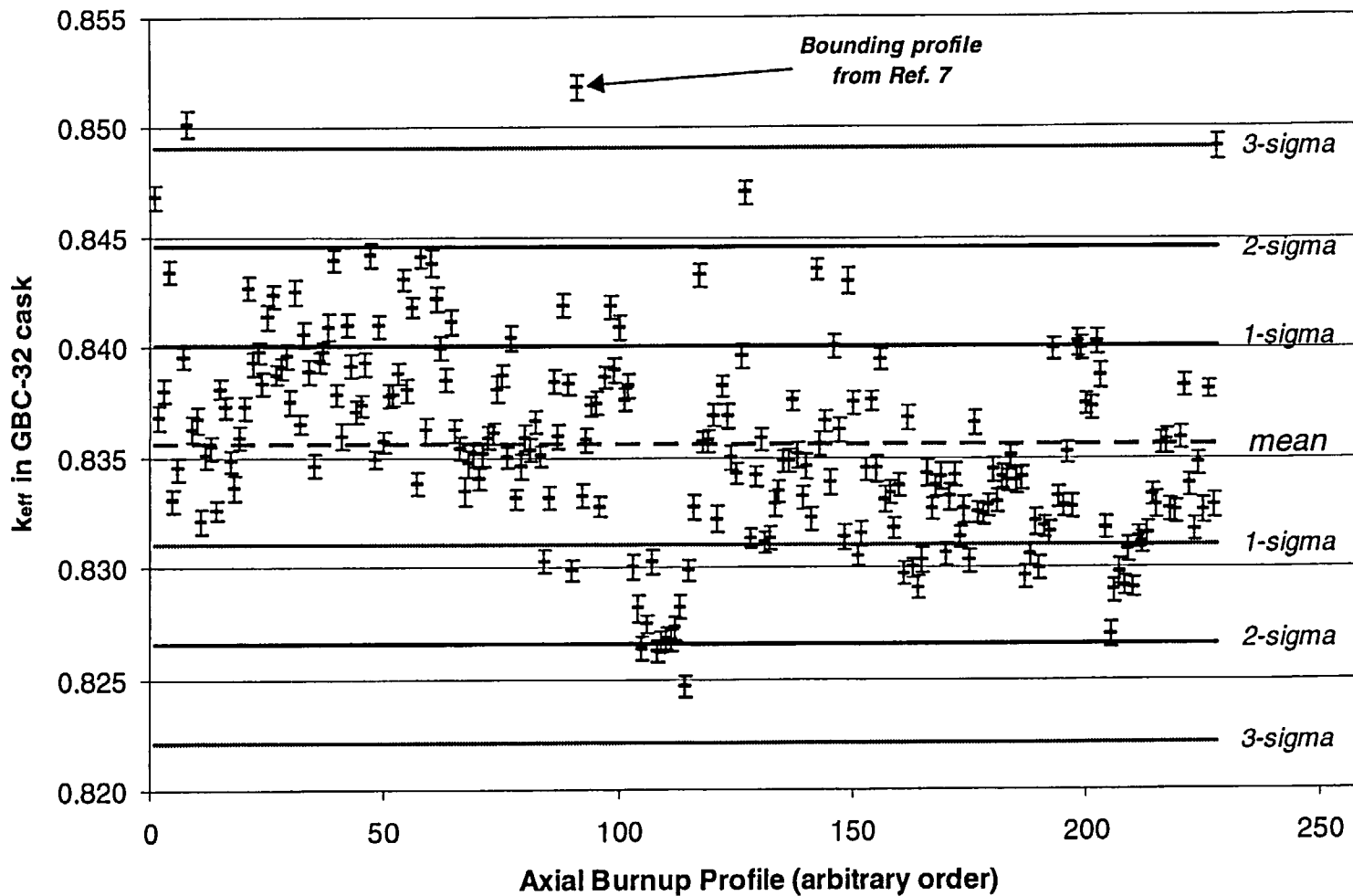
Figure B.3 Plot of k_{eff} values for axial burnup profiles in burnup group 3 ( 38 < \text{burnup} < 42 GWd/MTU). Total number of profiles in this burnup group is 228.
