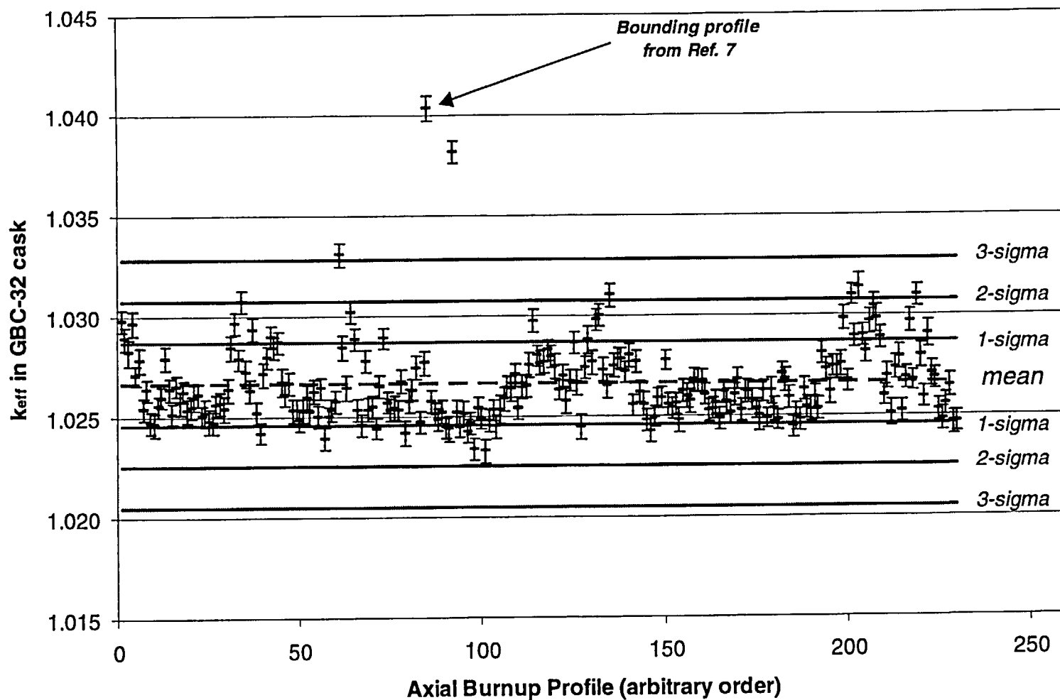
Figure B.10 Plot of k_{eff} values for axial burnup profiles in burnup group 10 ( 10 < \text{burnup} < 14 \text{ GWd/MTU} ). Total number of profiles in this burnup group is 230.
