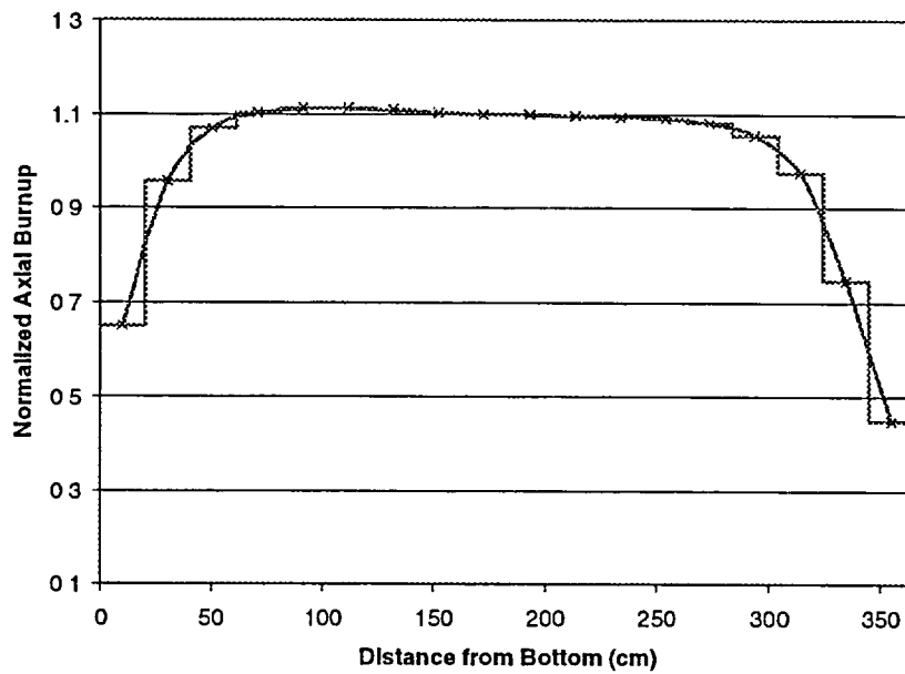
Figure 10 Bounding profile for burnup group 4 ( 34 < \text{burnup} < 38 GWd/MTU)
