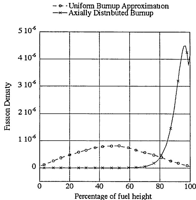
Figure A.1 Comparison of fission densities computed for uniform and axially distributed burnup profiles
