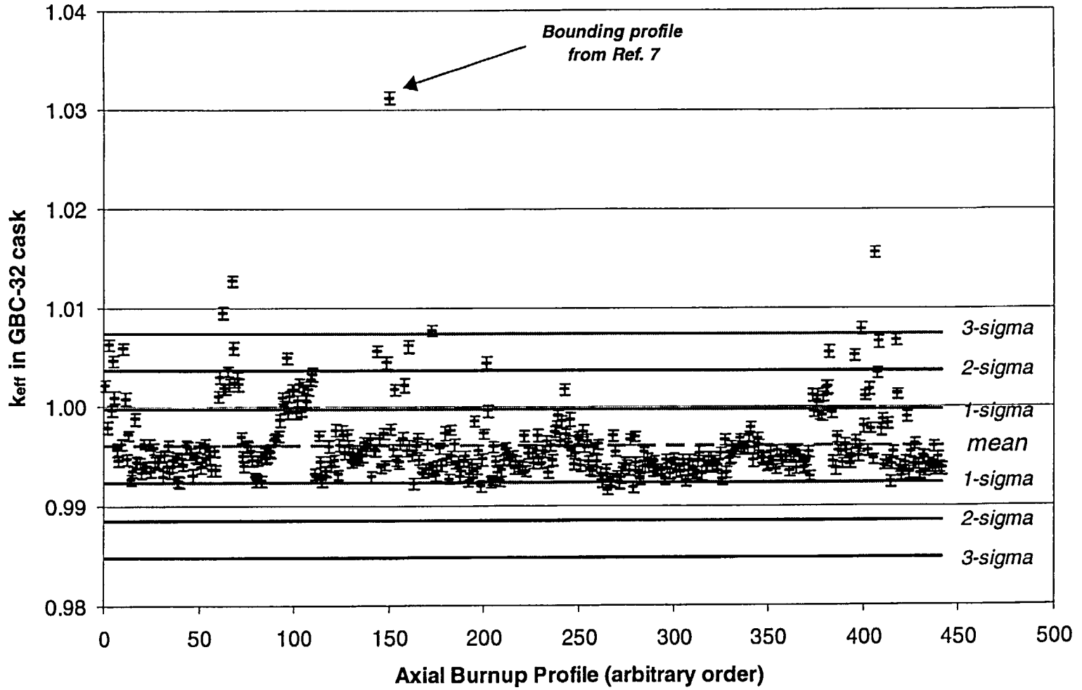
Figure B.9 Plot of k_{eff} values for axial burnup profiles in burnup group 9 ( 14 < \text{burnup} < 18 \text{ GWd/MTU} ). Total number of profiles in this burnup group is 441.
