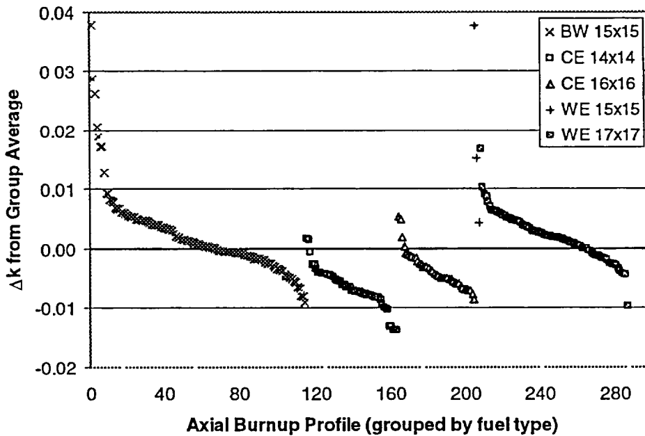
Figure 33 \Delta k values plotted in terms of fuel type for axial-burnup profiles in burnup group 3 ( 38 < \text{burnup} < 42 \text{ GWd/MTU} )
