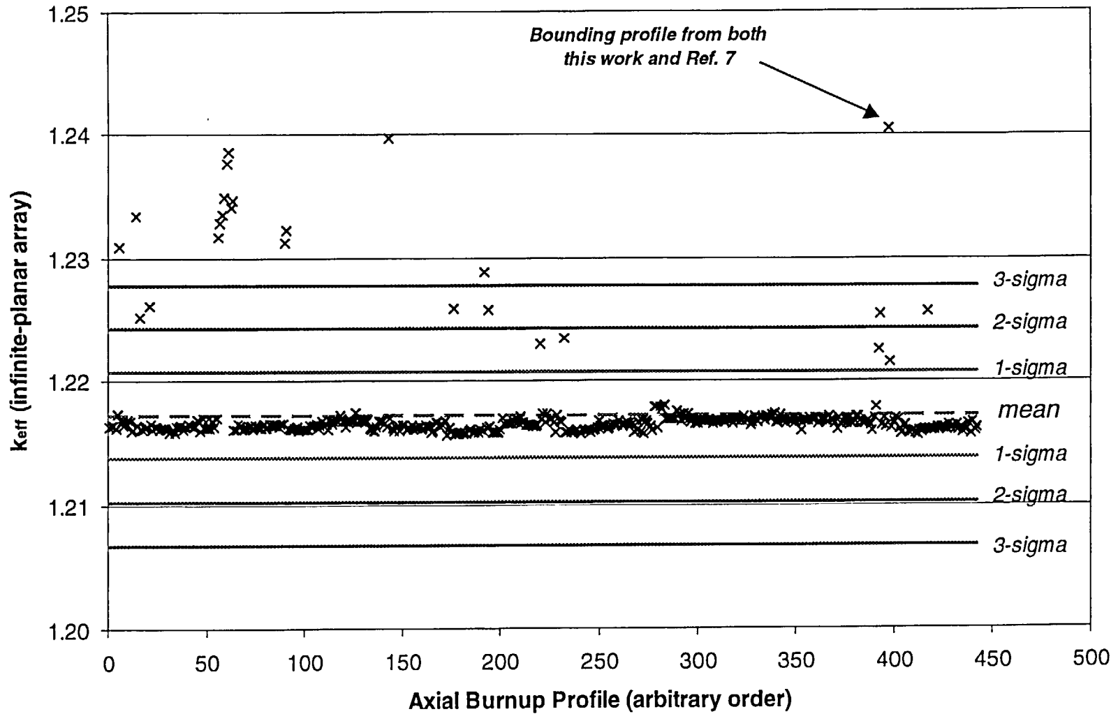
Figure 26 Plot of k_{eff} values for axial-burnup profiles in burnup group 8 ( 18 < \text{burnup} < 22 GWd/MTU). Total number of profiles in this burnup group is 442.
