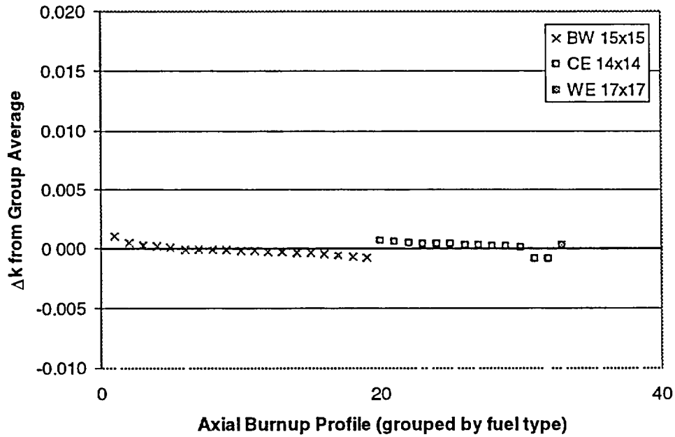
Figure 42 \Delta k values plotted in terms of fuel type for axial-burnup profiles in burnup group 12 ( \text{burnup} < 6 \text{ GWd/MTU} )
