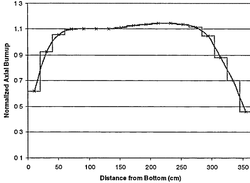
Figure 12 Bounding profile for burnup group 6 (26 < burnup < 30 GWd/MTU)
