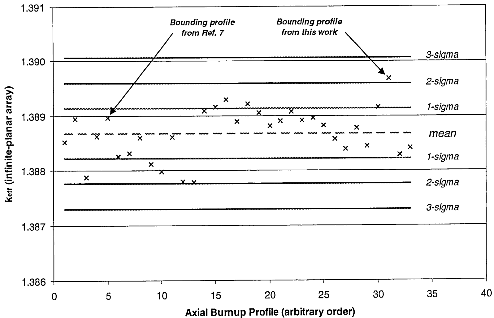
Figure 30 Plot of k_{eff} values for axial-burnup profiles in burnup group 12 (burnup < 6 GWd/MTU). Total number of profiles in this burnup group is 33.
