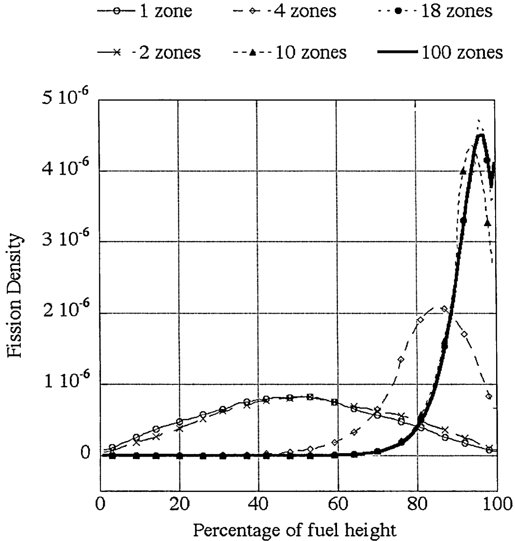
Figure A.18 Fission density profiles for different burnup discretization approximations
