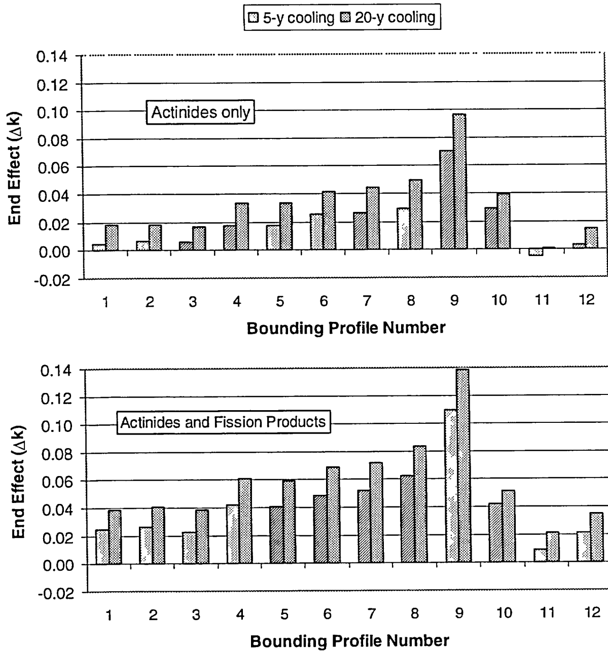
Figure 57 Comparison of end effect values resulting from the use of the 12 bounding profiles (from Table 5) for a fixed burnup of 40 GWd/MTU
