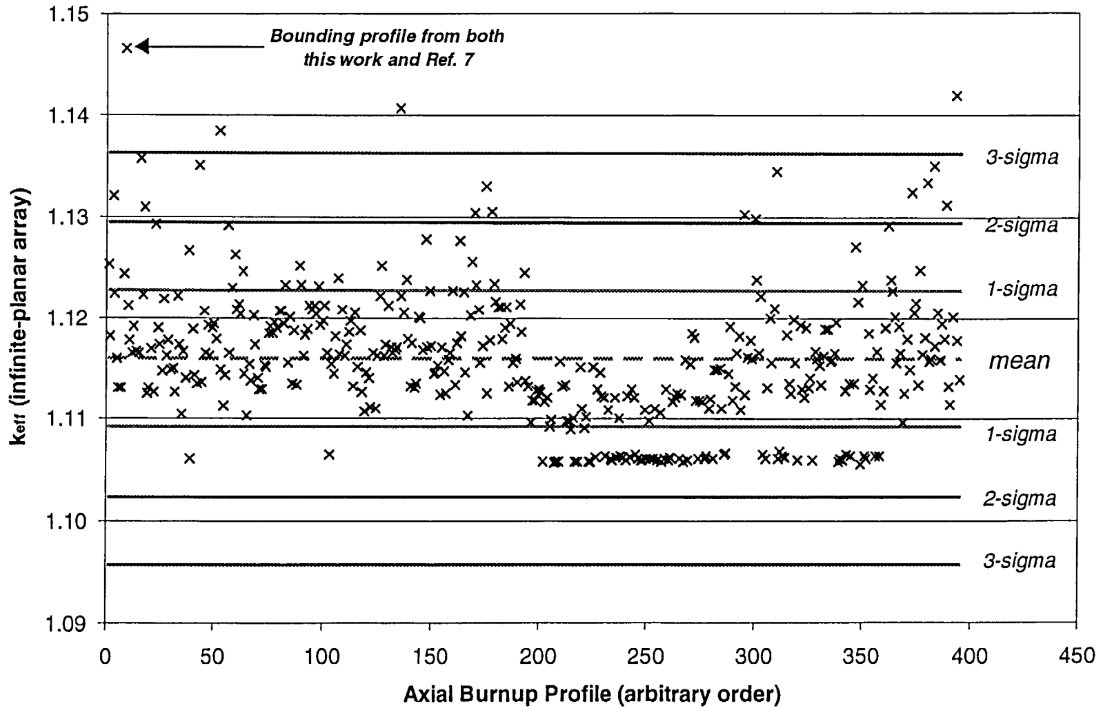
Figure 23 Plot of k_{eff} values for axial-burnup profiles in burnup group 5 ( 30 < \text{burnup} < 34 GWd/MTU). Total number of profiles in this burnup group is 395.
