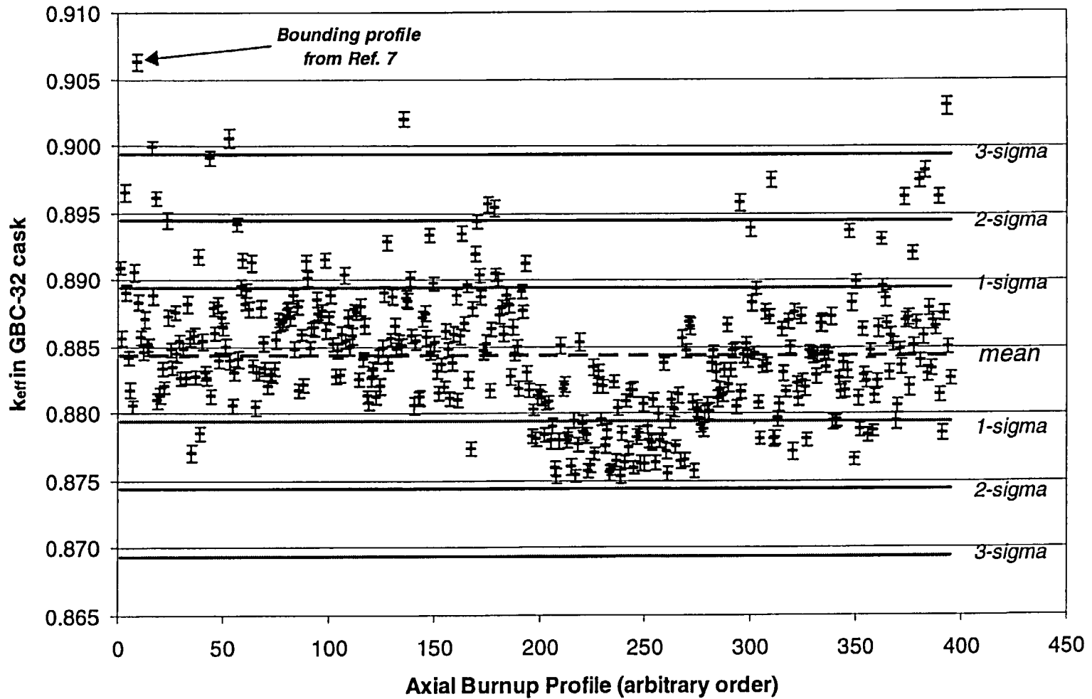
Figure B.5 Plot of k_{eff} values for axial burnup profiles in burnup group 5 ( 30 < \text{burnup} < 34 \text{ GWd/MTU} ). Total number of profiles in this burnup group is 395.
