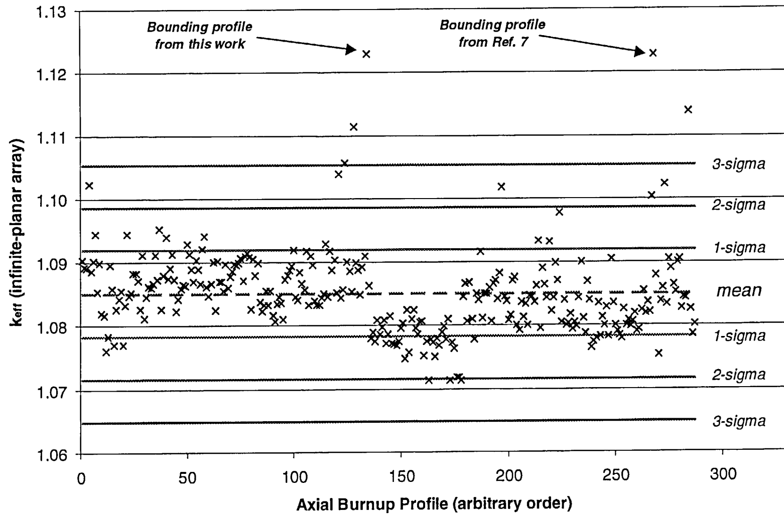
Figure 22 Plot of k_{eff} values for axial-burnup profiles in burnup group 4 ( 34 < \text{burnup} < 38 \text{ GWd/MTU} ). Total number of profiles in this burnup group is 287.
