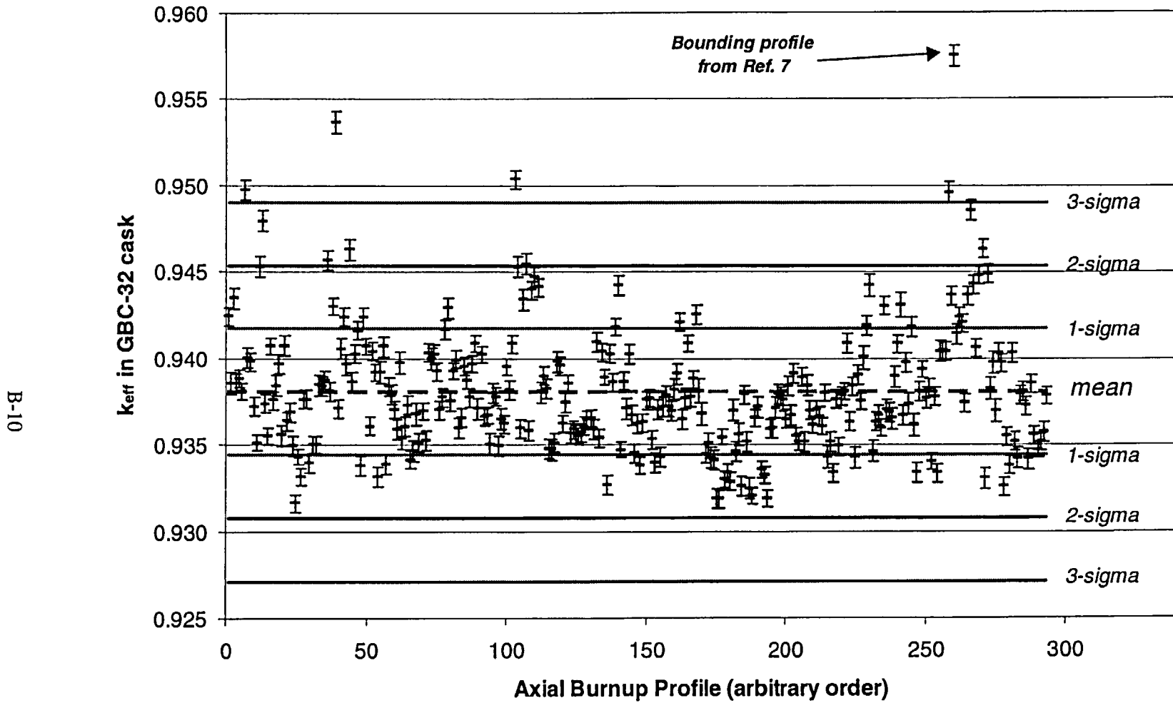
Figure B.7 Plot of k_{eff} values for axial burnup profiles in burnup group 7 ( 22 < \text{burnup} < 26 \text{ GWd/MTU} ). Total number of profiles in this burnup group is 293.
