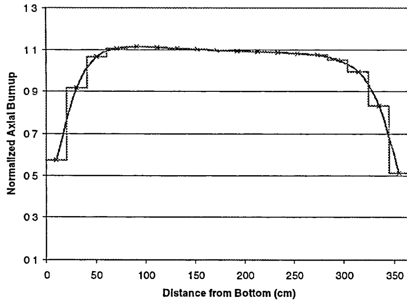
Figure 7 Bounding profile for burnup group 1 (burnup > 46 GWd/MTU)
