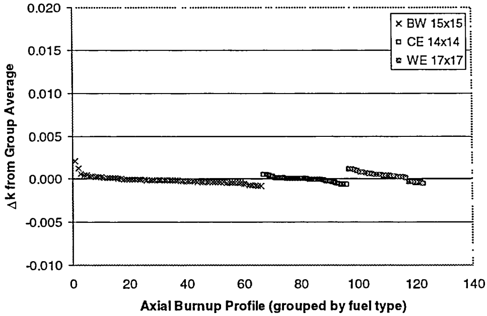
Figure 41 \Delta k values plotted in terms of fuel type for axial-burnup profiles in burnup group 11 ( 6 < \text{burnup} < 10 \text{ GWd/MTU} )
