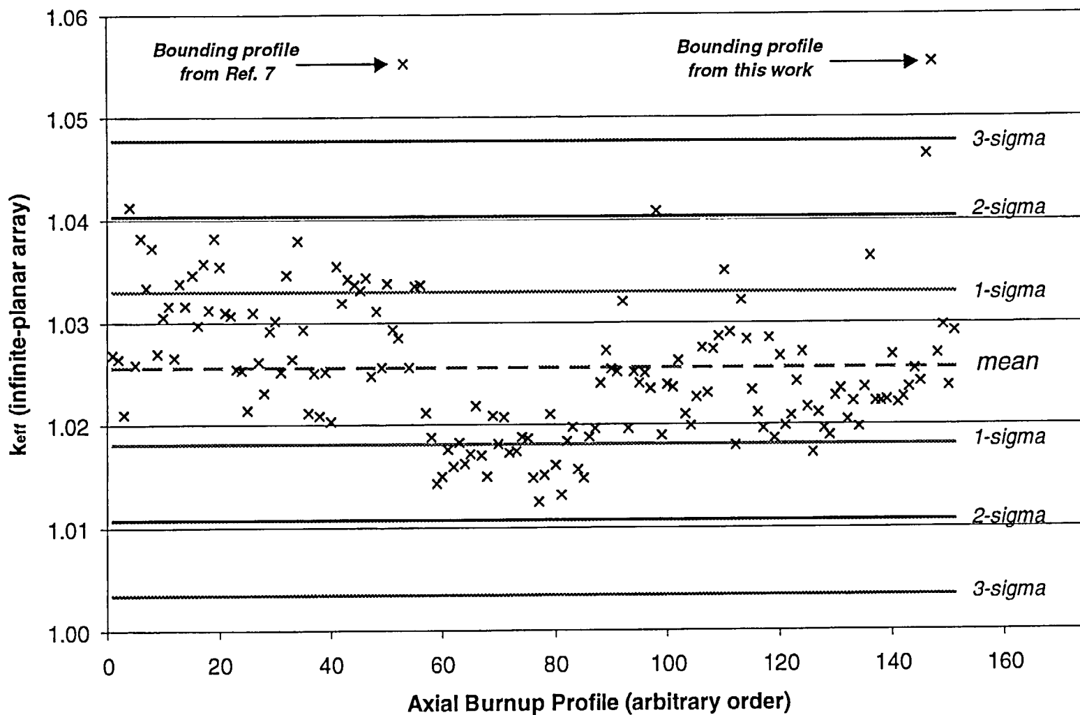
Figure 20 Plot of k_{eff} values for axial-burnup profiles in burnup group 2 ( 42 < \text{burnup} < 46 GWd/MTU). Total number of profiles in this burnup group is 151.
