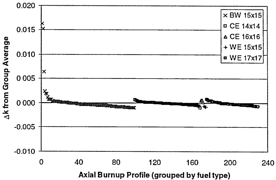
Figure 40 \Delta k values plotted in terms of fuel type for axial-burnup profiles in burnup group 10 ( 10 < \text{burnup} < 14 \text{ GWd/MTU} )
