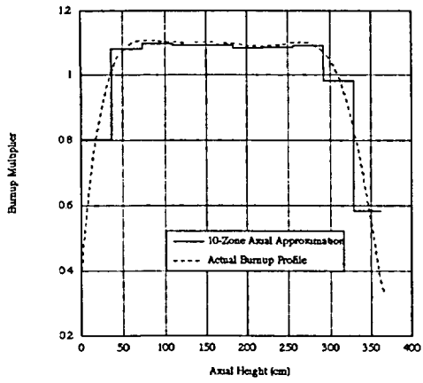
Figure A.2 10-Zone axial-burnup model
