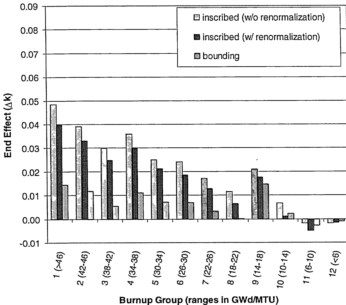
Figure 60 Illustration of the impact of profile inscribing (with and without profile renormalization) on the end effect in the GBC-32 cask without fission products present (5-year cooling)
