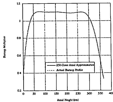
Figure A.6 250-Zone axial-burnup model
