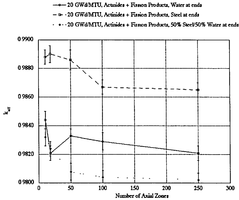
Figure A.12 Computed results for 20 GWd/MTU burnup fuel, actinides and fission products
