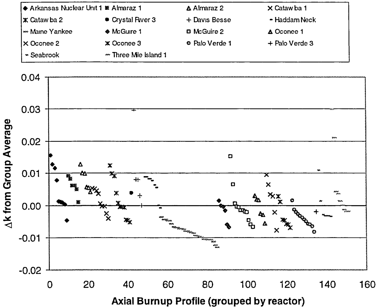
Figure 44 \Delta k values plotted in terms of reactor for axial-burnup profiles in burnup group 2 (42 < burnup < 46 GWd/MTU)
