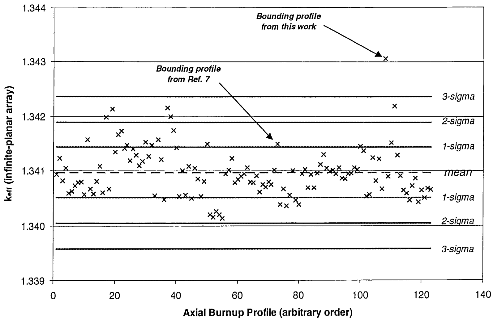
Figure 29 Plot of k_{eff} values for axial-burnup profiles in burnup group 11 ( 6 < \text{burnup} < 10 GWd/MTU). Total number of profiles in this burnup group is 123.
