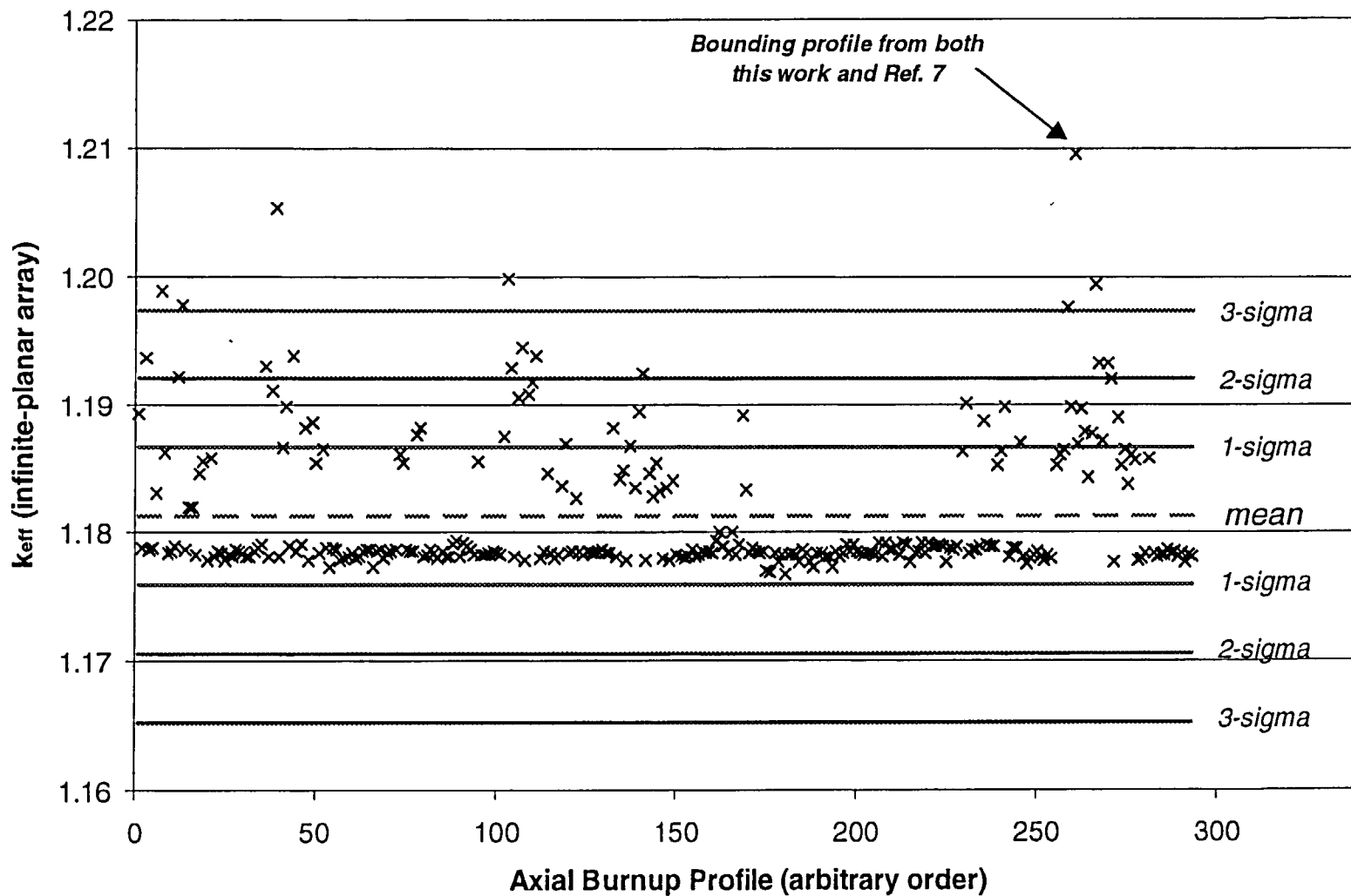
Figure 25 Plot of k_{eff} values for axial-burnup profiles in burnup group 7 ( 22 < \text{burnup} < 26 GWd/MTU). Total number of profiles in this burnup group is 293.
