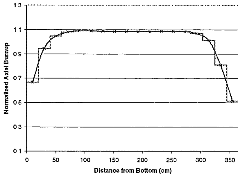
Figure 8 Bounding profile for burnup group 2 (42 < burnup < 46 GWd/MTU)
