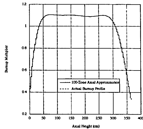
Figure A.5 100-Zone axial-burnup model
