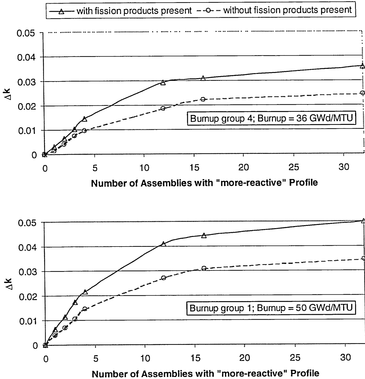
Figure 61 \Delta k consequence of loading various numbers of assemblies with a "more reactive" axial-burnup profile (based on inscribing) into the GBC-32 cask in which the remaining assemblies have the "actual bounding" axial-burnup profile (5-year cooling)
