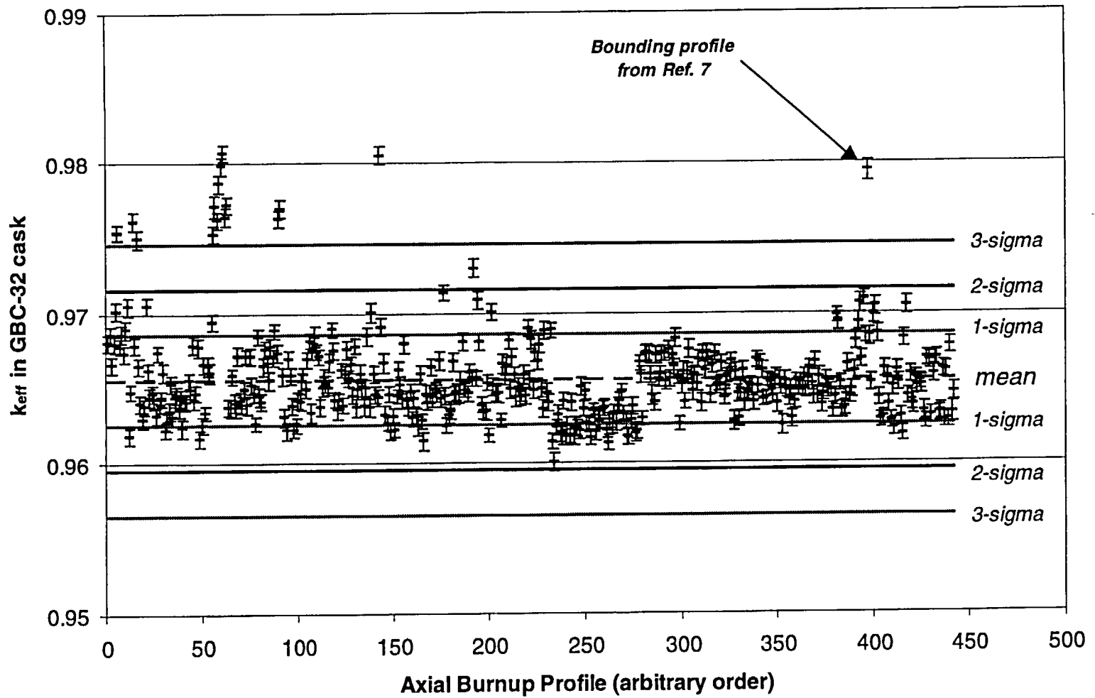
Figure B.8 Plot of k_{eff} values for axial burnup profiles in burnup group 8 ( 18 < \text{burnup} < 22 GWd/MTU). Total number of profiles in this burnup group is 442.
