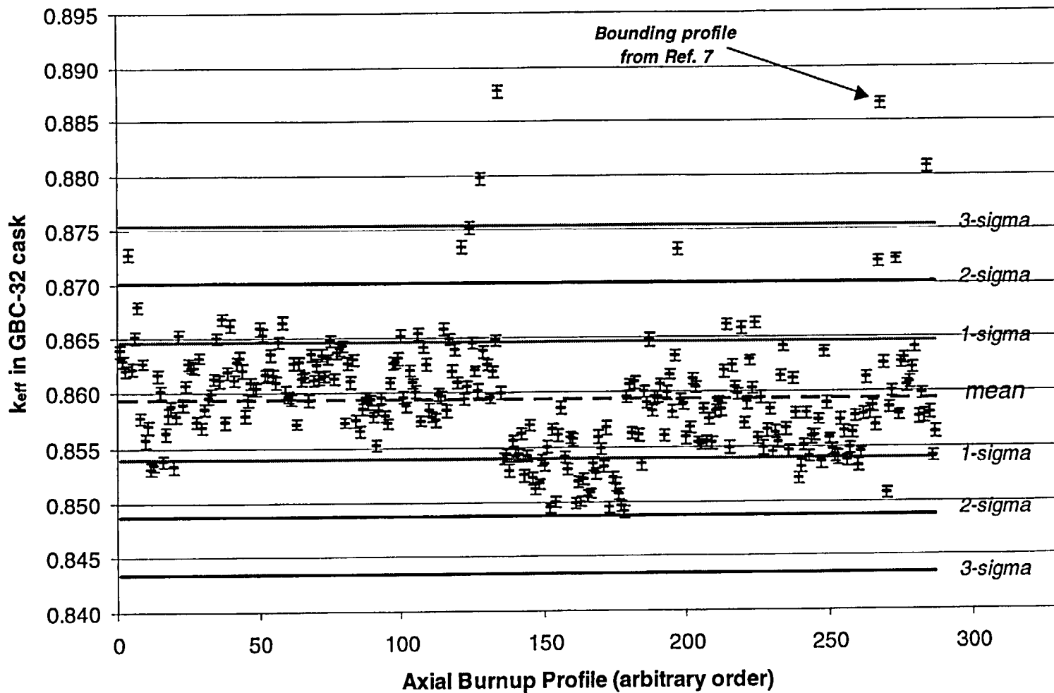
Figure B.4 Plot of k_{eff} values for axial burnup profiles in burnup group 4 ( 34 < \text{burnup} < 38 \text{ GWd/MTU} ). Total number of profiles in this burnup group is 287.
