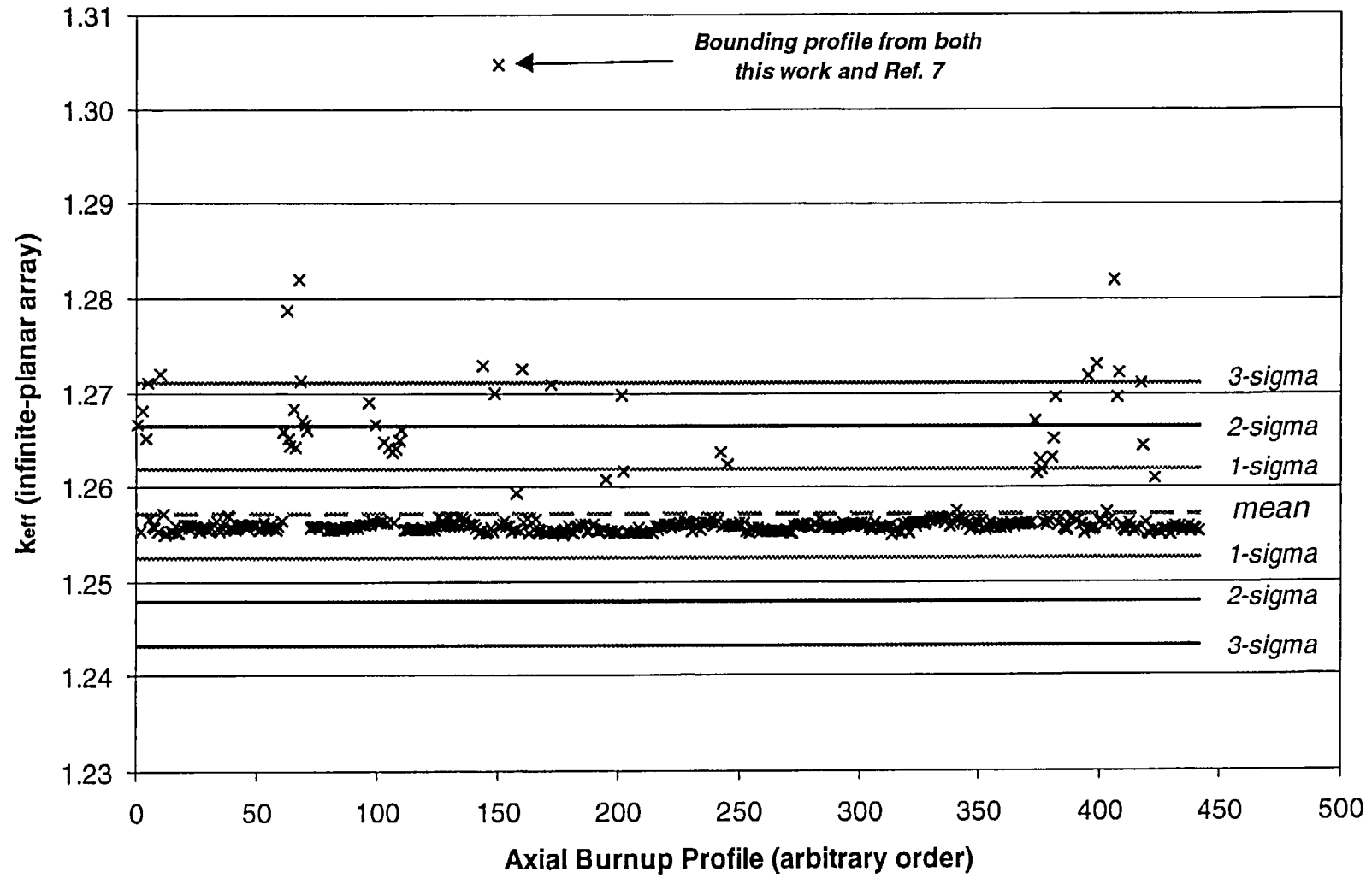
Figure 27 Plot of k_{eff} values for axial-burnup profiles in burnup group 9 ( 14 < \text{burnup} < 18 \text{ GWd/MTU} ). Total number of profiles in this burnup group is 441.
