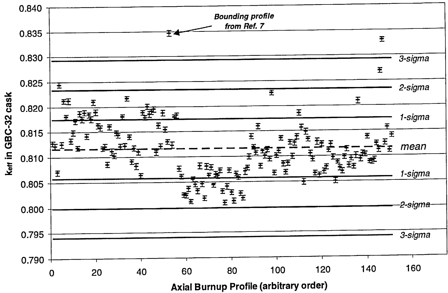
Figure B.2 Plot of k_{eff} values for axial burnup profiles in burnup group 2 ( 42 < \text{burnup} < 46 GWd/MTU). Total number of profiles in this burnup group is 151.
