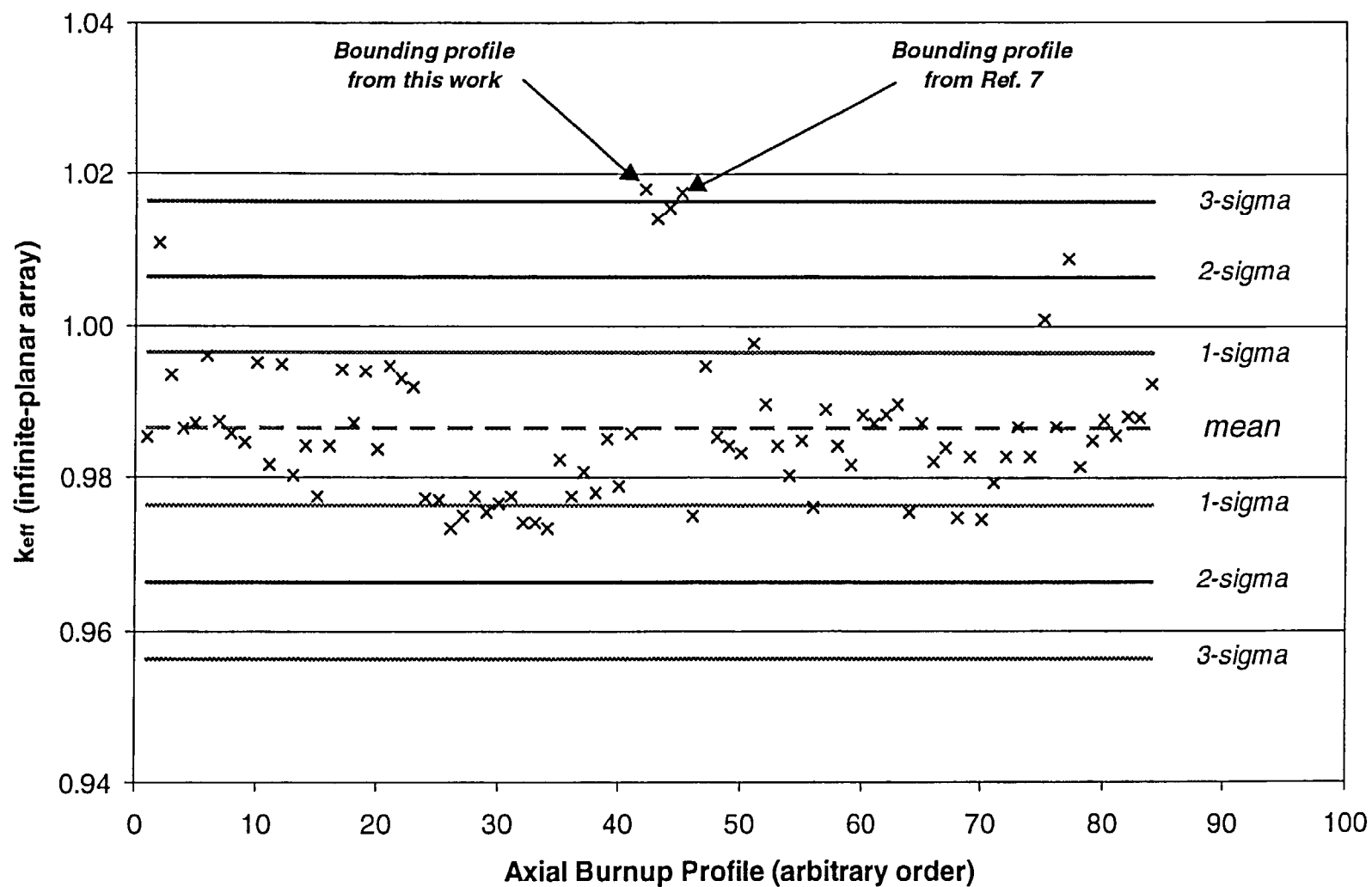
Figure 19 Plot of k_{eff} values for axial-burnup profiles in burnup group 1 (burnup > 46 GWd/MTU). Total number of profiles in this burnup group is 84.
