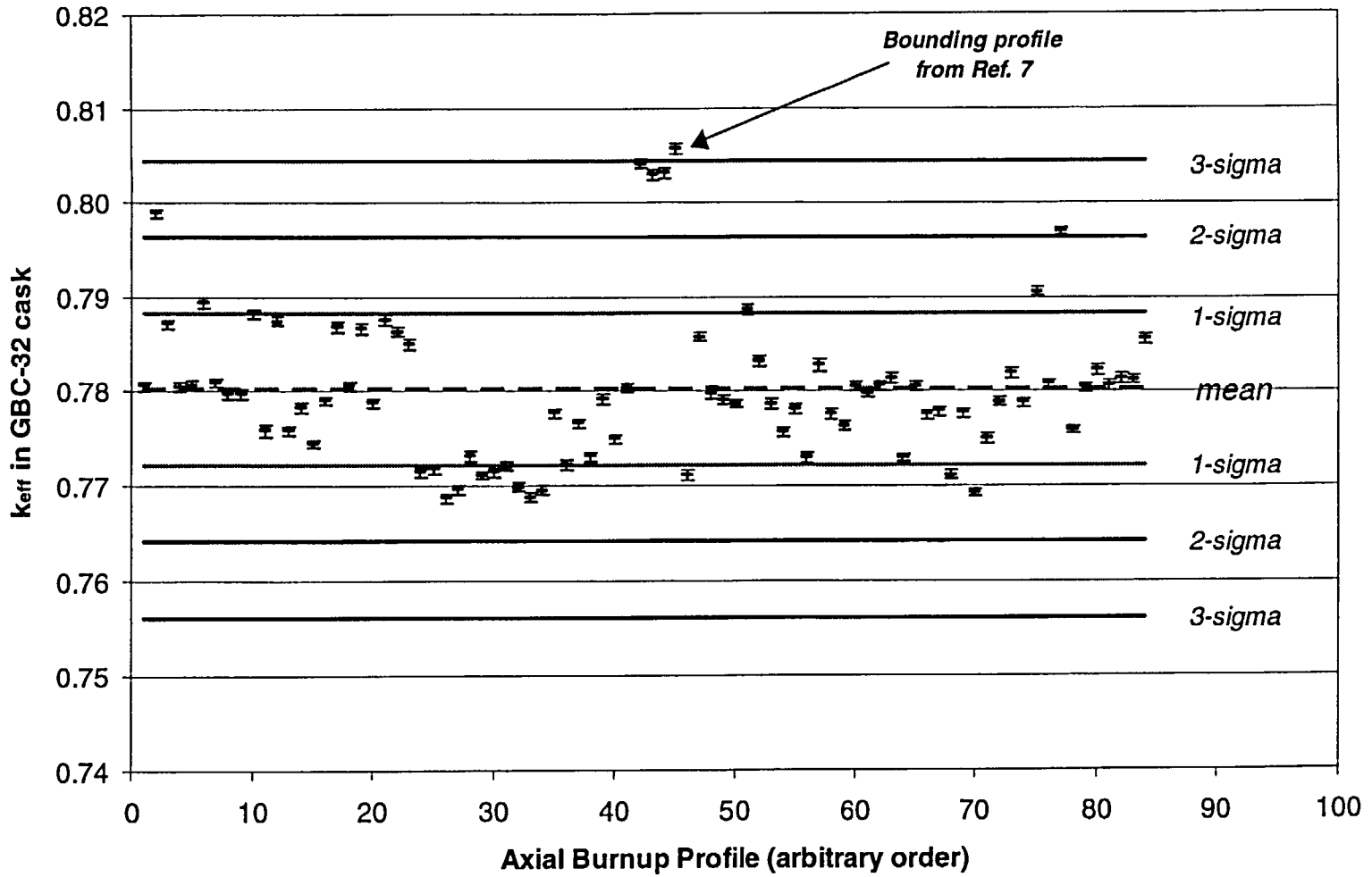
Figure B.1 Plot of k_{eff} values for axial burnup profiles in burnup group 1 (burnup > 46 GWd/MTU). Total number of profiles in this burnup group is 84.
