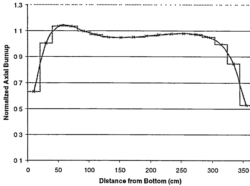
Figure 18 Bounding profile for burnup group 12 ( \text{burnup} < 6 \text{ GWd/MTU} )
