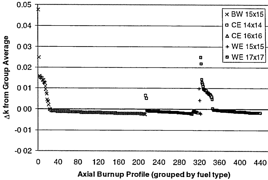
Figure 39 \Delta k values plotted in terms of fuel type for axial-burnup profiles in burnup group 9 ( 14 < \text{burnup} < 18 \text{ GWd/MTU} )
