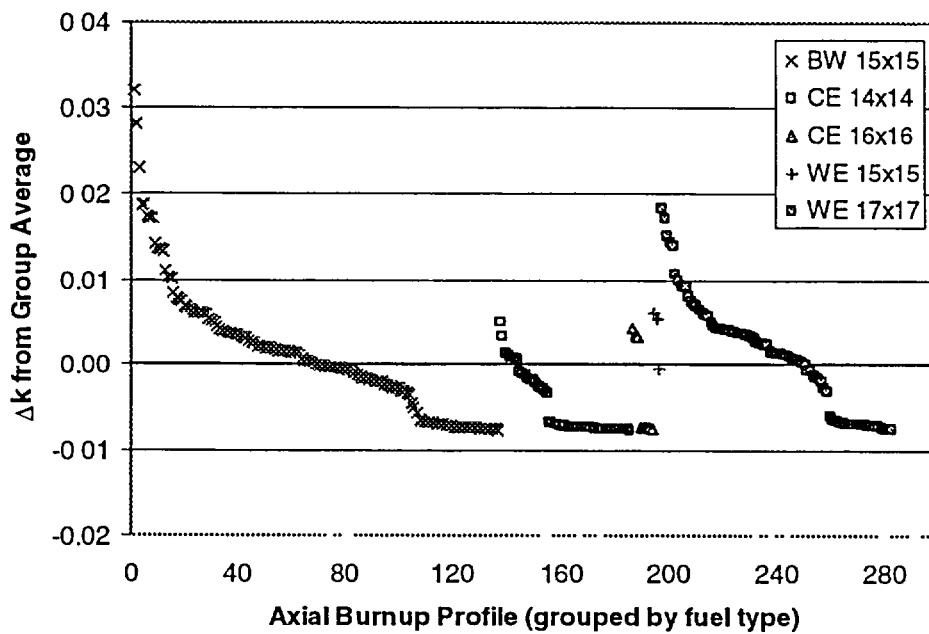
Figure 36 \Delta k values plotted in terms of fuel type for axial-burnup profiles in burnup group 6 ( 26 < \text{burnup} < 30 \text{ GWd/MTU} )
