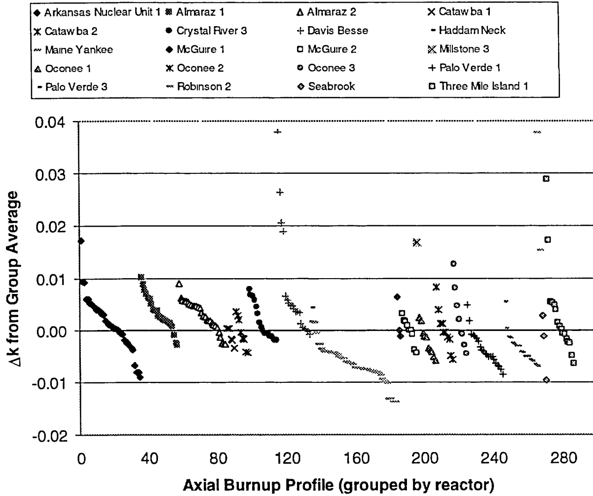
Figure 46 \Delta k values plotted in terms of reactor for axial-burnup profiles in burnup group 4 (34 < burnup < 38 GWd/MTU)
