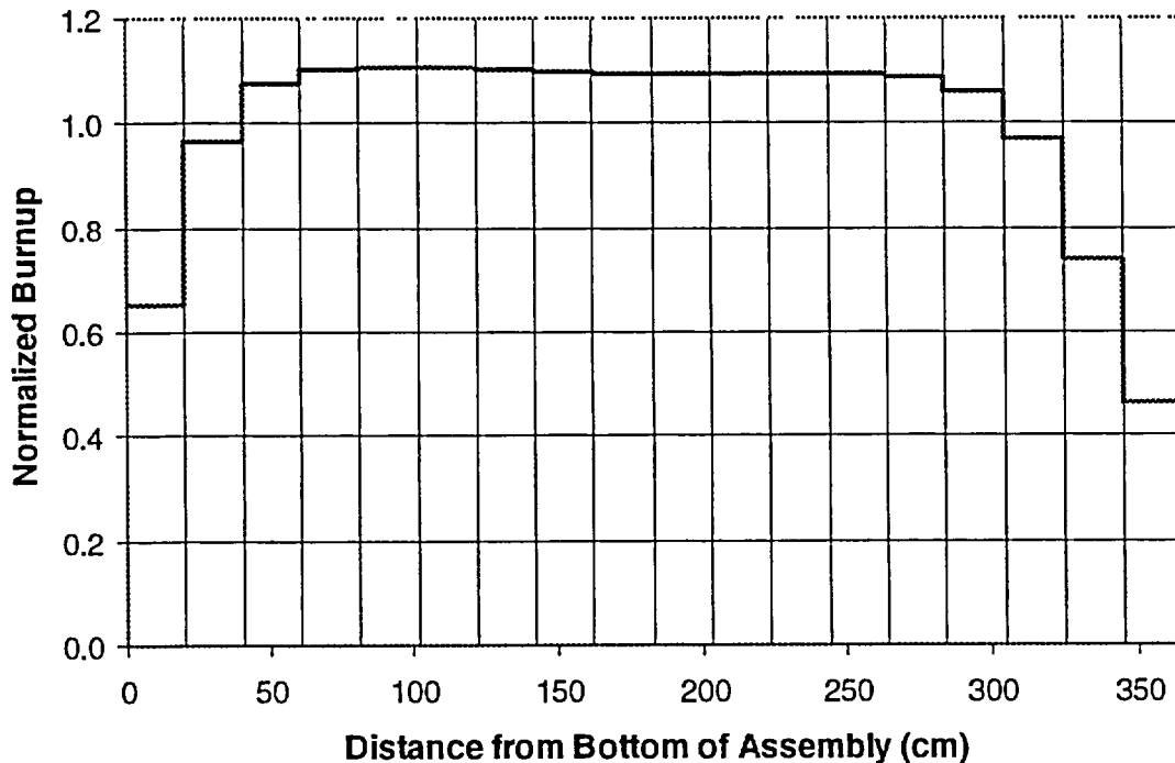
Figure 1 Representative normalized PWR axial-burnup distribution
