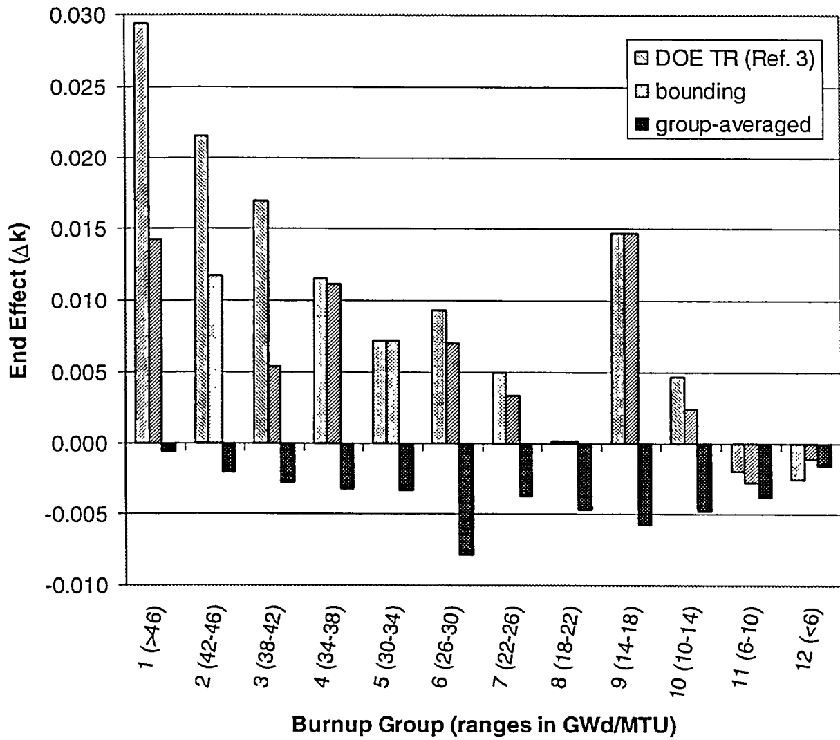
Figure 56 Comparison of end effect for actinide-only calculations in the GBC-32 cask (5-year cooling)
