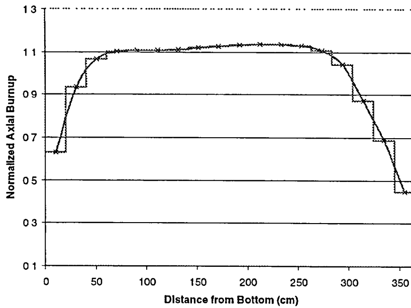
Figure 13 Bounding profile for burnup group 7 (22 < burnup < 26 GWd/MTU)
