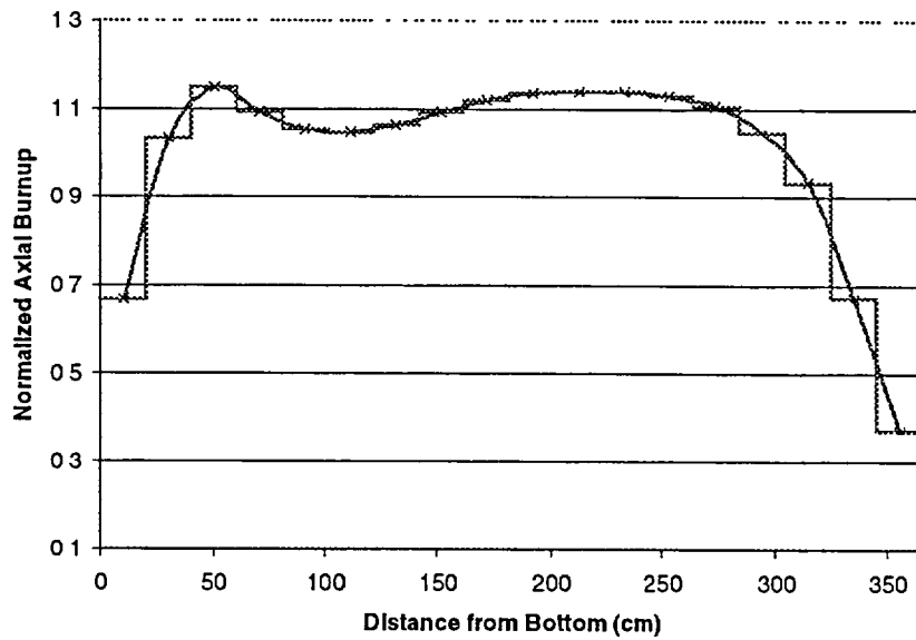
Figure 14 Bounding profile for burnup group 8 (18 < burnup < 22 GWd/MTU)
