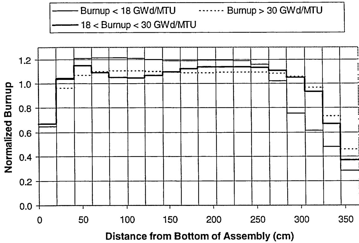
Figure 6 Proposed bounding axial profiles from Ref. 3
