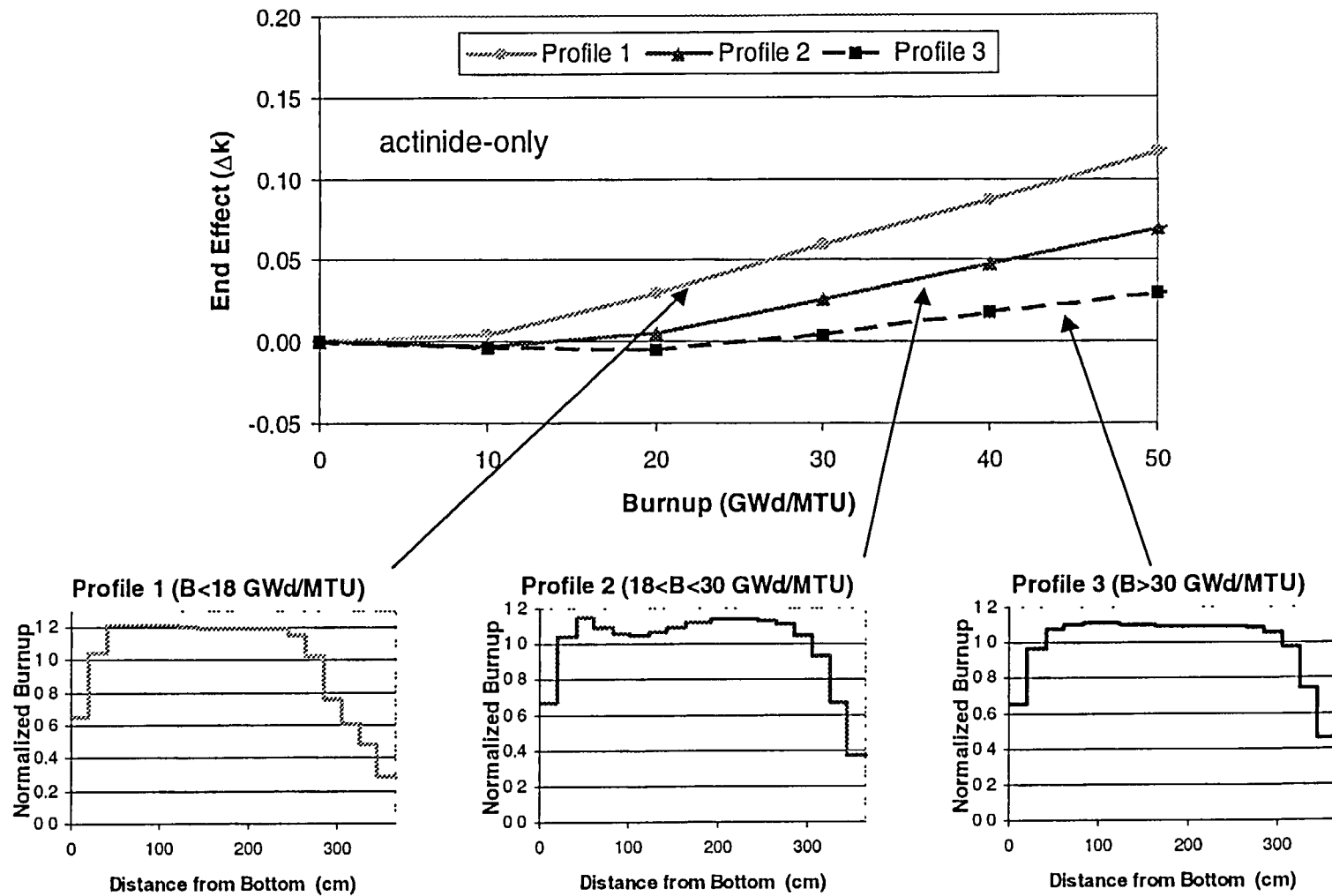
Figure 3 Examples of end effect as a function of burnup for three different axial-burnup profiles for fuel with 4.0 wt % ^{235}\text{U} enrichment and actinide-only nuclides. The profiles correspond to the suggested profiles from Ref. 3 for the specified burnup ranges.
