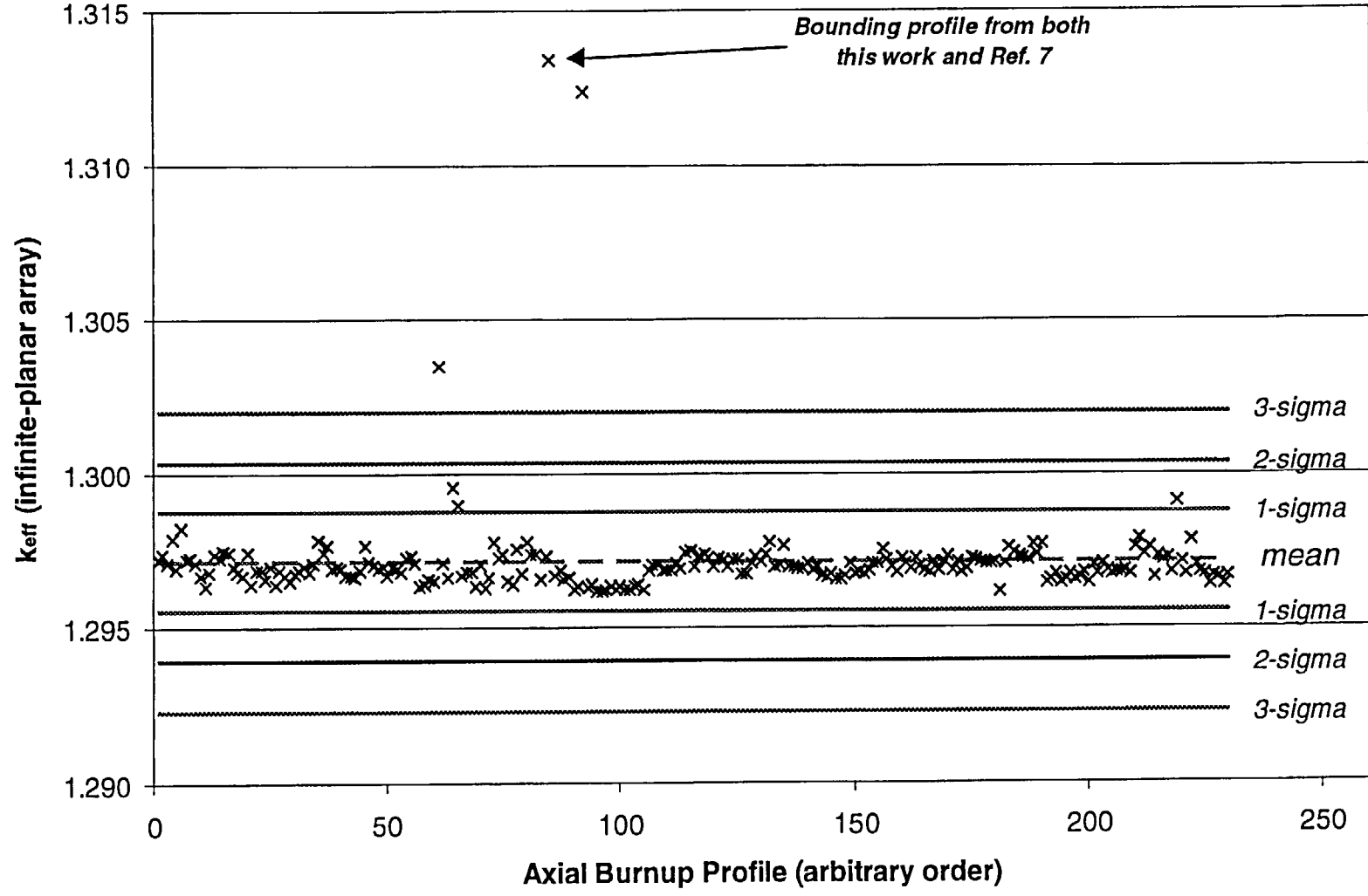
Figure 28 Plot of k_{eff} values for axial-burnup profiles in burnup group 10 ( 10 < \text{burnup} < 14 \text{ GWd/MTU} ). Total number of profiles in this burnup group is 230.
