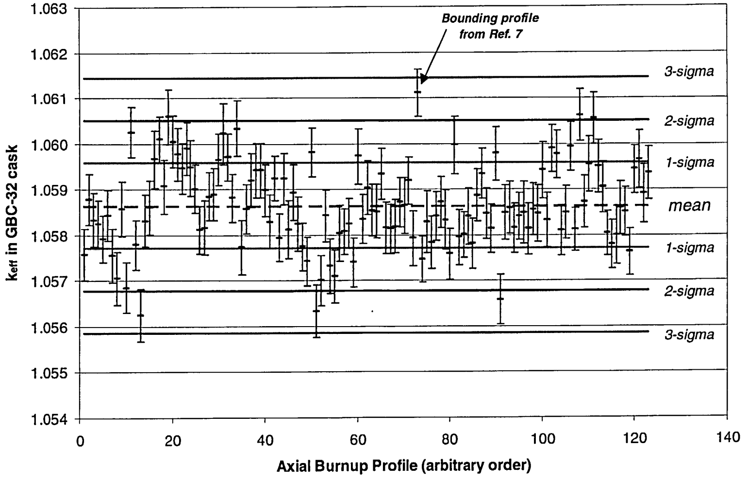
Figure B.11 Plot of k_{eff} values for axial burnup profiles in burnup group 11 ( 6 < \text{burnup} < 10 \text{ GWd/MTU} ). Total number of profiles in this burnup group is 123.
