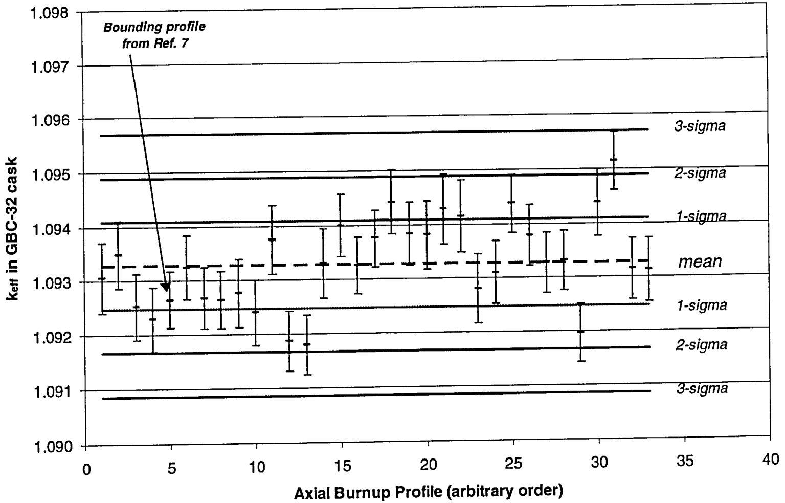
Figure B.12 Plot of k_{eff} values for axial burnup profiles in burnup group 12 (burnup < 6 GWd/MTU). Total number of profiles in this burnup group is 33.
