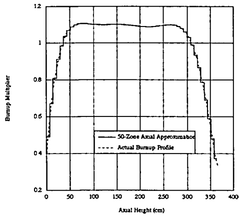
Figure A.4 50-Zone axial-burnup model
