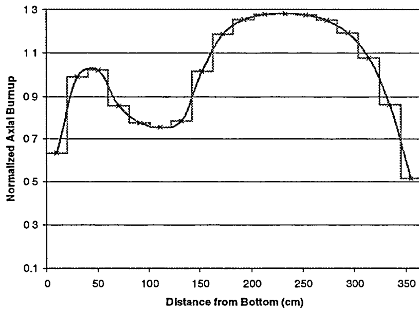
Figure 16 Bounding profile for burnup group 10 (10 < burnup < 14 GWd/MTU)
