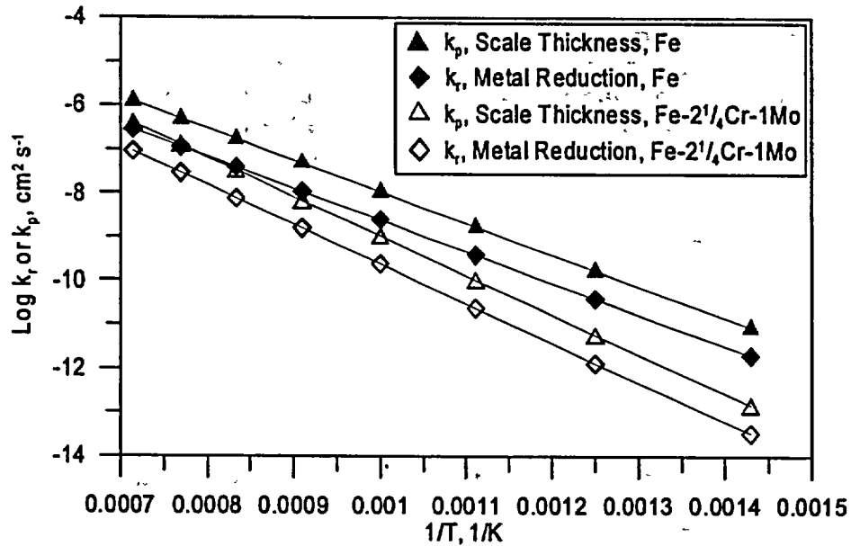
Figure 4-1. Oxidation Rate Constants for Fe-2 \frac{1}{4} Cr-1Mo Steel and Iron as a Function of Temperature Based on Results Reported by Simms and Little (1987) and Kubaschewski and Hopkins (1962)
