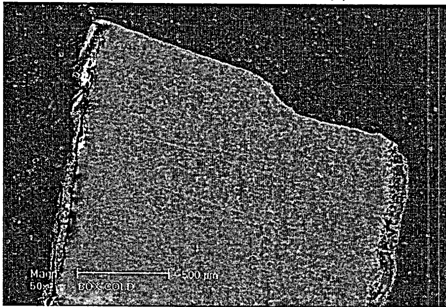
Figure 4-7. Cross Section of Car 50 Roof Approximately 40 cm [16 in] from the Edge Directly Exposed to the Fire. Thickness of the Metal Was Approximately 1,761 \mu\text{m} [0.069 in].
