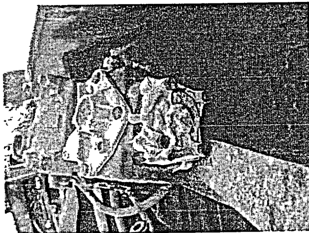
Figure 6-1. Air Brake Valve Found 20+ m [66+ ft] from Fuel Spill Site (Note Only Partial Melting at This Location)
