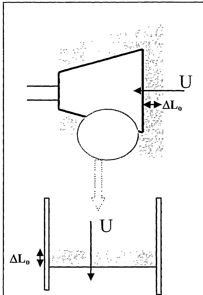
Figure 7-5 Equivalency Between a Truncated Cone Strainer Debris Accumulation and Flat-Plate Strainer Simulation
