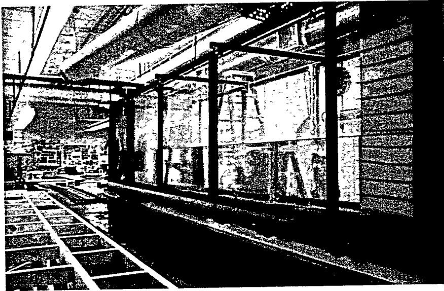
Figure 5-5 Photo of Large UNM Flume Test Apparatus
