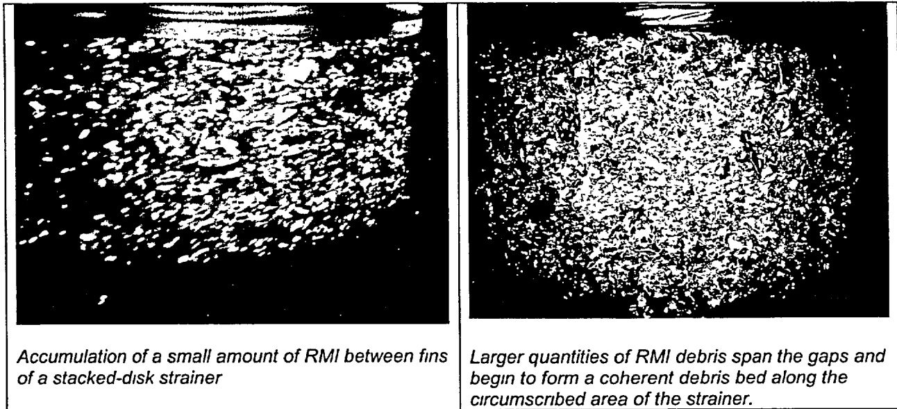
Figure 6-8 RMI Debris Accumulation on a Stacked-Disk Strainer 6-8
