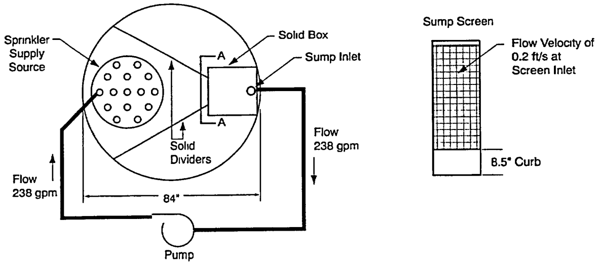
Figure 5-23 Configuration of Millstone-2 Debris-Transport Experiment
