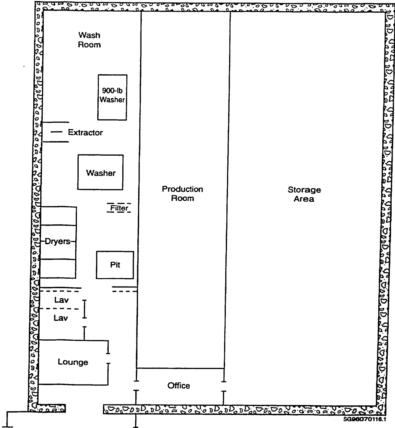
Figure 3.4 Layout of the radiological laundry facility
