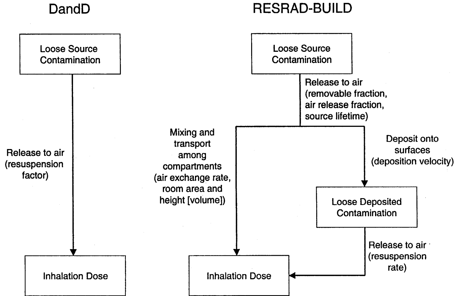
Figure 2.2 Inhalation Pathway in DandD and RESRAD-BUILD Codes
