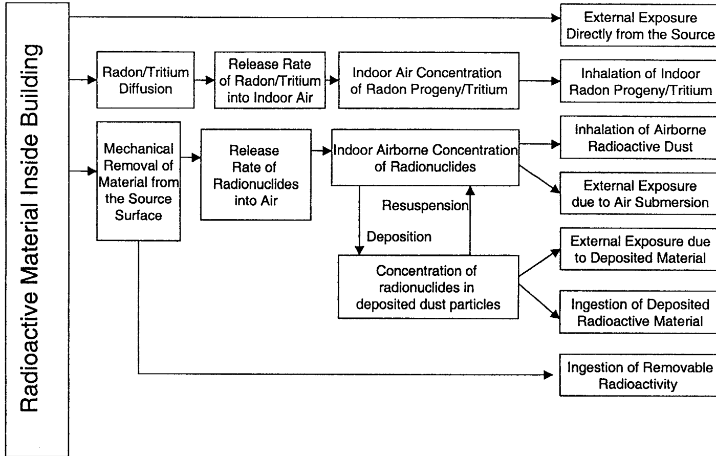
Figure 2.1 Exposure Pathways in the RESRAD-BUILD Code
