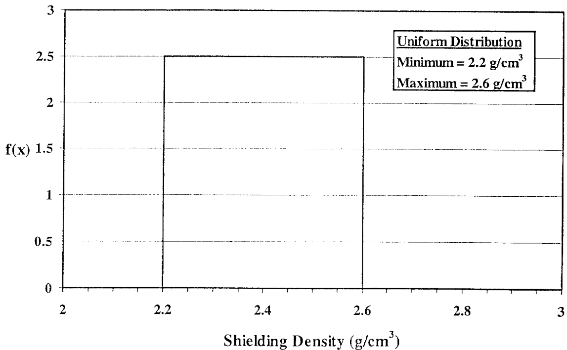
Figure A.1. Concrete Shielding Density Probability Density Function
