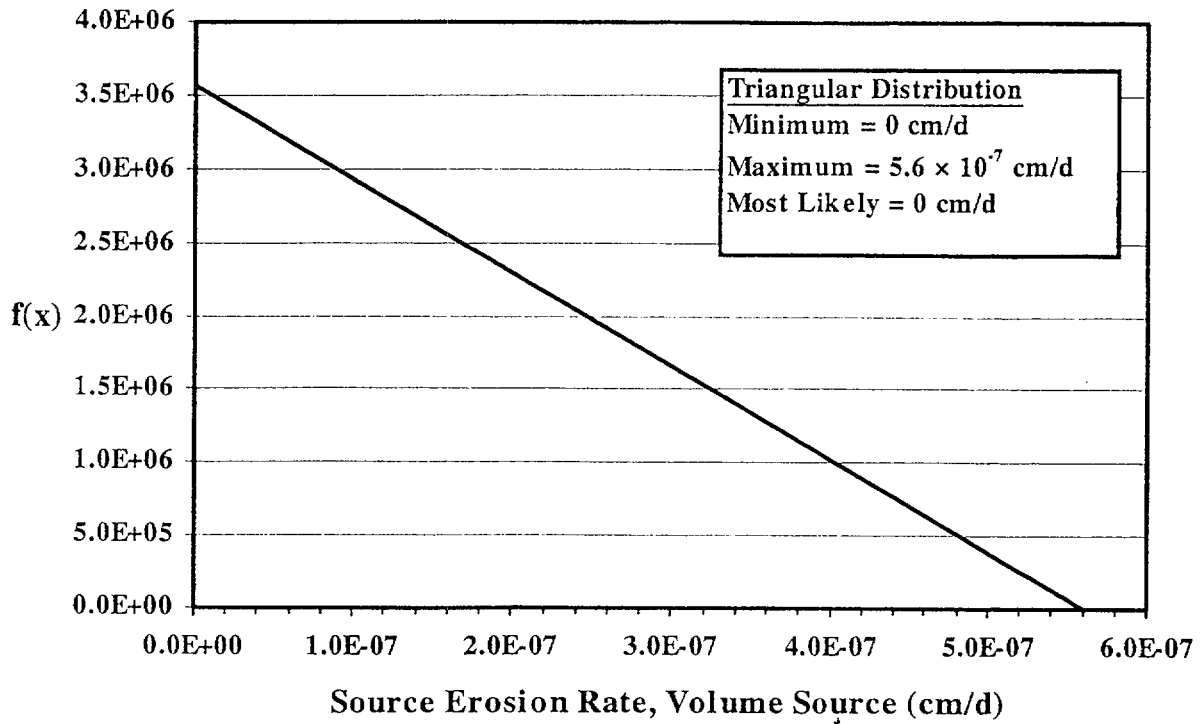
Figure 3.6 Source Erosion Rate Probability Density Function
