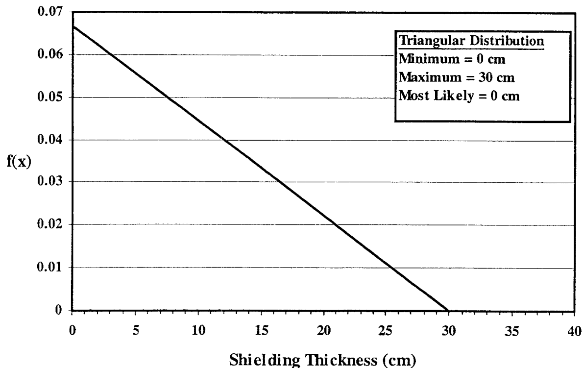
Figure A.5. Shielding Thickness Probability Density Function
