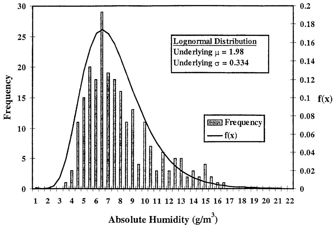
Figure A.7. Alternative Absolute Humidity Probability Density Function Based on Outdoor Humidity Levels
