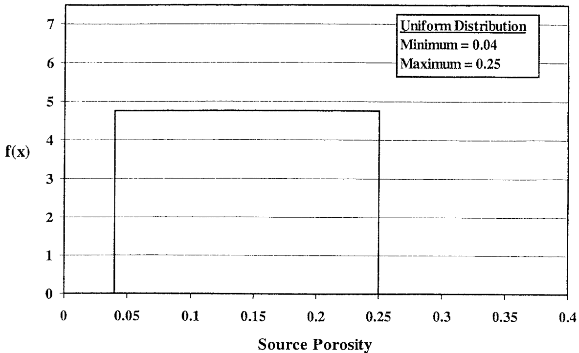
Figure A.9. Concrete Source Porosity Probability Density Function
