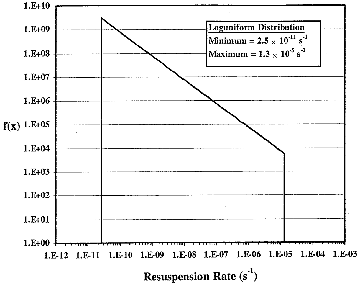
Figure 3.1. Indoor Resuspension Rate Probability Density Function
