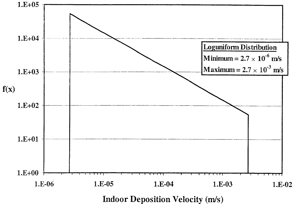
Figure 3.5 Indoor Deposition Velocity Probability Distribution
