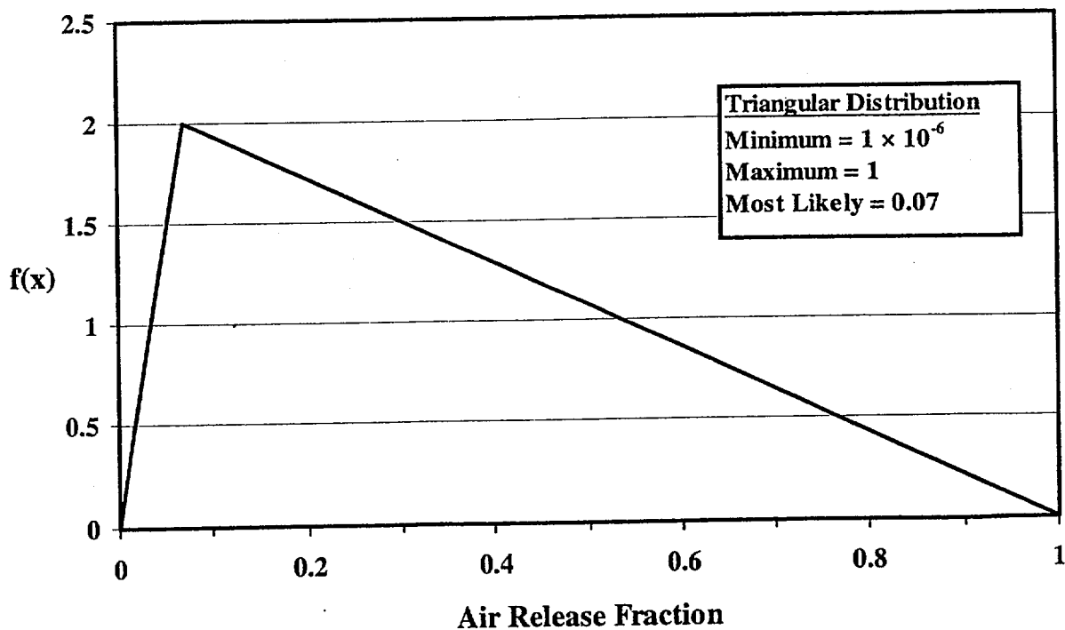
Figure A.10. Air Release Fraction Probability Density Function
