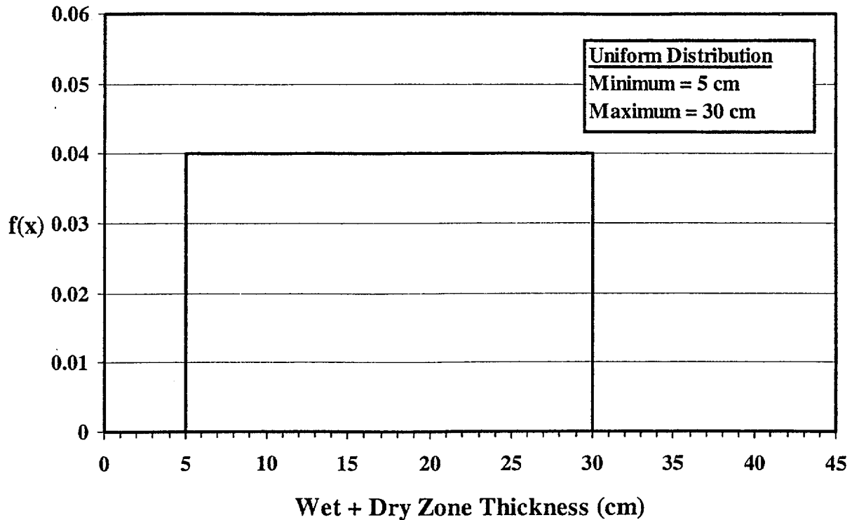
Figure A.11. Wet + Dry Zone Thickness Probability Density Function
