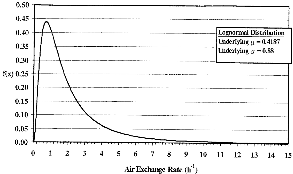
Figure 3.2. Building and Room Air Exchange Rate Probability Density Function
