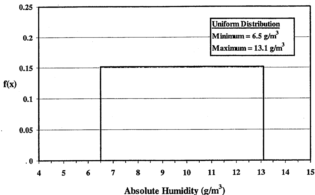
Figure A.6. Absolute Humidity Probability Density Function for RESRAD-BUILD
