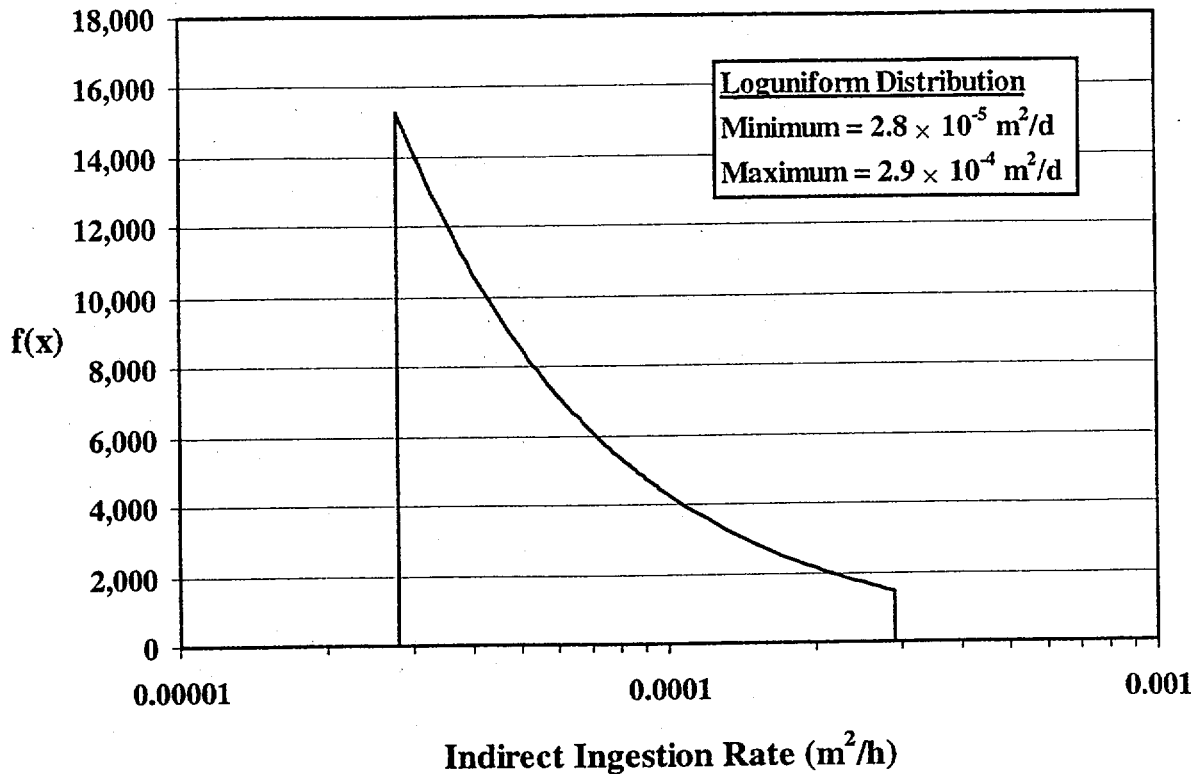
Figure A.14. Indirect Ingestion Rate Probability Density Function
