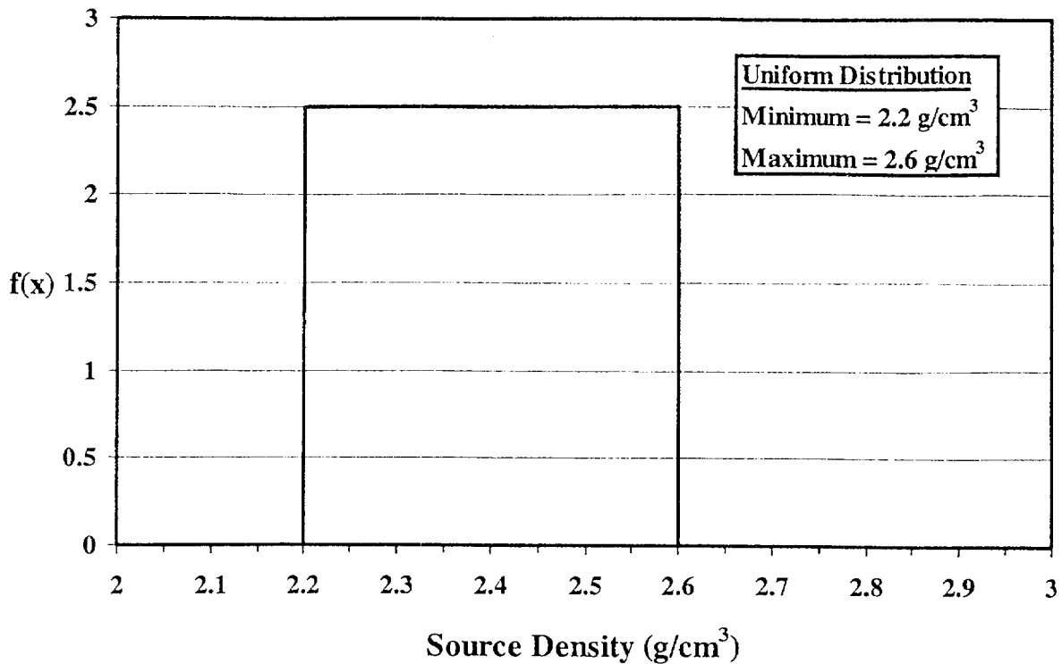
Figure A.8. Concrete Source Density Probability Distribution Function
