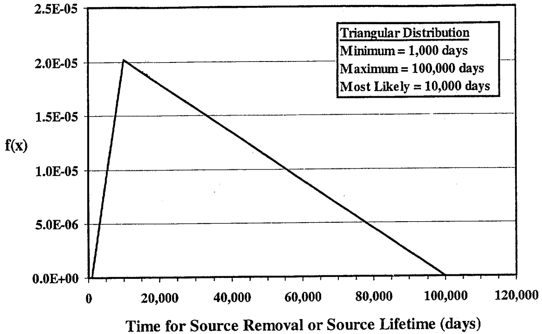
Figure 3.8. Time for Source Removal or Source Lifetime Probability Density Function
