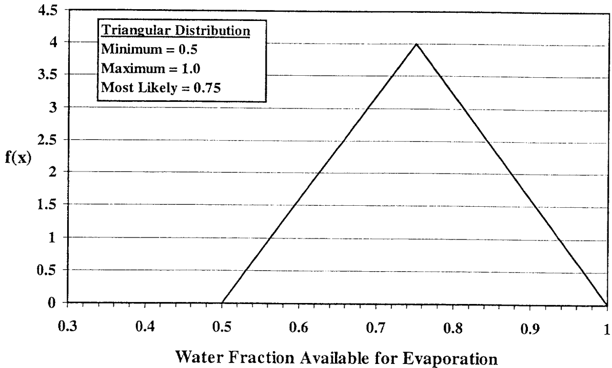
Figure A.13. Water Fraction Available for Evaporation
