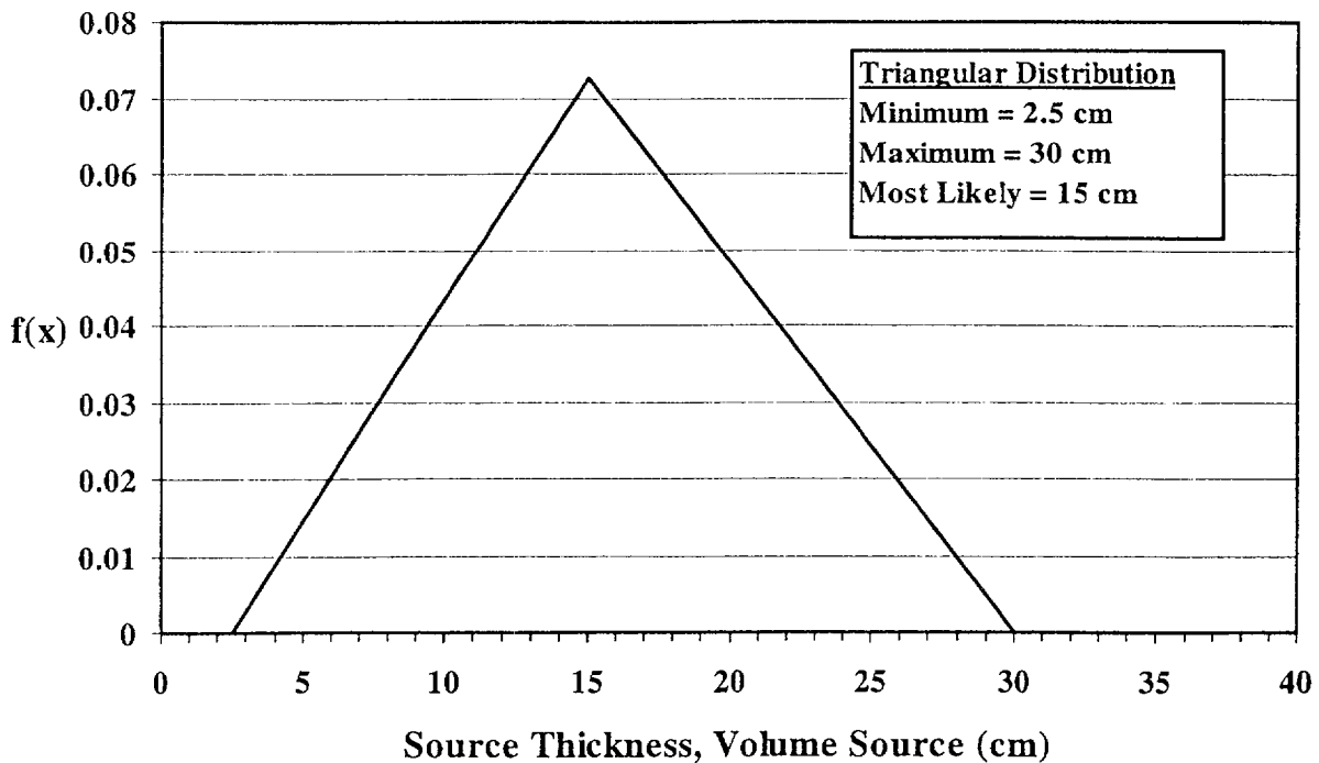
Figure A.12. Source Thickness Probability Density Function
