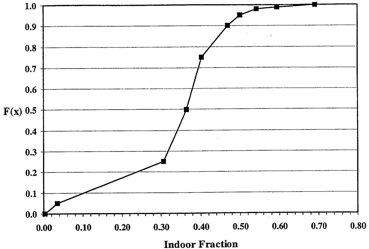
Figure A.2. Indoor Fraction Cumulative Distribution Function for RESRAD-BUILD
