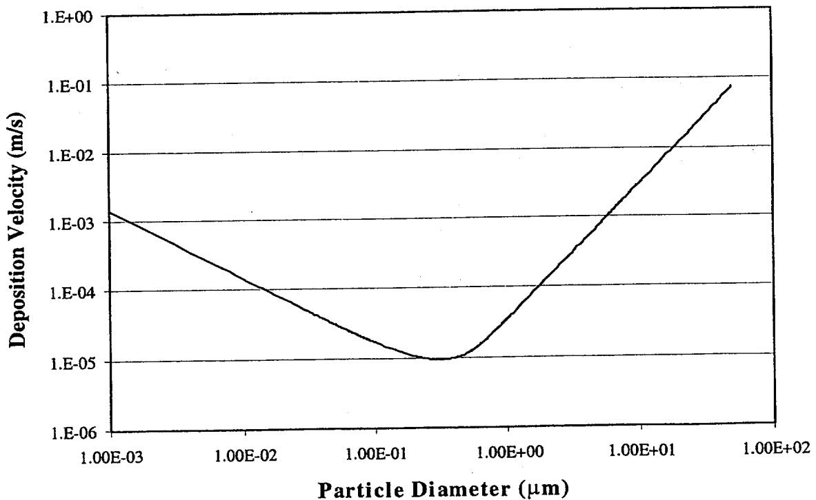
Figure 3.3. Idealized Representation of Indoor Particle Deposition Velocity
