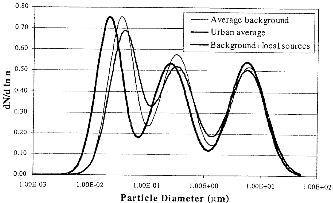
Figure 3.4 Trimodal Nature of Aerosol Particle Size Distribution
