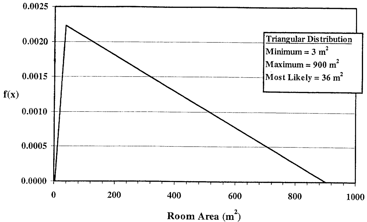
Figure A.3. Probability Density Function for Room Area
