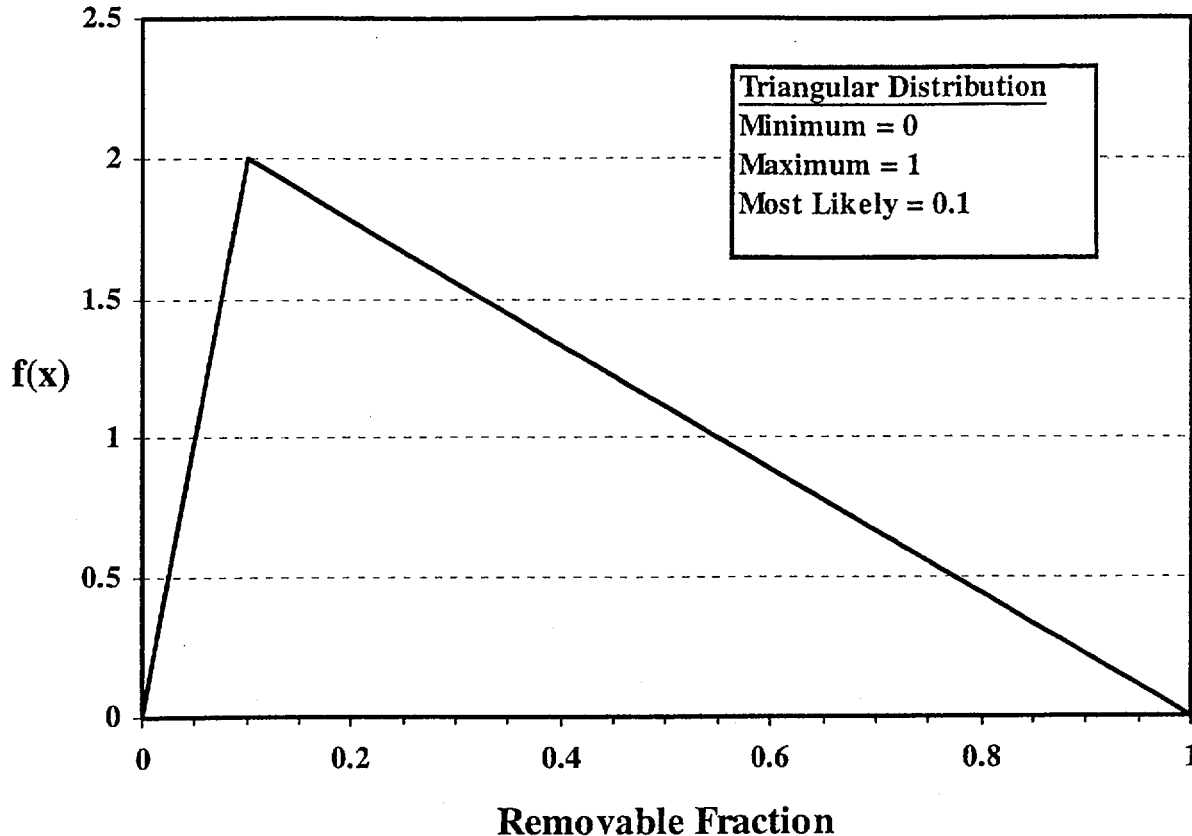
Figure 3.7 Removable Fraction Probability Distribution
