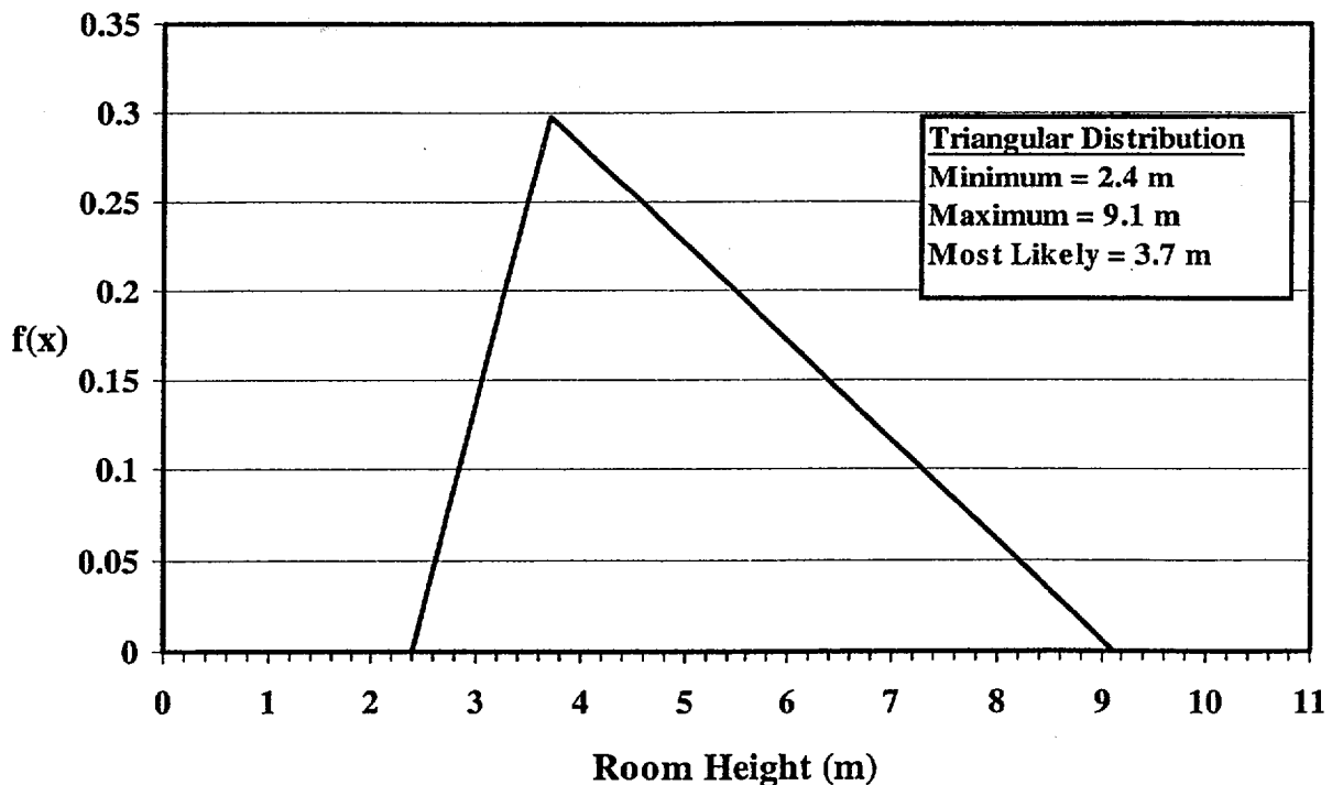
Figure A.4. Room Height Probability Density Function
