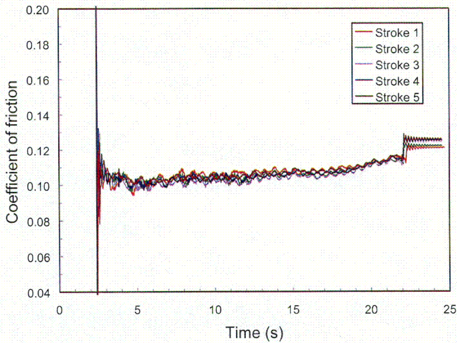
Figure 13. The five cold baseline tests for stem 2 with SRI show no variation in stem coefficient of friction.
