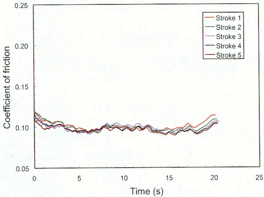
Figure 6. The five cold load tests for stem 2 with EP1 show little variation in the stem coefficient of friction.
