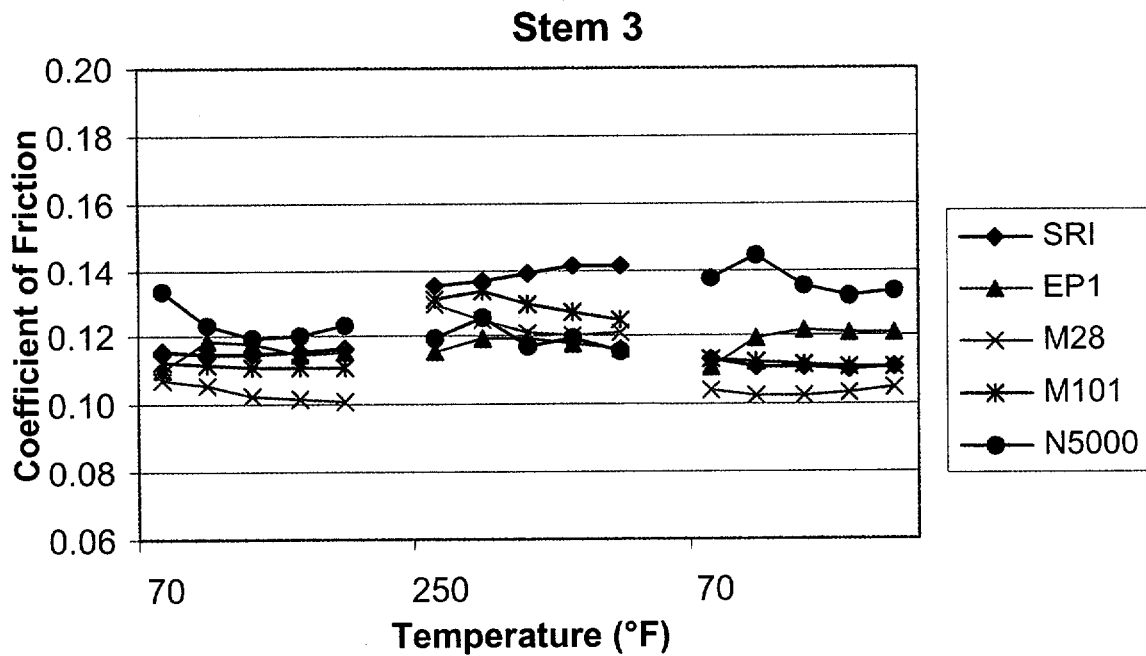
Figure 36. Stem nut coefficient of friction for each stroke of the single step tests with Stem 3.
