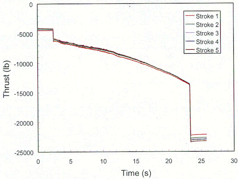
Figure 5. The five cold load tests for stem 2 with EP1 show no variation in the stem thrust between strokes.
