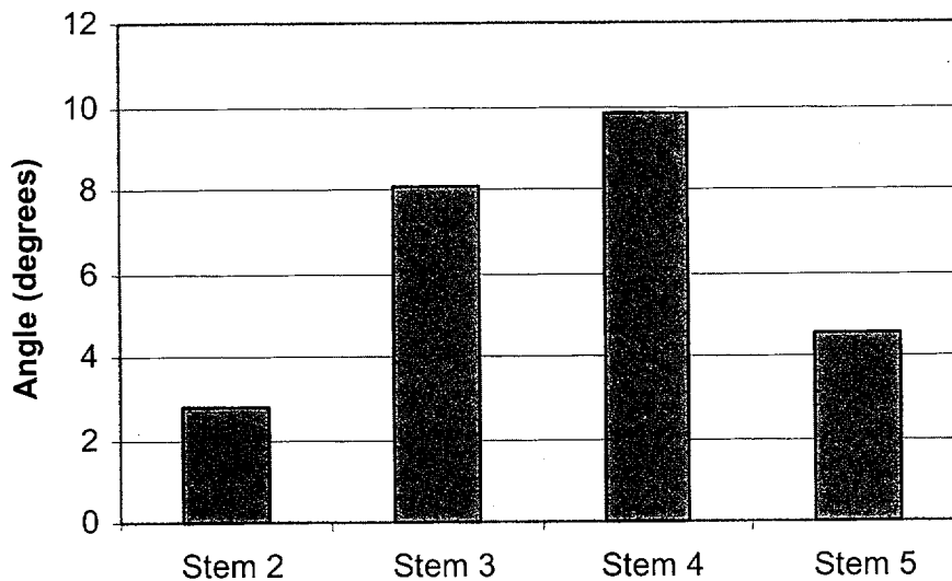
Figure 33. Stem thread angle for each stem tested at elevated temperature.
