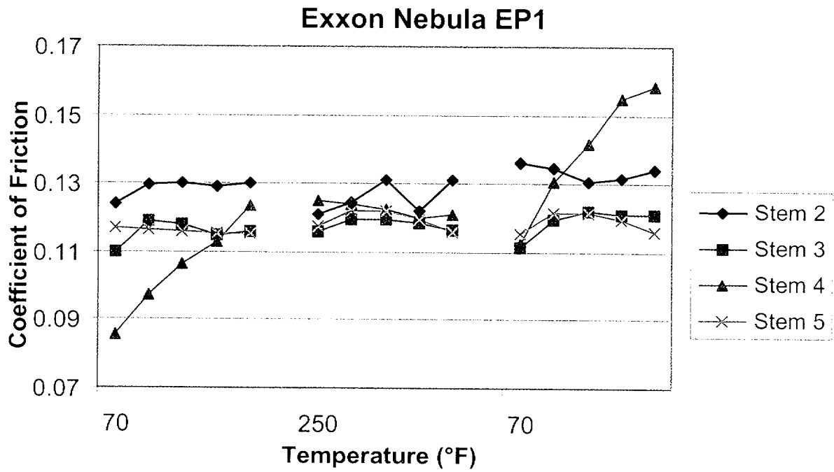
Figure 20. Stem nut coefficient of friction for each stroke of the single step tests with EP1.
