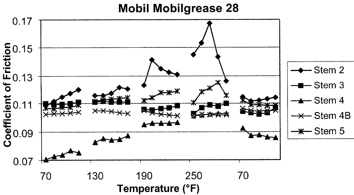
Figure 25. Stem nut coefficient of friction for each stroke of the multiple step tests with Mobil 28.
