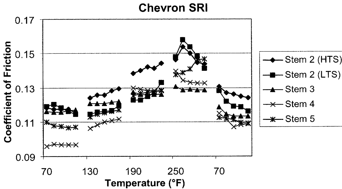
Figure 23. Stem nut coefficient of friction for each stroke of the multiple step tests with SRI.
