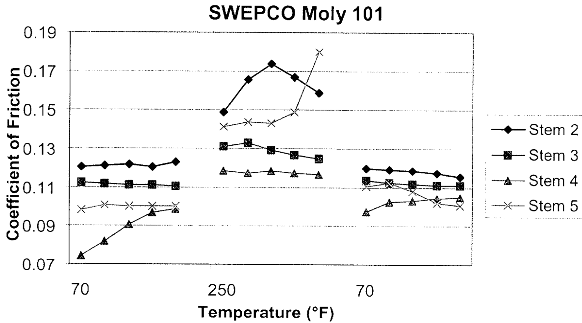
Figure 26. Stem nut coefficient of friction for each stroke of the single step tests with Moly 101.
