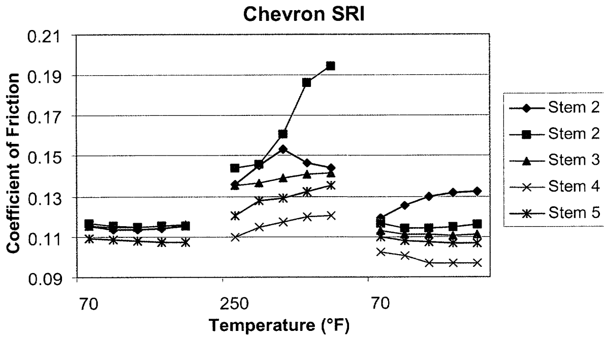
Figure 22. Stem nut coefficient of friction for each stroke of the single step tests with SRI.
