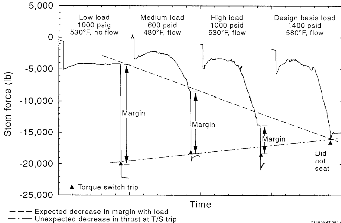
Figure 2. During actual MOV testing, the rate-of-loading changes with stem load.
