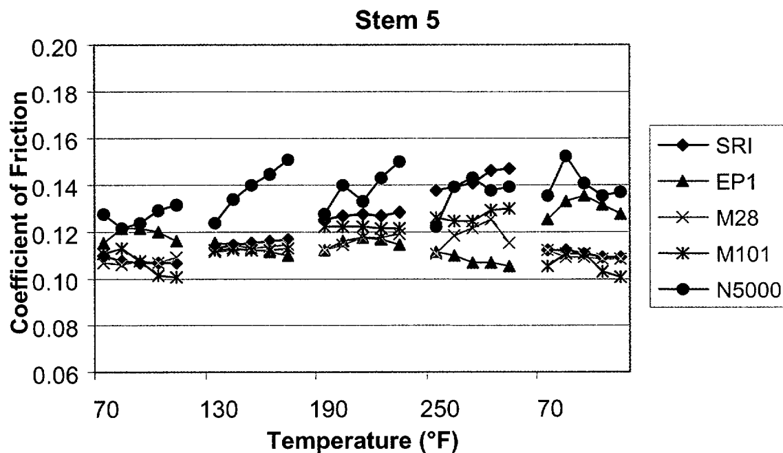
Figure 41. Stem nut coefficient of friction for each stroke of the multiple step tests with Stem 5.
