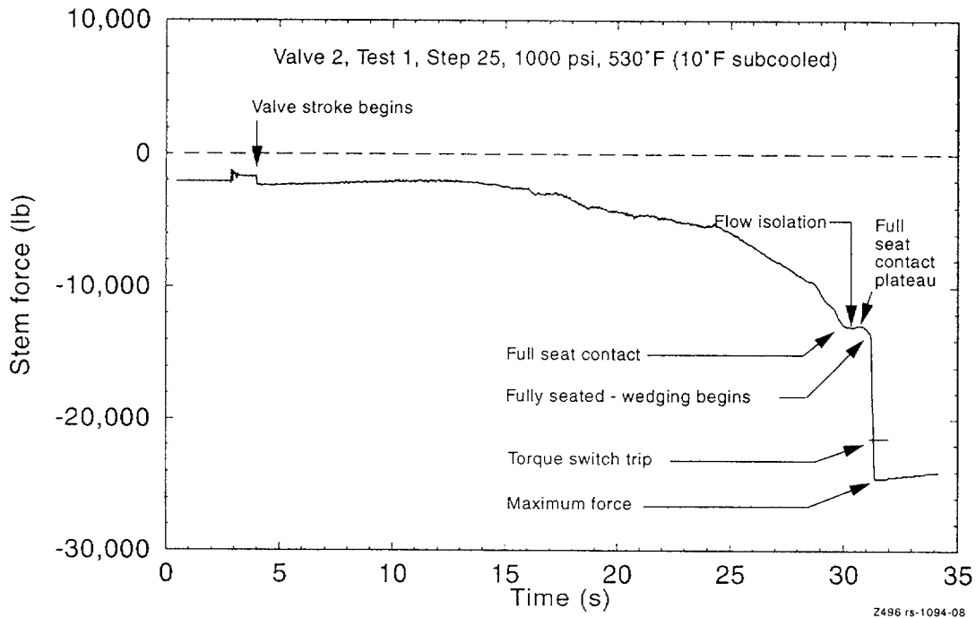
Figure 32. Data trace from a high flow closure test of a flexible-wedge gate valve.
