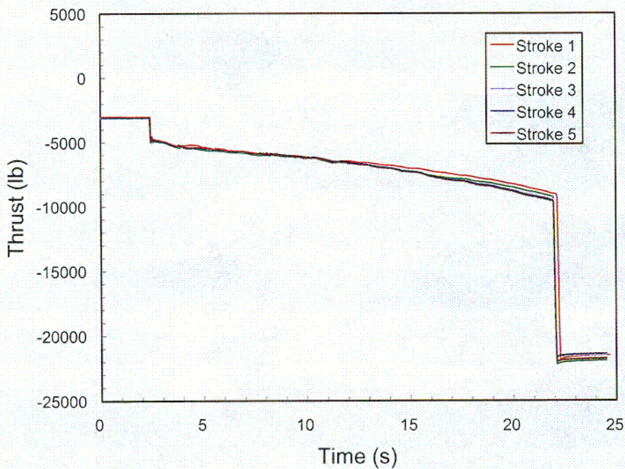
Figure 11. The five cold baseline tests for stem 2 with SRI show no variation in stem thrust between strokes.
