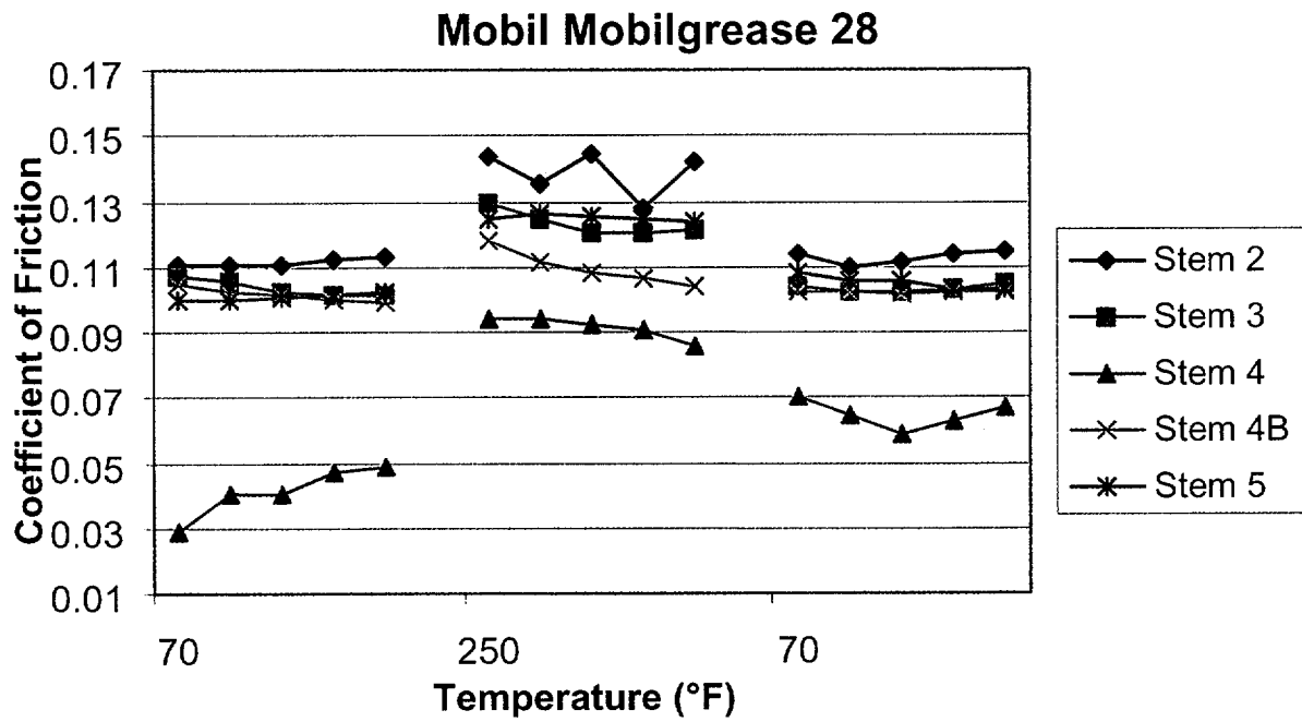
Figure 24. Stem nut coefficient of friction for each stroke of the single step tests with Mobil 28.
