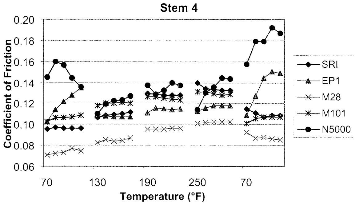
Figure 39. Stem nut coefficient of friction for each stroke of the multiple step tests with Stem 4.
