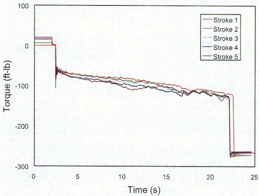
Figure 15. The five hot baseline tests for stem 2 with SRI show an increase in stem torque with each stroke.
