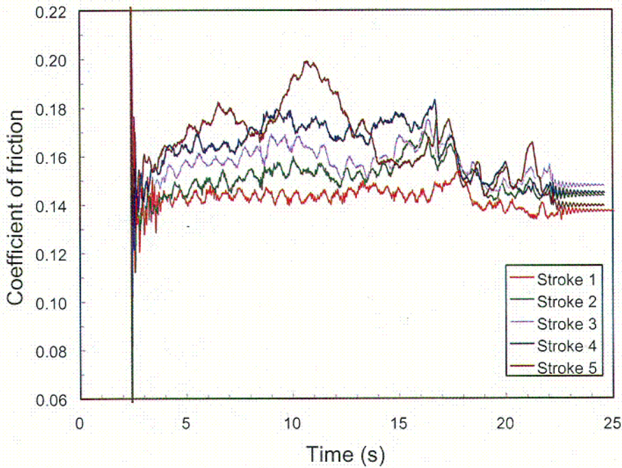
Figure 16. The five hot baseline tests for stem 2 with SRI show significant increase in stem friction.
