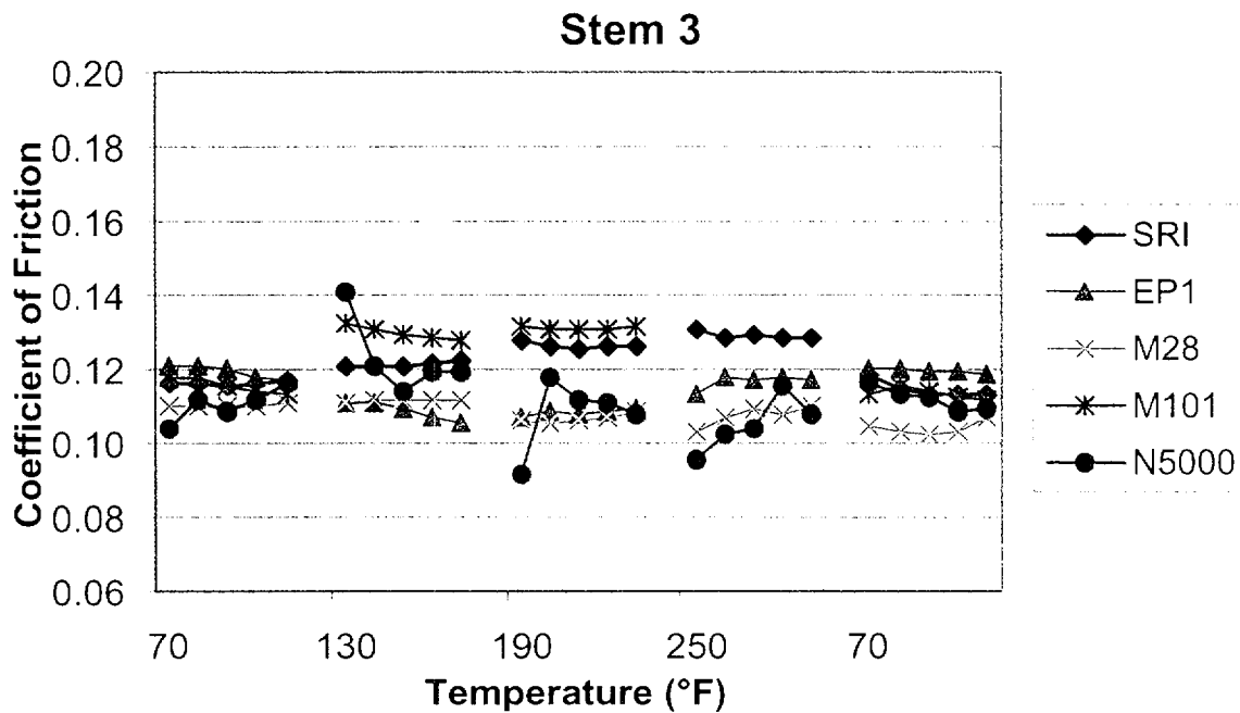
Figure 37. Stem nut coefficient of friction for each stroke of the multiple step tests with Stem 3.
