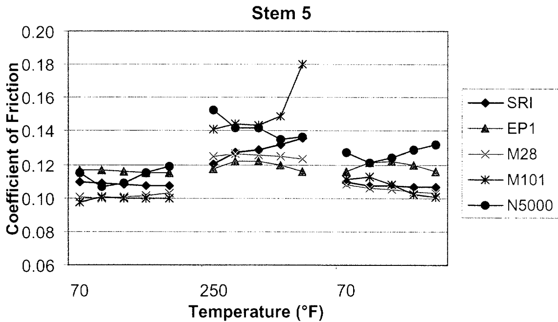
Figure 40. Stem nut coefficient of friction for each stroke of the single step tests with Stem 5.
