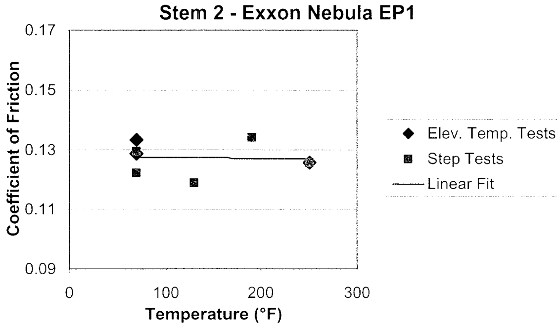
Figure 30. Typical flat or decreasing change in stem nut friction at elevated temperature.
