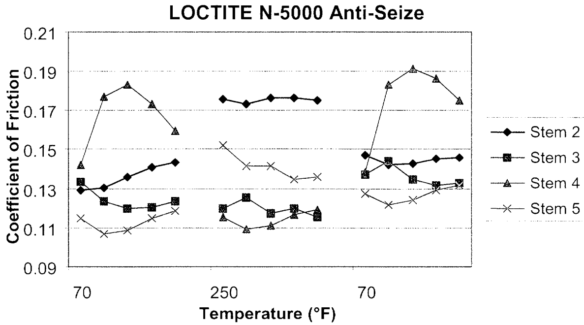
Figure 28. Stem nut coefficient of friction for each stroke of the single step tests with N-5000.
