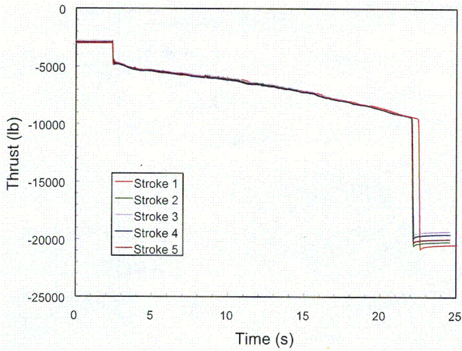
Figure 14. The five hot baseline tests for stem 2 with SRI show no variation in stem thrust between strokes.
