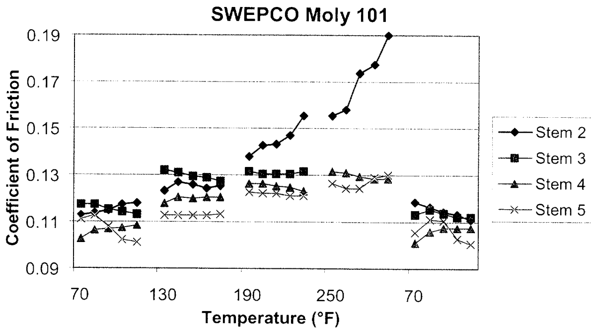
Figure 27. Stem nut coefficient of friction for each stroke of the multiple step tests with Moly 101.
