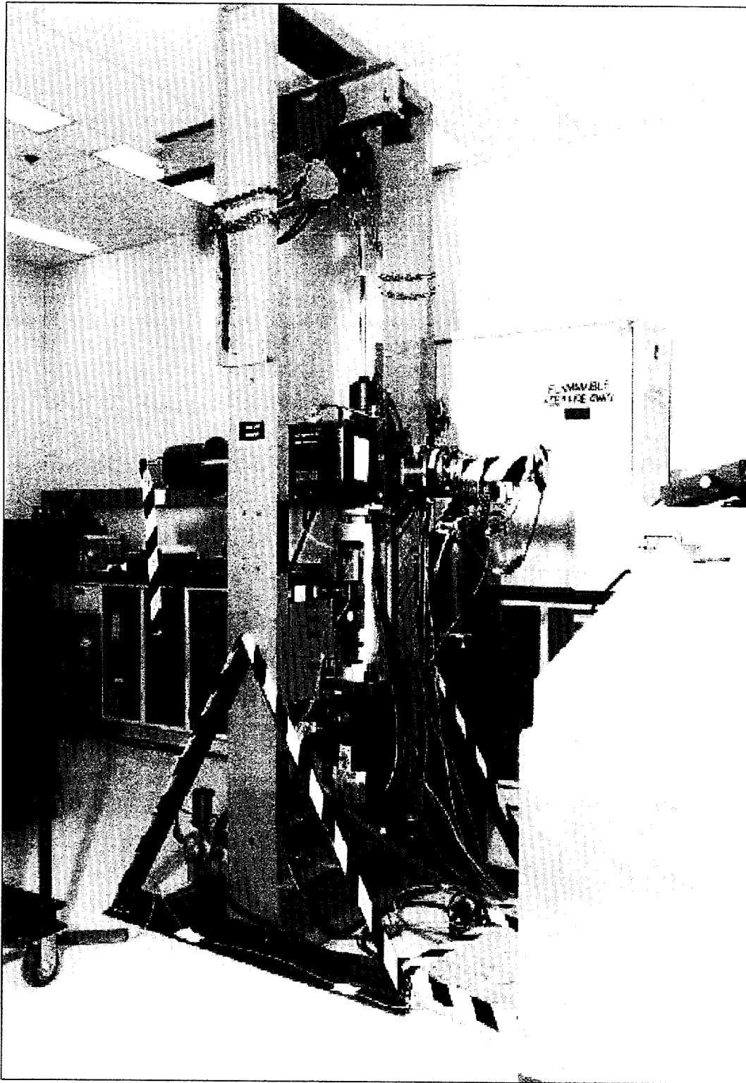
Figure 3. INEEL motor operated valve load simulator (MOVLS).
