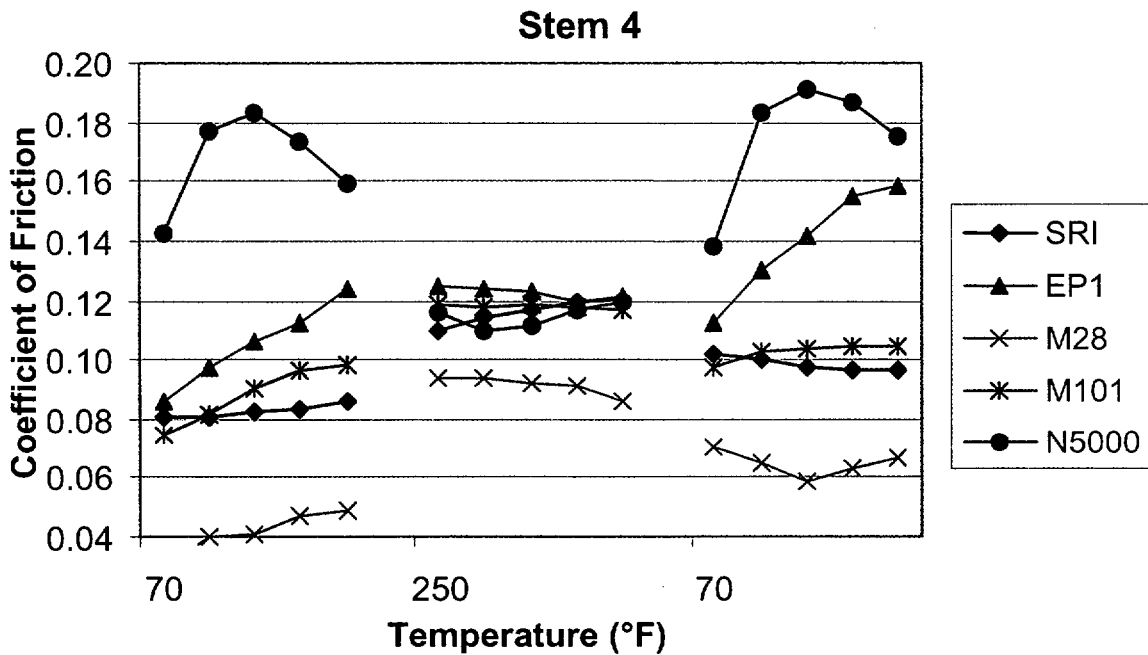
Figure 38. Stem nut coefficient of friction for each stroke of the single step tests with Stem 4.
