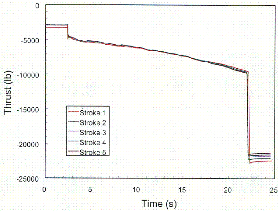
Figure 17. The five final cold tests for stem 2 with SRI show little variation in stem thrust between strokes.
