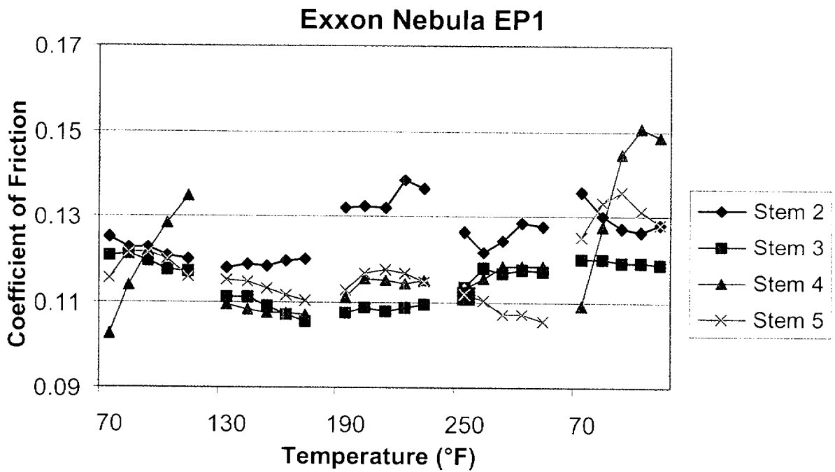
Figure 21. Stem nut coefficient of friction for each stroke of the multiple step tests with EP1.
