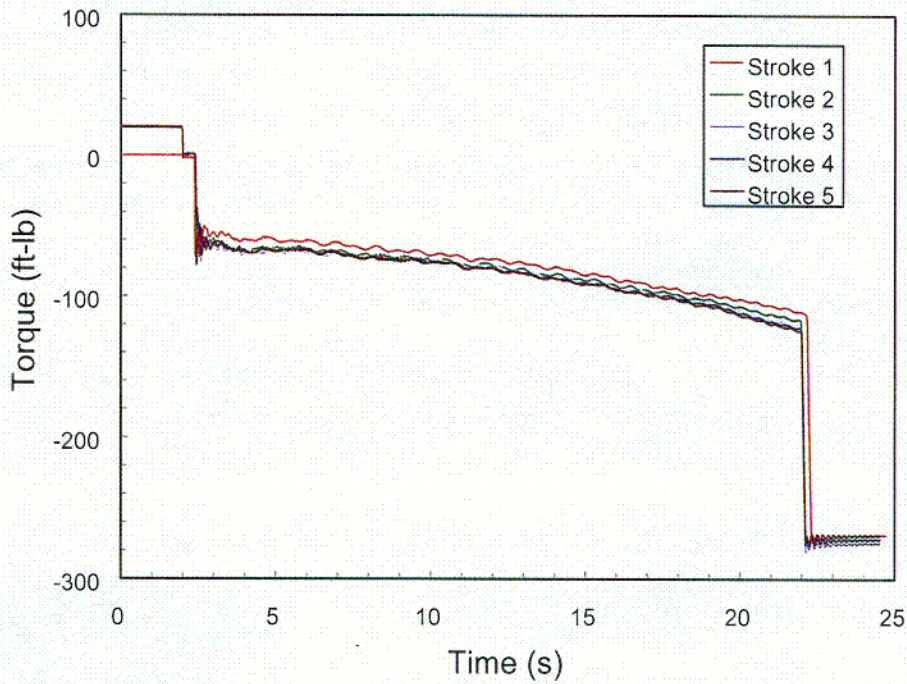
Figure 18. The five final cold tests for stem 2 with SRI show a small variation in stem torque between strokes.
