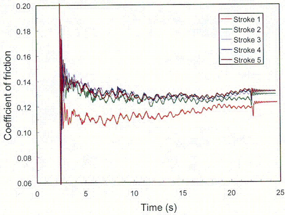
Figure 19. The five cold tests for stem 2 with SRI show a significant variation in stem friction after the first stroke.
