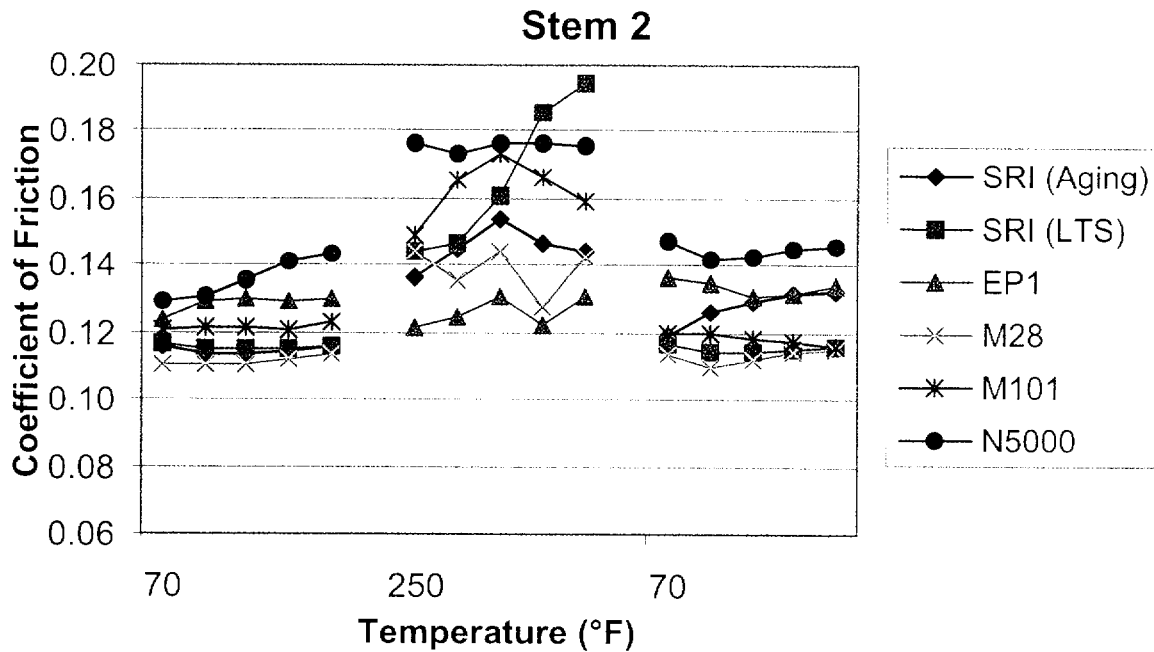
Figure 34. Stem nut coefficient of friction for each stroke of the single step tests with Stem 2.
