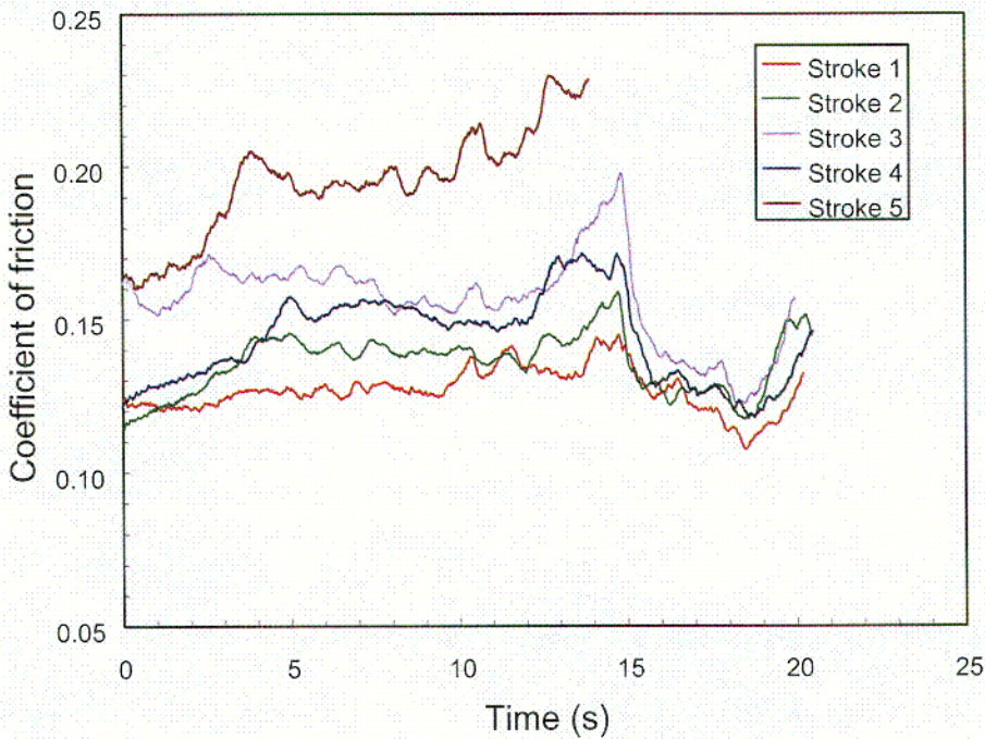
Figure 8. The five hot load tests for stem 2 with EP1 show significant variation in the stem coefficient of friction.
