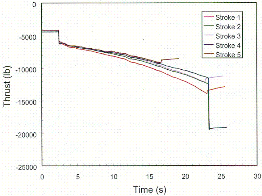
Figure 7. The five hot load tests for stem 2 with EP1 required changes to the MOVLS settings to produce full closure.
