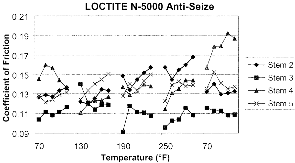
Figure 29. Stem nut coefficient of friction for each stroke of the multiple step tests with N-5000.
