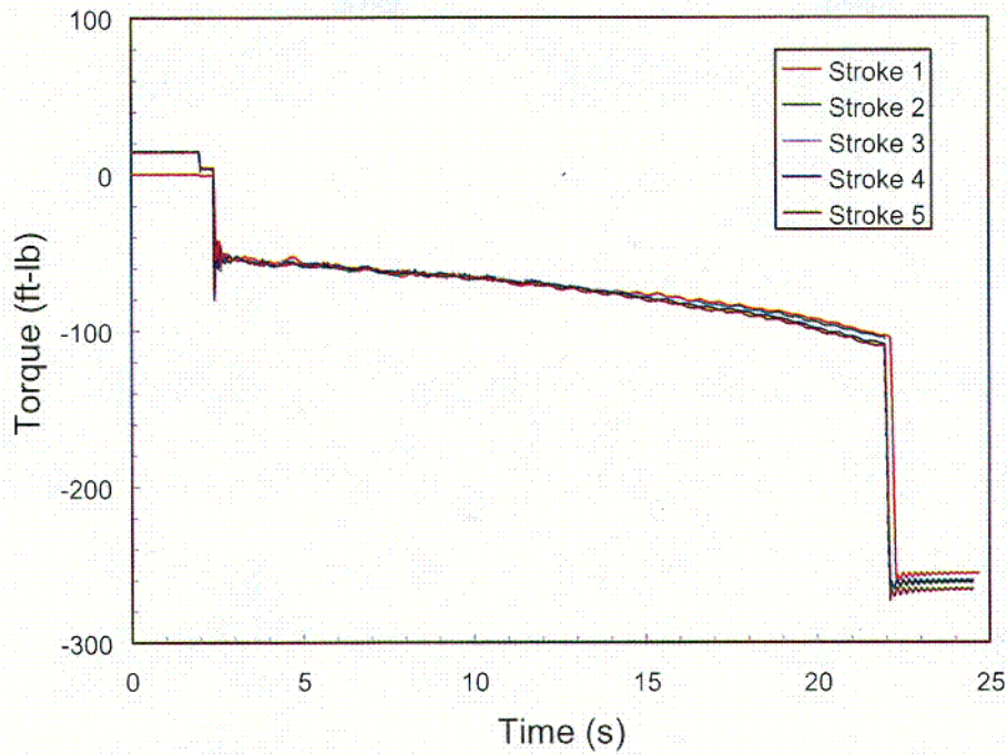
Figure 12. The five cold baseline tests for stem 2 with SRI show no variation in stem torque between strokes.
