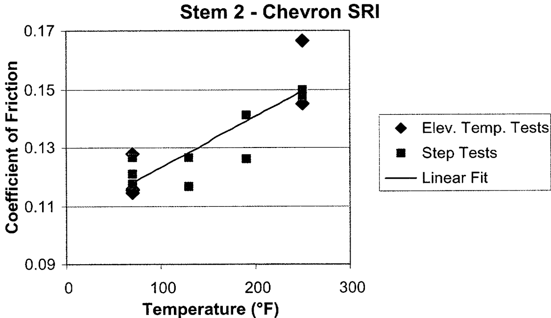
Figure 31. Typical increasing change in stem nut friction at elevated temperature.
