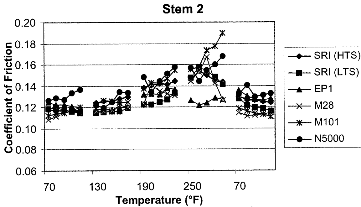
Figure 35. Stem nut coefficient of friction for each stroke of the multiple step tests with Stem 2.
