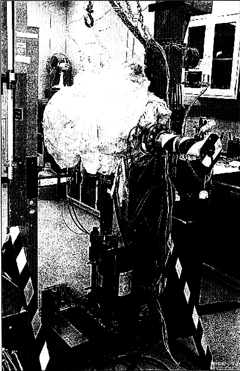
Figure 4. Actuators were heated to design basis temperatures.
