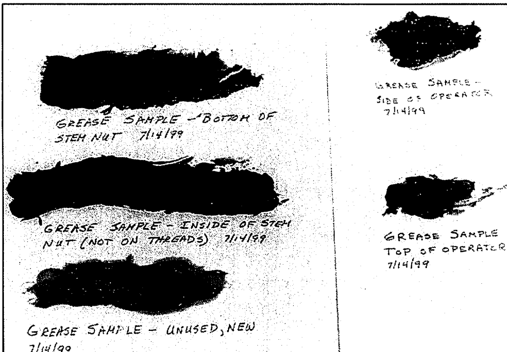
Figure 10. After testing, smear samples from the stem show that the EP1 changed from tan to brown and hardened. Smear samples from inside the sealed gearbox did not change significantly.
