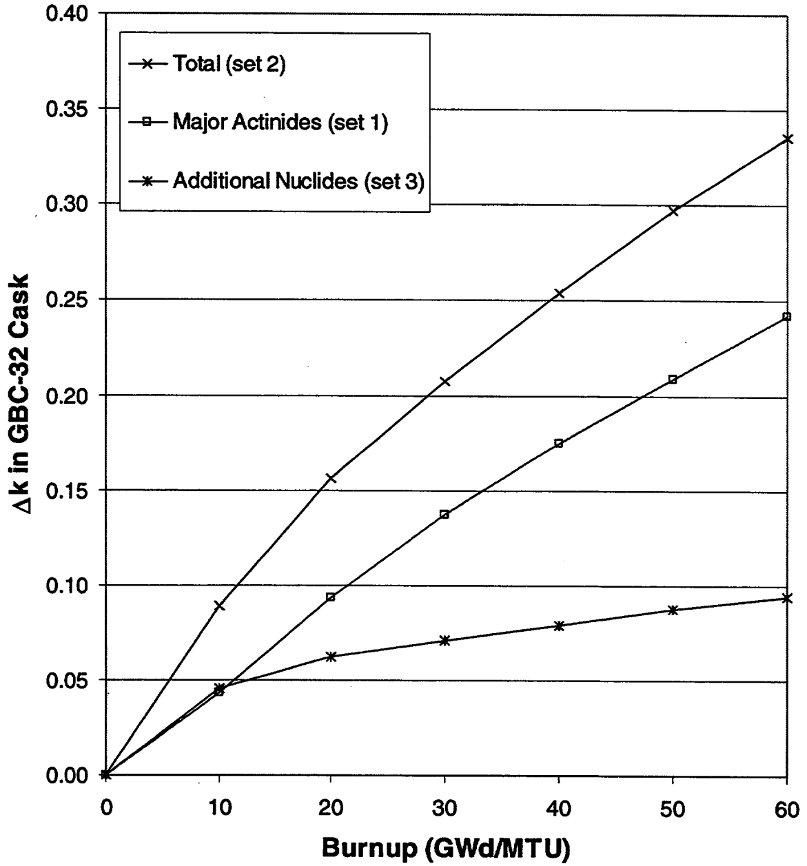
Figure D.8 \Delta k values (relative to fresh fuel) in the GBC-32 cask as a function of burnup using the different nuclide sets and 5-year cooling time for fuel of 5 wt % ^{235}\text{U} initial enrichment
