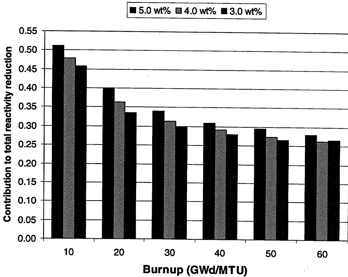
Figure D.16 Effect of initial enrichment on the contribution to total reduction in k_{eff} due to the additional nuclides (set 3) as a function of burnup for 5-year cooling time
