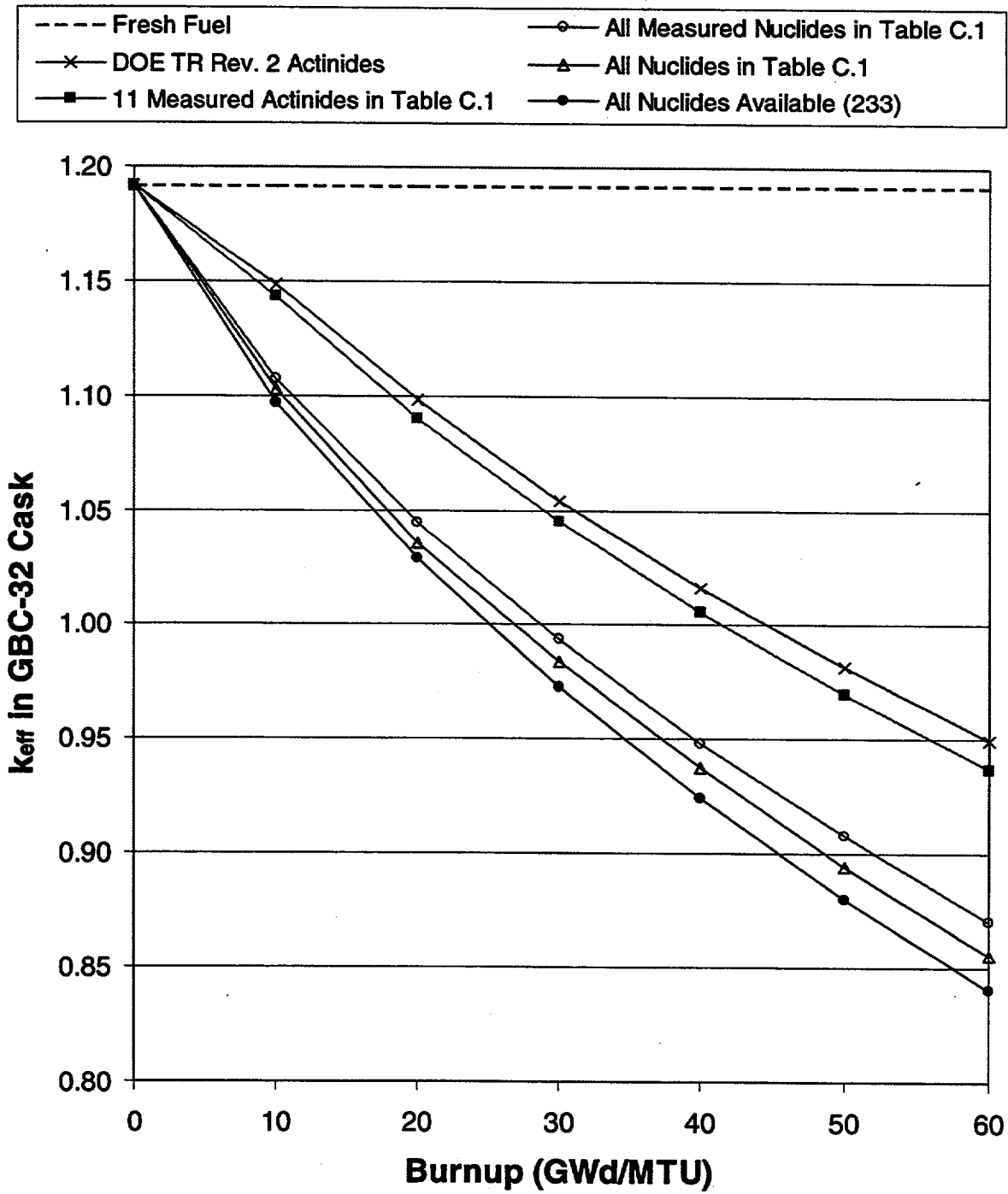
Figure C.7 Values of k_{eff} in the GBC-32 cask as a function of burnup using various nuclide sets and 5-year cooling time for fuel of 5 wt % ^{235}\text{U} initial enrichment
