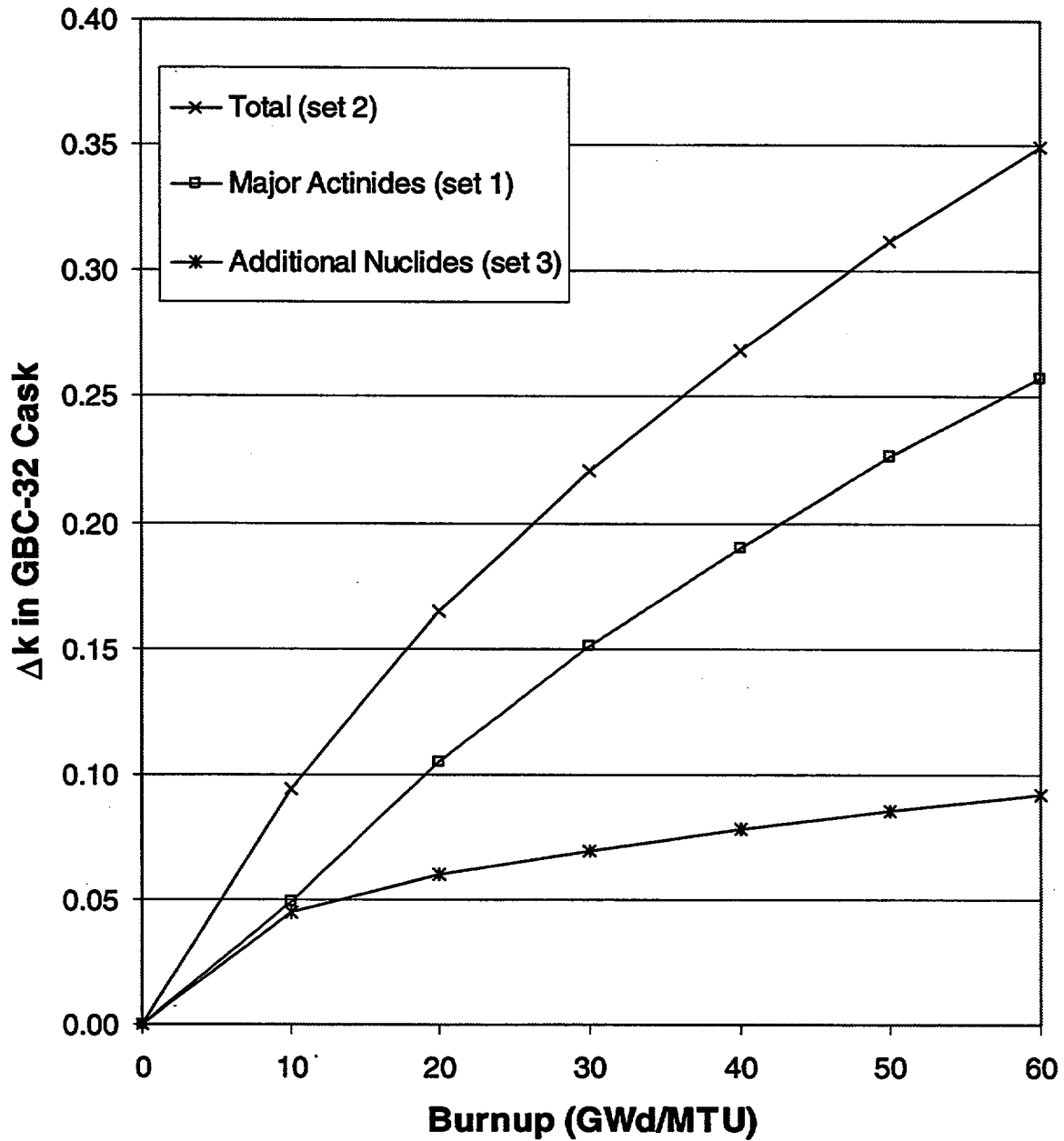
Figure D.7 \Delta k values (relative to fresh fuel) in the GBC-32 cask as a function of burnup using the different nuclide sets and 5-year cooling time for fuel of 4 wt % ^{235}\text{U} initial enrichment
