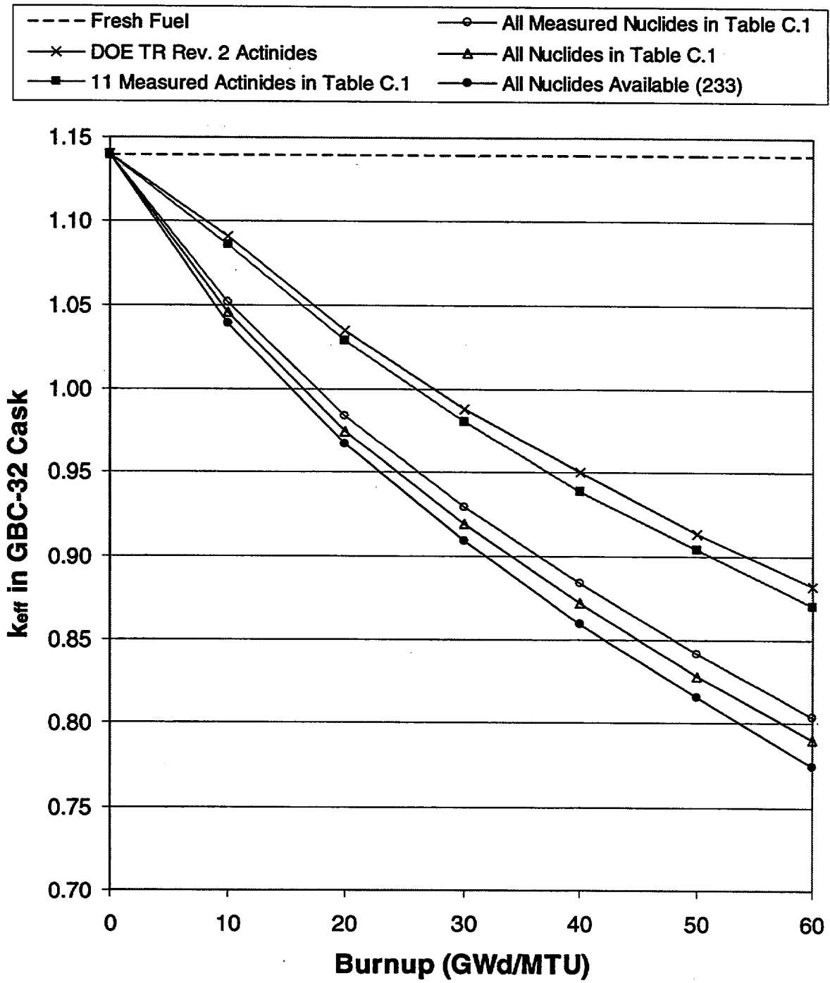
Figure C.5 Values of k_{eff} in the GBC-32 cask as a function of burnup using various nuclide sets and 5-year cooling time for fuel of 4 wt % ^{235}\text{U} initial enrichment
