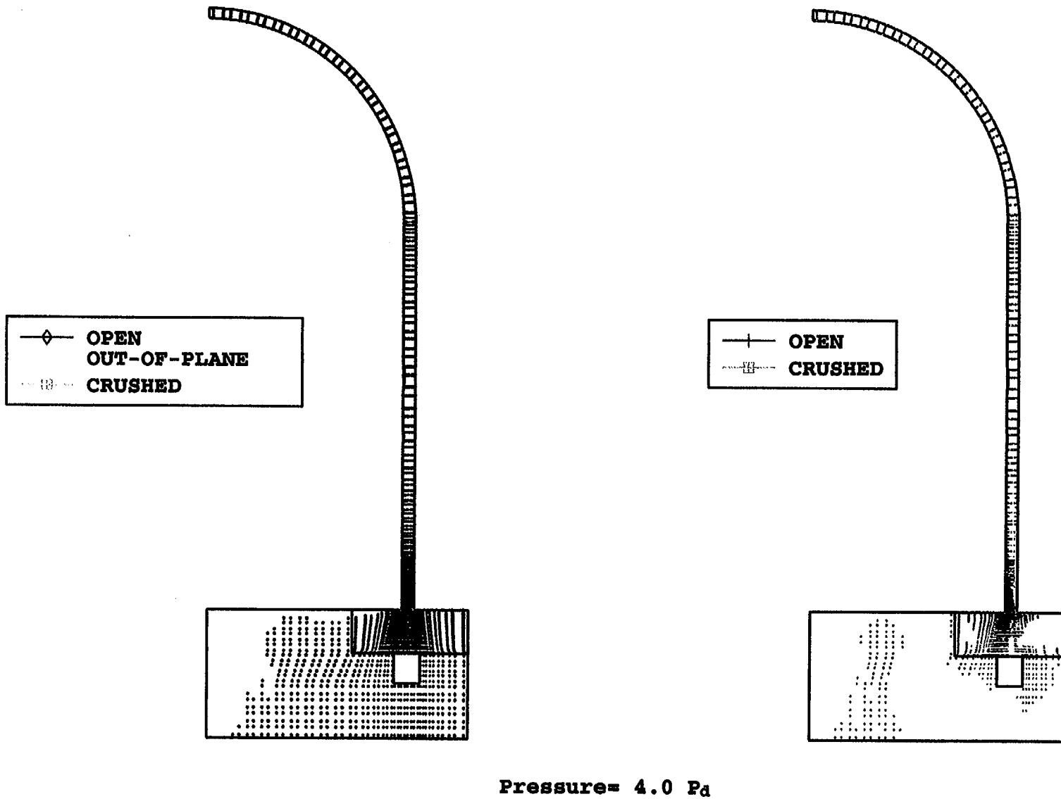
Figure 6-5a. Crack Patterns of Axisymmetric Model at 4.0 x P d Pressure
