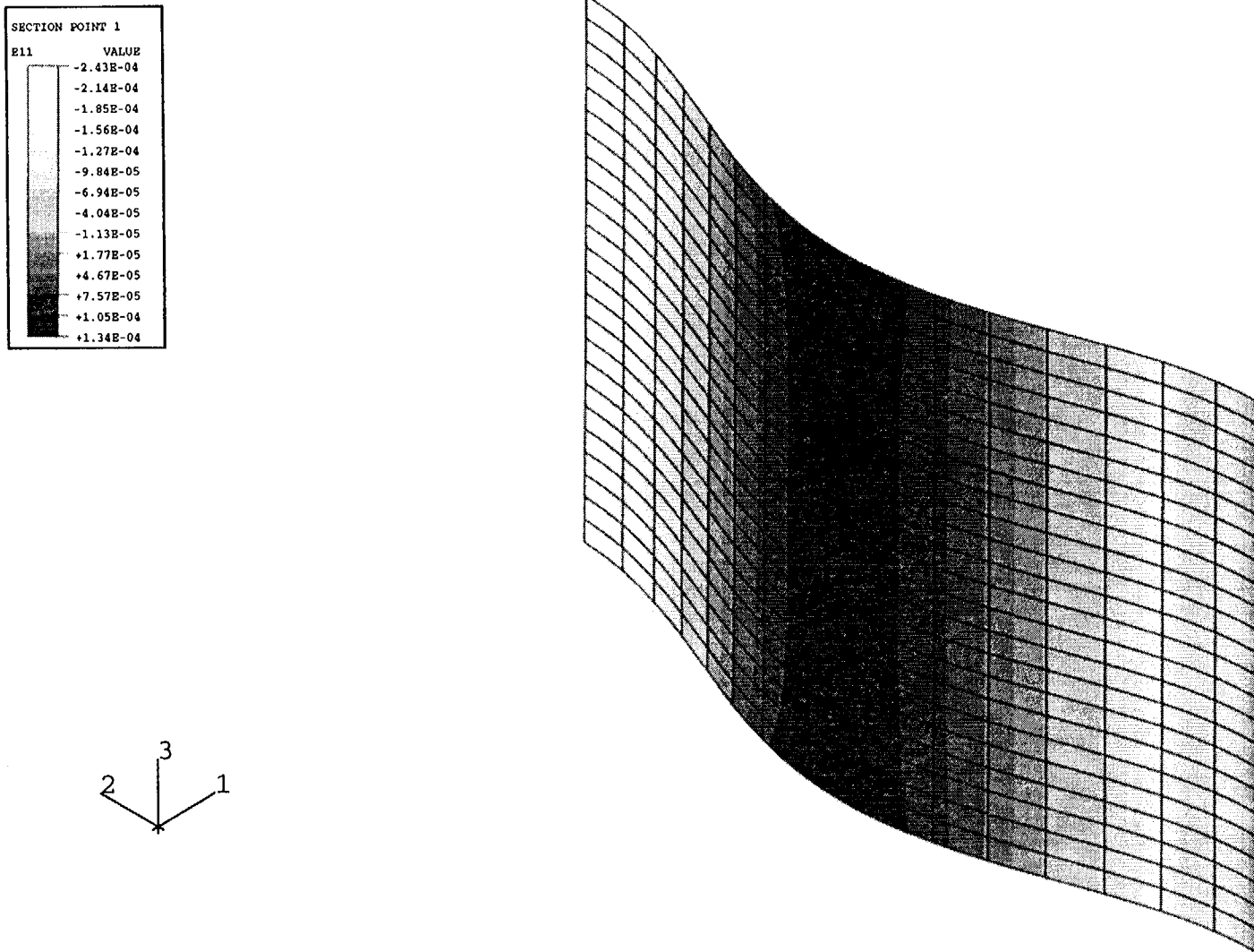
Figure 3-5. Hoop Strain Contours of Slight Imperfection Buckle Model at Prestress, Far-field Strain = -1.5E-4 (mag. factor =25.0) buckle.inp
