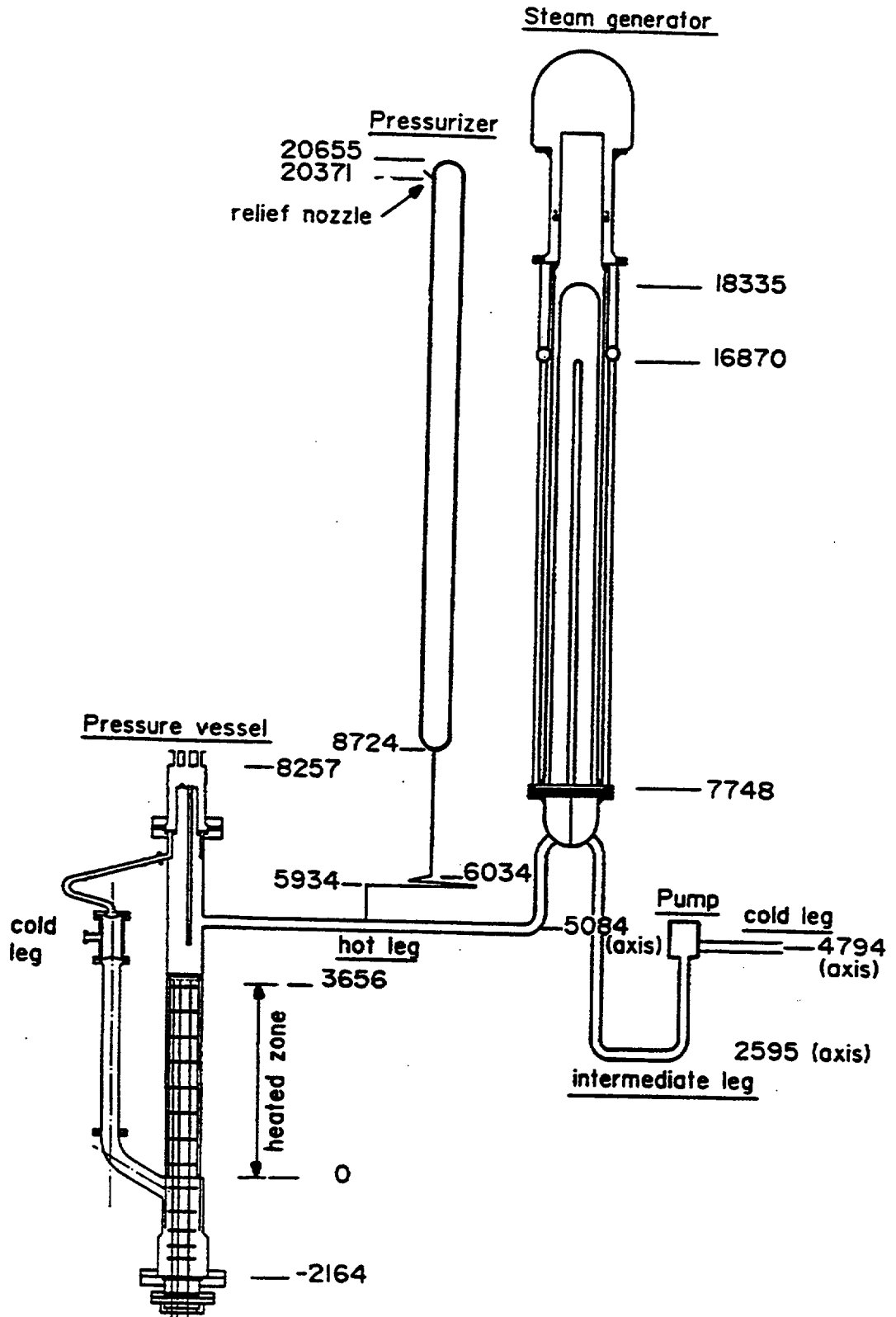
Figure 3 - Primary cooling system - elevations
