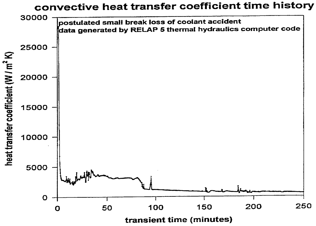
Figure 3.4 Averaged heat transfer coefficient between the fluid in the downcomer and the inside RPV wall (transient T1)
