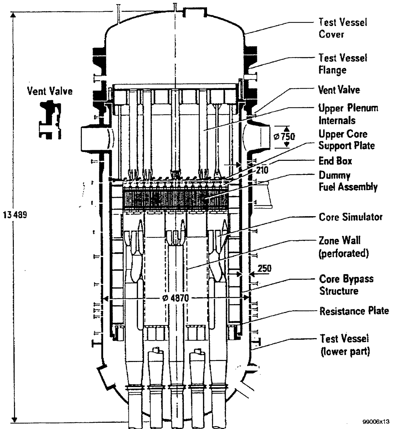
Figure 3.19 UPTF test vessel and its internals, to be used for the geometry of the RPV internals, not to be used concerning the RPV-wall thickness.
