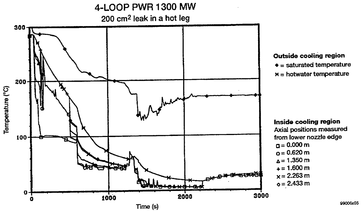
Figure 3.13 Fluid temperatures in the RPV downcomer near the inside RPV wall (transient T3)
