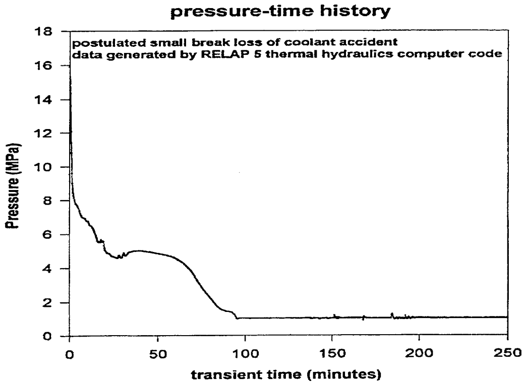
Figure 3.2 Pressure in the primary system (transient T1)
