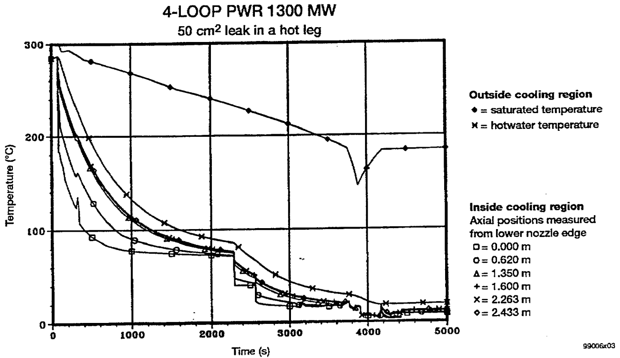
Figure 3.7 Fluid temperatures in the RPV downcomer near the inside RPV wall (transient T2)
