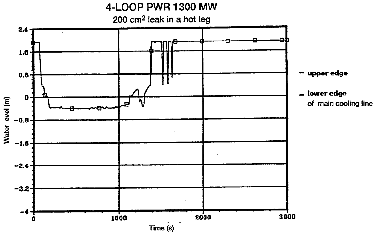
Figure 3.14 Water level in the RPV-downcomer (transient T3)
