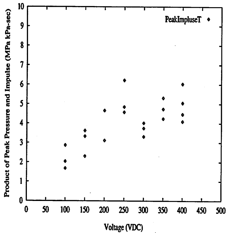
Figure 4.7: Product of the Peak Pressure and Impulse at the First Pressure Transducer with respect to Supplied Voltages
