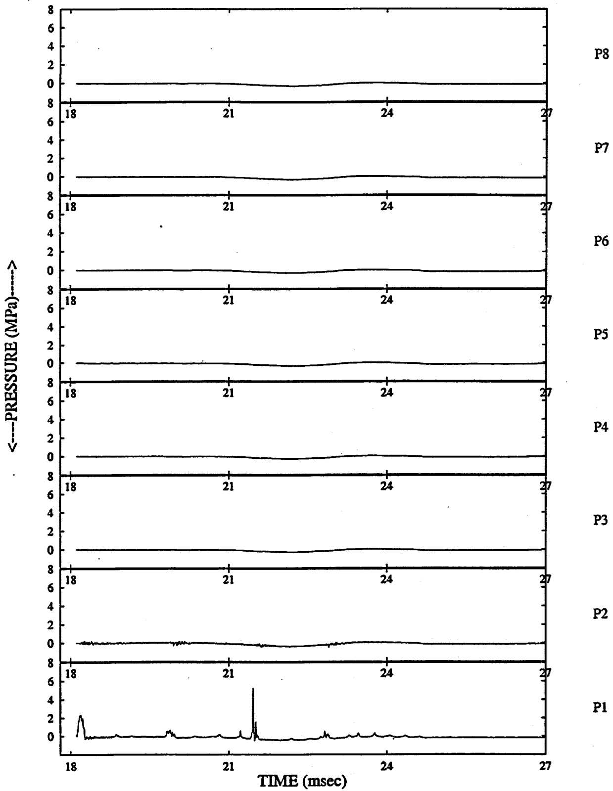
Figure 50: WFCI-K-03 transient pressure histories NUREG/CR-6623
