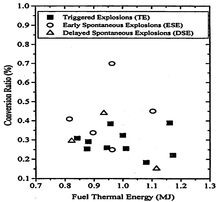
Figure 5.2: Conversion Ratios with respect to the Fuel Thermal Energies
