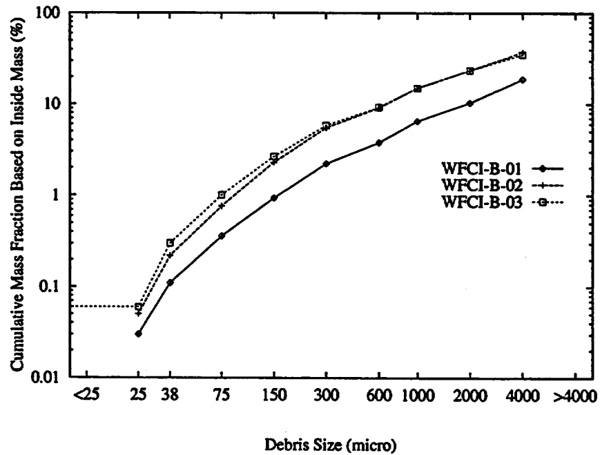
Figure A.2: Cumulative Debris Distribution for the WFCI-B Series
