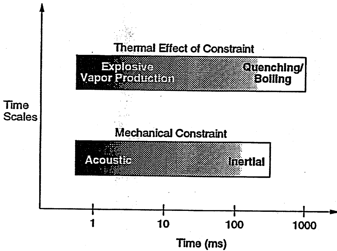
Figure 4.26: Time Scales with respect to the System Constraint
