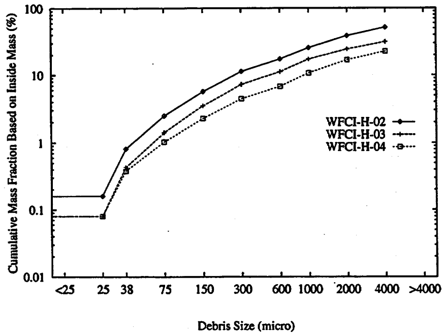
Figure A.6: Cumulative Debris Distribution for the WFCI-H Series
