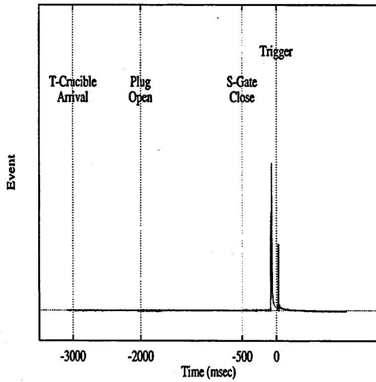
Figure 4.2: Sequential Events of the WFCI-A-01 Test
