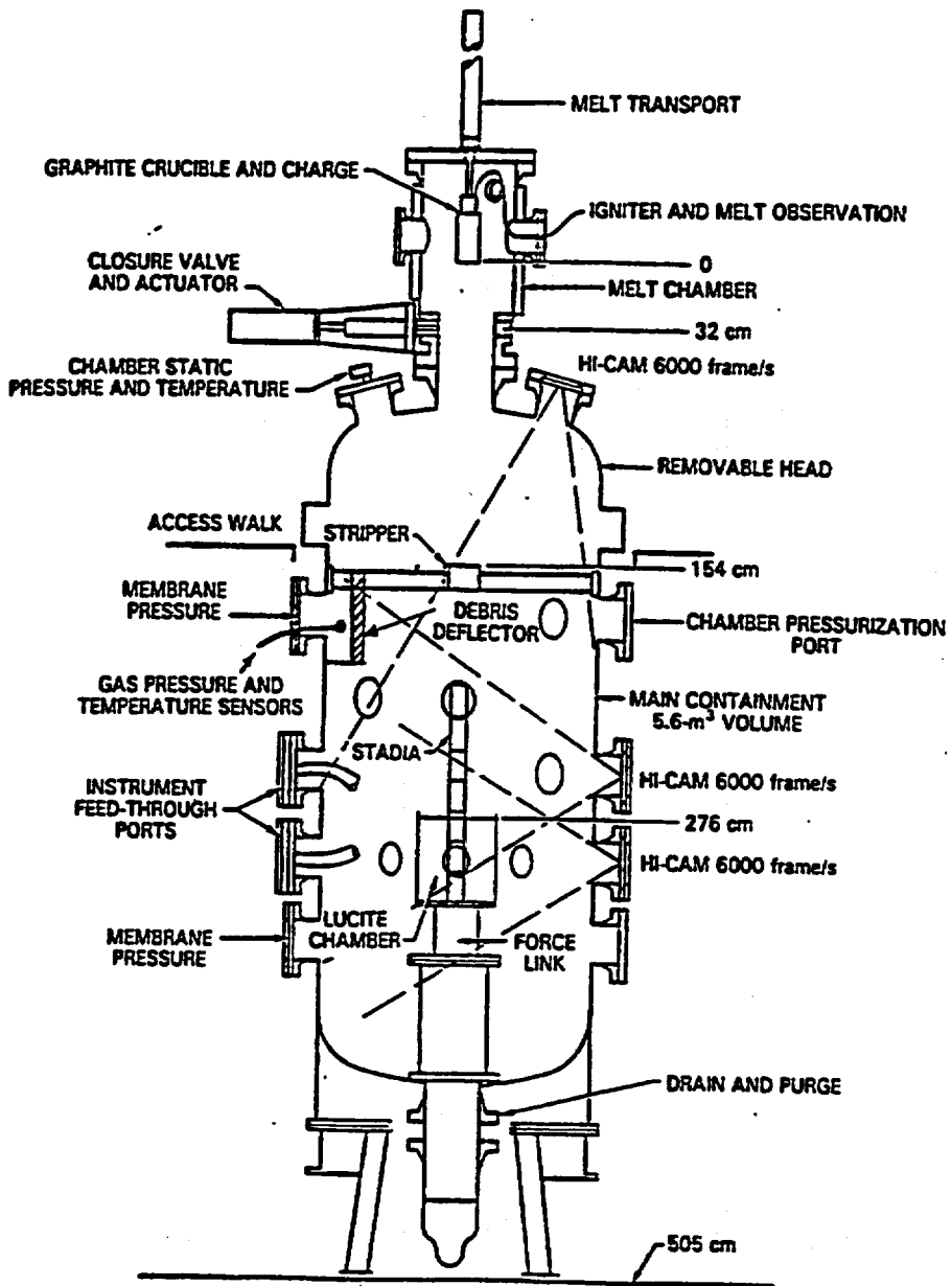
Figure 2.5: Schematic Illustration of the FITS Facility [40]
