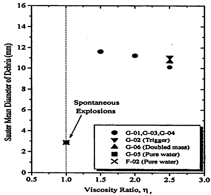
Figure 4.38: Sauter Mean Diameters of Collected Debris in the WFCI-G and F Series Tests
