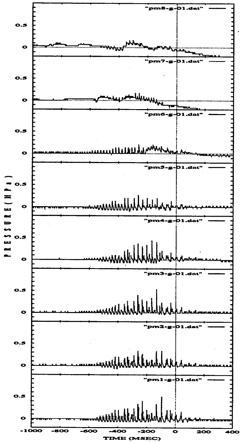
Figure 4.33: Typical Pressure Traces in Polymer Solution (WFCI-G-01)
