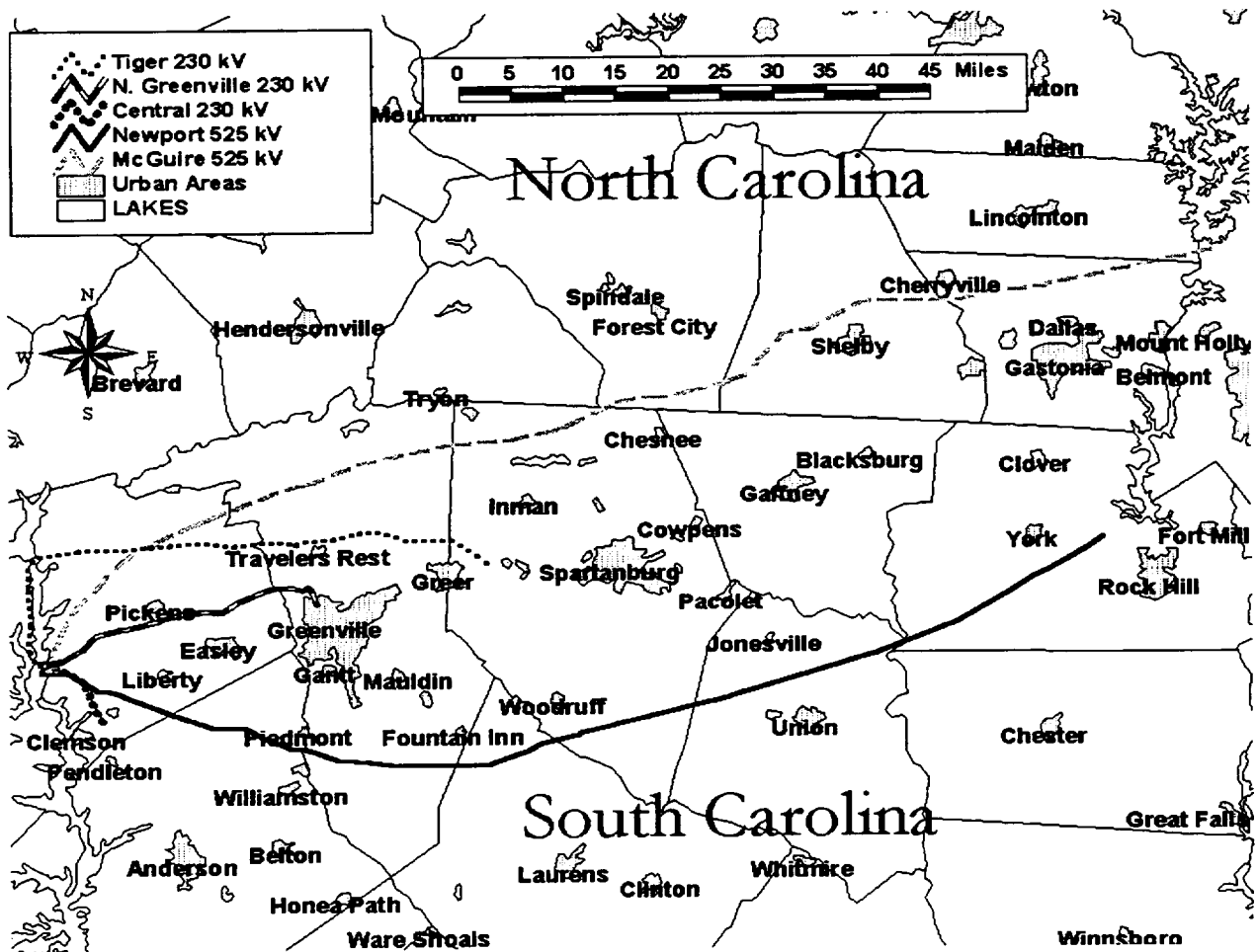
Figure 2-6. Transmission Lines Attributable to the Oconee Nuclear Station in the Final Environmental Statement (AEC 1972)
