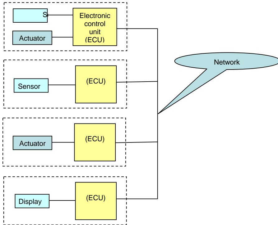
Fig. 2.5 OSEKtime-based system architecture.
