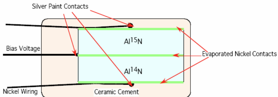
Fig. 3.4. Fabrication concept of the solid-state fuel monitor.
