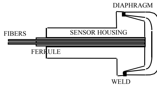
Fig. 3.13. Sensor head design.
