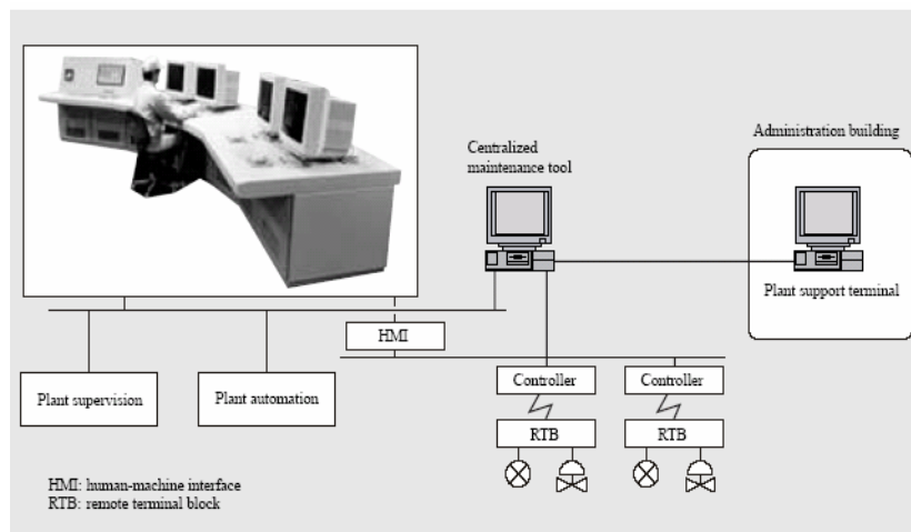
Fig. 2.11. General-purpose and open network technologies can be used to configure a compact, human-friendly supervisory control system.
