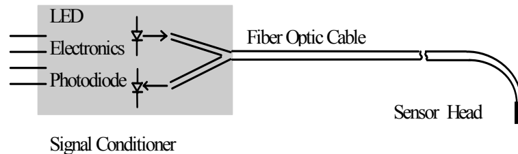
Fig. 3.14. Sensor block diagram.
