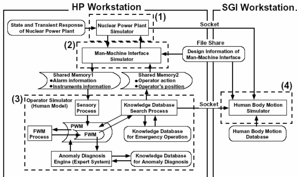
Fig. 2.13. System architecture of a virtual collaborator.
