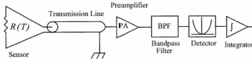
Fig. 3.8. Basic components of a Johnson noise thermometer.
