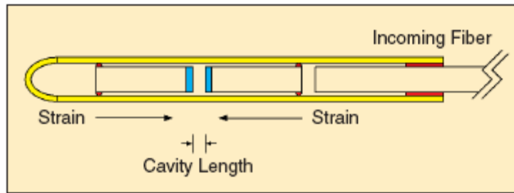
Fig. 3.15. Fabry-Perot cavity.
