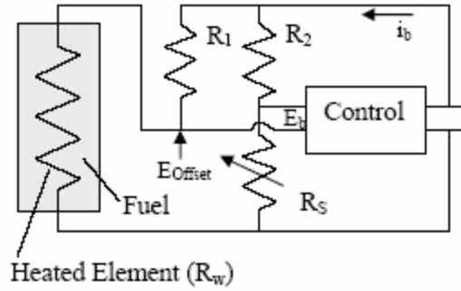
Fig. 3.5. Constant-temperature power sensor Wheatstone bridge control circuit.
