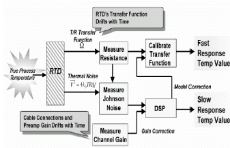
Fig. 3.9. Schematic for automatic recalibration of RTD from Johnson noise measurement [Source: Kisner 2005].
