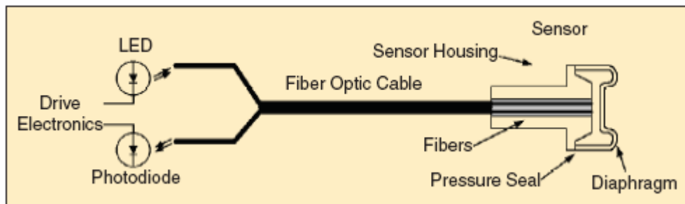
Fig. 3.12. Fiber-optic pressure transducer.
