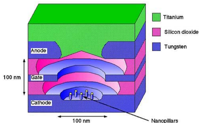
Fig. 2.3. Schematic of a nanotriode ( http://www.aip.org/png/html/nanotriodes.html ).
