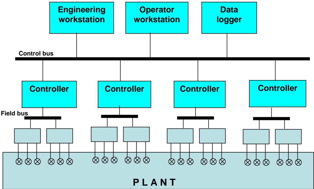
Fig. 2.8. Generic decentralized control system.
