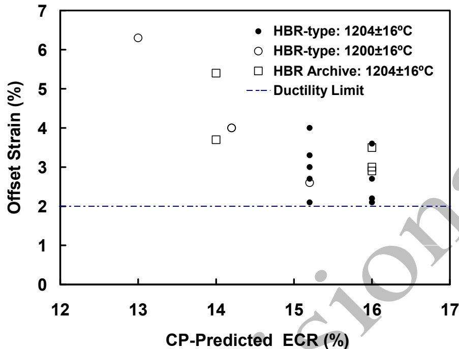
Figure 3. Offset strains determined for as-fabricated HBR-type 15×15 Zry-4 oxidized at \approx 1,200 °C and quenched at 800 °C (see Figure 2 for corresponding permanent strains).
