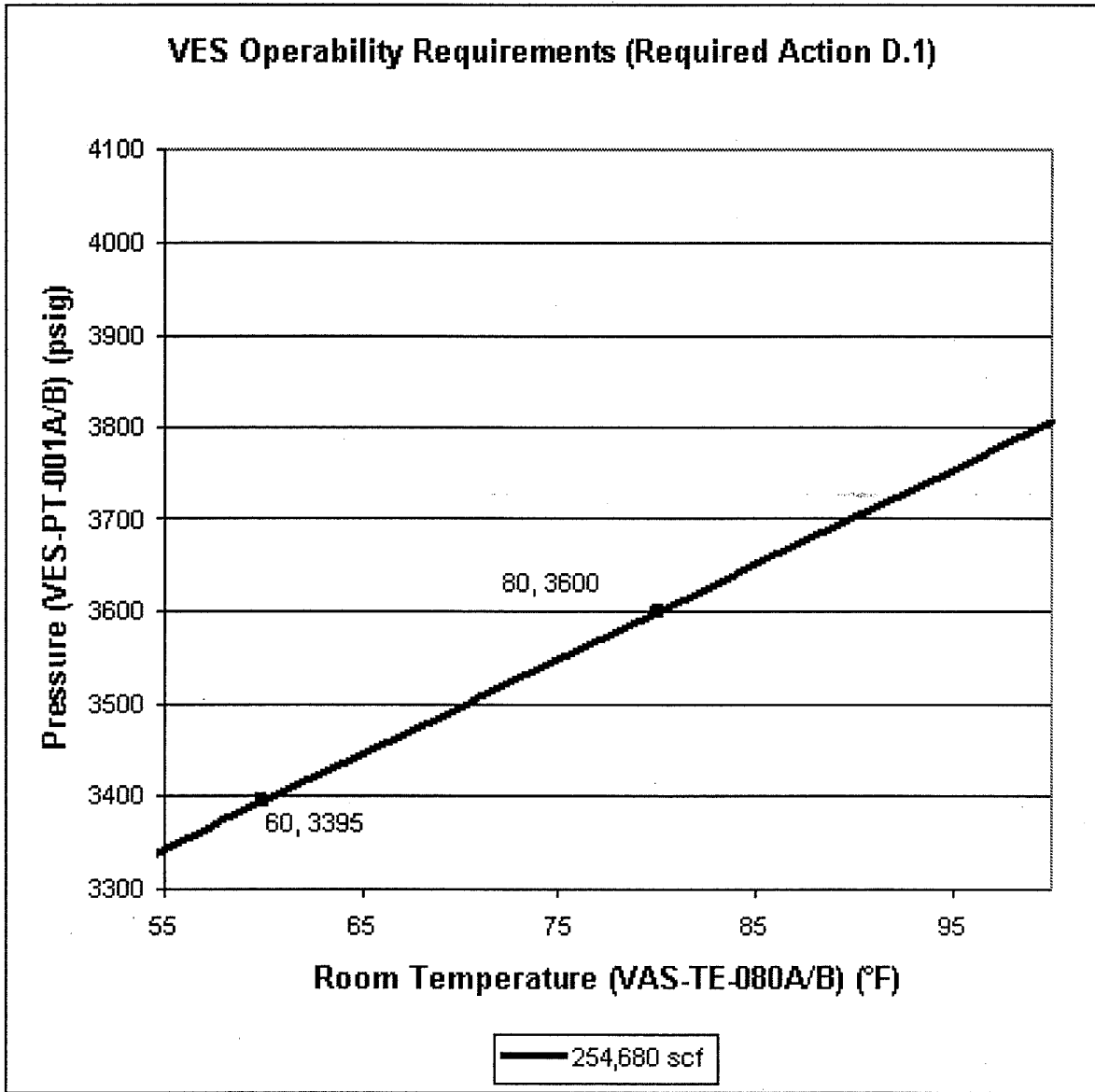
Figure B 3.7.6-2 Compressed Air Storage Tanks Minimum Volume – One Bank of VES Air Tanks (8 Tanks) Inoperable
