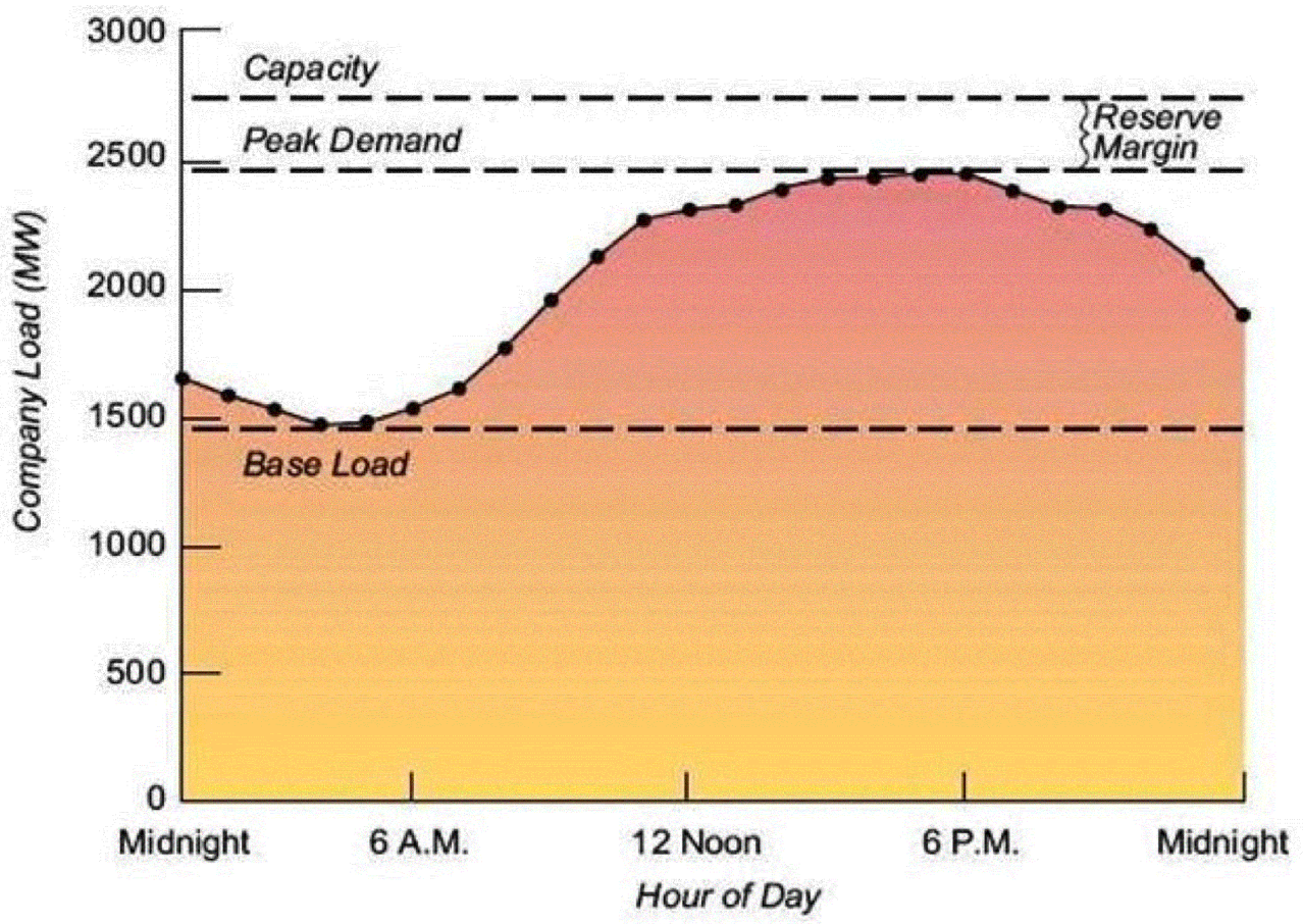
Figure 8.2-1—{Summer Power Demand}
